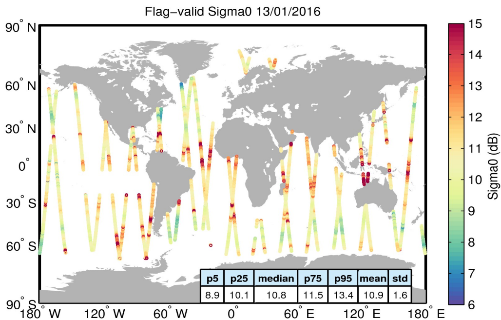
Figure 23. Geographical distribution of flag-valid sigma0 data over oceans and lakes for 13/01/2016. The statistical values shown in the table refer to the sigma0 in dB and are calculated over all measurements shown in the figure.
