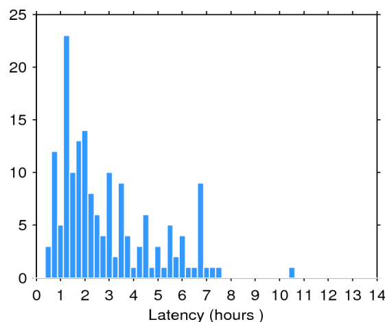
Figure 2. Histogram of the data latency for 13/01/2016. The y-axis denotes the number of files that are made available with a delay of x-hours with respect to the mean time of the records stored in the file.
