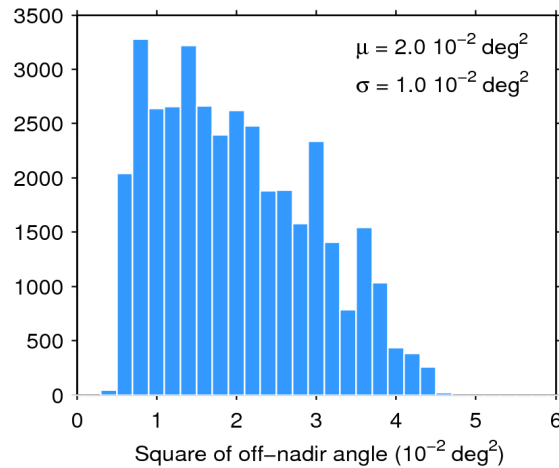
Figure 39. Histogram of flag-valid mispointing over oceans and lakes for 13/01/2016. The mean ( \mu ) and standard deviation ( \sigma ) are also shown. Note that values larger than 6 \cdot 10^{-2} \text{ deg}^2 are excluded from the histogram for the sake of readability but not from the computation of \mu and \sigma .
