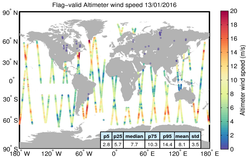
Figure 31. Geographical distribution of flag-valid wind data over oceans and lakes for 13/01/2016. The statistical values shown in the table refer to the wind in m/s and are calculated over all measurements shown in the figure.
