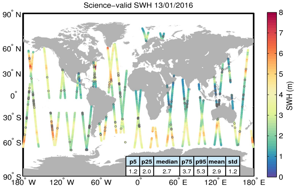
Figure 19. Geographical distribution of science-valid SWH data over oceans and lakes for 13/01/2016. The statistical values shown in the table refer to the SWH in m and are calculated over all measurements shown in the figure. Gray circles denote records that have been rejected based on the editing criteria described in Table 3.
