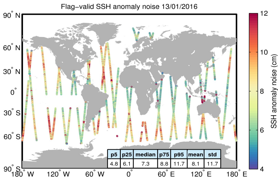
Figure 8. Geographical distribution of flag-valid 20-Hz SSH anomaly measurement noise over oceans and lakes for 13/01/2016. The statistical values shown in the table refer to the SSH anomaly noise and are calculated over all measurements shown in the figure.
