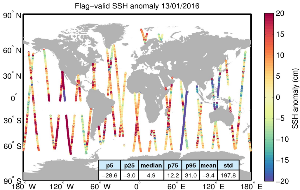
Figure 5. Geographical distribution of flag-valid 1-Hz SSH anomaly data over oceans and lakes for 13/01/2016. The statistical values shown in the table refer to the SSH anomaly in cm and are calculated over all measurements shown in the figure.
