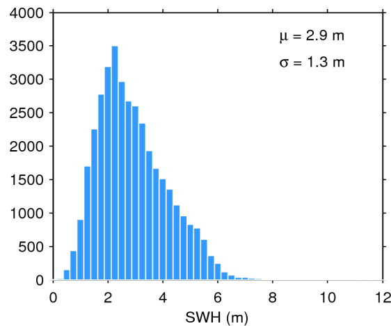
Figure 17. Histogram of flag-valid SWH over oceans and lakes for 13/01/2016. The mean ( \mu ) and standard deviation ( \sigma ) are also shown. Note that values larger than 12 m are excluded from the histogram for the sake of readability but not from the computation of \mu and \sigma .
