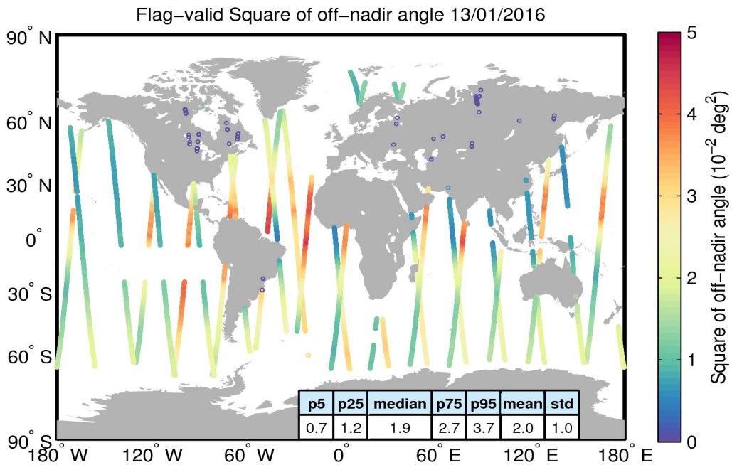
Figure 37. Geographical distribution of flag-valid mispointing data over oceans and lakes for 13/01/2016. The statistical values shown in the table refer to the mispointing in 10^{-2} \text{deg}^2 and are calculated over all measurements shown in the figure.
