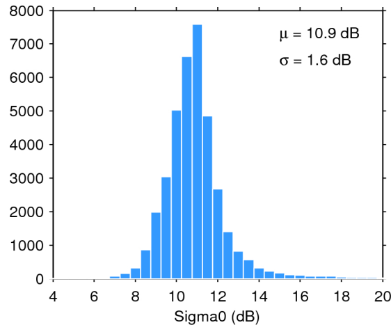
Figure 25. Histogram of flag-valid sigma0 over oceans and lakes for 13/01/2016. The mean ( \mu ) and standard deviation ( \sigma ) are also shown. Note that values outside [4 20] dB are excluded from the histogram for the sake of readability but not from the computation of \mu and \sigma .
