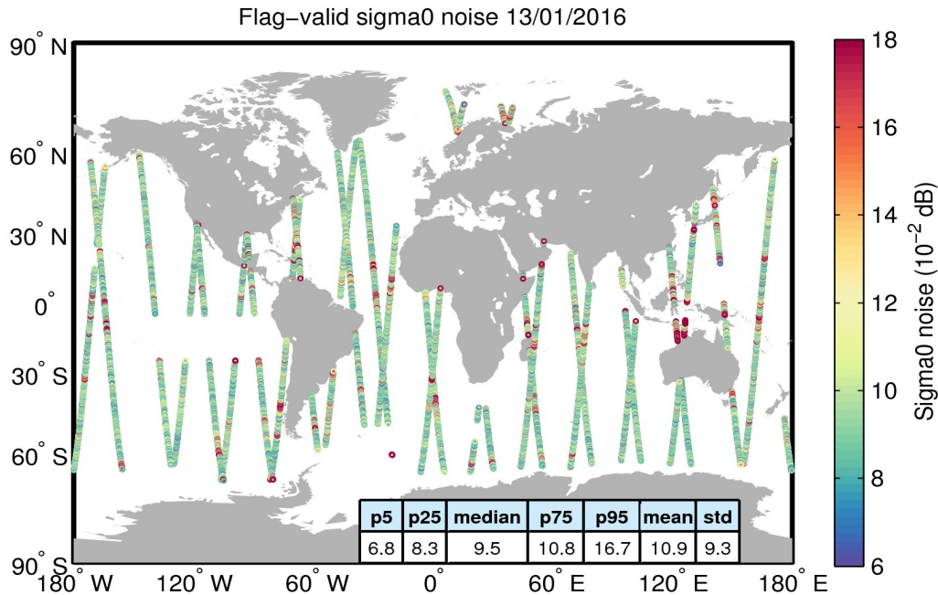
Figure 26. Geographical distribution of flag-valid 20-Hz sigma0 measurement noise over oceans and lakes for 13/01/2016. The statistical values shown in the table refer to the sigma0 noise and are calculated over all measurements shown in the figure.
