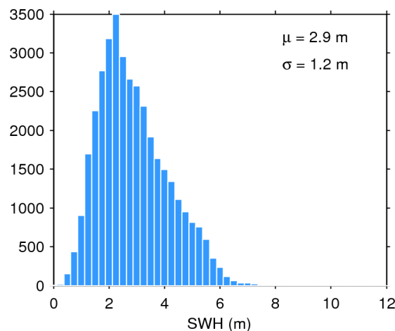
Figure 20. Histogram of science-valid SWH over oceans and lakes for 13/01/2016. The mean ( \mu ) and standard deviation ( \sigma ) are also shown. Note that values larger than 12 m are excluded from the histogram for the sake of readability but not from the computation of \mu and \sigma .
