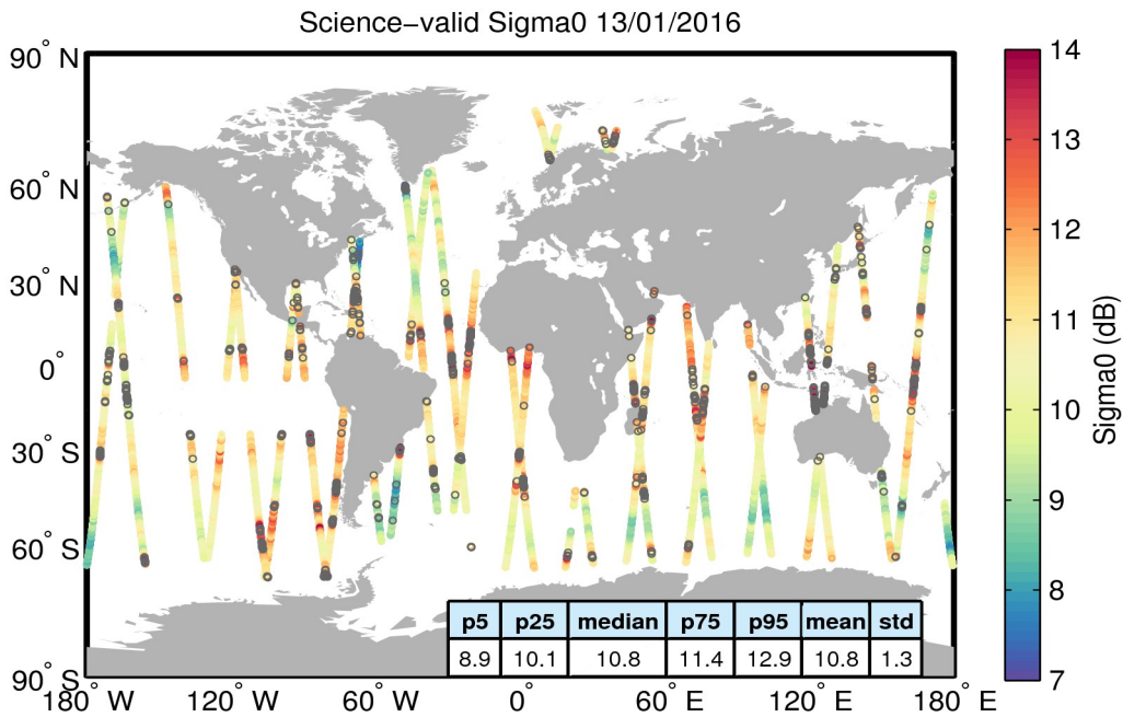
Figure 27. Geographical distribution of science-valid sigma0 data over oceans and lakes for 13/01/2016. The statistical values shown in the table refer to the sigma0 in dB and are calculated over all measurements shown in the figure. Gray circles denote records that have been rejected based on the editing criteria described in Table 4.
