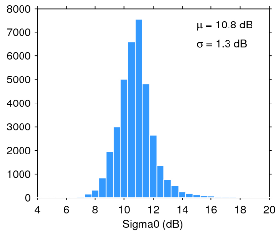
Figure 28. Histogram of science-valid sigma0 over oceans and lakes for 13/01/2016. The mean ( \mu ) and standard deviation ( \sigma ) are also shown. Note that values outside [4 20] dB are excluded from the histogram for the sake of readability but not from the computation of \mu and \sigma .
