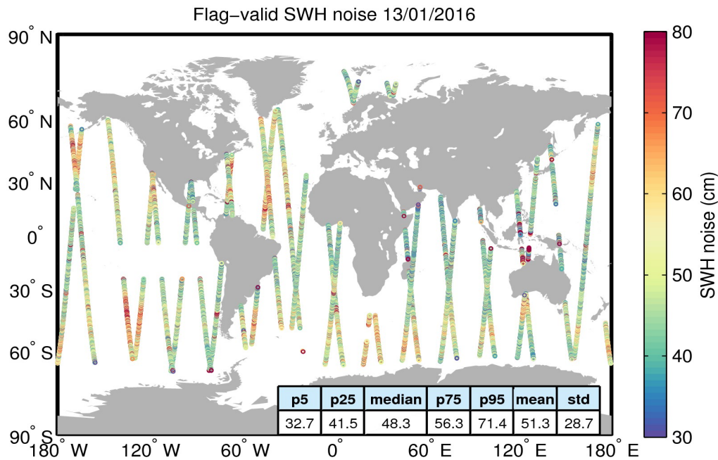
Figure 18. Geographical distribution of flag-valid 20-Hz SWH measurement noise over oceans and lakes for 13/01/2016. The statistical values shown in the table refer to the SWH noise and are calculated over all measurements shown in the figure.
