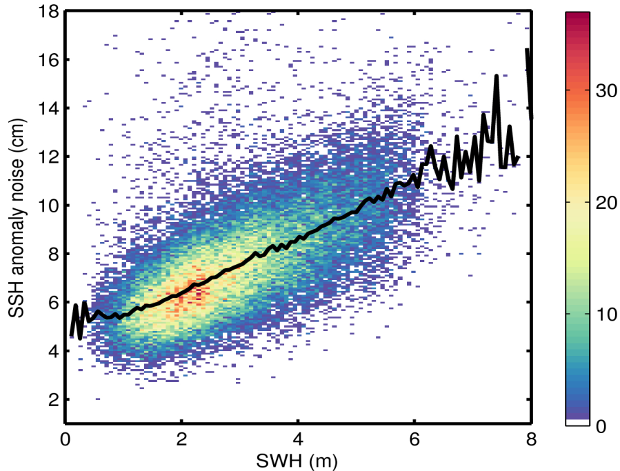
Figure 9. 2D histogram showing flag-valid SSH anomaly noise as a function of SWH for 13/01/2016. The black line denotes the median SSH anomaly noise as a function of SWH.
