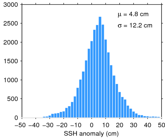
Figure 11. Histogram of science-valid SSH anomaly over oceans and lakes for 13/01/2016. The mean ( \mu ) and standard deviation ( \sigma ) are also shown. Note that values outside [-50 50] cm are excluded from the histogram for the sake of readability but not from the computation of \mu and \sigma .
