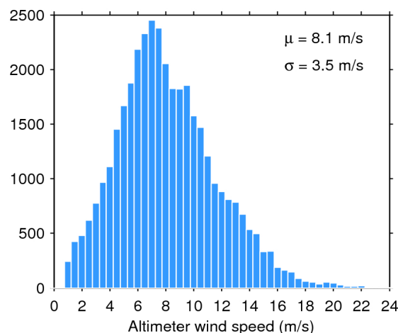
Figure 35. Histogram of science-valid wind over oceans and lakes for 13/01/2016. The mean ( \mu ) and standard deviation ( \sigma ) are also shown. Note that values larger than 24 m/s are excluded from the histogram for the sake of readability but not from the computation of \mu and \sigma .
