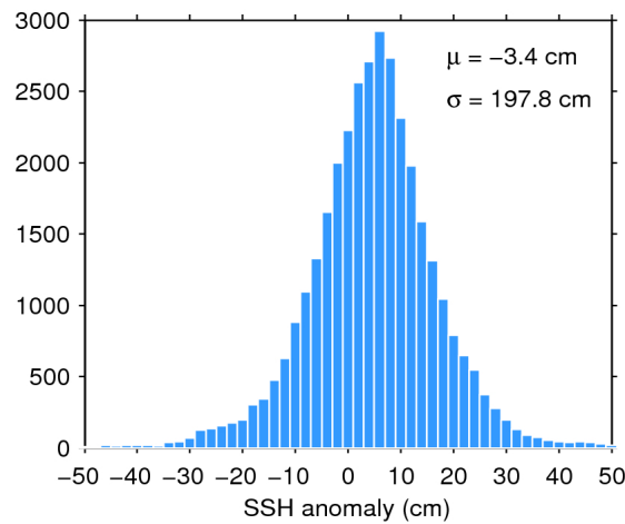
Figure 7. Histogram of flag-valid SSH anomaly over oceans and lakes for 13/01/2016. The mean ( \mu ) and standard deviation ( \sigma ) are also shown. Note that values outside [-50 50] cm are excluded from the histogram for the sake of readability but not from the computation of \mu and \sigma .
