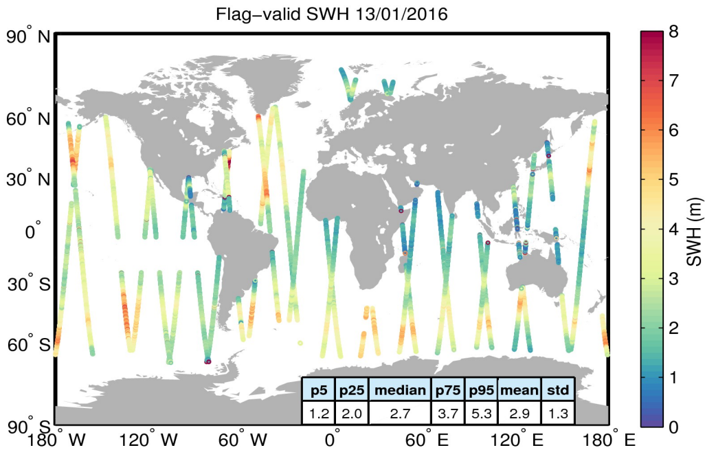
Figure 15. Geographical distribution of flag-valid SWH data over oceans and lakes for 13/01/2016. The statistical values shown in the table refer to the SWH in m and are calculated over all measurements shown in the figure.
