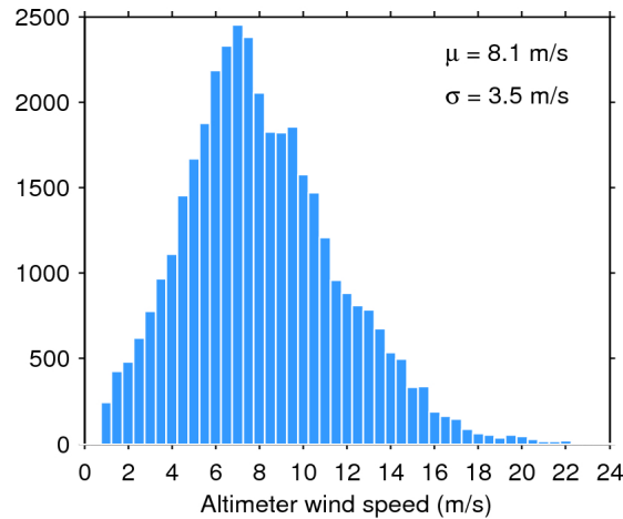
Figure 33. Histogram of flag-valid wind over oceans and lakes for 13/01/2016. The mean ( \mu ) and standard deviation ( \sigma ) are also shown. Note that values larger than 24 m/s are excluded from the histogram for the sake of readability but not from the computation of \mu and \sigma .
