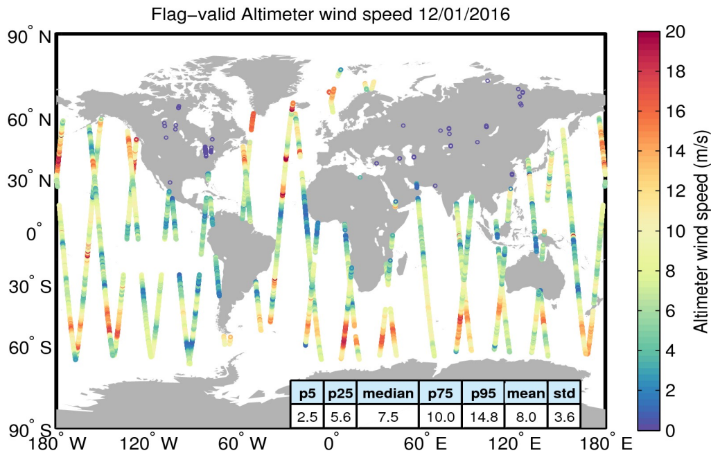
Figure 31. Geographical distribution of flag-valid wind data over oceans and lakes for 12/01/2016. The statistical values shown in the table refer to the wind in m/s and are calculated over all measurements shown in the figure.
