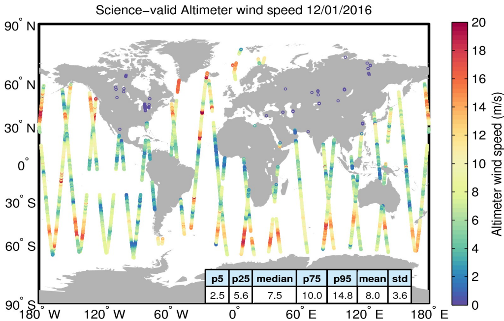
Figure 34. Geographical distribution of science-valid wind data over oceans and lakes for 12/01/2016. The statistical values shown in the table refer to the wind in m/s and are calculated over all measurements shown in the figure. Gray circles denote records that have been rejected based on the editing criteria described in Table 5.
