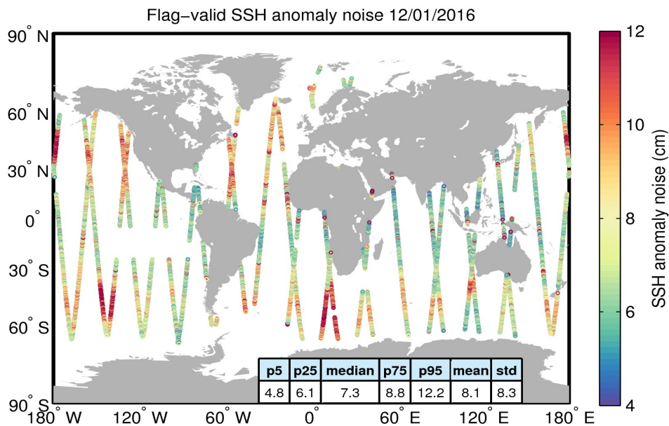
Figure 8. Geographical distribution of flag-valid 20-Hz SSH anomaly measurement noise over oceans and lakes for 12/01/2016. The statistical values shown in the table refer to the SSH anomaly noise and are calculated over all measurements shown in the figure.
