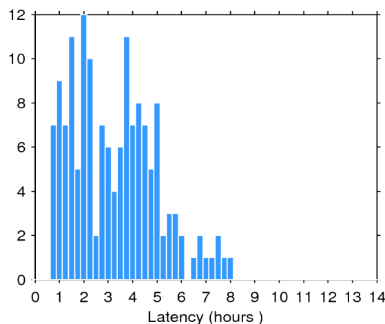
Figure 2. Histogram of the data latency for 12/01/2016. The y-axis denotes the number of files that are made available with a delay of x-hours with respect to the mean time of the records stored in the file.
