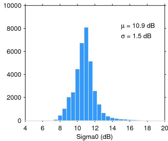
Figure 28. Histogram of science-valid sigma0 over oceans and lakes for 12/01/2016. The mean ( \mu ) and standard deviation ( \sigma ) are also shown. Note that values outside [4 20] dB are excluded from the histogram for the sake of readability but not from the computation of \mu and \sigma .
