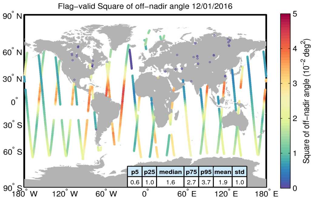
Figure 37. Geographical distribution of flag-valid mispointing data over oceans and lakes for 12/01/2016. The statistical values shown in the table refer to the mispointing in 10^{-2} deg 2 and are calculated over all measurements shown in the figure.
