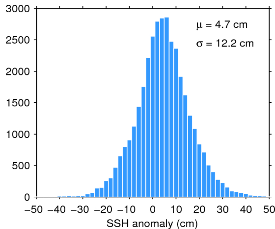
Figure 11. Histogram of science-valid SSH anomaly over oceans and lakes for 12/01/2016. The mean ( \mu ) and standard deviation ( \sigma ) are also shown. Note that values outside [-50 50] cm are excluded from the histogram for the sake of readability but not from the computation of \mu and \sigma .
