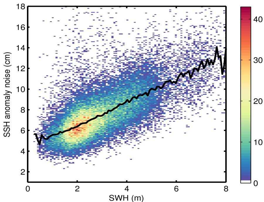
Figure 9. 2D histogram showing flag-valid SSH anomaly noise as a function of SWH for 12/01/2016. The black line denotes the median SSH anomaly noise as a function of SWH.
