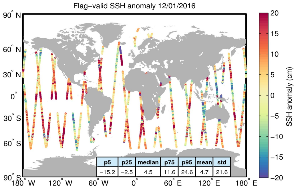
Figure 5. Geographical distribution of flag-valid 1-Hz SSH anomaly data over oceans and lakes for 12/01/2016. The statistical values shown in the table refer to the SSH anomaly in cm and are calculated over all measurements shown in the figure.
