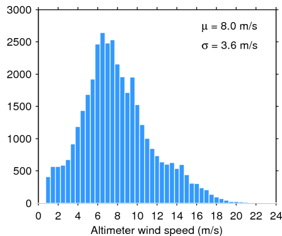
Figure 35. Histogram of science-valid wind over oceans and lakes for 12/01/2016. The mean ( \mu ) and standard deviation ( \sigma ) are also shown. Note that values larger than 24 m/s are excluded from the histogram for the sake of readability but not from the computation of \mu and \sigma .
