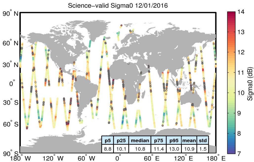
Figure 27. Geographical distribution of science-valid sigma0 data over oceans and lakes for 12/01/2016. The statistical values shown in the table refer to the sigma0 in dB and are calculated over all measurements shown in the figure. Gray circles denote records that have been rejected based on the editing criteria described in Table 4.
