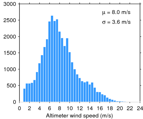
Figure 33. Histogram of flag-valid wind over oceans and lakes for 12/01/2016. The mean ( \mu ) and standard deviation ( \sigma ) are also shown. Note that values larger than 24 m/s are excluded from the histogram for the sake of readability but not from the computation of \mu and \sigma .
