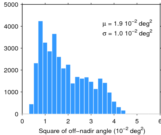
Figure 39. Histogram of flag-valid mispointing over oceans and lakes for 12/01/2016. The mean ( \mu ) and standard deviation ( \sigma ) are also shown. Note that values larger than 6 \cdot 10^{-2} \text{ deg}^2 are excluded from the histogram for the sake of readability but not from the computation of \mu and \sigma .
