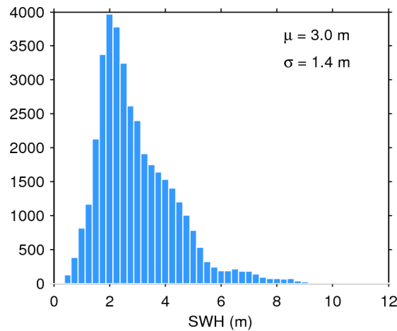
Figure 17. Histogram of flag-valid SWH over oceans and lakes for 12/01/2016. The mean ( \mu ) and standard deviation ( \sigma ) are also shown. Note that values larger than 12 m are excluded from the histogram for the sake of readability but not from the computation of \mu and \sigma .
