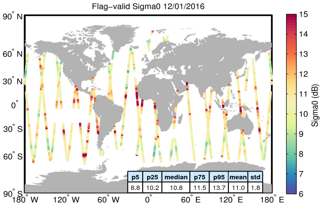
Figure 23. Geographical distribution of flag-valid sigma0 data over oceans and lakes for 12/01/2016. The statistical values shown in the table refer to the sigma0 in dB and are calculated over all measurements shown in the figure.
