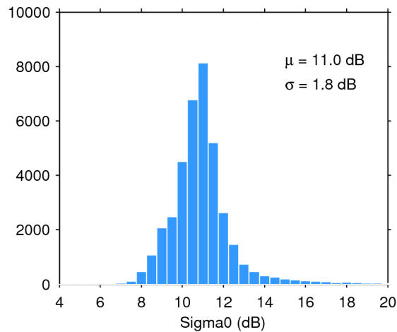
Figure 25. Histogram of flag-valid sigma0 over oceans and lakes for 12/01/2016. The mean ( \mu ) and standard deviation ( \sigma ) are also shown. Note that values outside [4 20] dB are excluded from the histogram for the sake of readability but not from the computation of \mu and \sigma .
