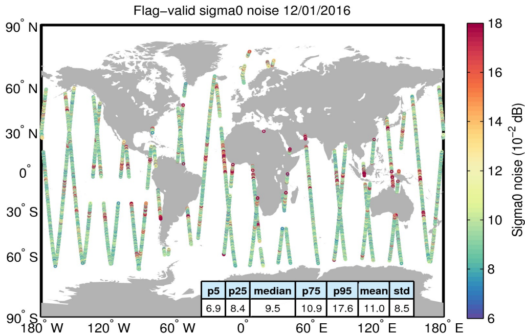
Figure 26. Geographical distribution of flag-valid 20-Hz sigma0 measurement noise over oceans and lakes for 12/01/2016. The statistical values shown in the table refer to the sigma0 noise and are calculated over all measurements shown in the figure.
