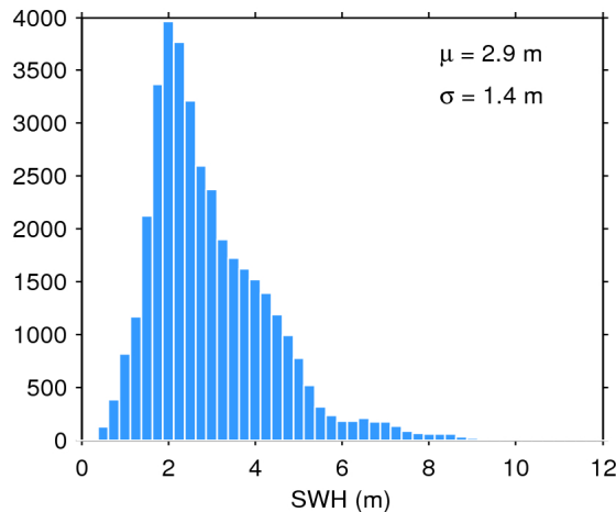
Figure 20. Histogram of science-valid SWH over oceans and lakes for 12/01/2016. The mean ( \mu ) and standard deviation ( \sigma ) are also shown. Note that values larger than 12 m are excluded from the histogram for the sake of readability but not from the computation of \mu and \sigma .
