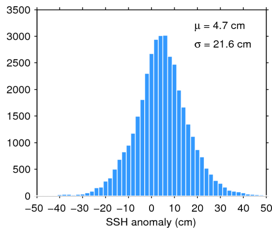
Figure 7. Histogram of flag-valid SSH anomaly over oceans and lakes for 12/01/2016. The mean ( \mu ) and standard deviation ( \sigma ) are also shown. Note that values outside [-50 50] cm are excluded from the histogram for the sake of readability but not from the computation of \mu and \sigma .
