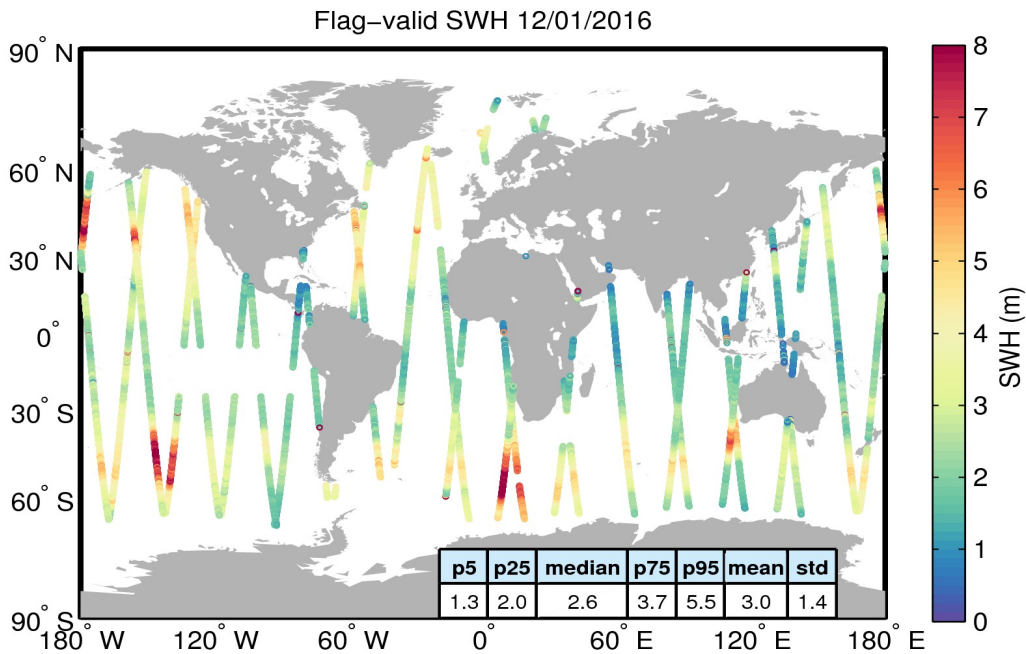
Figure 15. Geographical distribution of flag-valid SWH data over oceans and lakes for 12/01/2016. The statistical values shown in the table refer to the SWH in m and are calculated over all measurements shown in the figure.
