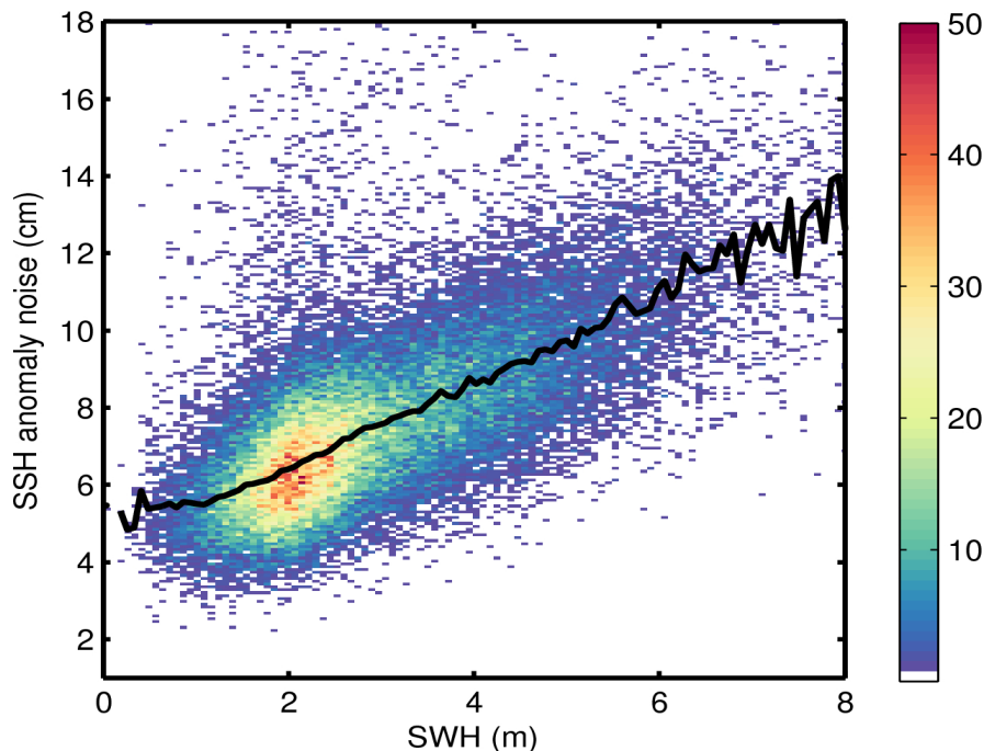
Figure 9. 2D histogram showing flag-valid SSH anomaly noise as a function of SWH for 11/01/2016. The black line denotes the median SSH anomaly noise as a function of SWH.
