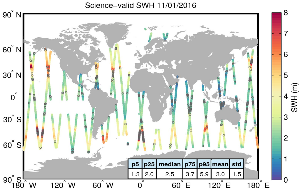
Figure 19. Geographical distribution of science-valid SWH data over oceans and lakes for 11/01/2016. The statistical values shown in the table refer to the SWH in m and are calculated over all measurements shown in the figure. Gray circles denote records that have been rejected based on the editing criteria described in Table 3.
