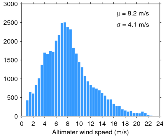
Figure 33. Histogram of flag-valid wind over oceans and lakes for 11/01/2016. The mean ( \mu ) and standard deviation ( \sigma ) are also shown. Note that values larger than 24 m/s are excluded from the histogram for the sake of readability but not from the computation of \mu and \sigma .
