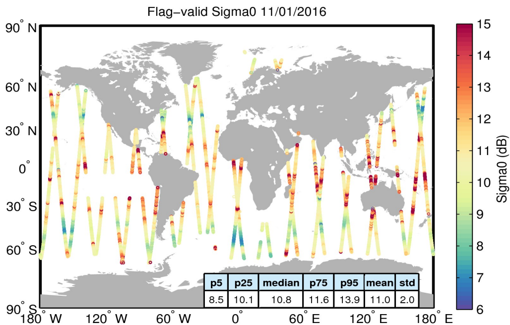
Figure 23. Geographical distribution of flag-valid sigma0 data over oceans and lakes for 11/01/2016. The statistical values shown in the table refer to the sigma0 in dB and are calculated over all measurements shown in the figure.
