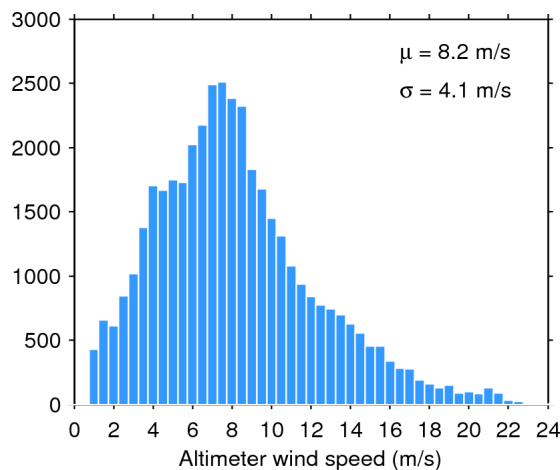
Figure 35. Histogram of science-valid wind over oceans and lakes for 11/01/2016. The mean ( \mu ) and standard deviation ( \sigma ) are also shown. Note that values larger than 24 m/s are excluded from the histogram for the sake of readability but not from the computation of \mu and \sigma .
