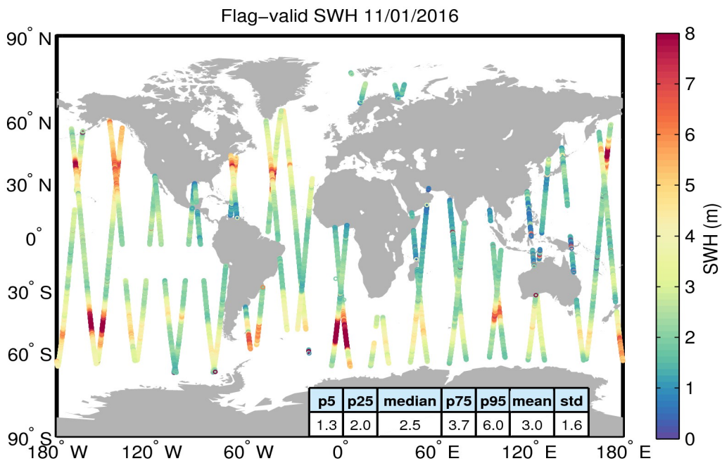
Figure 15. Geographical distribution of flag-valid SWH data over oceans and lakes for 11/01/2016. The statistical values shown in the table refer to the SWH in m and are calculated over all measurements shown in the figure.
