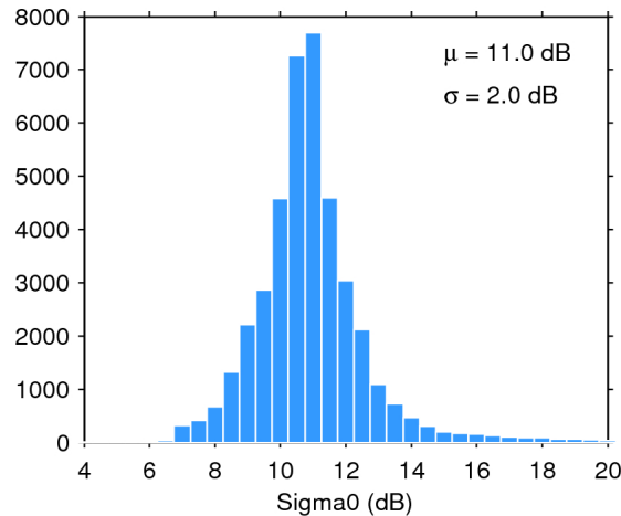
Figure 25. Histogram of flag-valid sigma0 over oceans and lakes for 11/01/2016. The mean ( \mu ) and standard deviation ( \sigma ) are also shown. Note that values outside [4 20] dB are excluded from the histogram for the sake of readability but not from the computation of \mu and \sigma .
