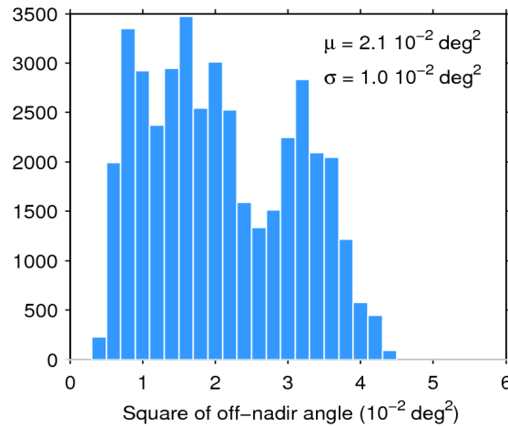
Figure 39. Histogram of flag-valid mispointing over oceans and lakes for 11/01/2016. The mean ( \mu ) and standard deviation ( \sigma ) are also shown. Note that values larger than 6 \cdot 10^{-2} \text{ deg}^2 are excluded from the histogram for the sake of readability but not from the computation of \mu and \sigma .
