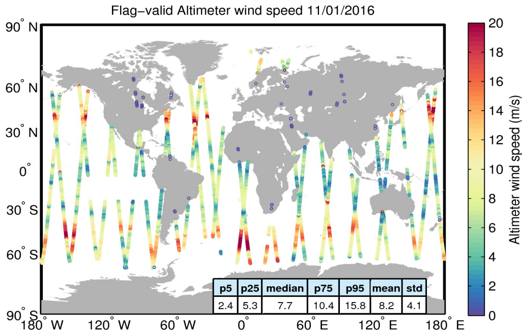
Figure 31. Geographical distribution of flag-valid wind data over oceans and lakes for 11/01/2016. The statistical values shown in the table refer to the wind in m/s and are calculated over all measurements shown in the figure.
