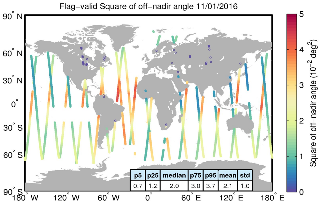
Figure 37. Geographical distribution of flag-valid mispointing data over oceans and lakes for 11/01/2016. The statistical values shown in the table refer to the mispointing in 10^{-2} \text{ deg}^2 and are calculated over all measurements shown in the figure.
