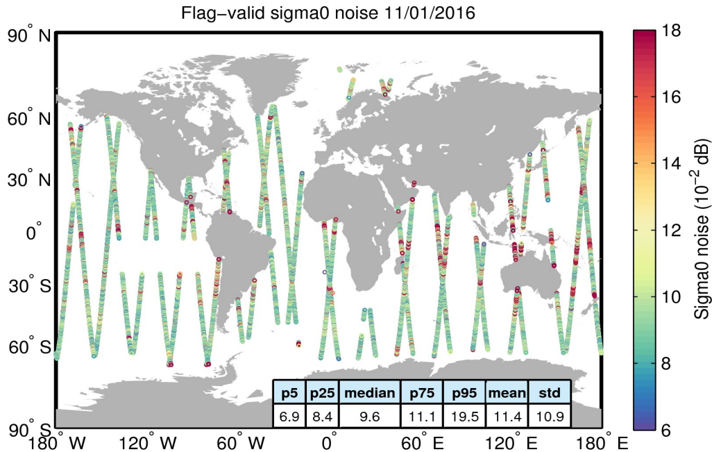
Figure 26. Geographical distribution of flag-valid 20-Hz sigma0 measurement noise over oceans and lakes for 11/01/2016. The statistical values shown in the table refer to the sigma0 noise and are calculated over all measurements shown in the figure.
