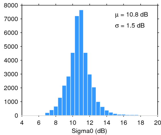
Figure 28. Histogram of science-valid sigma0 over oceans and lakes for 11/01/2016. The mean ( \mu ) and standard deviation ( \sigma ) are also shown. Note that values outside [4 20] dB are excluded from the histogram for the sake of readability but not from the computation of \mu and \sigma .
