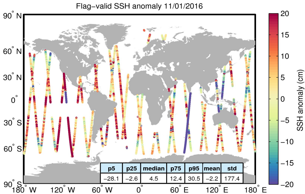
Figure 5. Geographical distribution of flag-valid 1-Hz SSH anomaly data over oceans and lakes for 11/01/2016. The statistical values shown in the table refer to the SSH anomaly in cm and are calculated over all measurements shown in the figure.
