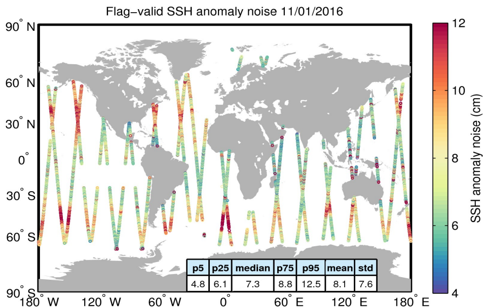
Figure 8. Geographical distribution of flag-valid 20-Hz SSH anomaly measurement noise over oceans and lakes for 11/01/2016. The statistical values shown in the table refer to the SSH anomaly noise and are calculated over all measurements shown in the figure.
