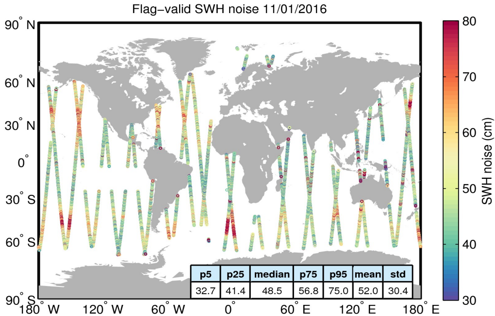
Figure 18. Geographical distribution of flag-valid 20-Hz SWH measurement noise over oceans and lakes for 11/01/2016. The statistical values shown in the figure refer to the SWH noise and are calculated over all measurements shown in the figure.
