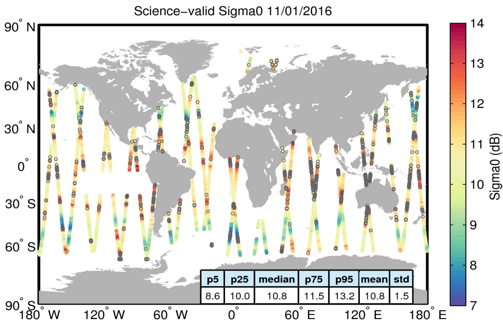
Figure 27. Geographical distribution of science-valid sigma0 data over oceans and lakes for 11/01/2016. The statistical values shown in the table refer to the sigma0 in dB and are calculated over all measurements shown in the figure. Gray circles denote records that have been rejected based on the editing criteria described in Table 4.
