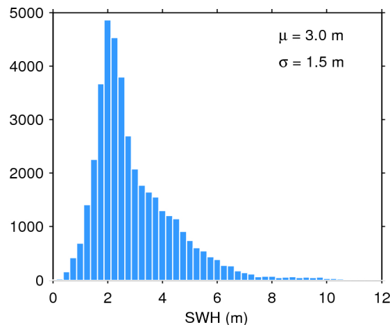
Figure 20. Histogram of science-valid SWH over oceans and lakes for 11/01/2016. The mean ( \mu ) and standard deviation ( \sigma ) are also shown. Note that values larger than 12 m are excluded from the histogram for the sake of readability but not from the computation of \mu and \sigma .
