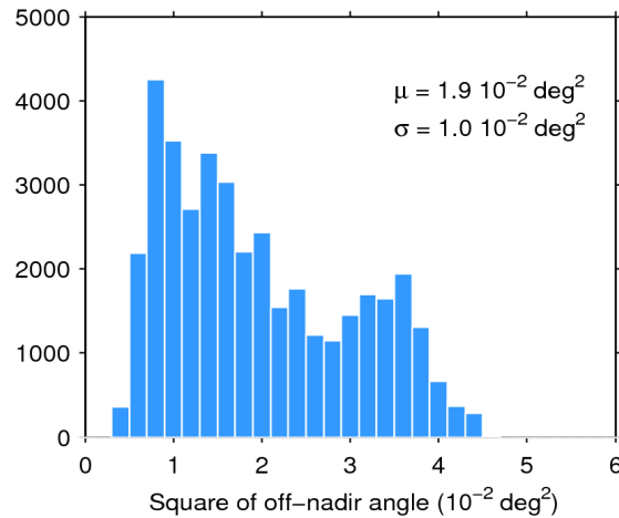
Figure 39. Histogram of flag-valid mispointing over oceans and lakes for 10/01/2016. The mean ( \mu ) and standard deviation ( \sigma ) are also shown. Note that values larger than 6 \cdot 10^{-2} \text{ deg}^2 are excluded from the histogram for the sake of readability but not from the computation of \mu and \sigma .
