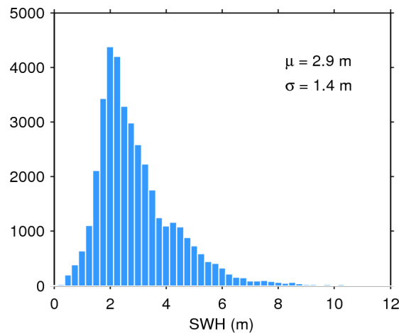
Figure 20. Histogram of science-valid SWH over oceans and lakes for 10/01/2016. The mean ( \mu ) and standard deviation ( \sigma ) are also shown. Note that values larger than 12 m are excluded from the histogram for the sake of readability but not from the computation of \mu and \sigma .
