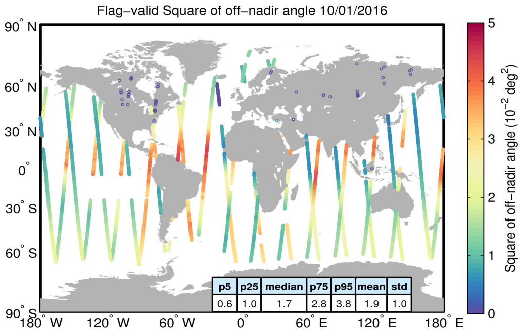
Figure 37. Geographical distribution of flag-valid mispointing data over oceans and lakes for 10/01/2016. The statistical values shown in the table refer to the mispointing in 10^{-2} deg 2 and are calculated over all measurements shown in the figure.
