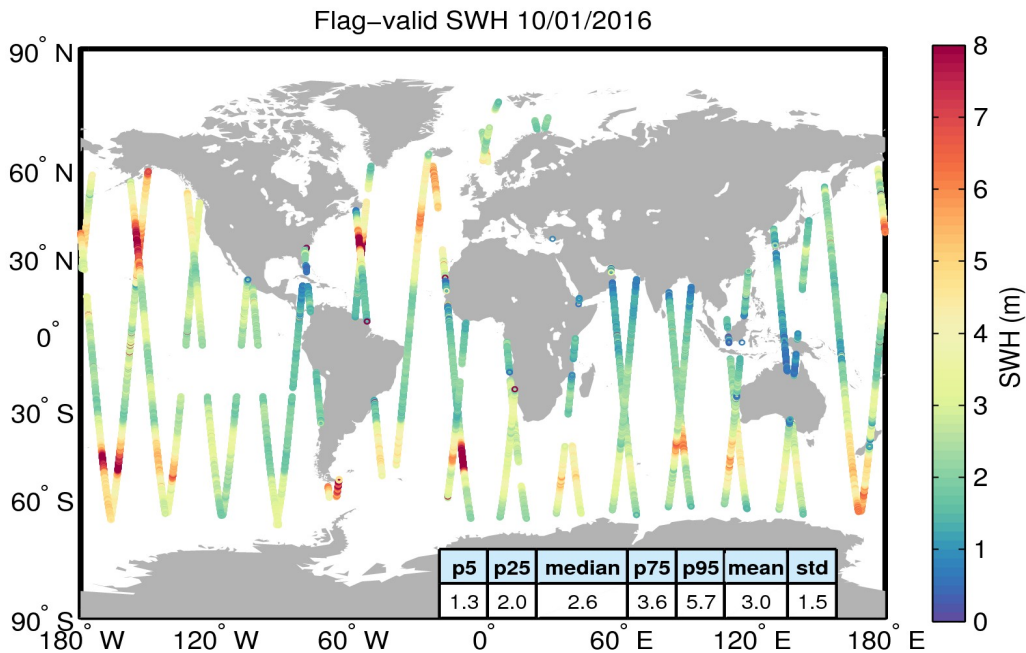
Figure 15. Geographical distribution of flag-valid SWH data over oceans and lakes for 10/01/2016. The statistical values shown in the table refer to the SWH in m and are calculated over all measurements shown in the figure.
