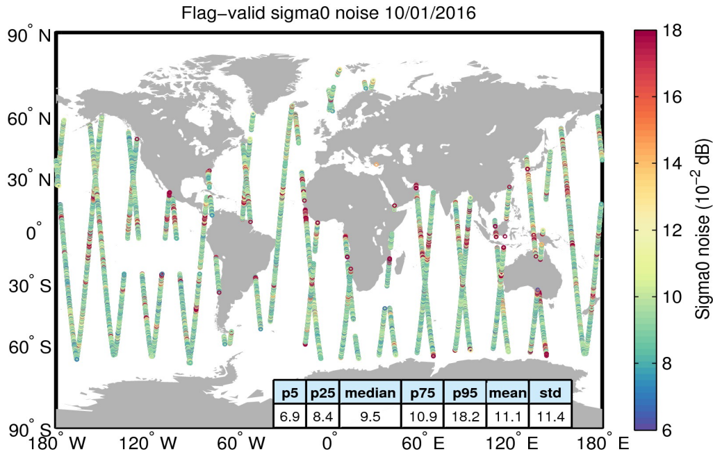
Figure 26. Geographical distribution of flag-valid 20-Hz sigma0 measurement noise over oceans and lakes for 10/01/2016. The statistical values shown in the table refer to the sigma0 noise and are calculated over all measurements shown in the figure.
