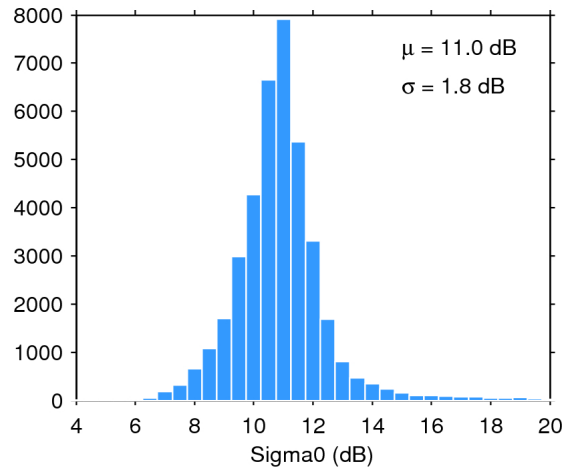
Figure 25. Histogram of flag-valid sigma0 over oceans and lakes for 10/01/2016. The mean ( \mu ) and standard deviation ( \sigma ) are also shown. Note that values outside [4 20] dB are excluded from the histogram for the sake of readability but not from the computation of \mu and \sigma .
