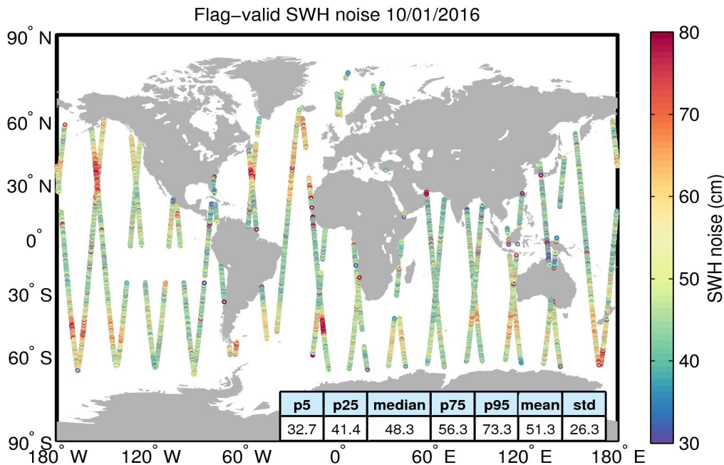
Figure 18. Geographical distribution of flag-valid 20-Hz SWH measurement noise over oceans and lakes for 10/01/2016. The statistical values shown in the figure refer to the SWH noise and are calculated over all measurements shown in the figure.
