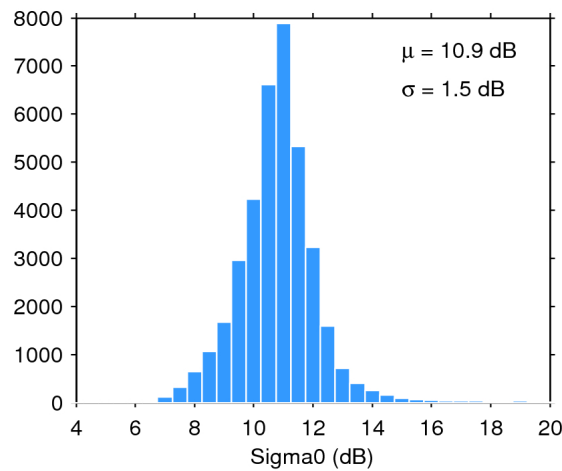
Figure 28. Histogram of science-valid sigma0 over oceans and lakes for 10/01/2016. The mean ( \mu ) and standard deviation ( \sigma ) are also shown. Note that values outside [4 20] dB are excluded from the histogram for the sake of readability but not from the computation of \mu and \sigma .
