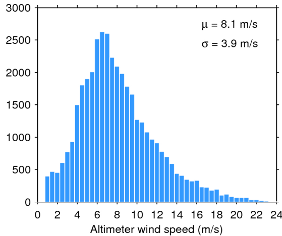
Figure 33. Histogram of flag-valid wind over oceans and lakes for 10/01/2016. The mean ( \mu ) and standard deviation ( \sigma ) are also shown. Note that values larger than 24 m/s are excluded from the histogram for the sake of readability but not from the computation of \mu and \sigma .
