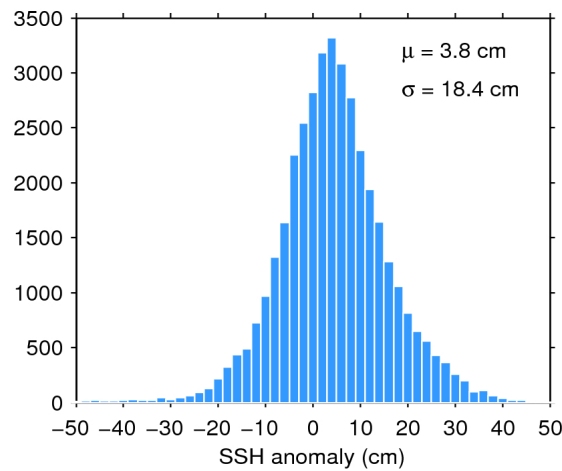
Figure 7. Histogram of flag-valid SSH anomaly over oceans and lakes for 10/01/2016. The mean ( \mu ) and standard deviation ( \sigma ) are also shown. Note that values outside [-50\ 50] cm are excluded from the histogram for the sake of readability but not from the computation of \mu and \sigma .
