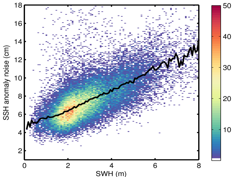
Figure 9. 2D histogram showing flag-valid SSH anomaly noise as a function of SWH for 10/01/2016. The black line denotes the median SSH anomaly noise as a function of SWH.
