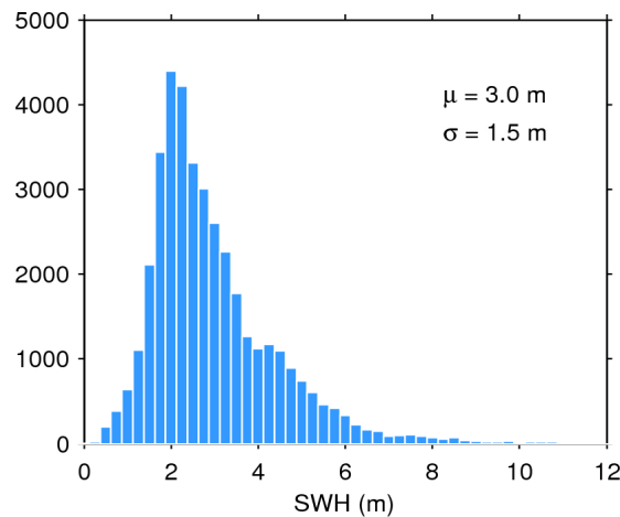
Figure 17. Histogram of flag-valid SWH over oceans and lakes for 10/01/2016. The mean ( \mu ) and standard deviation ( \sigma ) are also shown. Note that values larger than 12 m are excluded from the histogram for the sake of readability but not from the computation of \mu and \sigma .
