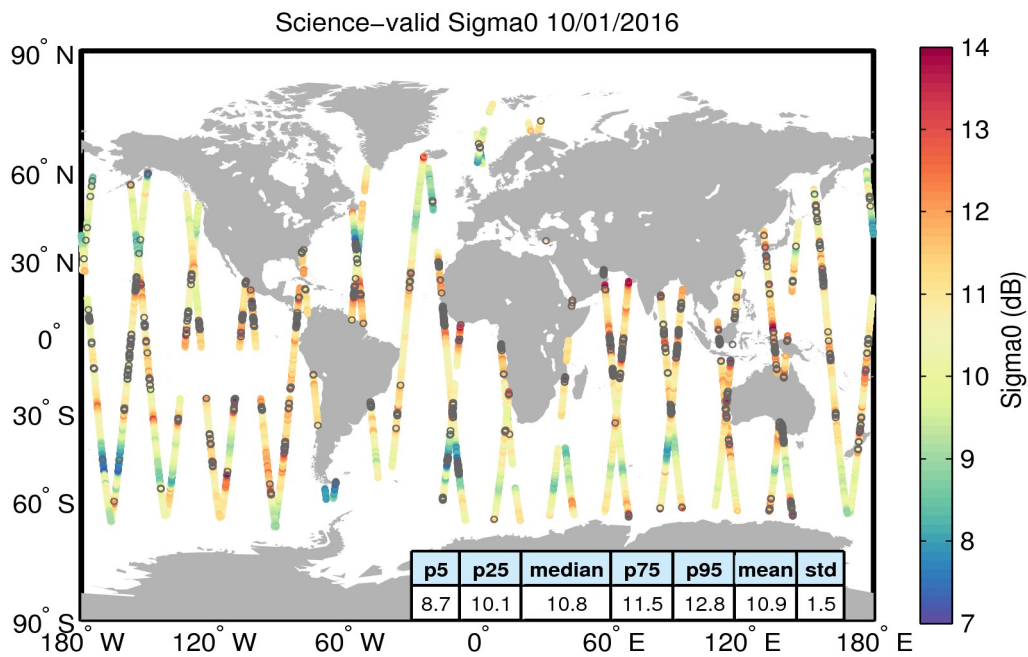
Figure 27. Geographical distribution of science-valid sigma0 data over oceans and lakes for 10/01/2016. The statistical values shown in the table refer to the sigma0 in dB and are calculated over all measurements shown in the figure. Gray circles denote records that have been rejected based on the editing criteria described in Table 4.
