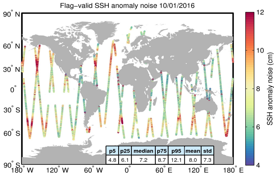
Figure 8. Geographical distribution of flag-valid 20-Hz SSH anomaly measurement noise over oceans and lakes for 10/01/2016. The statistical values shown in the table refer to the SSH anomaly noise and are calculated over all measurements shown in the figure.
