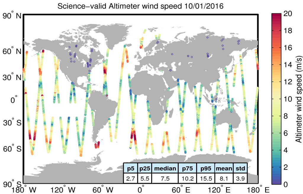
Figure 34. Geographical distribution of science-valid wind data over oceans and lakes for 10/01/2016. The statistical values shown in the table refer to the wind in m/s and are calculated over all measurements shown in the figure. Gray circles denote records that have been rejected based on the editing criteria described in Table 5.
