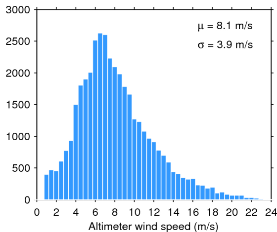
Figure 35. Histogram of science-valid wind over oceans and lakes for 10/01/2016. The mean ( \mu ) and standard deviation ( \sigma ) are also shown. Note that values larger than 24 m/s are excluded from the histogram for the sake of readability but not from the computation of \mu and \sigma .
