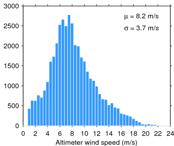
Figure 35. Histogram of science-valid wind over oceans and lakes for 09/01/2016. The mean ( \mu ) and standard deviation ( \sigma ) are also shown. Note that values larger than 24 m/s are excluded from the histogram for the sake of readability but not from the computation of \mu and \sigma .
