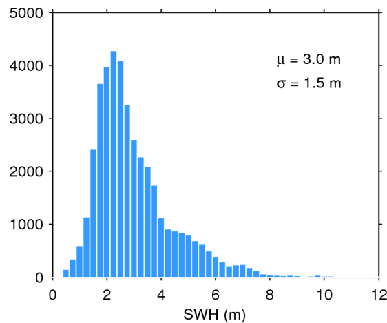
Figure 17. Histogram of flag-valid SWH over oceans and lakes for 09/01/2016. The mean ( \mu ) and standard deviation ( \sigma ) are also shown. Note that values larger than 12 m are excluded from the histogram for the sake of readability but not from the computation of \mu and \sigma .
