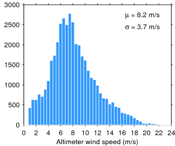
Figure 33. Histogram of flag-valid wind over oceans and lakes for 09/01/2016. The mean ( \mu ) and standard deviation ( \sigma ) are also shown. Note that values larger than 24 m/s are excluded from the histogram for the sake of readability but not from the computation of \mu and \sigma .
