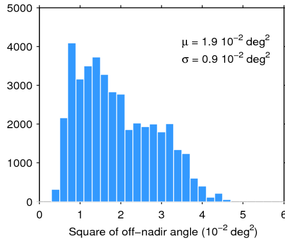
Figure 39. Histogram of flag-valid mispointing over oceans and lakes for 09/01/2016. The mean ( \mu ) and standard deviation ( \sigma ) are also shown. Note that values larger than 6 \cdot 10^{-2} \text{ deg}^2 are excluded from the histogram for the sake of readability but not from the computation of \mu and \sigma .
