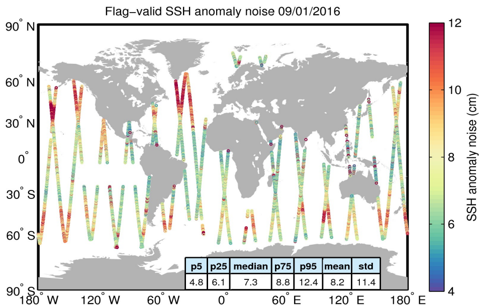
Figure 8. Geographical distribution of flag-valid 20-Hz SSH anomaly measurement noise over oceans and lakes for 09/01/2016. The statistical values shown in the table refer to the SSH anomaly noise and are calculated over all measurements shown in the figure.
