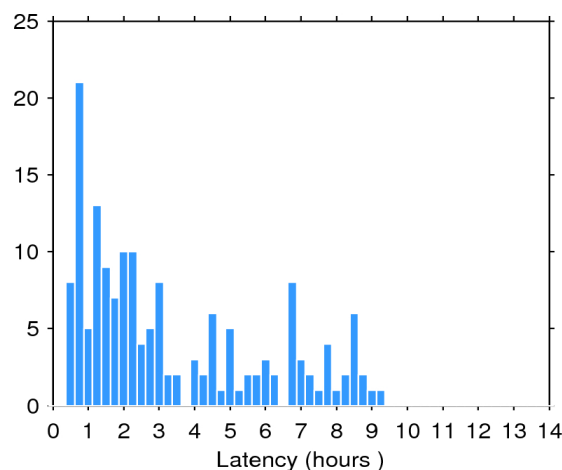
Figure 2. Histogram of the data latency for 09/01/2016. The y-axis denotes the number of files that are made available with a delay of x-hours with respect to the mean time of the records stored in the file.
