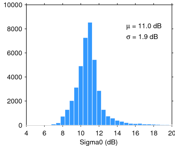
Figure 25. Histogram of flag-valid sigma0 over oceans and lakes for 09/01/2016. The mean ( \mu ) and standard deviation ( \sigma ) are also shown. Note that values outside [4 20] dB are excluded from the histogram for the sake of readability but not from the computation of \mu and \sigma .
