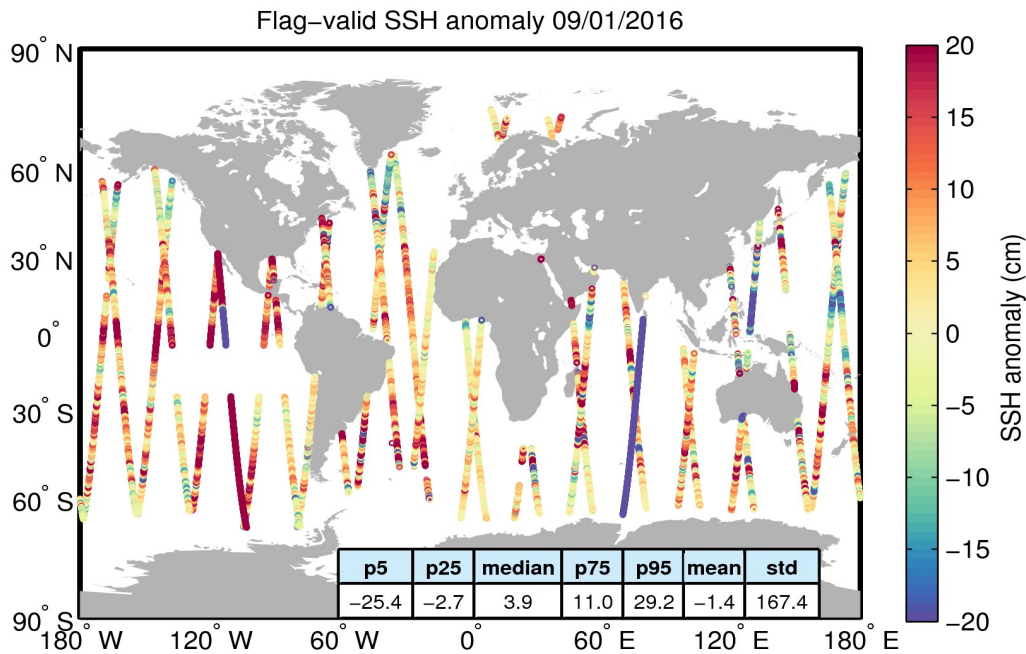
Figure 5. Geographical distribution of flag-valid 1-Hz SSH anomaly data over oceans and lakes for 09/01/2016. The statistical values shown in the table refer to the SSH anomaly in cm and are calculated over all measurements shown in the figure.
