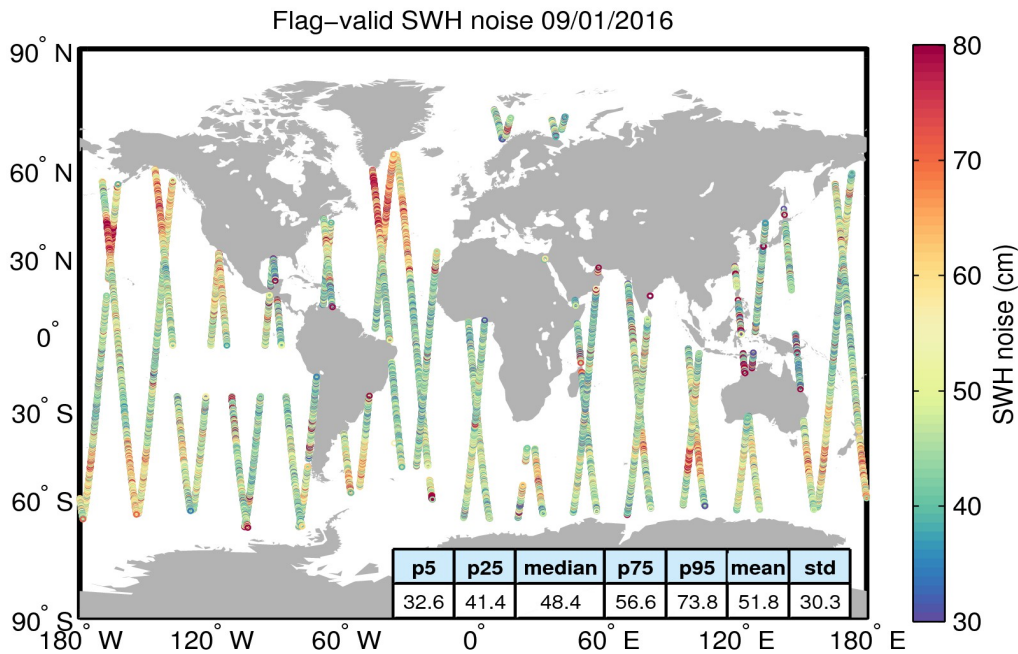
Figure 18. Geographical distribution of flag-valid 20-Hz SWH measurement noise over oceans and lakes for 09/01/2016. The statistical values shown in the table refer to the SWH noise and are calculated over all measurements shown in the figure.
