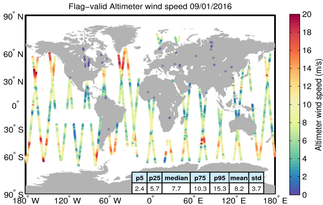
Figure 31. Geographical distribution of flag-valid wind data over oceans and lakes for 09/01/2016. The statistical values shown in the table refer to the wind in m/s and are calculated over all measurements shown in the figure.
