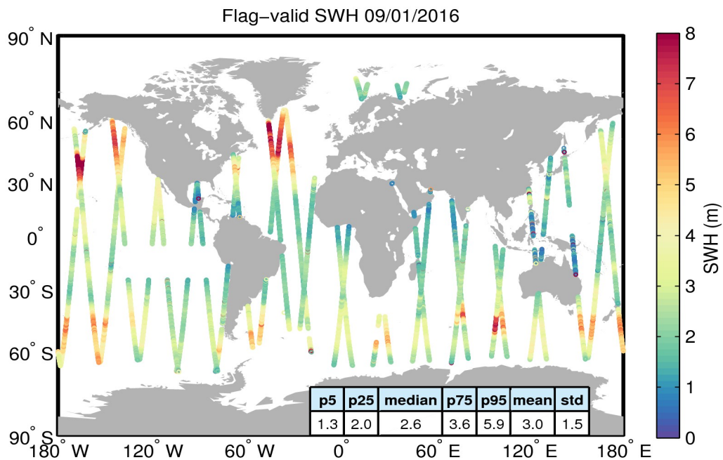
Figure 15. Geographical distribution of flag-valid SWH data over oceans and lakes for 09/01/2016. The statistical values shown in the table refer to the SWH in m and are calculated over all measurements shown in the figure.
