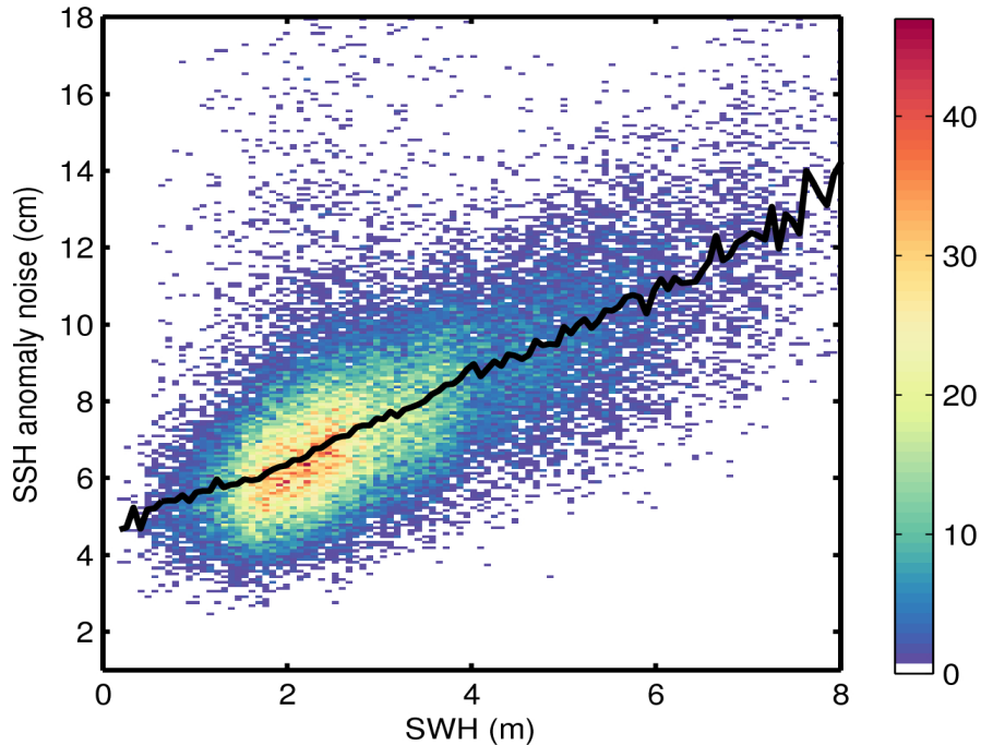
Figure 9. 2D histogram showing flag-valid SSH anomaly noise as a function of SWH for 09/01/2016. The black line denotes the median SSH anomaly noise as a function of SWH.
