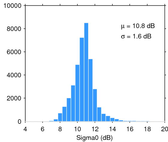
Figure 28. Histogram of science-valid sigma0 over oceans and lakes for 09/01/2016. The mean ( \mu ) and standard deviation ( \sigma ) are also shown. Note that values outside [4 20] dB are excluded from the histogram for the sake of readability but not from the computation of \mu and \sigma .
