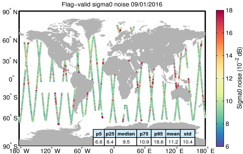
Figure 26. Geographical distribution of flag-valid 20-Hz sigma0 measurement noise over oceans and lakes for 09/01/2016. The statistical values shown in the table refer to the sigma0 noise and are calculated over all measurements shown in the figure.
