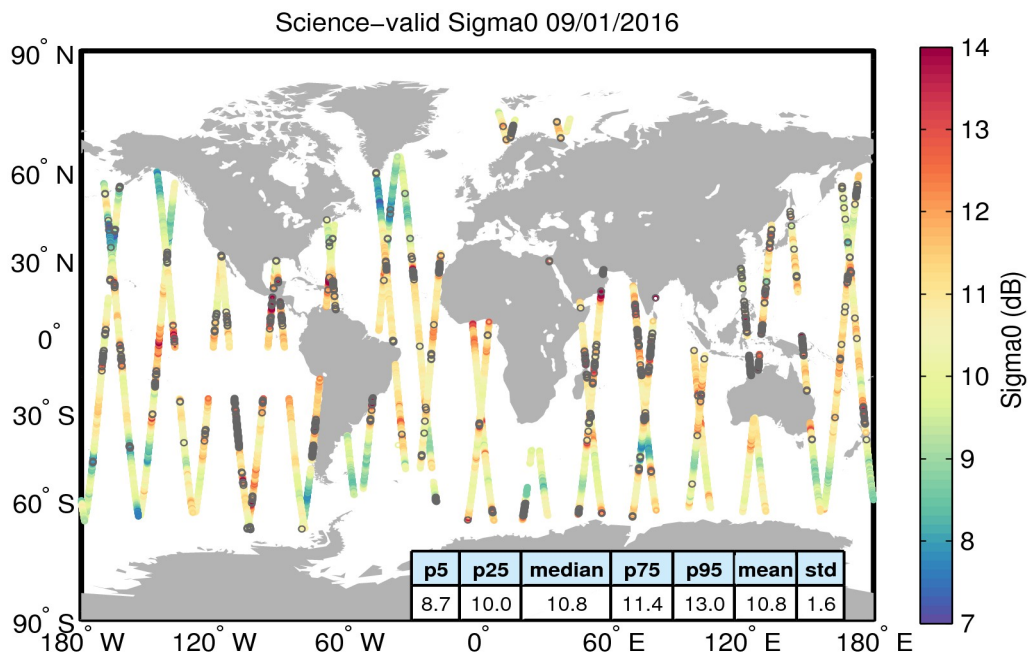
Figure 27. Geographical distribution of science-valid sigma0 data over oceans and lakes for 09/01/2016. The statistical values shown in the table refer to the sigma0 in dB and are calculated over all measurements shown in the figure. Gray circles denote records that have been rejected based on the editing criteria described in Table 4.
