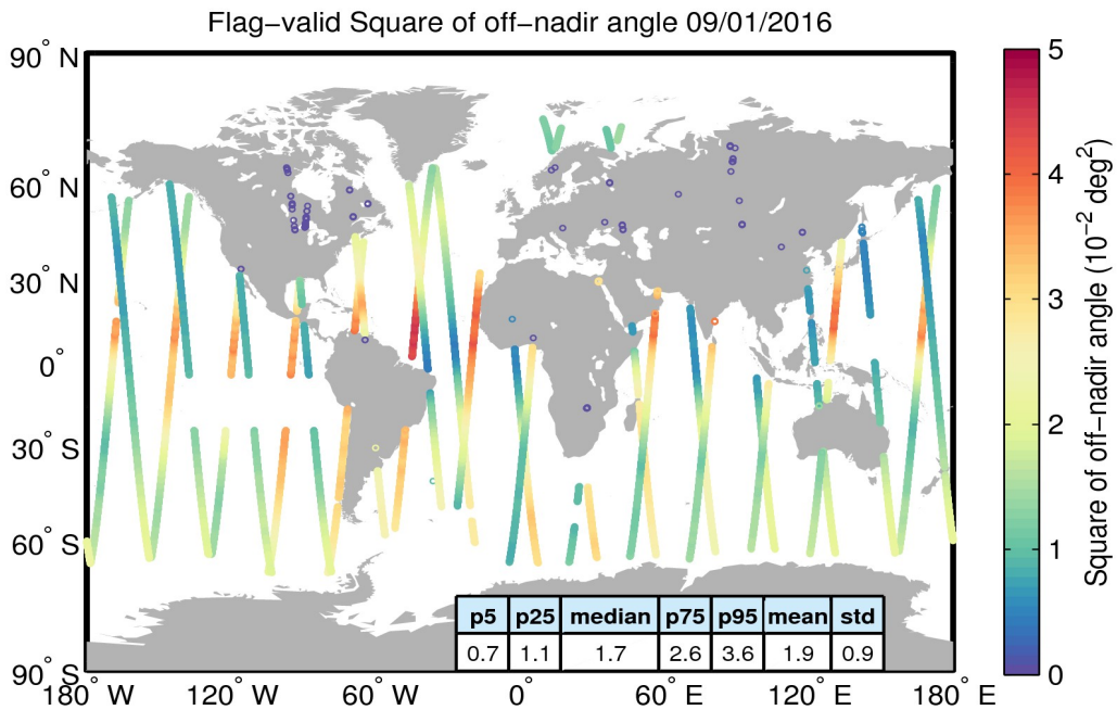
Figure 37. Geographical distribution of flag-valid mispointing data over oceans and lakes for 09/01/2016. The statistical values shown in the table refer to the mispointing in 10^{-2} deg 2 and are calculated over all measurements shown in the figure.
