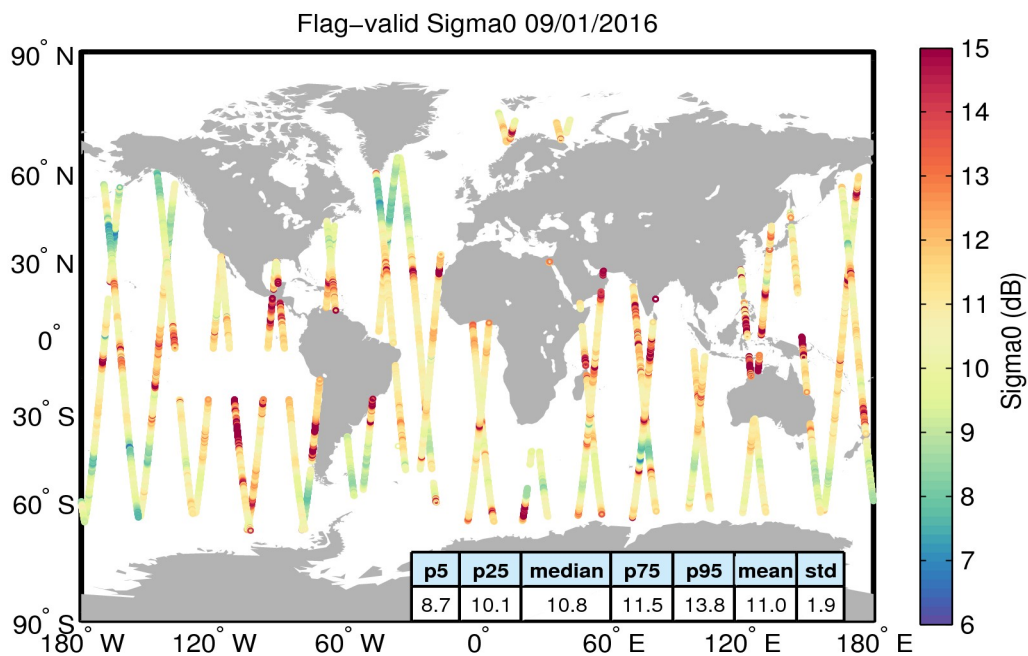
Figure 23. Geographical distribution of flag-valid sigma0 data over oceans and lakes for 09/01/2016. The statistical values shown in the table refer to the sigma0 in dB and are calculated over all measurements shown in the figure.
