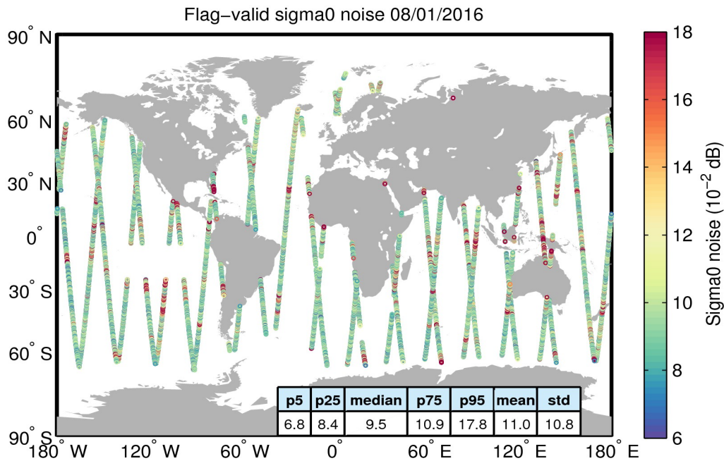
Figure 26. Geographical distribution of flag-valid 20-Hz sigma0 measurement noise over oceans and lakes for 08/01/2016. The statistical values shown in the table refer to the sigma0 noise and are calculated over all measurements shown in the figure.
