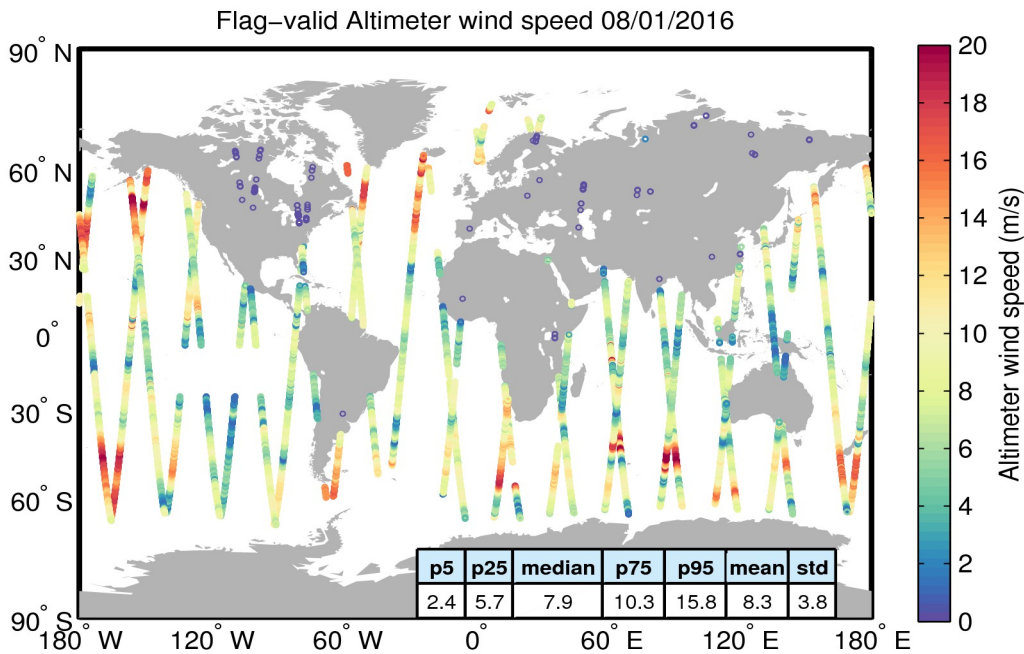
Figure 31. Geographical distribution of flag-valid wind data over oceans and lakes for 08/01/2016. The statistical values shown in the table refer to the wind in m/s and are calculated over all measurements shown in the figure.
