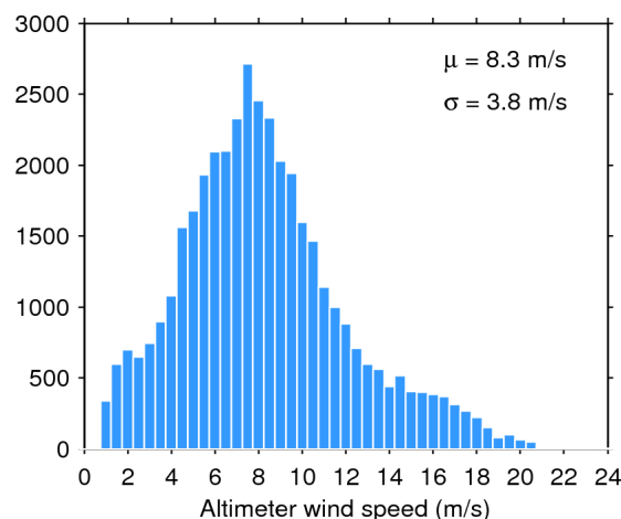
Figure 35. Histogram of science-valid wind over oceans and lakes for 08/01/2016. The mean ( \mu ) and standard deviation ( \sigma ) are also shown. Note that values larger than 24 m/s are excluded from the histogram for the sake of readability but not from the computation of \mu and \sigma .
