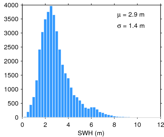
Figure 17. Histogram of flag-valid SWH over oceans and lakes for 08/01/2016. The mean ( \mu ) and standard deviation ( \sigma ) are also shown. Note that values larger than 12 m are excluded from the histogram for the sake of readability but not from the computation of \mu and \sigma .
