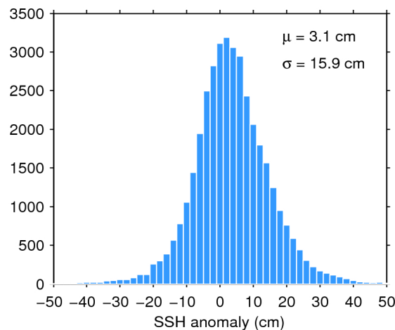
Figure 11. Histogram of science-valid SSH anomaly over oceans and lakes for 08/01/2016. The mean ( \mu ) and standard deviation ( \sigma ) are also shown. Note that values outside [-50 50] cm are excluded from the histogram for the sake of readability but not from the computation of \mu and \sigma .
