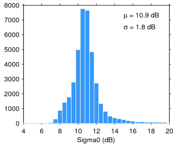
Figure 25. Histogram of flag-valid sigma0 over oceans and lakes for 08/01/2016. The mean ( \mu ) and standard deviation ( \sigma ) are also shown. Note that values outside [4 20] dB are excluded from the histogram for the sake of readability but not from the computation of \mu and \sigma .
