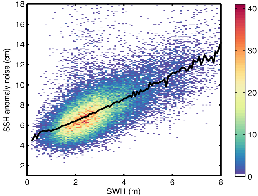
Figure 9. 2D histogram showing flag-valid SSH anomaly noise as a function of SWH for 08/01/2016. The black line denotes the median SSH anomaly noise as a function of SWH.
