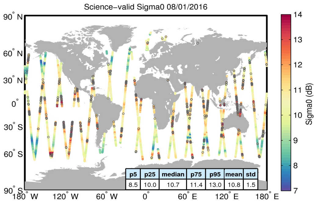
Figure 27. Geographical distribution of science-valid sigma0 data over oceans and lakes for 08/01/2016. The statistical values shown in the table refer to the sigma0 in dB and are calculated over all measurements shown in the figure. Gray circles denote records that have been rejected based on the editing criteria described in Table 4.
