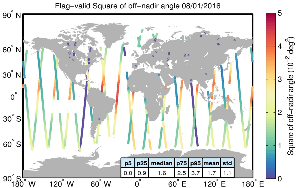
Figure 37. Geographical distribution of flag-valid mispointing data over oceans and lakes for 08/01/2016. The statistical values shown in the table refer to the mispointing in 10^{-2} deg 2 and are calculated over all measurements shown in the figure.
