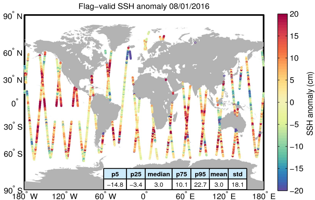
Figure 5. Geographical distribution of flag-valid 1-Hz SSH anomaly data over oceans and lakes for 08/01/2016. The statistical values shown in the table refer to the SSH anomaly in cm and are calculated over all measurements shown in the figure.
