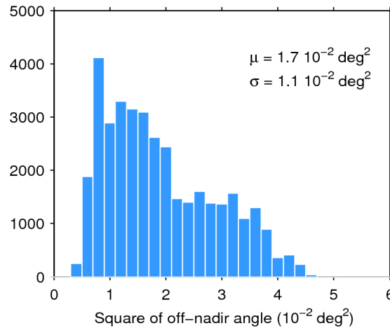
Figure 39. Histogram of flag-valid mispointing over oceans and lakes for 08/01/2016. The mean ( \mu ) and standard deviation ( \sigma ) are also shown. Note that values larger than 6 \cdot 10^{-2} \text{ deg}^2 are excluded from the histogram for the sake of readability but not from the computation of \mu and \sigma .
