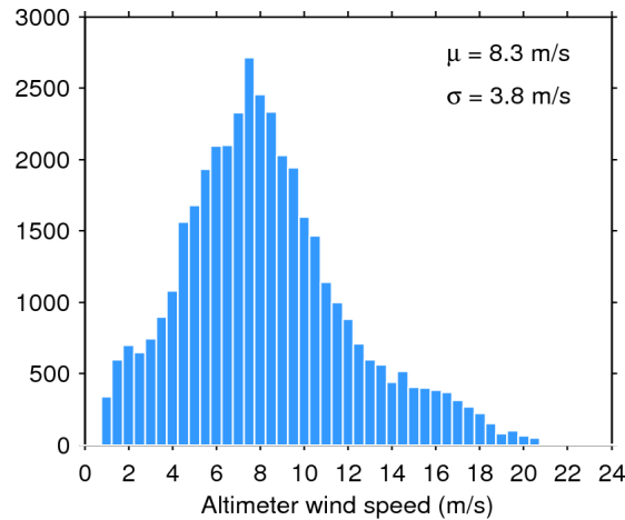
Figure 33. Histogram of flag-valid wind over oceans and lakes for 08/01/2016. The mean ( \mu ) and standard deviation ( \sigma ) are also shown. Note that values larger than 24 m/s are excluded from the histogram for the sake of readability but not from the computation of \mu and \sigma .
