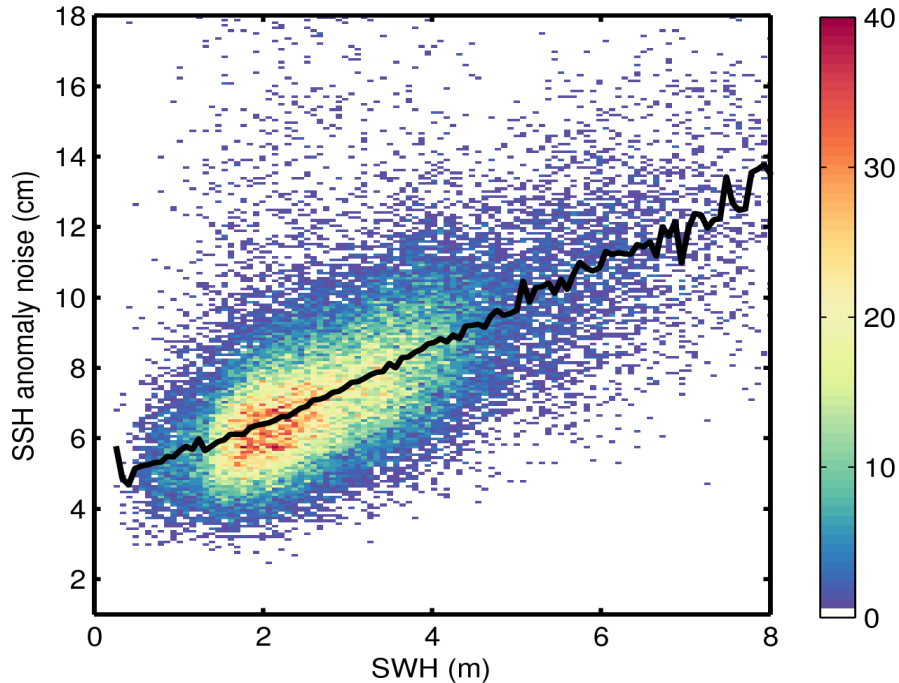
Figure 9. 2D histogram showing flag-valid SSH anomaly noise as a function of SWH for 07/01/2016. The black line denotes the median SSH anomaly noise as a function of SWH.
