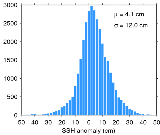
Figure 11. Histogram of science-valid SSH anomaly over oceans and lakes for 07/01/2016. The mean ( \mu ) and standard deviation ( \sigma ) are also shown. Note that values outside [-50 50] cm are excluded from the histogram for the sake of readability but not from the computation of \mu and \sigma .
