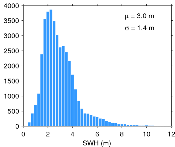
Figure 20. Histogram of science-valid SWH over oceans and lakes for 07/01/2016. The mean ( \mu ) and standard deviation ( \sigma ) are also shown. Note that values larger than 12 m are excluded from the histogram for the sake of readability but not from the computation of \mu and \sigma .
