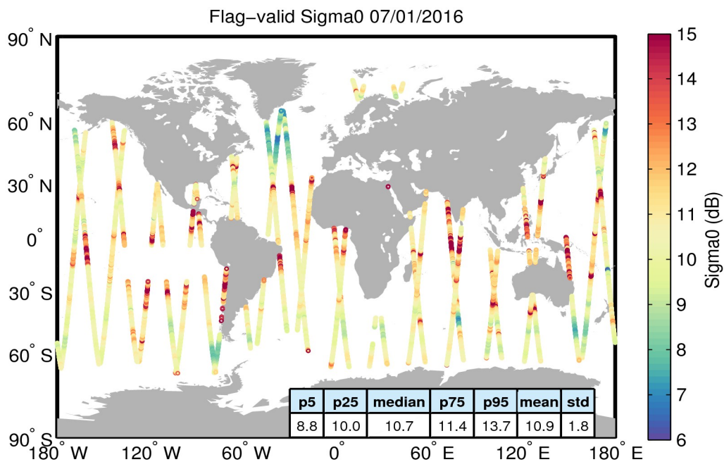
Figure 23. Geographical distribution of flag-valid sigma0 data over oceans and lakes for 07/01/2016. The statistical values shown in the table refer to the sigma0 in dB and are calculated over all measurements shown in the figure.
