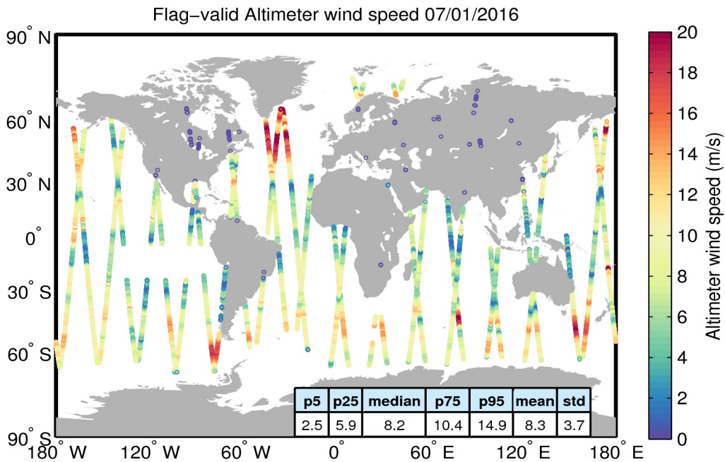
Figure 31. Geographical distribution of flag-valid wind data over oceans and lakes for 07/01/2016. The statistical values shown in the table refer to the wind in m/s and are calculated over all measurements shown in the figure.
