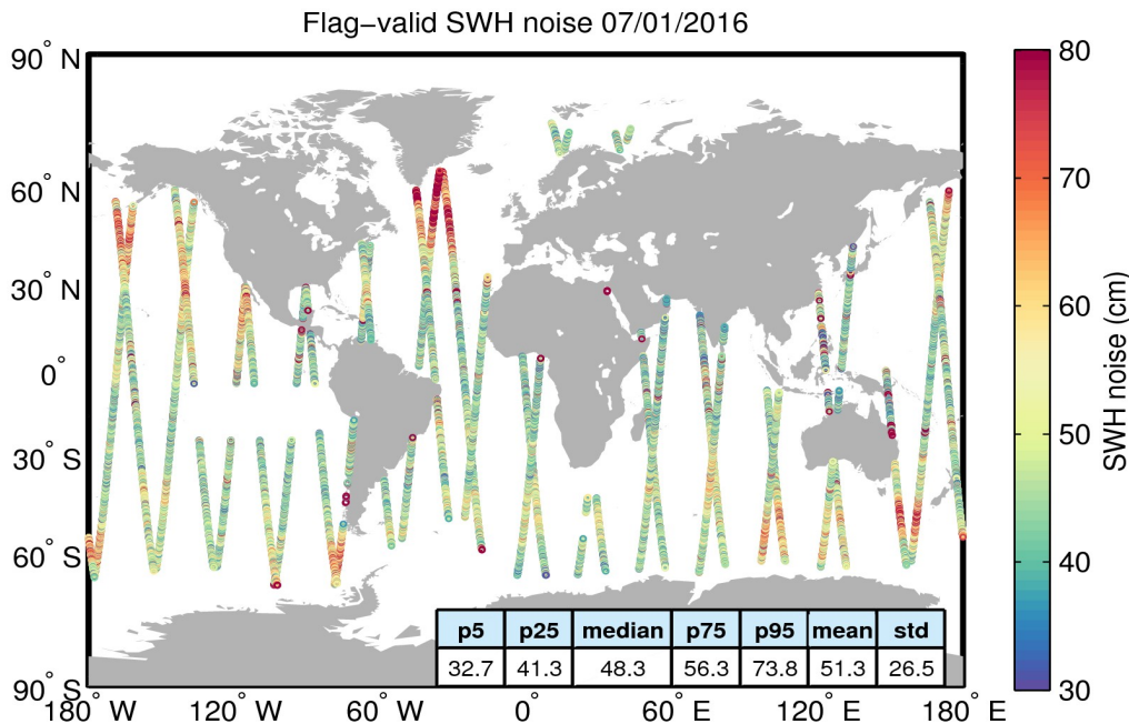
Figure 18. Geographical distribution of flag-valid 20-Hz SWH measurement noise over oceans and lakes for 07/01/2016. The statistical values shown in the table refer to the SWH noise and are calculated over all measurements shown in the figure.
