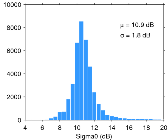
Figure 25. Histogram of flag-valid sigma0 over oceans and lakes for 07/01/2016. The mean ( \mu ) and standard deviation ( \sigma ) are also shown. Note that values outside [4 20] dB are excluded from the histogram for the sake of readability but not from the computation of \mu and \sigma .
