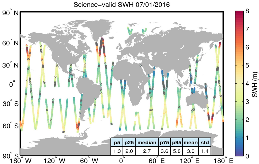
Figure 19. Geographical distribution of science-valid SWH data over oceans and lakes for 07/01/2016. The statistical values shown in the table refer to the SWH in m and are calculated over all measurements shown in the figure. Gray circles denote records that have been rejected based on the editing criteria described in Table 3.
