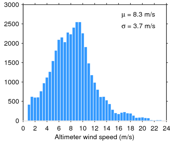
Figure 33. Histogram of flag-valid wind over oceans and lakes for 07/01/2016. The mean ( \mu ) and standard deviation ( \sigma ) are also shown. Note that values larger than 24 m/s are excluded from the histogram for the sake of readability but not from the computation of \mu and \sigma .
