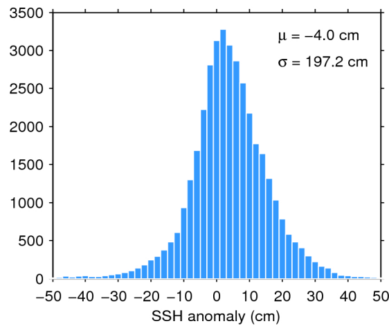
Figure 7. Histogram of flag-valid SSH anomaly over oceans and lakes for 07/01/2016. The mean ( \mu ) and standard deviation ( \sigma ) are also shown. Note that values outside [-50\ 50] cm are excluded from the histogram for the sake of readability but not from the computation of \mu and \sigma .
