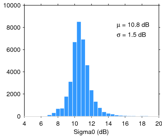
Figure 28. Histogram of science-valid sigma0 over oceans and lakes for 07/01/2016. The mean ( \mu ) and standard deviation ( \sigma ) are also shown. Note that values outside [4 20] dB are excluded from the histogram for the sake of readability but not from the computation of \mu and \sigma .
