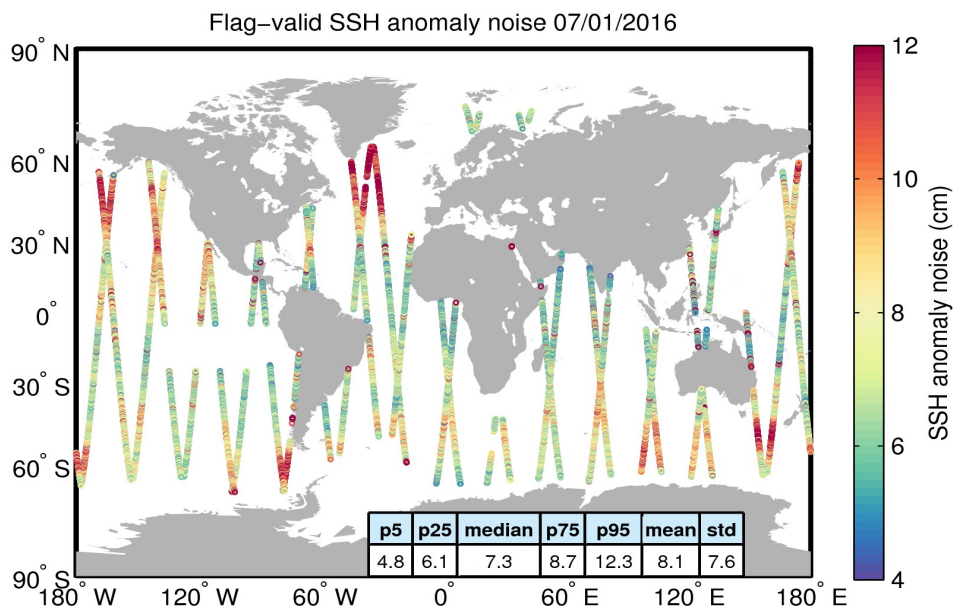
Figure 8. Geographical distribution of flag-valid 20-Hz SSH anomaly measurement noise over oceans and lakes for 07/01/2016. The statistical values shown in the table refer to the SSH anomaly noise and are calculated over all measurements shown in the figure.
