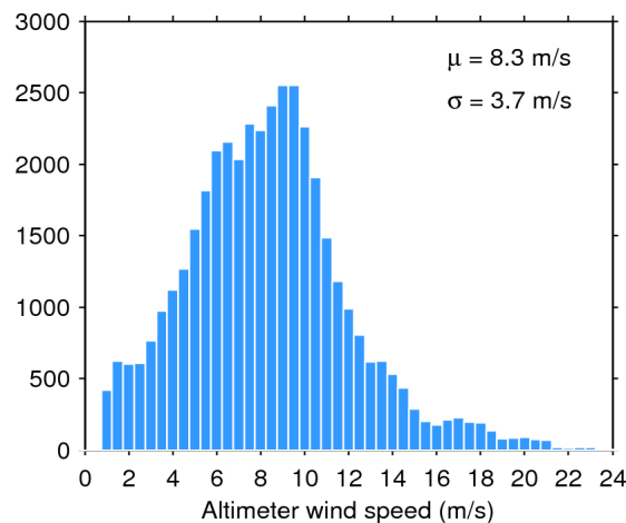
Figure 35. Histogram of science-valid wind over oceans and lakes for 07/01/2016. The mean ( \mu ) and standard deviation ( \sigma ) are also shown. Note that values larger than 24 m/s are excluded from the histogram for the sake of readability but not from the computation of \mu and \sigma .
