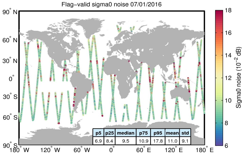
Figure 26. Geographical distribution of flag-valid 20-Hz sigma0 measurement noise over oceans and lakes for 07/01/2016. The statistical values shown in the table refer to the sigma0 noise and are calculated over all measurements shown in the figure.
