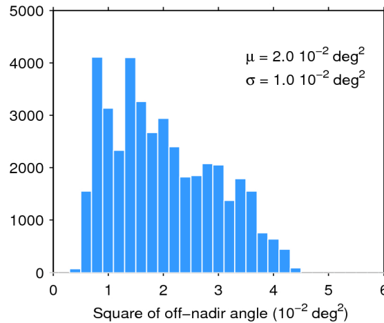
Figure 39. Histogram of flag-valid mispointing over oceans and lakes for 07/01/2016. The mean ( \mu ) and standard deviation ( \sigma ) are also shown. Note that values larger than 6 \cdot 10^{-2} \text{ deg}^2 are excluded from the histogram for the sake of readability but not from the computation of \mu and \sigma .
