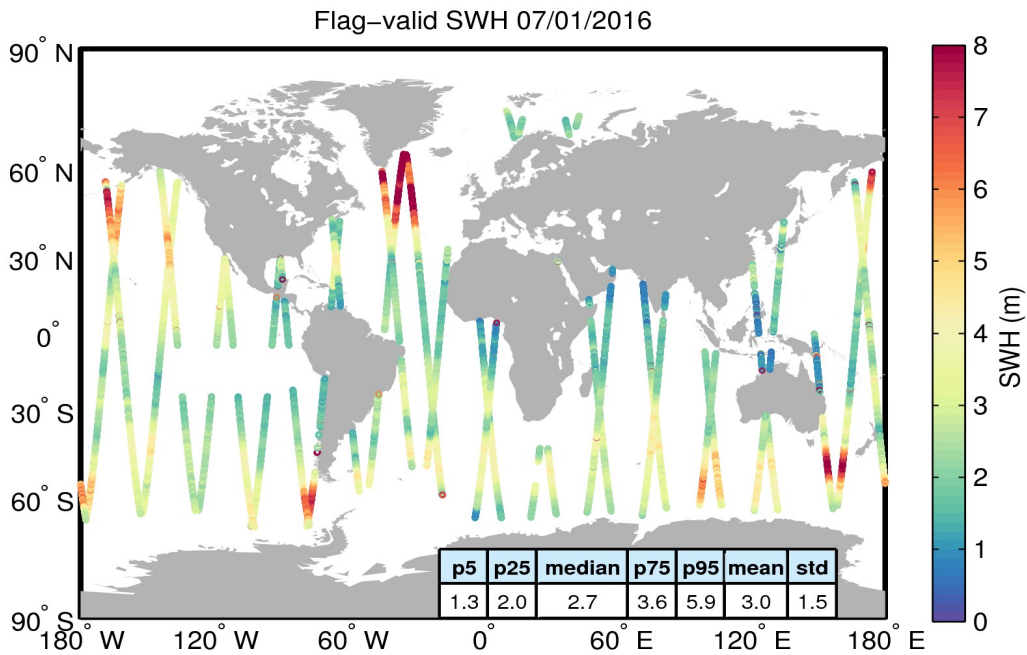
Figure 15. Geographical distribution of flag-valid SWH data over oceans and lakes for 07/01/2016. The statistical values shown in the table refer to the SWH in m and are calculated over all measurements shown in the figure.
