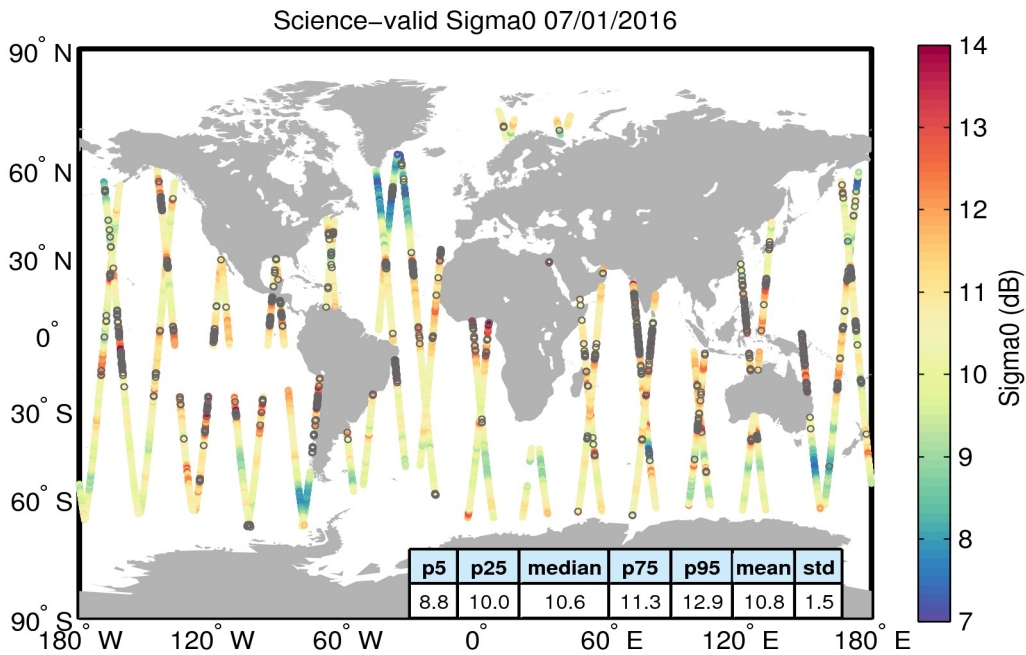
Figure 27. Geographical distribution of science-valid sigma0 data over oceans and lakes for 07/01/2016. The statistical values shown in the table refer to the sigma0 in dB and are calculated over all measurements shown in the figure. Gray circles denote records that have been rejected based on the editing criteria described in Table 4.
