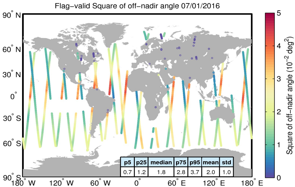
Figure 37. Geographical distribution of flag-valid mispointing data over oceans and lakes for 07/01/2016. The statistical values shown in the table refer to the mispointing in 10^{-2} deg 2 and are calculated over all measurements shown in the figure.
