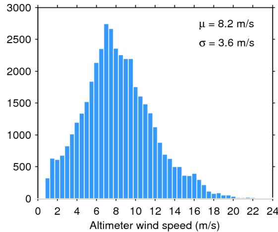
Figure 33. Histogram of flag-valid wind over oceans and lakes for 05/01/2016. The mean ( \mu ) and standard deviation ( \sigma ) are also shown. Note that values larger than 24 m/s are excluded from the histogram for the sake of readability but not from the computation of \mu and \sigma .
