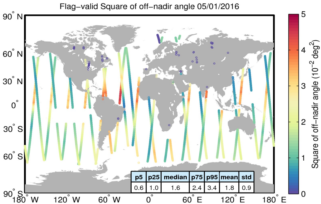
Figure 37. Geographical distribution of flag-valid mispointing data over oceans and lakes for 05/01/2016. The statistical values shown in the table refer to the mispointing in 10^{-2} \text{ deg}^2 and are calculated over all measurements shown in the figure.
