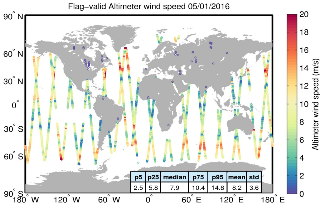
Figure 31. Geographical distribution of flag-valid wind data over oceans and lakes for 05/01/2016. The statistical values shown in the table refer to the wind in m/s and are calculated over all measurements shown in the figure.
