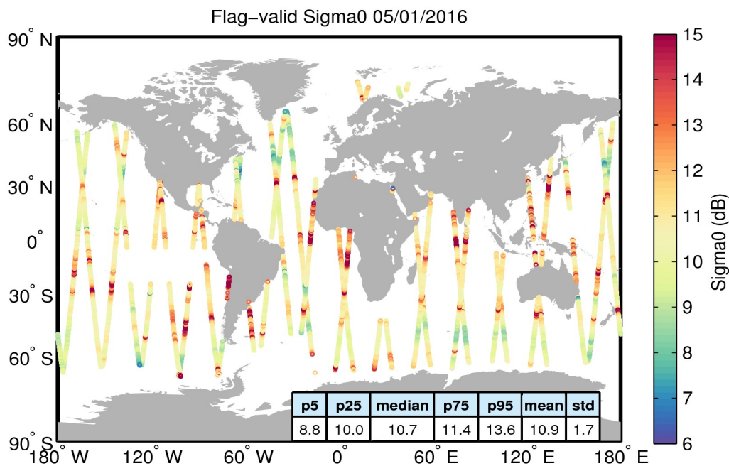
Figure 23. Geographical distribution of flag-valid sigma0 data over oceans and lakes for 05/01/2016. The statistical values shown in the table refer to the sigma0 in dB and are calculated over all measurements shown in the figure.
