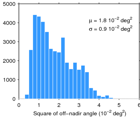
Figure 39. Histogram of flag-valid mispointing over oceans and lakes for 05/01/2016. The mean ( \mu ) and standard deviation ( \sigma ) are also shown. Note that values larger than 6 \cdot 10^{-2} \text{ deg}^2 are excluded from the histogram for the sake of readability but not from the computation of \mu and \sigma .
