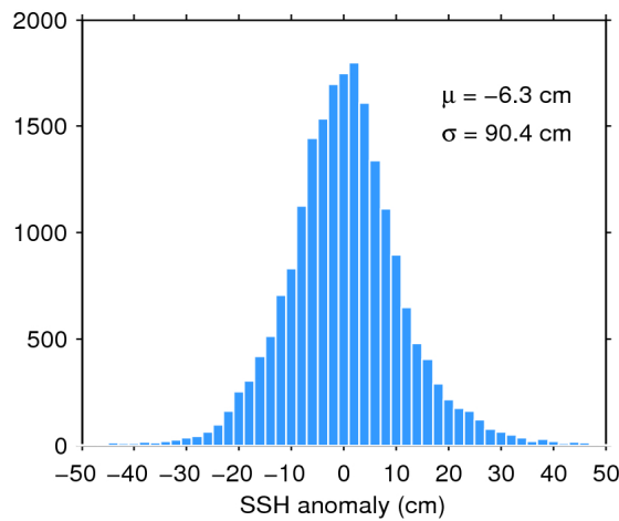
Figure 7. Histogram of flag-valid SSH anomaly over oceans and lakes for 05/01/2016. The mean ( \mu ) and standard deviation ( \sigma ) are also shown. Note that values outside [-50\ 50] cm are excluded from the histogram for the sake of readability but not from the computation of \mu and \sigma .
