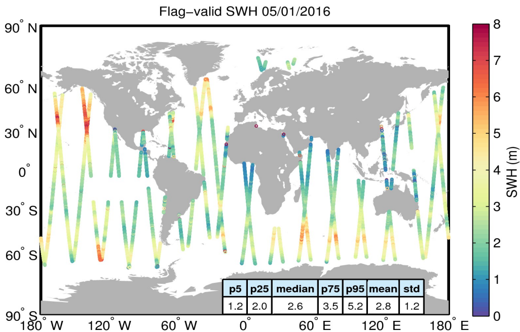
Figure 15. Geographical distribution of flag-valid SWH data over oceans and lakes for 05/01/2016. The statistical values shown in the table refer to the SWH in m and are calculated over all measurements shown in the figure.
