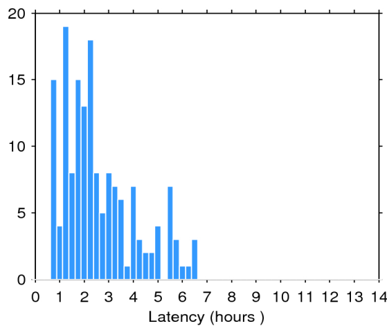
Figure 2. Histogram of the data latency for 05/01/2016. The y-axis denotes the number of files that are made available with a delay of x-hours with respect to the mean time of the records stored in the file.
