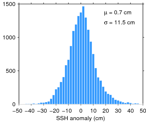
Figure 11. Histogram of science-valid SSH anomaly over oceans and lakes for 05/01/2016. The mean ( \mu ) and standard deviation ( \sigma ) are also shown. Note that values outside [-50 50] cm are excluded from the histogram for the sake of readability but not from the computation of \mu and \sigma .
