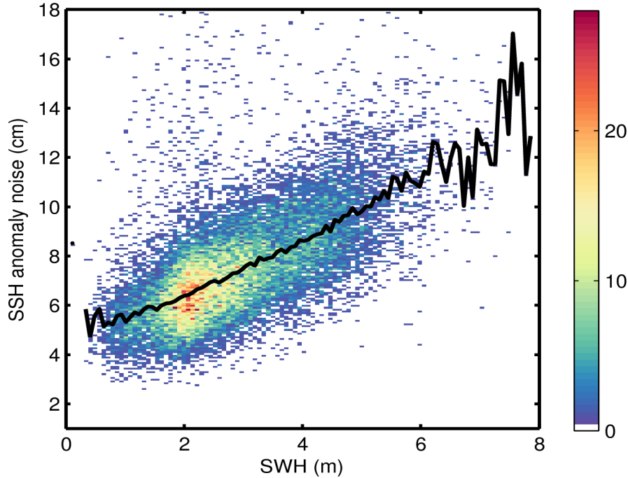
Figure 9. 2D histogram showing flag-valid SSH anomaly noise as a function of SWH for 05/01/2016. The black line denotes the median SSH anomaly noise as a function of SWH.
