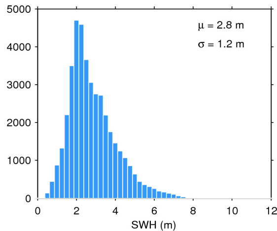
Figure 17. Histogram of flag-valid SWH over oceans and lakes for 05/01/2016. The mean ( \mu ) and standard deviation ( \sigma ) are also shown. Note that values larger than 12 m are excluded from the histogram for the sake of readability but not from the computation of \mu and \sigma .
