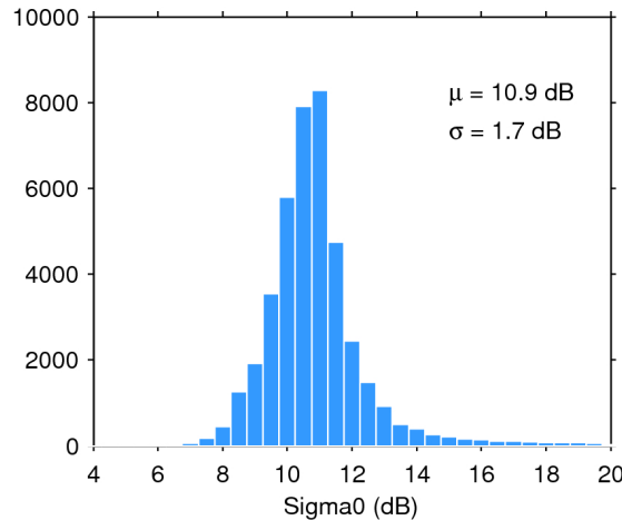
Figure 25. Histogram of flag-valid sigma0 over oceans and lakes for 05/01/2016. The mean ( \mu ) and standard deviation ( \sigma ) are also shown. Note that values outside [4 20] dB are excluded from the histogram for the sake of readability but not from the computation of \mu and \sigma .
