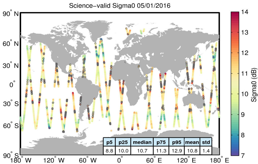
Figure 27. Geographical distribution of science-valid sigma0 data over oceans and lakes for 05/01/2016. The statistical values shown in the table refer to the sigma0 in dB and are calculated over all measurements shown in the figure. Gray circles denote records that have been rejected based on the editing criteria described in Table 4.
