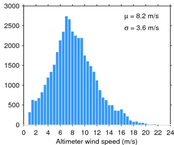
Figure 35. Histogram of science-valid wind over oceans and lakes for 05/01/2016. The mean ( \mu ) and standard deviation ( \sigma ) are also shown. Note that values larger than 24 m/s are excluded from the histogram for the sake of readability but not from the computation of \mu and \sigma .
