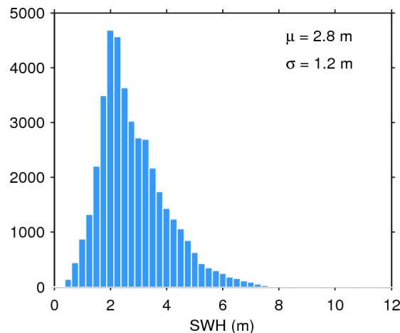
Figure 20. Histogram of science-valid SWH over oceans and lakes for 05/01/2016. The mean ( \mu ) and standard deviation ( \sigma ) are also shown. Note that values larger than 12 m are excluded from the histogram for the sake of readability but not from the computation of \mu and \sigma .
