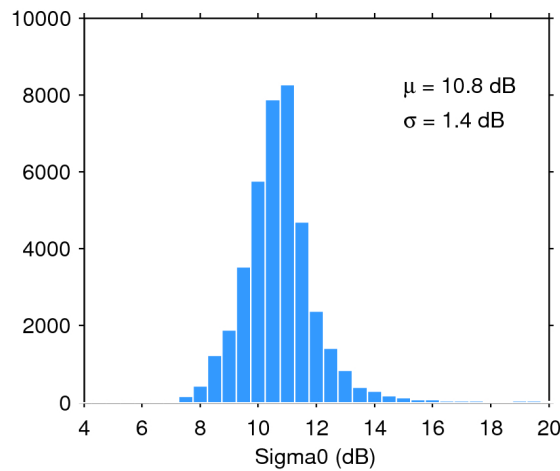
Figure 28. Histogram of science-valid sigma0 over oceans and lakes for 05/01/2016. The mean ( \mu ) and standard deviation ( \sigma ) are also shown. Note that values outside [4 20] dB are excluded from the histogram for the sake of readability but not from the computation of \mu and \sigma .
