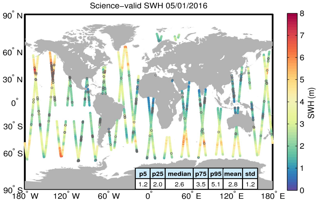
Figure 19. Geographical distribution of science-valid SWH data over oceans and lakes for 05/01/2016. The statistical values shown in the table refer to the SWH in m and are calculated over all measurements shown in the figure. Gray circles denote records that have been rejected based on the editing criteria described in Table 3.
