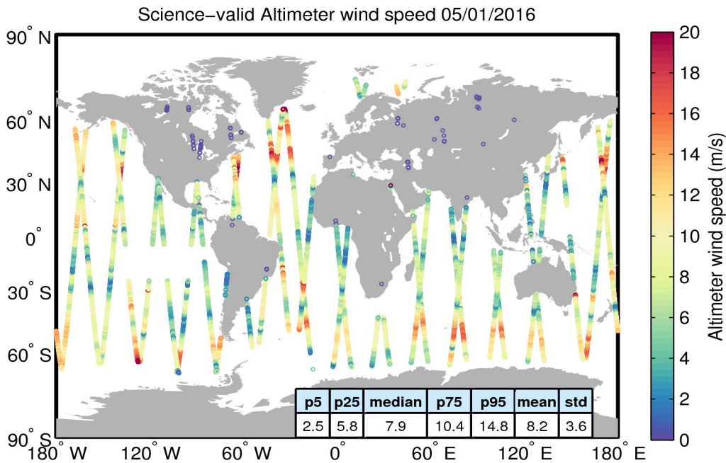
Figure 34. Geographical distribution of science-valid wind data over oceans and lakes for 05/01/2016. The statistical values shown in the table refer to the wind in m/s and are calculated over all measurements shown in the figure. Gray circles denote records that have been rejected based on the editing criteria described in Table 5.
