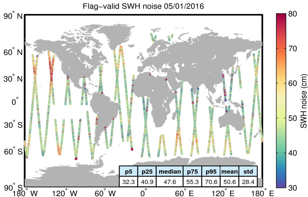
Figure 18. Geographical distribution of flag-valid 20-Hz SWH measurement noise over oceans and lakes for 05/01/2016. The statistical values shown in the figure refer to the SWH noise and are calculated over all measurements shown in the figure.
