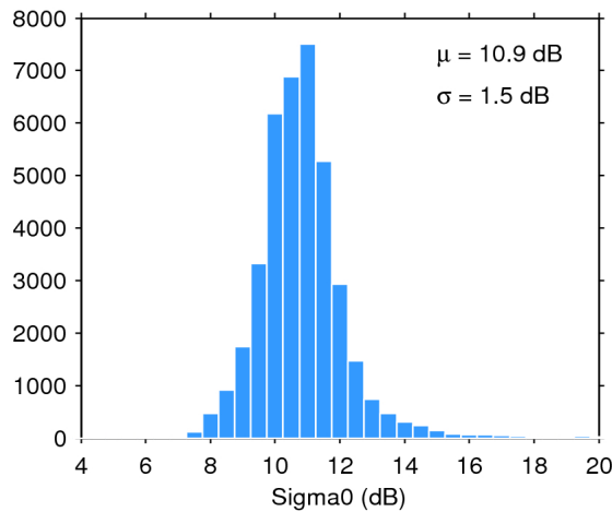
Figure 28. Histogram of science-valid sigma0 over oceans and lakes for 04/01/2016. The mean ( \mu ) and standard deviation ( \sigma ) are also shown. Note that values outside [4 20] dB are excluded from the histogram for the sake of readability but not from the computation of \mu and \sigma .
