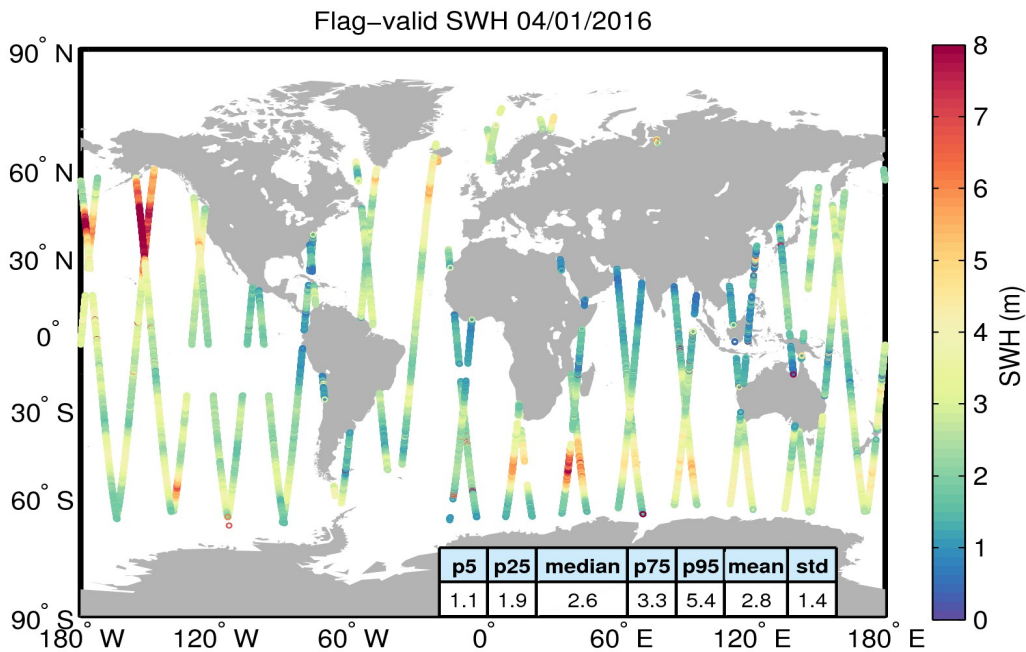
Figure 15. Geographical distribution of flag-valid SWH data over oceans and lakes for 04/01/2016. The statistical values shown in the table refer to the SWH in m and are calculated over all measurements shown in the figure.
