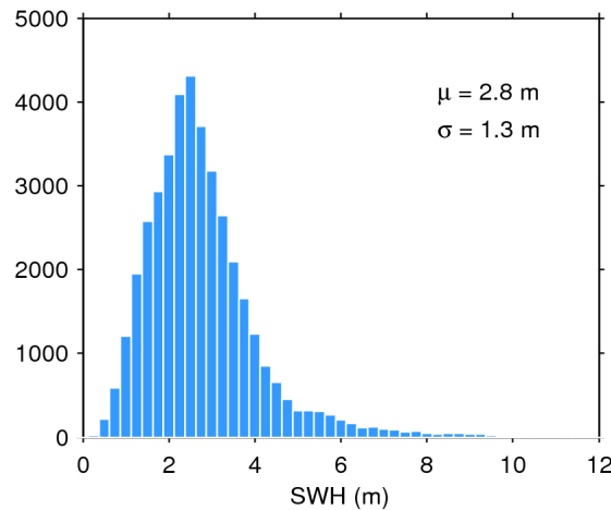
Figure 20. Histogram of science-valid SWH over oceans and lakes for 04/01/2016. The mean ( \mu ) and standard deviation ( \sigma ) are also shown. Note that values larger than 12 m are excluded from the histogram for the sake of readability but not from the computation of \mu and \sigma .
