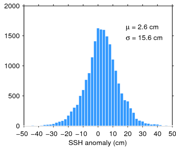
Figure 7. Histogram of flag-valid SSH anomaly over oceans and lakes for 04/01/2016. The mean ( \mu ) and standard deviation ( \sigma ) are also shown. Note that values outside [-50\ 50] cm are excluded from the histogram for the sake of readability but not from the computation of \mu and \sigma .
