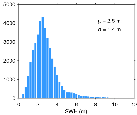
Figure 17. Histogram of flag-valid SWH over oceans and lakes for 04/01/2016. The mean ( \mu ) and standard deviation ( \sigma ) are also shown. Note that values larger than 12 m are excluded from the histogram for the sake of readability but not from the computation of \mu and \sigma .
