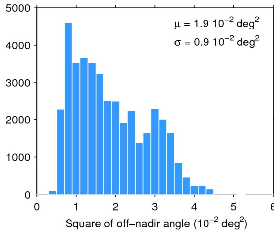
Figure 39. Histogram of flag-valid mispointing over oceans and lakes for 04/01/2016. The mean ( \mu ) and standard deviation ( \sigma ) are also shown. Note that values larger than 6 \cdot 10^{-2} \text{ deg}^2 are excluded from the histogram for the sake of readability but not from the computation of \mu and \sigma .
