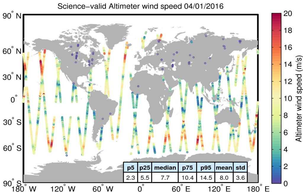
Figure 34. Geographical distribution of science-valid wind data over oceans and lakes for 04/01/2016. The statistical values shown in the table refer to the wind in m/s and are calculated over all measurements shown in the figure. Gray circles denote records that have been rejected based on the editing criteria described in Table 5.
