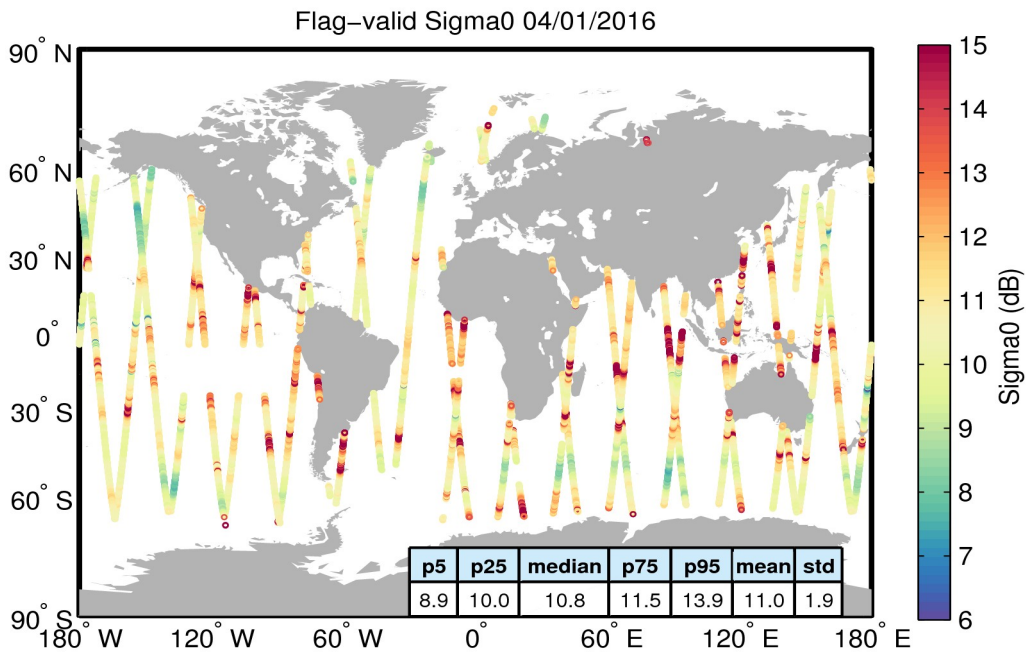
Figure 23. Geographical distribution of flag-valid sigma0 data over oceans and lakes for 04/01/2016. The statistical values shown in the table refer to the sigma0 in dB and are calculated over all measurements shown in the figure.
