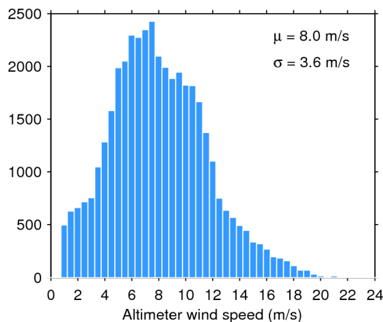
Figure 35. Histogram of science-valid wind over oceans and lakes for 04/01/2016. The mean ( \mu ) and standard deviation ( \sigma ) are also shown. Note that values larger than 24 m/s are excluded from the histogram for the sake of readability but not from the computation of \mu and \sigma .
