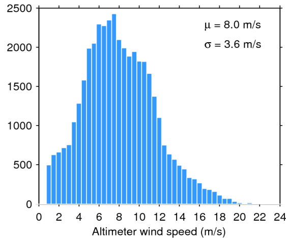
Figure 33. Histogram of flag-valid wind over oceans and lakes for 04/01/2016. The mean ( \mu ) and standard deviation ( \sigma ) are also shown. Note that values larger than 24 m/s are excluded from the histogram for the sake of readability but not from the computation of \mu and \sigma .
