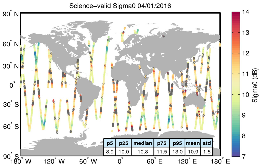
Figure 27. Geographical distribution of science-valid sigma0 data over oceans and lakes for 04/01/2016. The statistical values shown in the table refer to the sigma0 in dB and are calculated over all measurements shown in the figure. Gray circles denote records that have been rejected based on the editing criteria described in Table 4.
