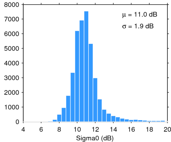
Figure 25. Histogram of flag-valid sigma0 over oceans and lakes for 04/01/2016. The mean ( \mu ) and standard deviation ( \sigma ) are also shown. Note that values outside [4 20] dB are excluded from the histogram for the sake of readability but not from the computation of \mu and \sigma .
