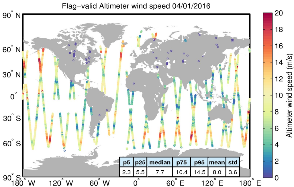
Figure 31. Geographical distribution of flag-valid wind data over oceans and lakes for 04/01/2016. The statistical values shown in the table refer to the wind in m/s and are calculated over all measurements shown in the figure.
