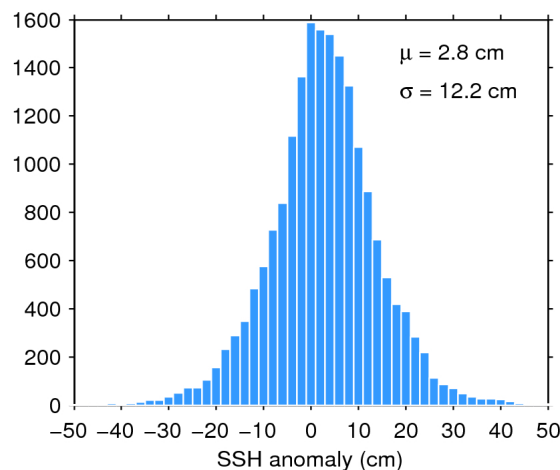
Figure 11. Histogram of science-valid SSH anomaly over oceans and lakes for 04/01/2016. The mean ( \mu ) and standard deviation ( \sigma ) are also shown. Note that values outside [-50 50] cm are excluded from the histogram for the sake of readability but not from the computation of \mu and \sigma .
