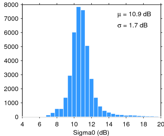
Figure 25. Histogram of flag-valid sigma0 over oceans and lakes for 03/01/2016. The mean ( \mu ) and standard deviation ( \sigma ) are also shown. Note that values outside [4 20] dB are excluded from the histogram for the sake of readability but not from the computation of \mu and \sigma .
