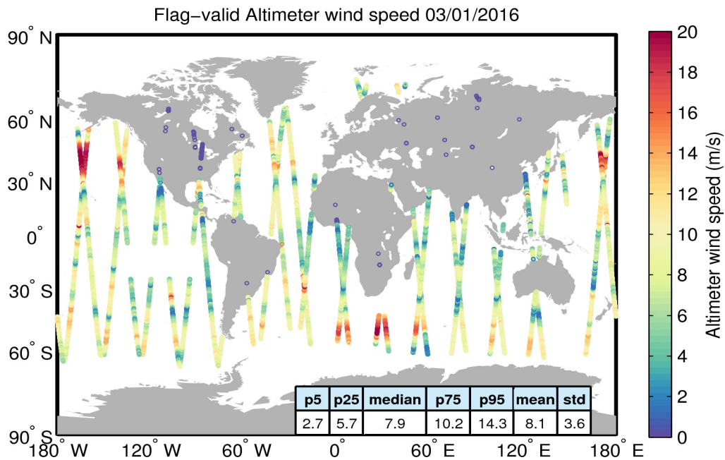
Figure 31. Geographical distribution of flag-valid wind data over oceans and lakes for 03/01/2016. The statistical values shown in the table refer to the wind in m/s and are calculated over all measurements shown in the figure.
