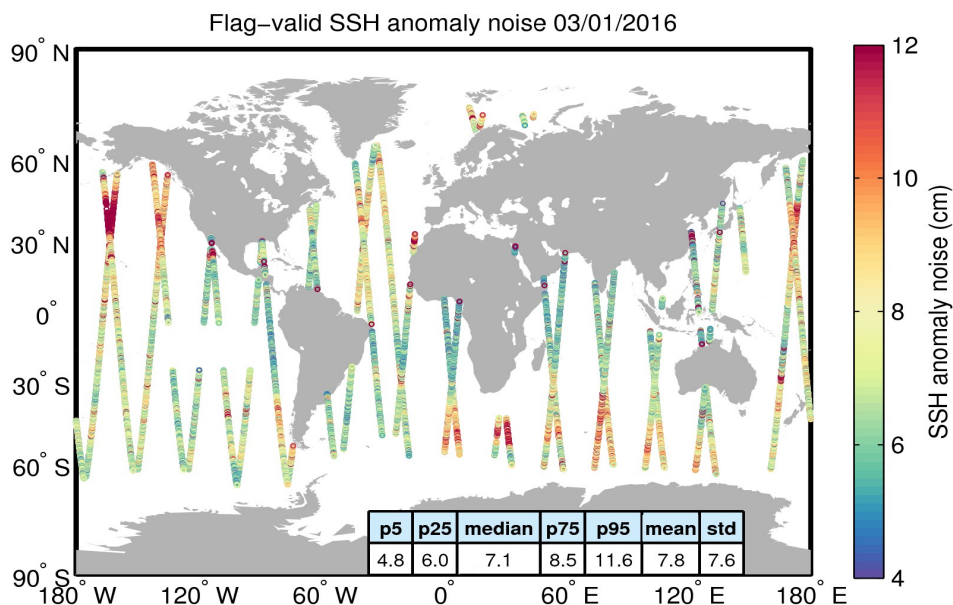
Figure 8. Geographical distribution of flag-valid 20-Hz SSH anomaly measurement noise over oceans and lakes for 03/01/2016. The statistical values shown in the table refer to the SSH anomaly noise and are calculated over all measurements shown in the figure.
