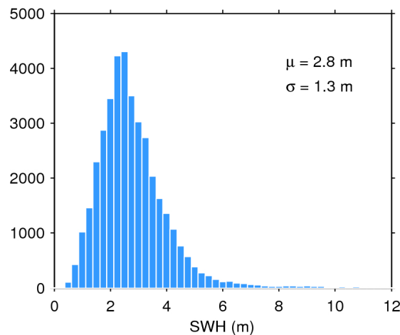
Figure 20. Histogram of science-valid SWH over oceans and lakes for 03/01/2016. The mean ( \mu ) and standard deviation ( \sigma ) are also shown. Note that values larger than 12 m are excluded from the histogram for the sake of readability but not from the computation of \mu and \sigma .
