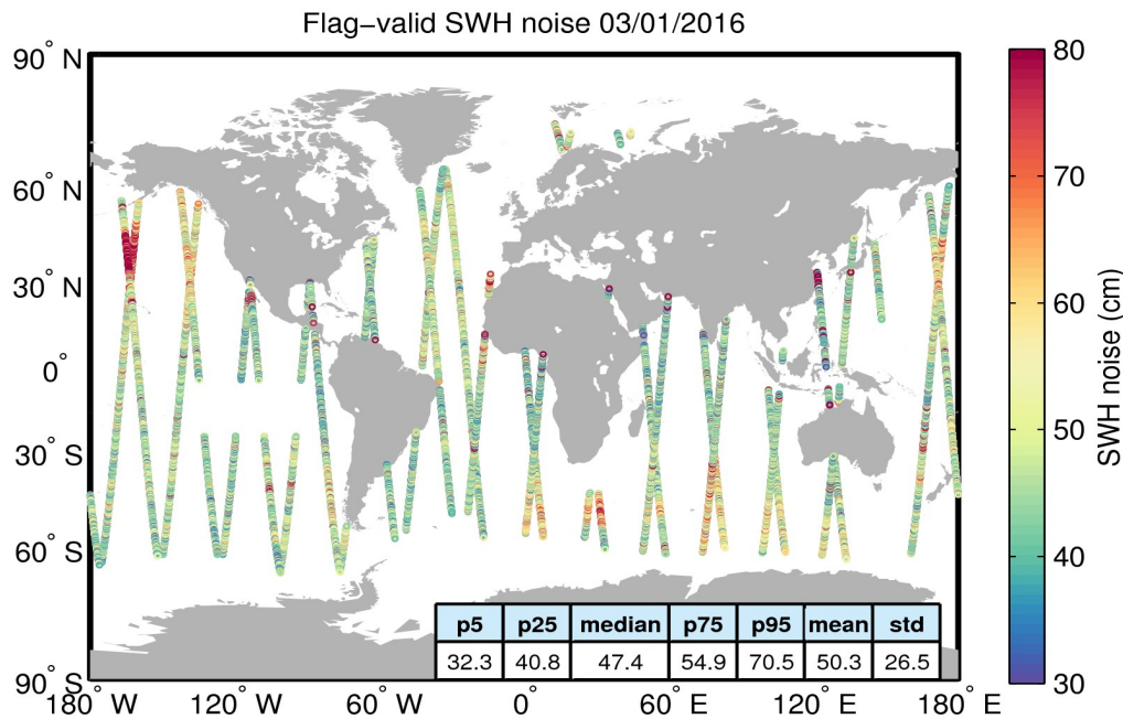
Figure 18. Geographical distribution of flag-valid 20-Hz SWH measurement noise over oceans and lakes for 03/01/2016. The statistical values shown in the figure refer to the SWH noise and are calculated over all measurements shown in the figure.
