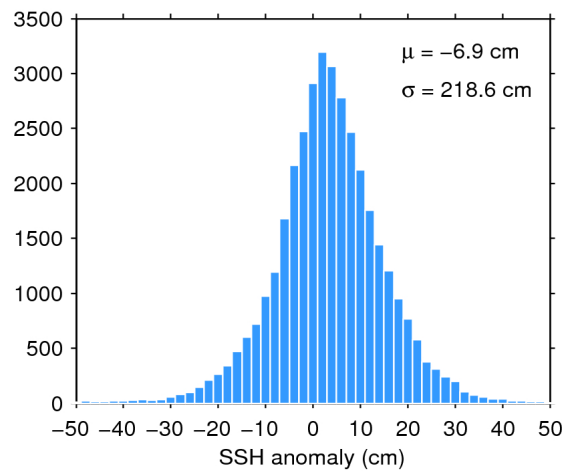
Figure 7. Histogram of flag-valid SSH anomaly over oceans and lakes for 03/01/2016. The mean ( \mu ) and standard deviation ( \sigma ) are also shown. Note that values outside [-50\ 50] cm are excluded from the histogram for the sake of readability but not from the computation of \mu and \sigma .
