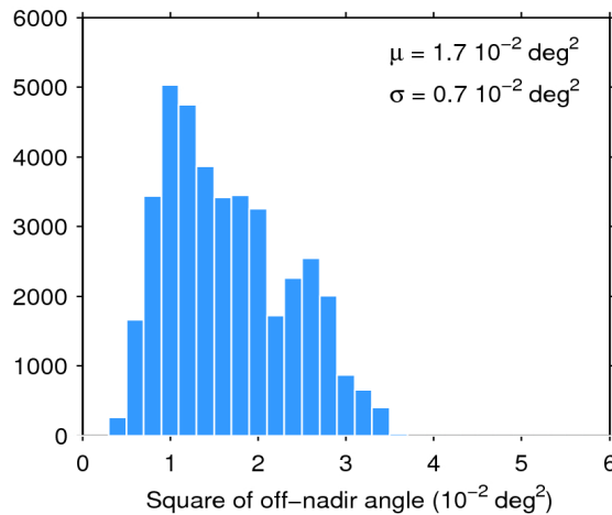
Figure 39. Histogram of flag-valid mispointing over oceans and lakes for 03/01/2016. The mean ( \mu ) and standard deviation ( \sigma ) are also shown. Note that values larger than 6 \cdot 10^{-2} \text{ deg}^2 are excluded from the histogram for the sake of readability but not from the computation of \mu and \sigma .
