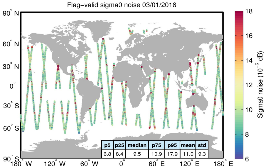
Figure 26. Geographical distribution of flag-valid 20-Hz sigma0 measurement noise over oceans and lakes for 03/01/2016. The statistical values shown in the table refer to the sigma0 noise and are calculated over all measurements shown in the figure.
