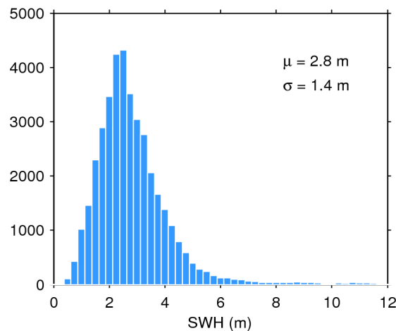
Figure 17. Histogram of flag-valid SWH over oceans and lakes for 03/01/2016. The mean ( \mu ) and standard deviation ( \sigma ) are also shown. Note that values larger than 12 m are excluded from the histogram for the sake of readability but not from the computation of \mu and \sigma .
