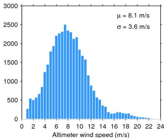
Figure 35. Histogram of science-valid wind over oceans and lakes for 03/01/2016. The mean ( \mu ) and standard deviation ( \sigma ) are also shown. Note that values larger than 24 m/s are excluded from the histogram for the sake of readability but not from the computation of \mu and \sigma .
