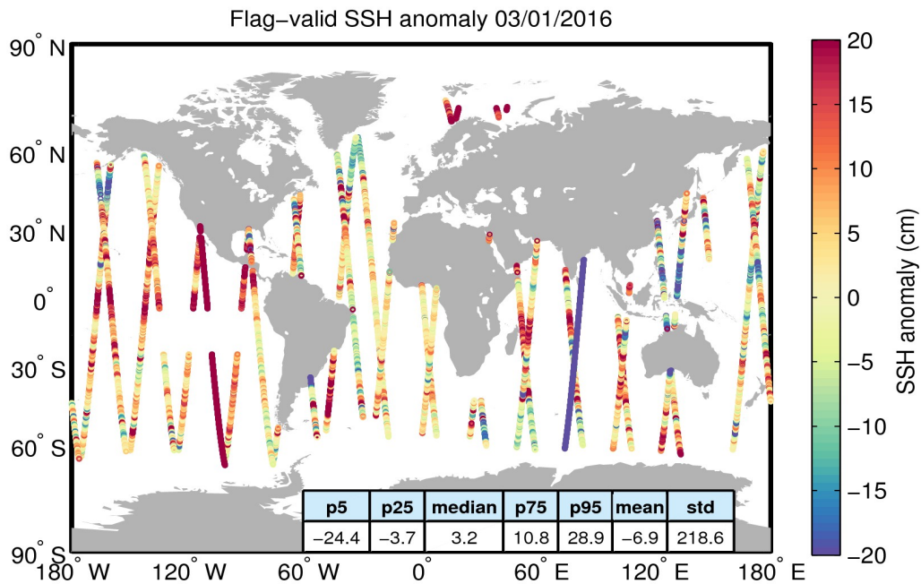
Figure 5. Geographical distribution of flag-valid 1-Hz SSH anomaly data over oceans and lakes for 03/01/2016. The statistical values shown in the table refer to the SSH anomaly in cm and are calculated over all measurements shown in the figure.
