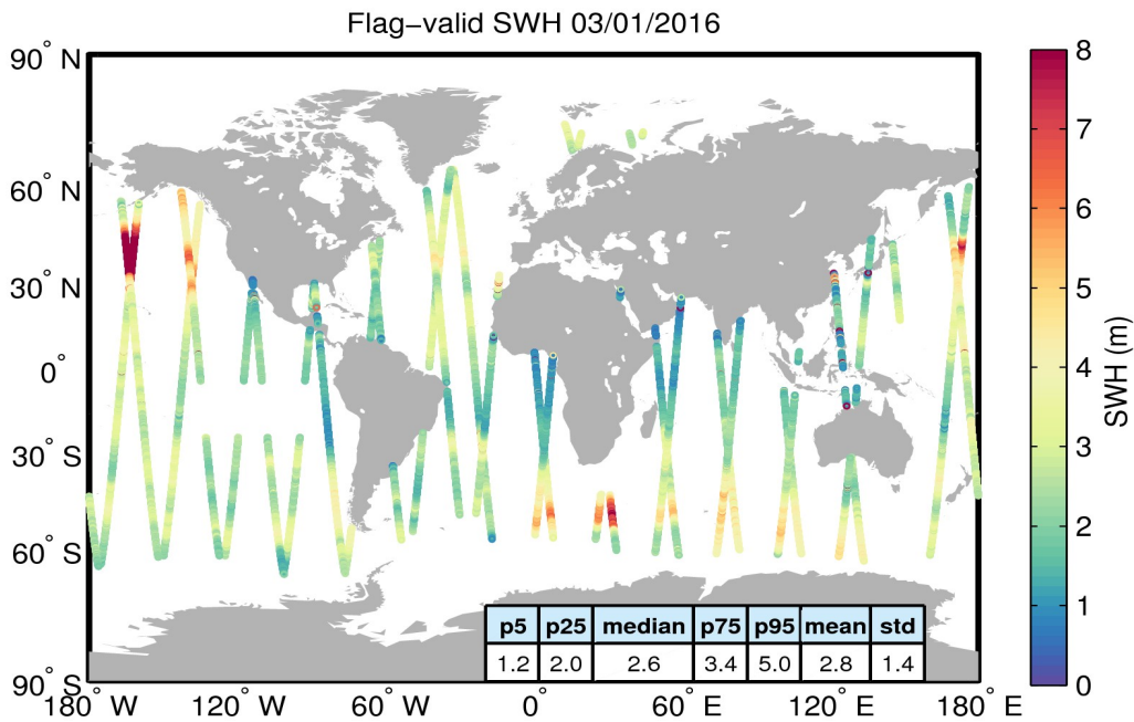
Figure 15. Geographical distribution of flag-valid SWH data over oceans and lakes for 03/01/2016. The statistical values shown in the table refer to the SWH in m and are calculated over all measurements shown in the figure.
