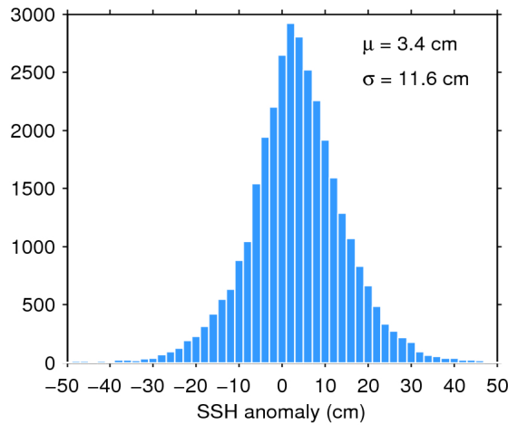
Figure 11. Histogram of science-valid SSH anomaly over oceans and lakes for 03/01/2016. The mean ( \mu ) and standard deviation ( \sigma ) are also shown. Note that values outside [-50 50] cm are excluded from the histogram for the sake of readability but not from the computation of \mu and \sigma .
