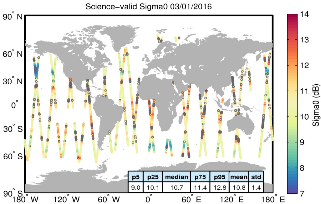
Figure 27. Geographical distribution of science-valid sigma0 data over oceans and lakes for 03/01/2016. The statistical values shown in the table refer to the sigma0 in dB and are calculated over all measurements shown in the figure. Gray circles denote records that have been rejected based on the editing criteria described in Table 4.
