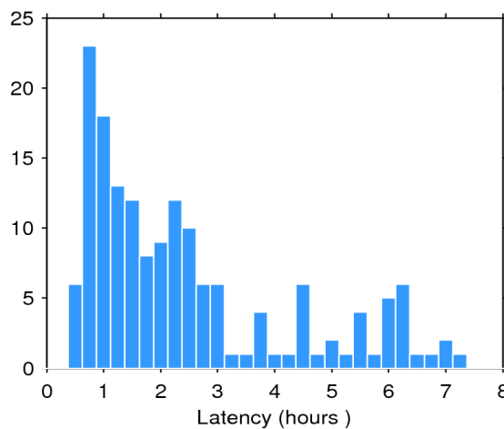
Figure 2. Histogram of the data latency for 03/01/2016. The y-axis denotes the number of files that are made available with a delay of x-hours with respect to the mean time of the records stored in the file.
