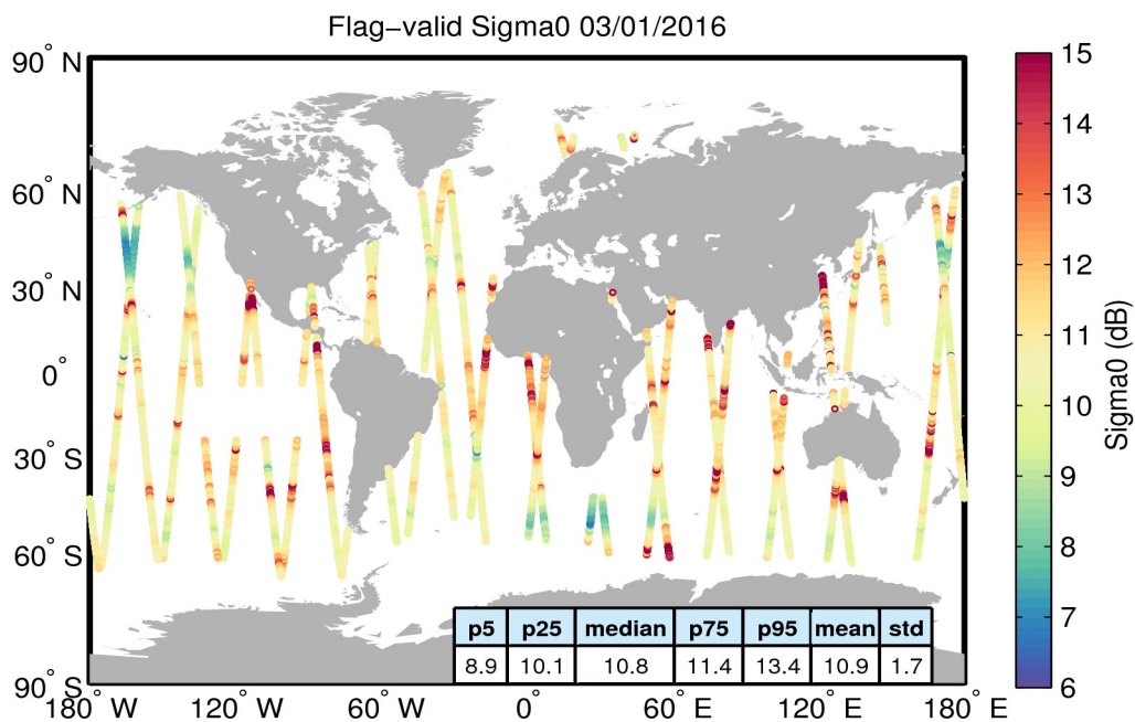
Figure 23. Geographical distribution of flag-valid sigma0 data over oceans and lakes for 03/01/2016. The statistical values shown in the table refer to the sigma0 in dB and are calculated over all measurements shown in the figure.
