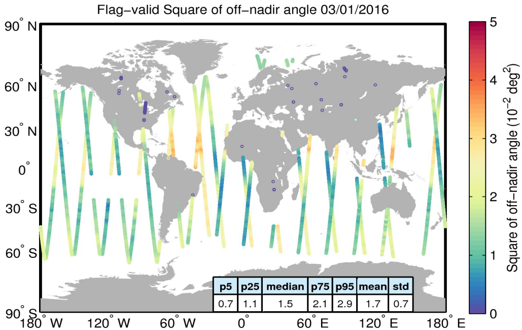
Figure 37. Geographical distribution of flag-valid mispointing data over oceans and lakes for 03/01/2016. The statistical values shown in the table refer to the mispointing in 10^{-2} \text{ deg}^2 and are calculated over all measurements shown in the figure.
