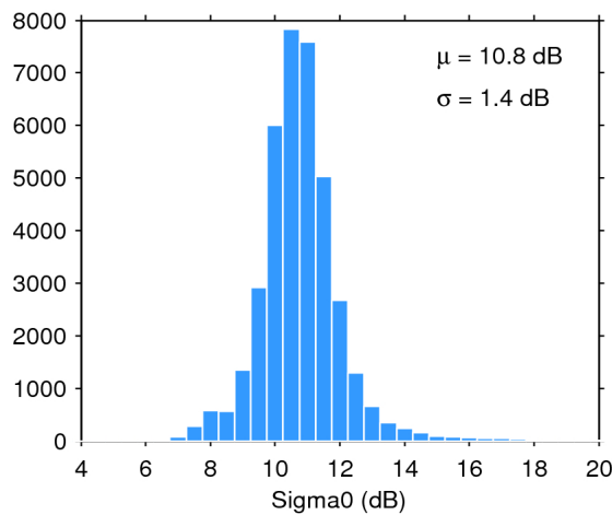
Figure 28. Histogram of science-valid sigma0 over oceans and lakes for 03/01/2016. The mean ( \mu ) and standard deviation ( \sigma ) are also shown. Note that values outside [4 20] dB are excluded from the histogram for the sake of readability but not from the computation of \mu and \sigma .
