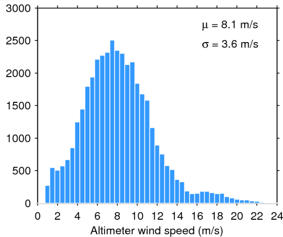
Figure 33. Histogram of flag-valid wind over oceans and lakes for 03/01/2016. The mean ( \mu ) and standard deviation ( \sigma ) are also shown. Note that values larger than 24 m/s are excluded from the histogram for the sake of readability but not from the computation of \mu and \sigma .
