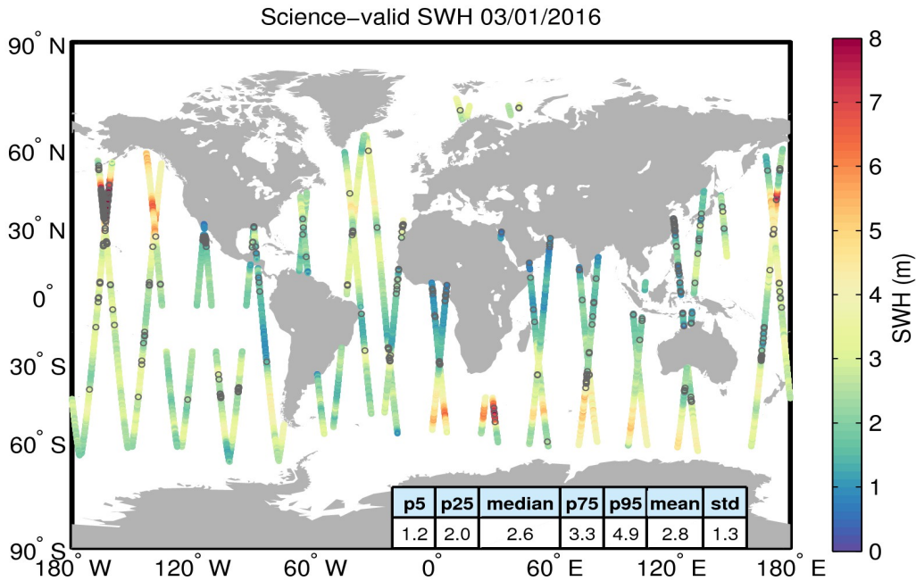
Figure 19. Geographical distribution of science-valid SWH data over oceans and lakes for 03/01/2016. The statistical values shown in the table refer to the SWH in m and are calculated over all measurements shown in the figure. Gray circles denote records that have been rejected based on the editing criteria described in Table 3.
