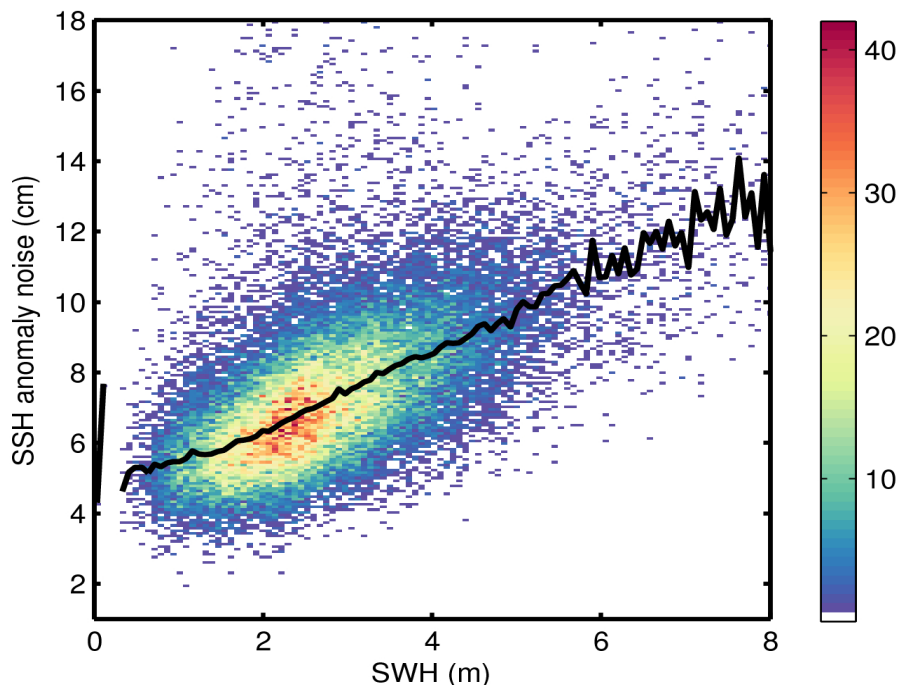
Figure 9. 2D histogram showing flag-valid SSH anomaly noise as a function of SWH for 03/01/2016. The black line denotes the median SSH anomaly noise as a function of SWH.
