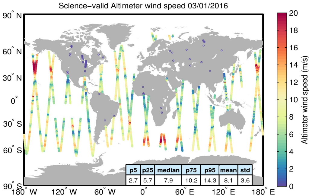
Figure 34. Geographical distribution of science-valid wind data over oceans and lakes for 03/01/2016. The statistical values shown in the table refer to the wind in m/s and are calculated over all measurements shown in the figure. Gray circles denote records that have been rejected based on the editing criteria described in Table 5.
