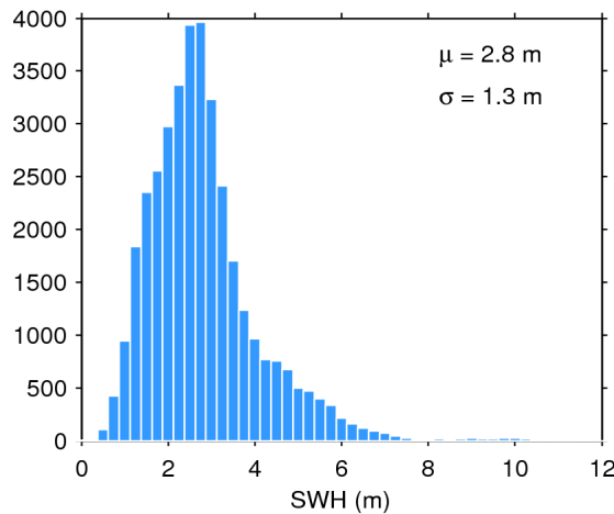
Figure 20. Histogram of science-valid SWH over oceans and lakes for 02/01/2016. The mean ( \mu ) and standard deviation ( \sigma ) are also shown. Note that values larger than 12 m are excluded from the histogram for the sake of readability but not from the computation of \mu and \sigma .
