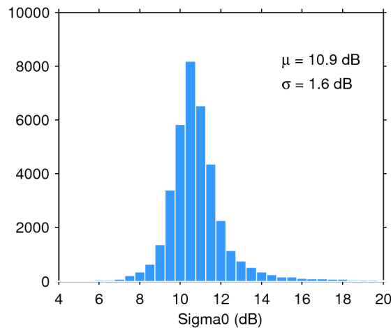
Figure 25. Histogram of flag-valid sigma0 over oceans and lakes for 02/01/2016. The mean ( \mu ) and standard deviation ( \sigma ) are also shown. Note that values outside [4 20] dB are excluded from the histogram for the sake of readability but not from the computation of \mu and \sigma .
