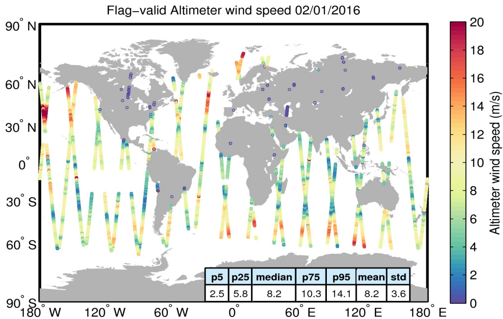
Figure 31. Geographical distribution of flag-valid wind data over oceans and lakes for 02/01/2016. The statistical values shown in the table refer to the wind in m/s and are calculated over all measurements shown in the figure.
