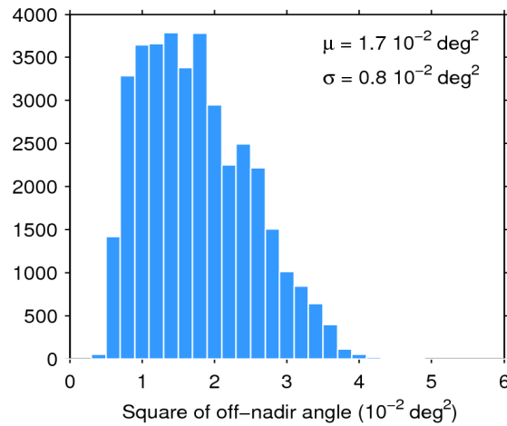
Figure 39. Histogram of flag-valid mispointing over oceans and lakes for 02/01/2016. The mean ( \mu ) and standard deviation ( \sigma ) are also shown. Note that values larger than 6 \cdot 10^{-2} \text{ deg}^2 are excluded from the histogram for the sake of readability but not from the computation of \mu and \sigma .
