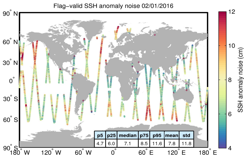
Figure 8. Geographical distribution of flag-valid 20-Hz SSH anomaly measurement noise over oceans and lakes for 02/01/2016. The statistical values shown in the table refer to the SSH anomaly noise and are calculated over all measurements shown in the figure.
