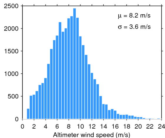
Figure 35. Histogram of science-valid wind over oceans and lakes for 02/01/2016. The mean ( \mu ) and standard deviation ( \sigma ) are also shown. Note that values larger than 24 m/s are excluded from the histogram for the sake of readability but not from the computation of \mu and \sigma .
