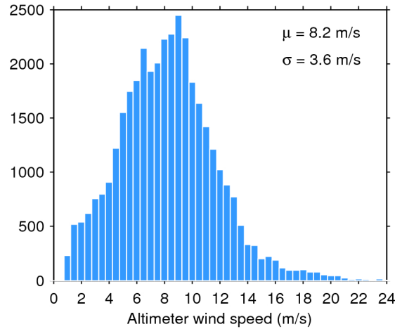
Figure 33. Histogram of flag-valid wind over oceans and lakes for 02/01/2016. The mean ( \mu ) and standard deviation ( \sigma ) are also shown. Note that values larger than 24 m/s are excluded from the histogram for the sake of readability but not from the computation of \mu and \sigma .
