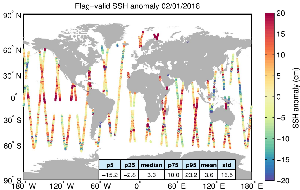
Figure 5. Geographical distribution of flag-valid 1-Hz SSH anomaly data over oceans and lakes for 02/01/2016. The statistical values shown in the table refer to the SSH anomaly in cm and are calculated over all measurements shown in the figure.
