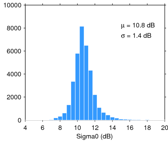
Figure 28. Histogram of science-valid sigma0 over oceans and lakes for 02/01/2016. The mean ( \mu ) and standard deviation ( \sigma ) are also shown. Note that values outside [4 20] dB are excluded from the histogram for the sake of readability but not from the computation of \mu and \sigma .
