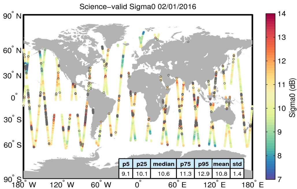
Figure 27. Geographical distribution of science-valid sigma0 data over oceans and lakes for 02/01/2016. The statistical values shown in the table refer to the sigma0 in dB and are calculated over all measurements shown in the figure. Gray circles denote records that have been rejected based on the editing criteria described in Table 4.
