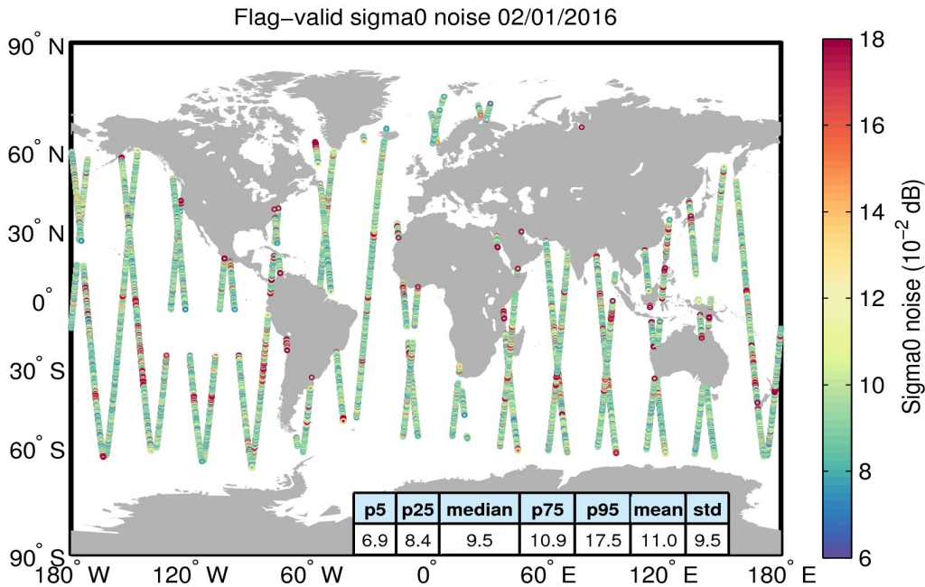
Figure 26. Geographical distribution of flag-valid 20-Hz sigma0 measurement noise over oceans and lakes for 02/01/2016. The statistical values shown in the table refer to the sigma0 noise and are calculated over all measurements shown in the figure.
