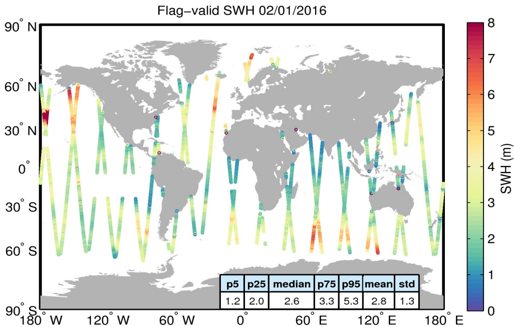
Figure 15. Geographical distribution of flag-valid SWH data over oceans and lakes for 02/01/2016. The statistical values shown in the table refer to the SWH in m and are calculated over all measurements shown in the figure.
