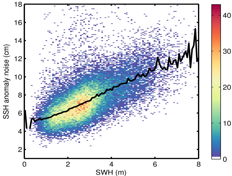
Figure 9. 2D histogram showing flag-valid SSH anomaly noise as a function of SWH for 02/01/2016. The black line denotes the median SSH anomaly noise as a function of SWH.
