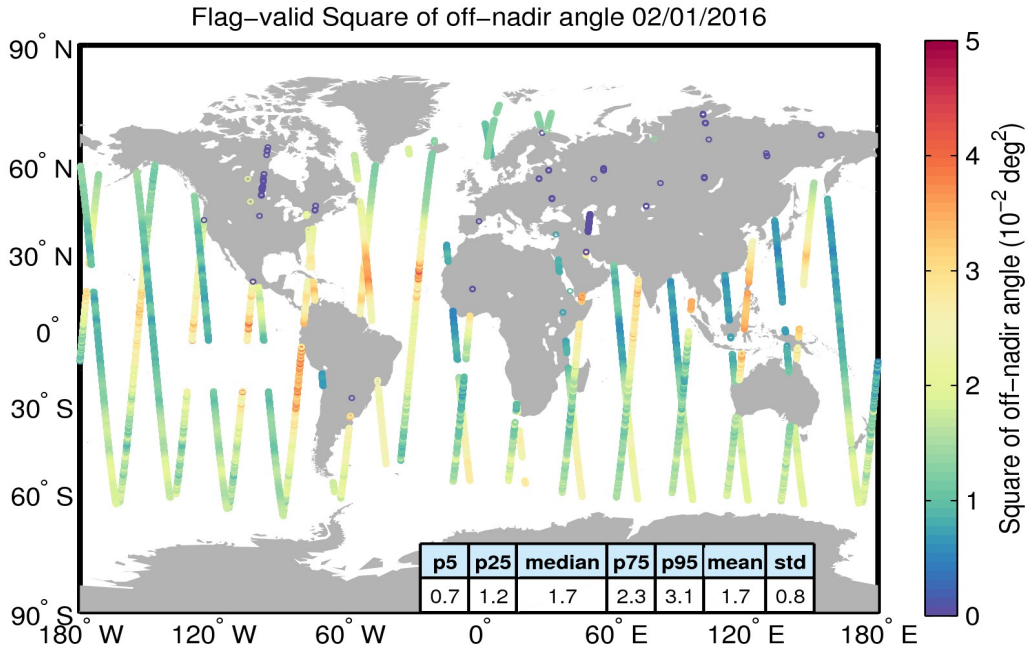
Figure 37. Geographical distribution of flag-valid mispointing data over oceans and lakes for 02/01/2016. The statistical values shown in the table refer to the mispointing in 10^{-2} \text{ deg}^2 and are calculated over all measurements shown in the figure.
