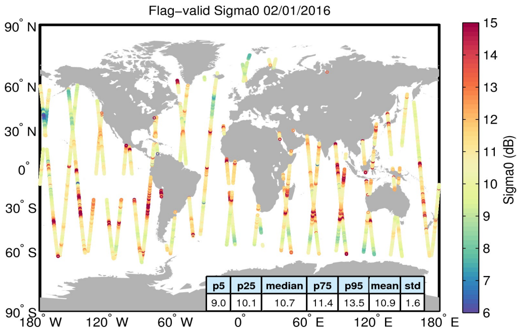
Figure 23. Geographical distribution of flag-valid sigma0 data over oceans and lakes for 02/01/2016. The statistical values shown in the table refer to the sigma0 in dB and are calculated over all measurements shown in the figure.
