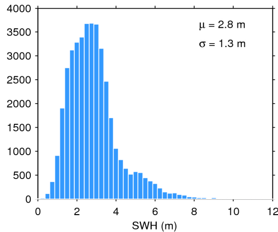
Figure 20. Histogram of science-valid SWH over oceans and lakes for 01/01/2016. The mean ( \mu ) and standard deviation ( \sigma ) are also shown. Note that values larger than 12 m are excluded from the histogram for the sake of readability but not from the computation of \mu and \sigma .
