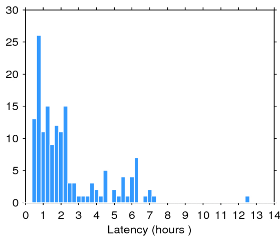
Figure 2. Histogram of the data latency for 01/01/2016. The y-axis denotes the number of files that are made available with a delay of x-hours with respect to the mean time of the records stored in the file.
