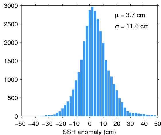
Figure 11. Histogram of science-valid SSH anomaly over oceans and lakes for 01/01/2016. The mean ( \mu ) and standard deviation ( \sigma ) are also shown. Note that values outside [-50 50] cm are excluded from the histogram for the sake of readability but not from the computation of \mu and \sigma .
