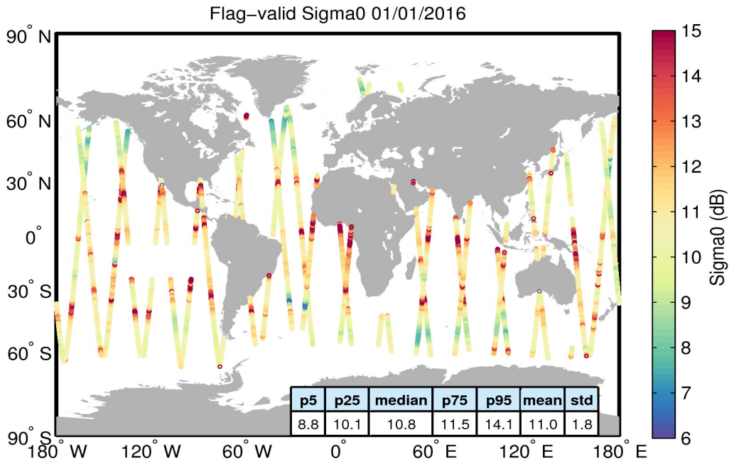
Figure 23. Geographical distribution of flag-valid sigma0 data over oceans and lakes for 01/01/2016. The statistical values shown in the table refer to the sigma0 in dB and are calculated over all measurements shown in the figure.
