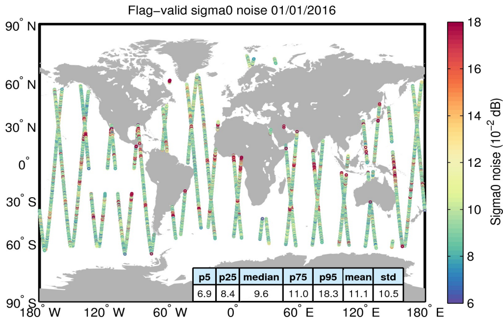
Figure 26. Geographical distribution of flag-valid 20-Hz sigma0 measurement noise over oceans and lakes for 01/01/2016. The statistical values shown in the figure refer to the sigma0 noise and are calculated over all measurements shown in the figure.
