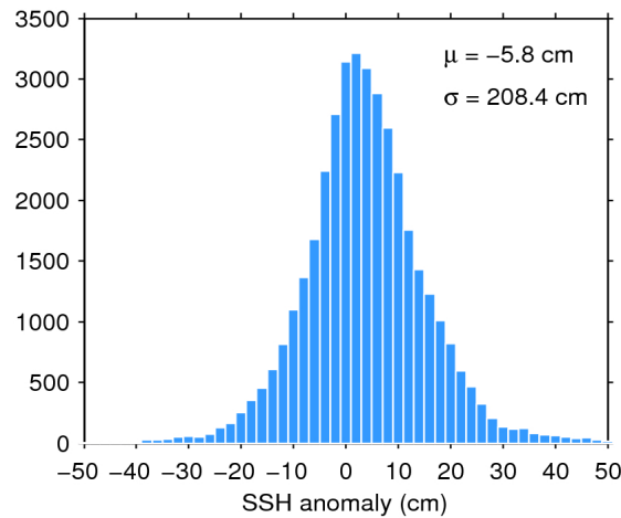
Figure 7. Histogram of flag-valid SSH anomaly over oceans and lakes for 01/01/2016. The mean ( \mu ) and standard deviation ( \sigma ) are also shown. Note that values outside [-50 50] cm are excluded from the histogram for the sake of readability but not from the computation of \mu and \sigma .
