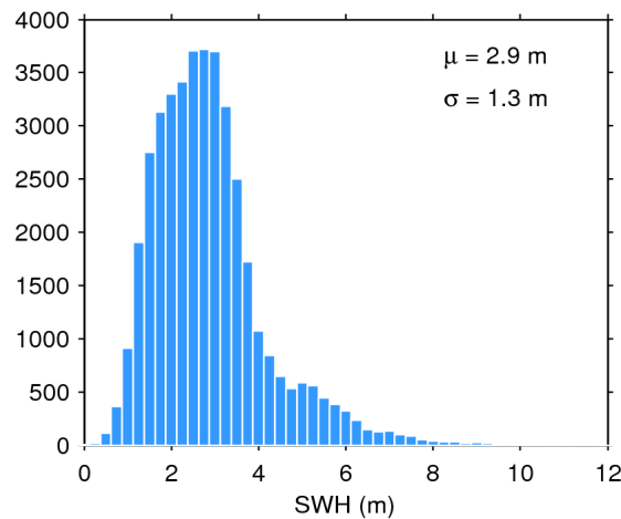
Figure 17. Histogram of flag-valid SWH over oceans and lakes for 01/01/2016. The mean ( \mu ) and standard deviation ( \sigma ) are also shown. Note that values larger than 12 m are excluded from the histogram for the sake of readability but not from the computation of \mu and \sigma .
