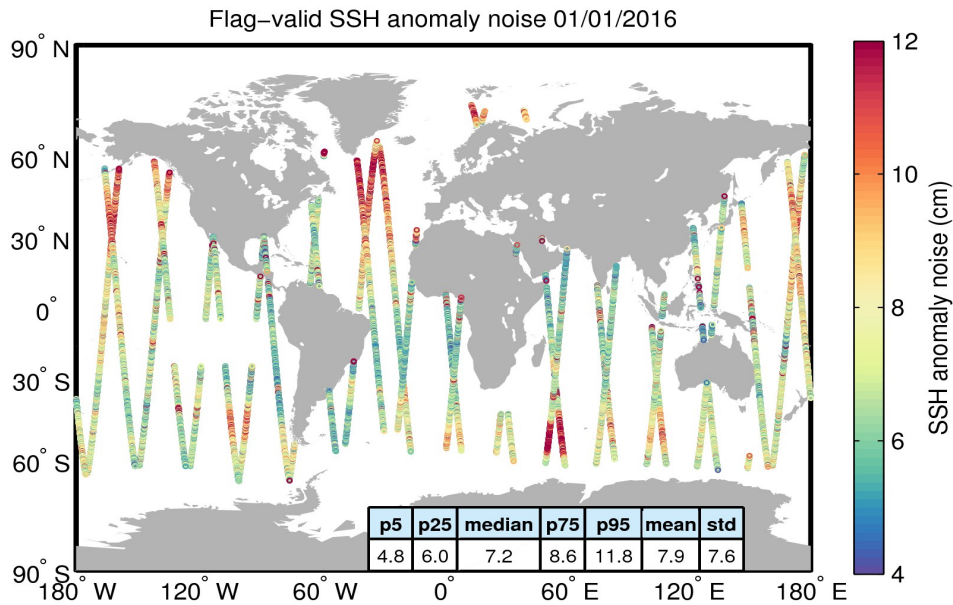
Figure 8. Geographical distribution of flag-valid 20-Hz SSH anomaly measurement noise over oceans and lakes for 01/01/2016. The statistical values shown in the table refer to the SSH anomaly noise and are calculated over all measurements shown in the figure.
