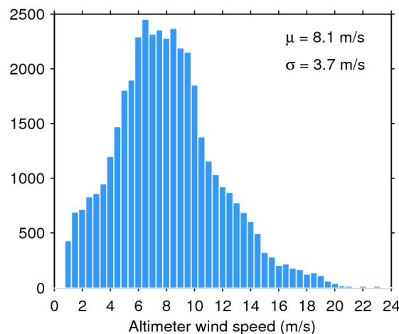
Figure 35. Histogram of science-valid wind over oceans and lakes for 01/01/2016. The mean ( \mu ) and standard deviation ( \sigma ) are also shown. Note that values larger than 24 m/s are excluded from the histogram for the sake of readability but not from the computation of \mu and \sigma .
