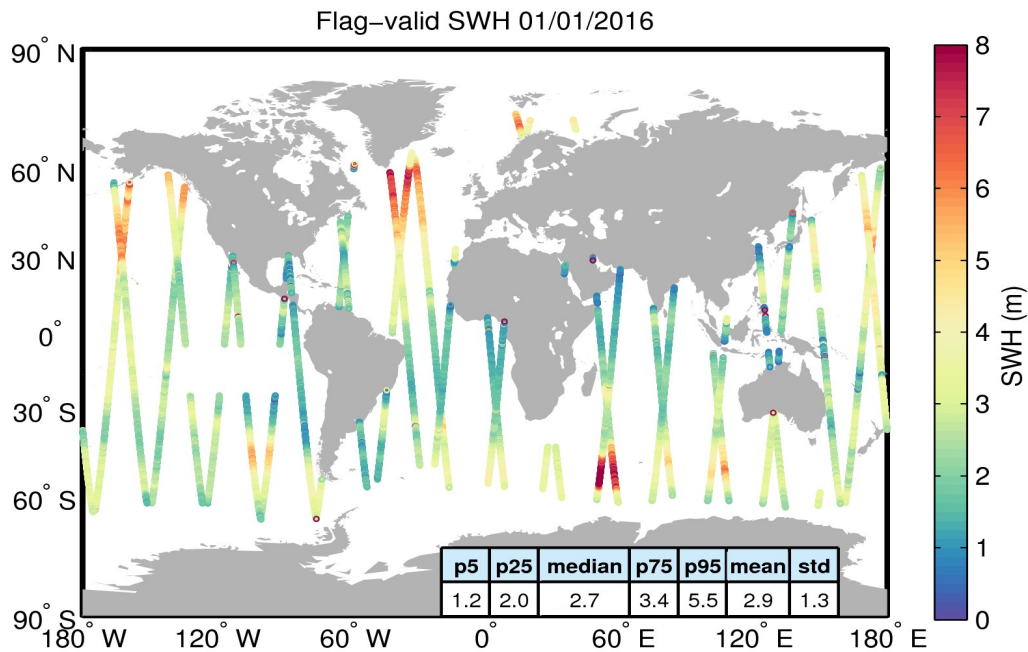
Figure 15. Geographical distribution of flag-valid SWH data over oceans and lakes for 01/01/2016. The statistical values shown in the table refer to the SWH in m and are calculated over all measurements shown in the figure.
