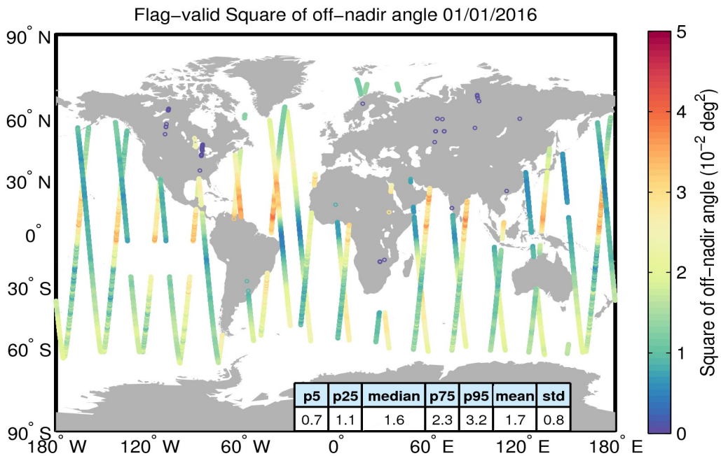
Figure 37. Geographical distribution of flag-valid mispointing data over oceans and lakes for 01/01/2016. The statistical values shown in the table refer to the mispointing in 10^{-2} \text{ deg}^2 and are calculated over all measurements shown in the figure.
