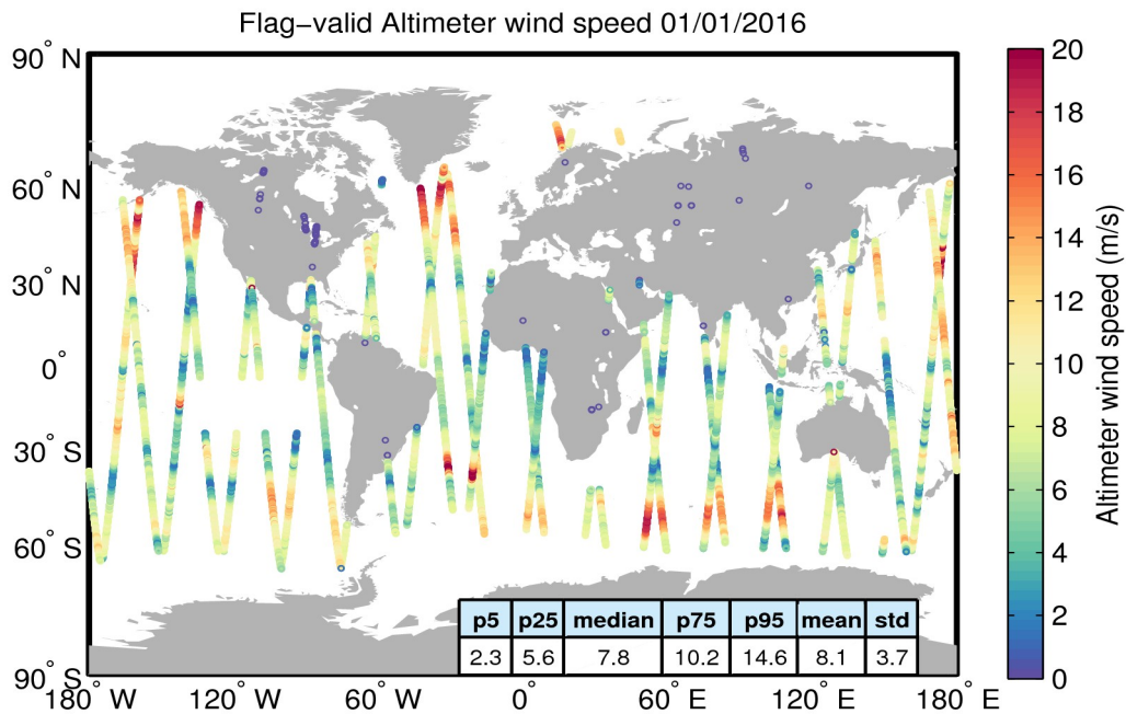
Figure 31. Geographical distribution of flag-valid wind data over oceans and lakes for 01/01/2016. The statistical values shown in the table refer to the wind in m/s and are calculated over all measurements shown in the figure.
