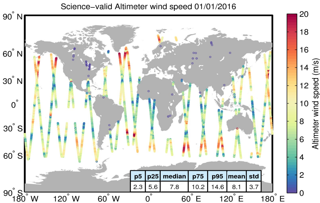
Figure 34. Geographical distribution of science-valid wind data over oceans and lakes for 01/01/2016. The statistical values shown in the table refer to the wind in m/s and are calculated over all measurements shown in the figure. Gray circles denote records that have been rejected based on the editing criteria described in Table 5.
