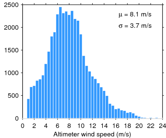
Figure 33. Histogram of flag-valid wind over oceans and lakes for 01/01/2016. The mean ( \mu ) and standard deviation ( \sigma ) are also shown. Note that values larger than 24 m/s are excluded from the histogram for the sake of readability but not from the computation of \mu and \sigma .
