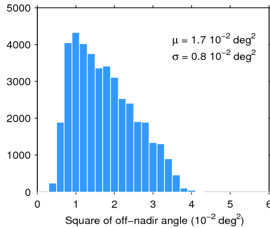
Figure 39. Histogram of flag-valid mispointing over oceans and lakes for 01/01/2016. The mean ( \mu ) and standard deviation ( \sigma ) are also shown. Note that values larger than 6 \cdot 10^{-2} \text{ deg}^2 are excluded from the histogram for the sake of readability but not from the computation of \mu and \sigma .
