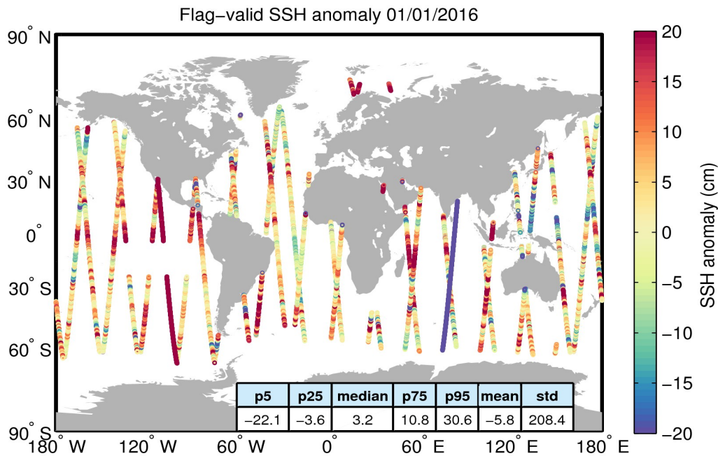
Figure 5. Geographical distribution of flag-valid 1-Hz SSH anomaly data over oceans and lakes for 01/01/2016. The statistical values shown in the table refer to the SSH anomaly in cm and are calculated over all measurements shown in the figure.
