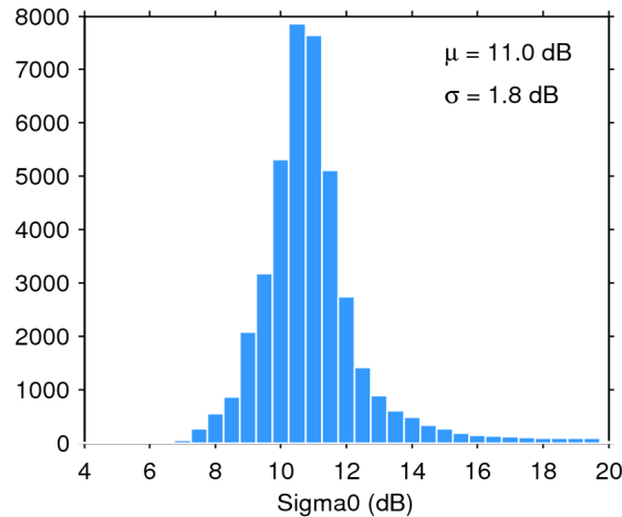
Figure 25. Histogram of flag-valid sigma0 over oceans and lakes for 01/01/2016. The mean ( \mu ) and standard deviation ( \sigma ) are also shown. Note that values outside [4 20] dB are excluded from the histogram for the sake of readability but not from the computation of \mu and \sigma .
