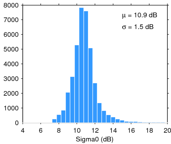
Figure 28. Histogram of science-valid sigma0 over oceans and lakes for 01/01/2016. The mean ( \mu ) and standard deviation ( \sigma ) are also shown. Note that values outside [4 20] dB are excluded from the histogram for the sake of readability but not from the computation of \mu and \sigma .
