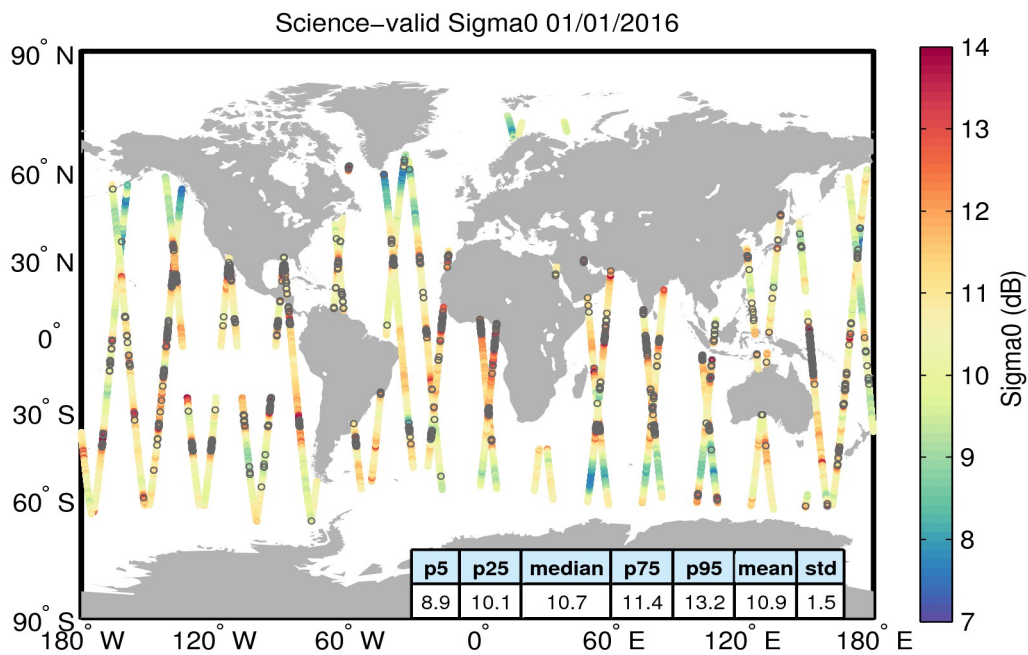
Figure 27. Geographical distribution of science-valid sigma0 data over oceans and lakes for 01/01/2016. The statistical values shown in the table refer to the sigma0 in dB and are calculated over all measurements shown in the figure. Gray circles denote records that have been rejected based on the editing criteria described in Table 4.
