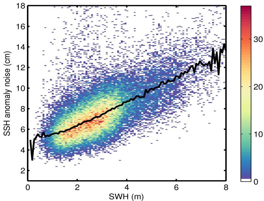
Figure 9. 2D histogram showing flag-valid SSH anomaly noise as a function of SWH for 01/01/2016. The black line denotes the median SSH anomaly noise as a function of SWH.
