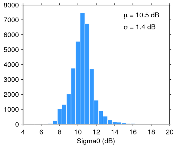
Figure 28. Histogram of science-valid sigma0 over oceans and lakes for 23/12/2015. The mean ( \mu ) and standard deviation ( \sigma ) are also shown. Note that values outside [4 20] dB are excluded from the histogram for the sake of readability but not from the computation of \mu and \sigma .
