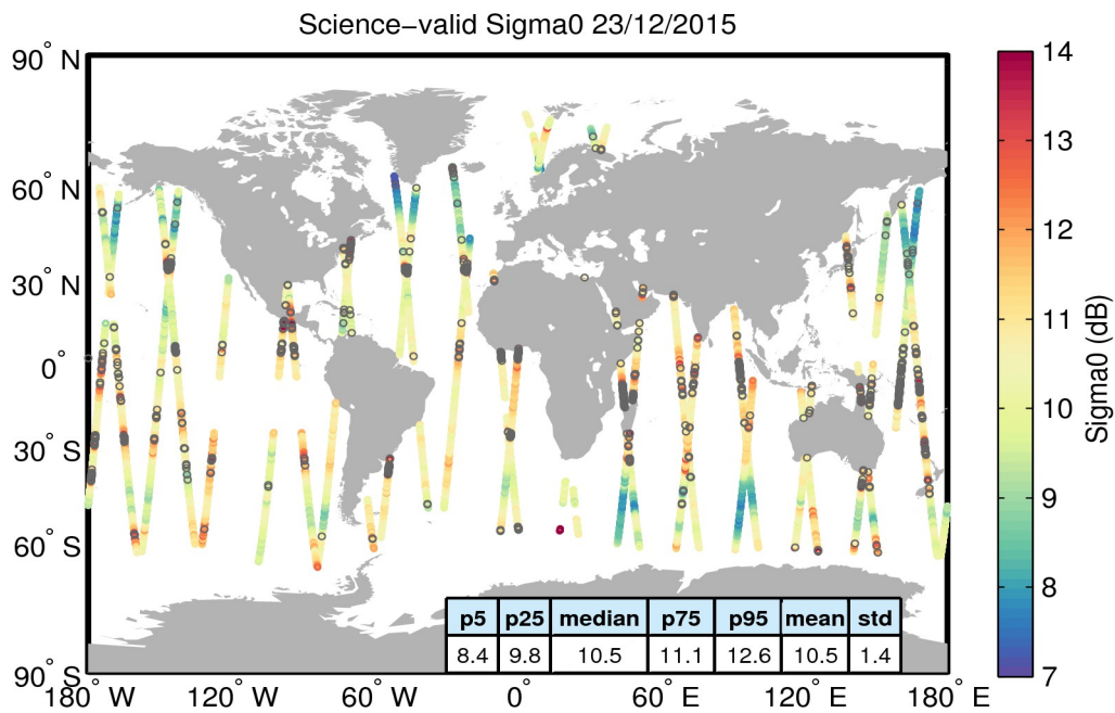
Figure 27. Geographical distribution of science-valid sigma0 data over oceans and lakes for 23/12/2015. The statistical values shown in the table refer to the sigma0 in dB and are calculated over all measurements shown in the figure. Gray circles denote records that have been rejected based on the editing criteria described in Table 4.
