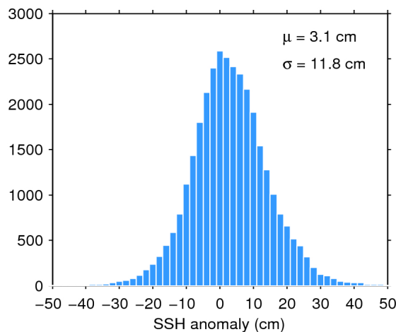
Figure 11. Histogram of science-valid SSH anomaly over oceans and lakes for 23/12/2015. The mean ( \mu ) and standard deviation ( \sigma ) are also shown. Note that values outside [-50 50] cm are excluded from the histogram for the sake of readability but not from the computation of \mu and \sigma .
