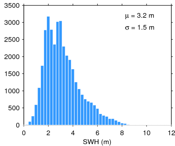
Figure 17. Histogram of flag-valid SWH over oceans and lakes for 23/12/2015. The mean ( \mu ) and standard deviation ( \sigma ) are also shown. Note that values larger than 12 m are excluded from the histogram for the sake of readability but not from the computation of \mu and \sigma .
