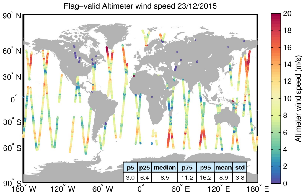
Figure 31. Geographical distribution of flag-valid wind data over oceans and lakes for 23/12/2015. The statistical values shown in the table refer to the wind in m/s and are calculated over all measurements shown in the figure.
