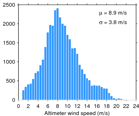
Figure 35. Histogram of science-valid wind over oceans and lakes for 23/12/2015. The mean ( \mu ) and standard deviation ( \sigma ) are also shown. Note that values larger than 24 m/s are excluded from the histogram for the sake of readability but not from the computation of \mu and \sigma .
