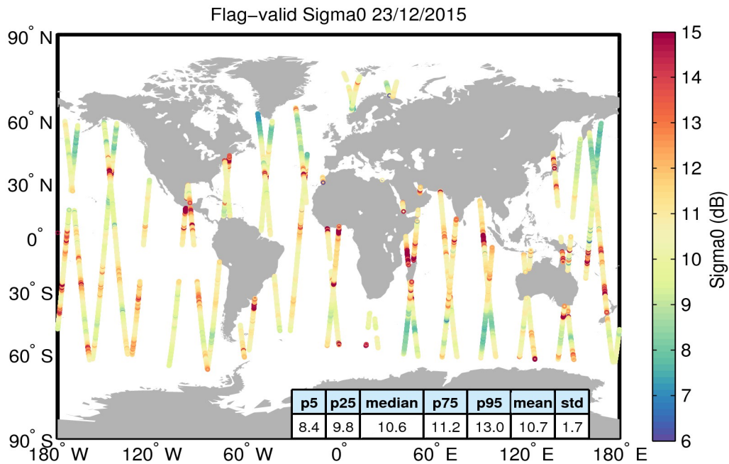
Figure 23. Geographical distribution of flag-valid sigma0 data over oceans and lakes for 23/12/2015. The statistical values shown in the table refer to the sigma0 in dB and are calculated over all measurements shown in the figure.
