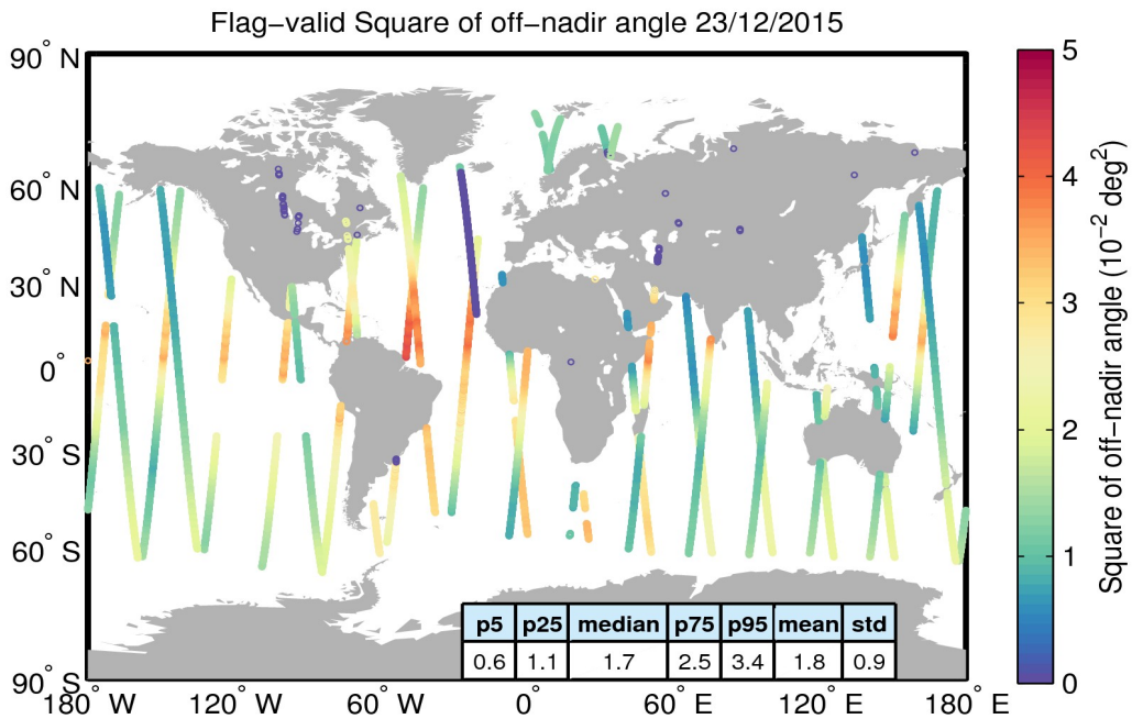
Figure 37. Geographical distribution of flag-valid mispointing data over oceans and lakes for 23/12/2015. The statistical values shown in the table refer to the mispointing in 10^{-2} \text{deg}^2 and are calculated over all measurements shown in the figure.
