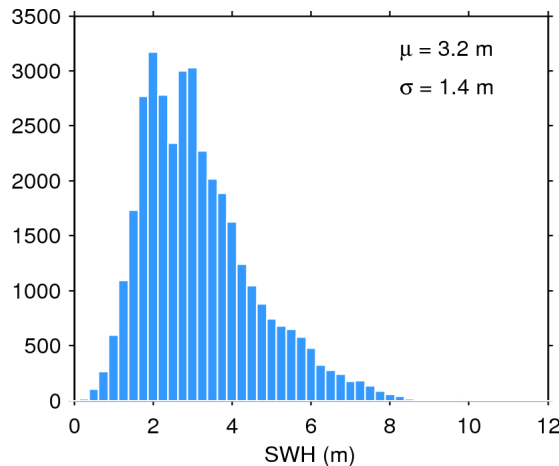
Figure 20. Histogram of science-valid SWH over oceans and lakes for 23/12/2015. The mean ( \mu ) and standard deviation ( \sigma ) are also shown. Note that values larger than 12 m are excluded from the histogram for the sake of readability but not from the computation of \mu and \sigma .
