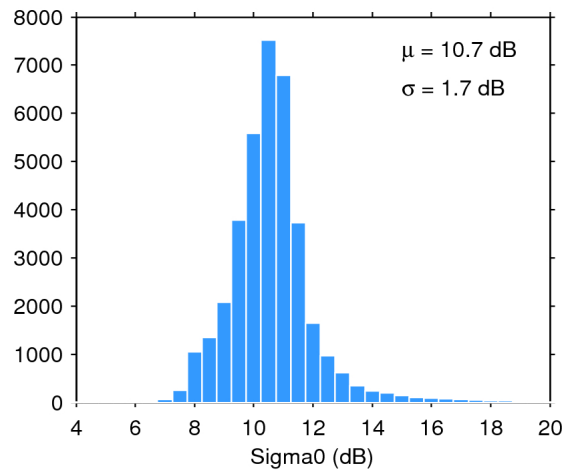
Figure 25. Histogram of flag-valid sigma0 over oceans and lakes for 23/12/2015. The mean ( \mu ) and standard deviation ( \sigma ) are also shown. Note that values outside [4 20] dB are excluded from the histogram for the sake of readability but not from the computation of \mu and \sigma .
