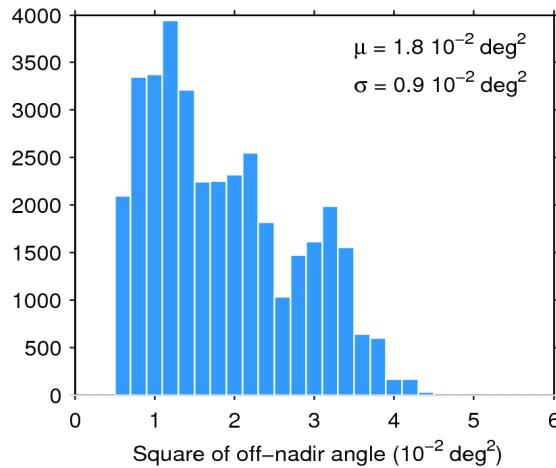
Figure 39. Histogram of flag-valid mispointing over oceans and lakes for 23/12/2015. The mean ( \mu ) and standard deviation ( \sigma ) are also shown. Note that values larger than 6 \cdot 10^{-2} \text{ deg}^2 are excluded from the histogram for the sake of readability but not from the computation of \mu and \sigma .
