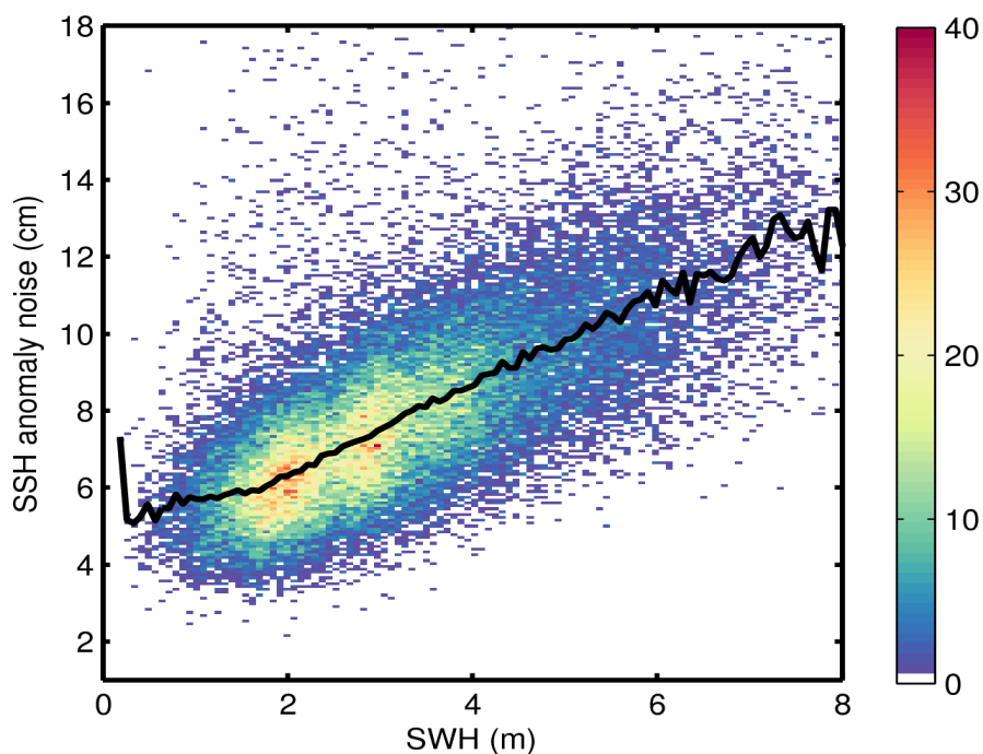
Figure 9. 2D histogram showing flag-valid SSH anomaly noise as a function of SWH for 23/12/2015. The black line denotes the median SSH anomaly noise as a function of SWH.
