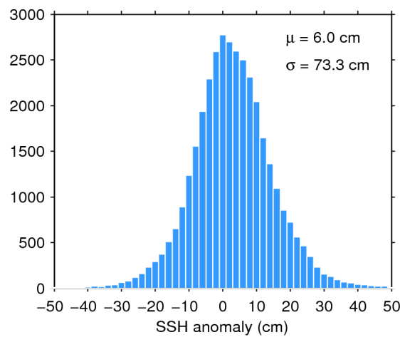
Figure 7. Histogram of flag-valid SSH anomaly over oceans and lakes for 23/12/2015. The mean ( \mu ) and standard deviation ( \sigma ) are also shown. Note that values outside [-50 50] cm are excluded from the histogram for the sake of readability but not from the computation of \mu and \sigma .
