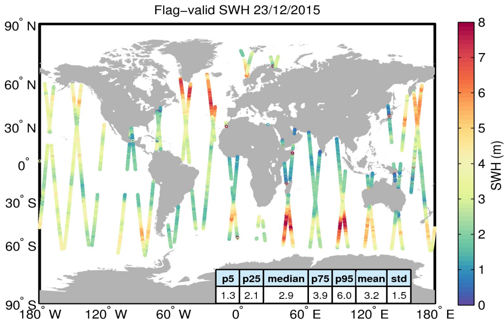
Figure 15. Geographical distribution of flag-valid SWH data over oceans and lakes for 23/12/2015. The statistical values shown in the table refer to the SWH in m and are calculated over all measurements shown in the figure.
