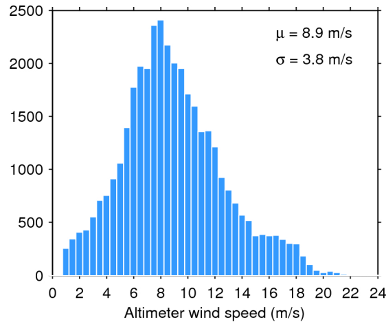
Figure 33. Histogram of flag-valid wind over oceans and lakes for 23/12/2015. The mean ( \mu ) and standard deviation ( \sigma ) are also shown. Note that values larger than 24 m/s are excluded from the histogram for the sake of readability but not from the computation of \mu and \sigma .
