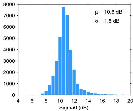
Figure 28. Histogram of science-valid sigma0 over oceans and lakes for 07/12/2015. The mean ( \mu ) and standard deviation ( \sigma ) are also shown. Note that values outside [4 20] dB are excluded from the histogram for the sake of readability but not from the computation of \mu and \sigma .
