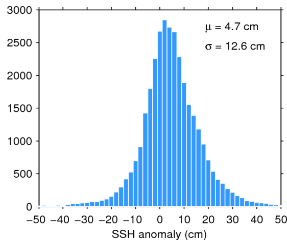
Figure 11. Histogram of science-valid SSH anomaly over oceans and lakes for 07/12/2015. The mean ( \mu ) and standard deviation ( \sigma ) are also shown. Note that values outside [-50 50] cm are excluded from the histogram for the sake of readability but not from the computation of \mu and \sigma .
