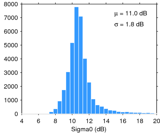
Figure 25. Histogram of flag-valid sigma0 over oceans and lakes for 07/12/2015. The mean ( \mu ) and standard deviation ( \sigma ) are also shown. Note that values outside [4 20] dB are excluded from the histogram for the sake of readability but not from the computation of \mu and \sigma .
