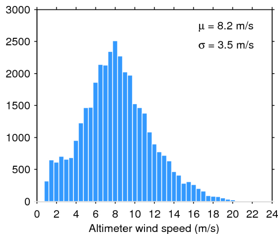
Figure 35. Histogram of science-valid wind over oceans and lakes for 07/12/2015. The mean ( \mu ) and standard deviation ( \sigma ) are also shown. Note that values larger than 24 m/s are excluded from the histogram for the sake of readability but not from the computation of \mu and \sigma .
