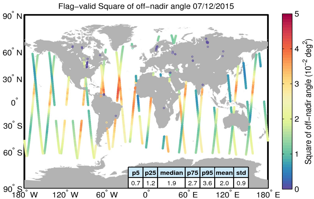
Figure 37. Geographical distribution of flag-valid mispointing data over oceans and lakes for 07/12/2015. The statistical values shown in the table refer to the mispointing in 10^{-2} \text{deg}^2 and are calculated over all measurements shown in the figure.
