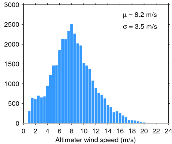
Figure 33. Histogram of flag-valid wind over oceans and lakes for 07/12/2015. The mean ( \mu ) and standard deviation ( \sigma ) are also shown. Note that values larger than 24 m/s are excluded from the histogram for the sake of readability but not from the computation of \mu and \sigma .
