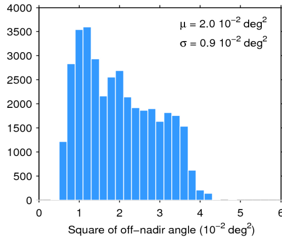
Figure 39. Histogram of flag-valid mispointing over oceans and lakes for 07/12/2015. The mean ( \mu ) and standard deviation ( \sigma ) are also shown. Note that values larger than 6 \cdot 10^{-2} \text{ deg}^2 are excluded from the histogram for the sake of readability but not from the computation of \mu and \sigma .
