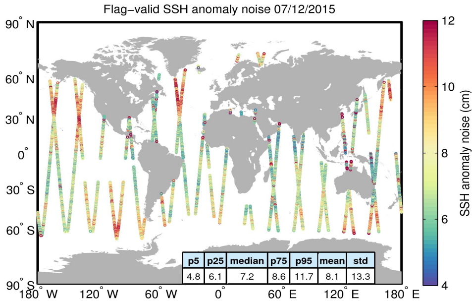
Figure 8. Geographical distribution of flag-valid 20-Hz SSH anomaly measurement noise over oceans and lakes for 07/12/2015. The statistical values shown in the table refer to the SSH anomaly noise and are calculated over all measurements shown in the figure.
