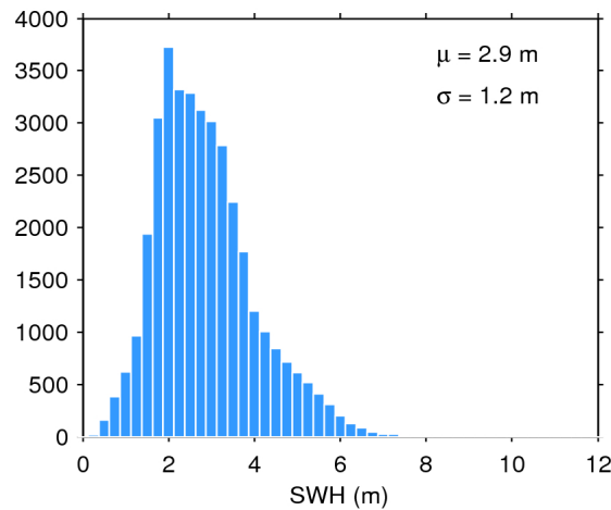
Figure 17. Histogram of flag-valid SWH over oceans and lakes for 07/12/2015. The mean ( \mu ) and standard deviation ( \sigma ) are also shown. Note that values larger than 12 m are excluded from the histogram for the sake of readability but not from the computation of \mu and \sigma .
