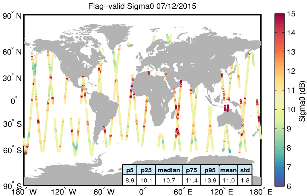
Figure 23. Geographical distribution of flag-valid sigma0 data over oceans and lakes for 07/12/2015. The statistical values shown in the table refer to the sigma0 in dB and are calculated over all measurements shown in the figure.
