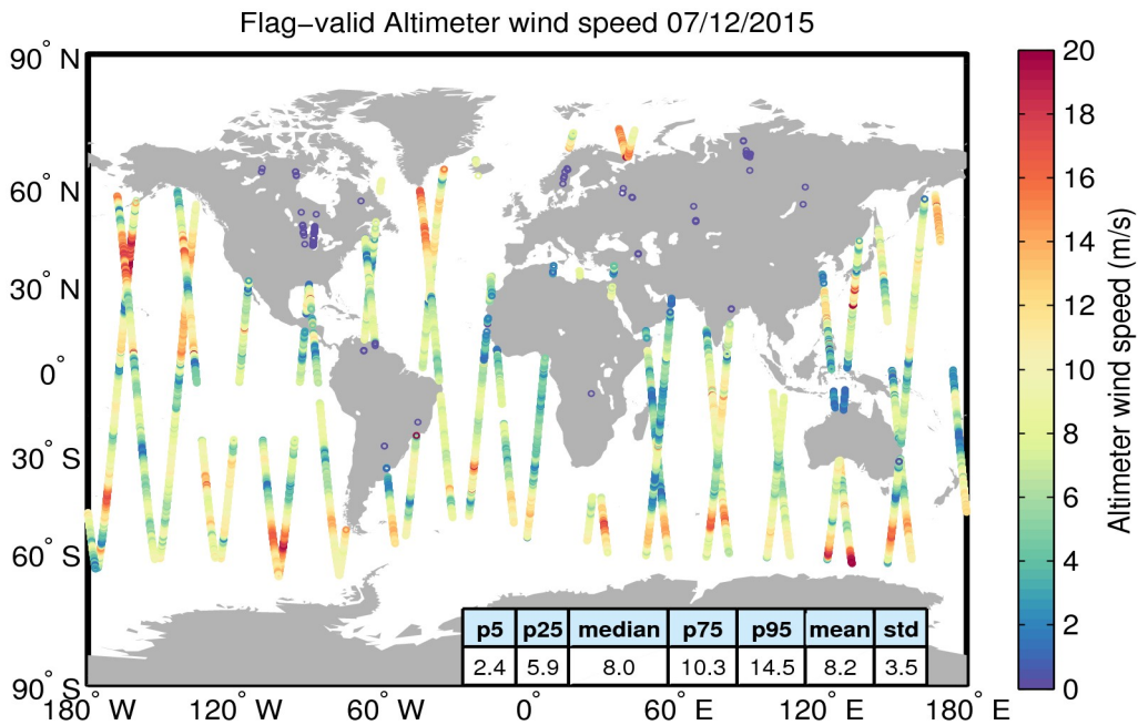
Figure 31. Geographical distribution of flag-valid wind data over oceans and lakes for 07/12/2015. The statistical values shown in the table refer to the wind in m/s and are calculated over all measurements shown in the figure.
