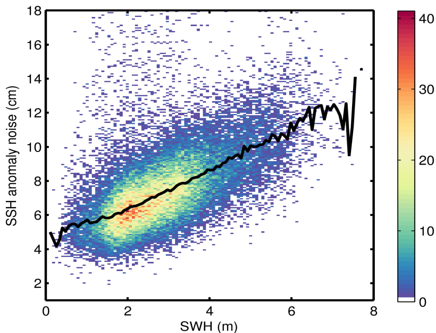
Figure 9. 2D histogram showing flag-valid SSH anomaly noise as a function of SWH for 07/12/2015. The black line denotes the median SSH anomaly noise as a function of SWH.
