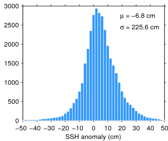
Figure 7. Histogram of flag-valid SSH anomaly over oceans and lakes for 07/12/2015. The mean ( \mu ) and standard deviation ( \sigma ) are also shown. Note that values outside [-50 50] cm are excluded from the histogram for the sake of readability but not from the computation of \mu and \sigma .
