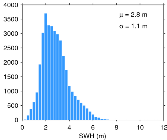
Figure 20. Histogram of science-valid SWH over oceans and lakes for 07/12/2015. The mean ( \mu ) and standard deviation ( \sigma ) are also shown. Note that values larger than 12 m are excluded from the histogram for the sake of readability but not from the computation of \mu and \sigma .
