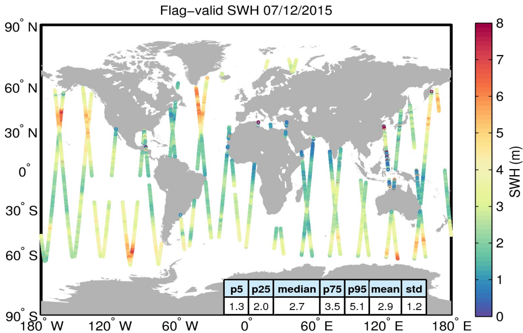
Figure 15. Geographical distribution of flag-valid SWH data over oceans and lakes for 07/12/2015. The statistical values shown in the table refer to the SWH in m and are calculated over all measurements shown in the figure.
