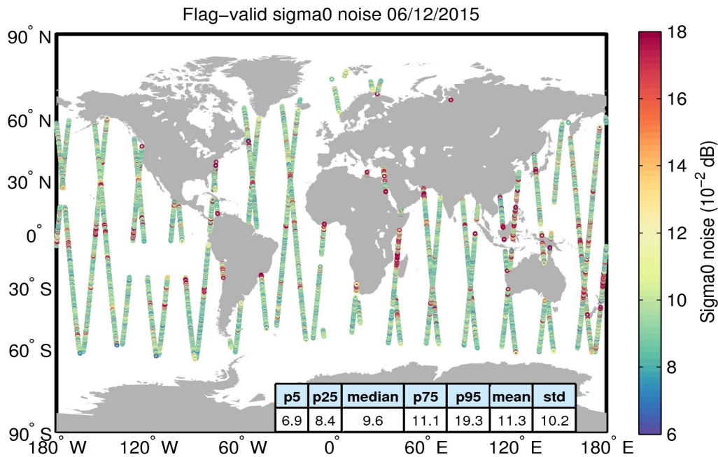
Figure 26. Geographical distribution of flag-valid 20-Hz sigma0 measurement noise over oceans and lakes for 06/12/2015. The statistical values shown in the table refer to the sigma0 noise and are calculated over all measurements shown in the figure.
