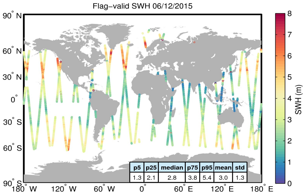
Figure 15. Geographical distribution of flag-valid SWH data over oceans and lakes for 06/12/2015. The statistical values shown in the table refer to the SWH in m and are calculated over all measurements shown in the figure.
