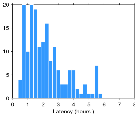
Figure 2. Histogram of the data latency for 06/12/2015. The y-axis denotes the number of files that are made available with a delay of x-hours with respect to the mean time of the records stored in the file.
