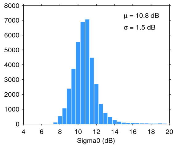
Figure 28. Histogram of science-valid sigma0 over oceans and lakes for 06/12/2015. The mean ( \mu ) and standard deviation ( \sigma ) are also shown. Note that values outside [4 20] dB are excluded from the histogram for the sake of readability but not from the computation of \mu and \sigma .
