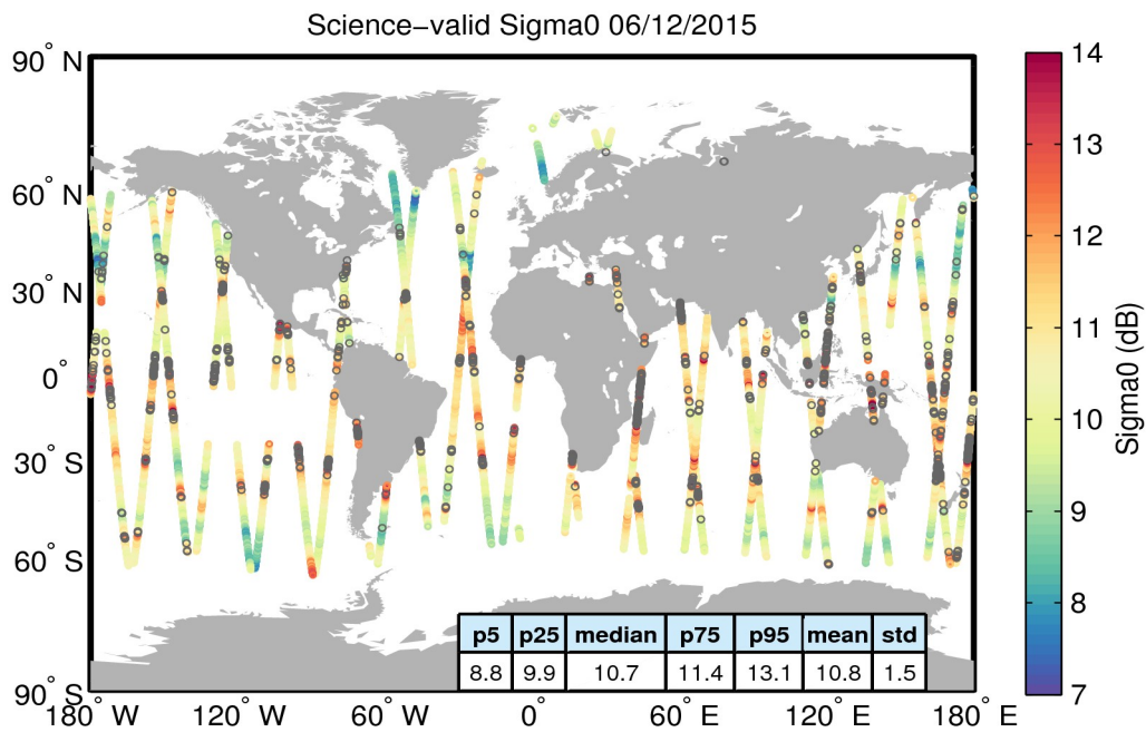
Figure 27. Geographical distribution of science-valid sigma0 data over oceans and lakes for 06/12/2015. The statistical values shown in the table refer to the sigma0 in dB and are calculated over all measurements shown in the figure. Gray circles denote records that have been rejected based on the editing criteria described in Table 4.
