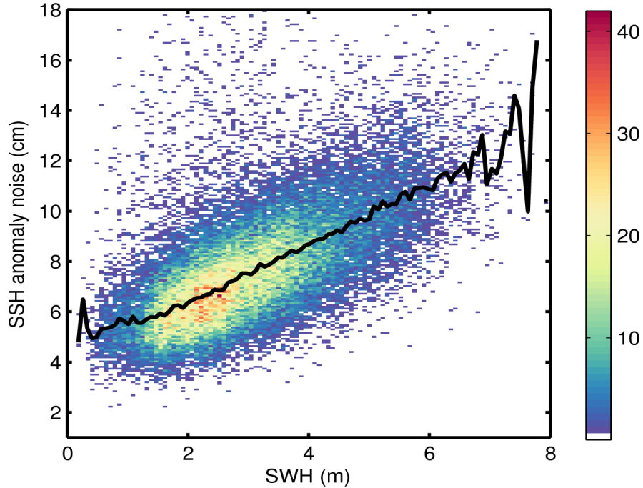
Figure 9. 2D histogram showing flag-valid SSH anomaly noise as a function of SWH for 06/12/2015. The black line denotes the median SSH anomaly noise as a function of SWH.
