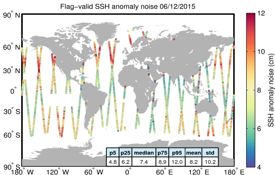
Figure 8. Geographical distribution of flag-valid 20-Hz SSH anomaly measurement noise over oceans and lakes for 06/12/2015. The statistical values shown in the table refer to the SSH anomaly noise and are calculated over all measurements shown in the figure.
