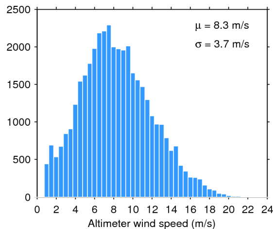
Figure 35. Histogram of science-valid wind over oceans and lakes for 06/12/2015. The mean ( \mu ) and standard deviation ( \sigma ) are also shown. Note that values larger than 24 m/s are excluded from the histogram for the sake of readability but not from the computation of \mu and \sigma .
