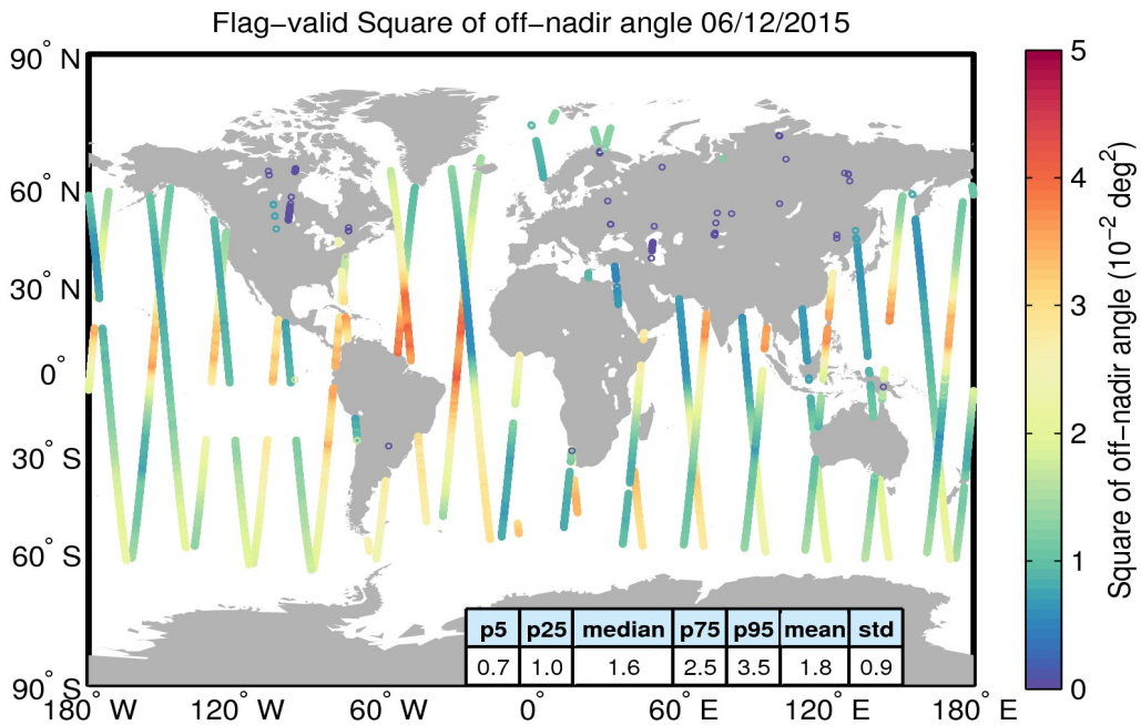
Figure 37. Geographical distribution of flag-valid mispointing data over oceans and lakes for 06/12/2015. The statistical values shown in the table refer to the mispointing in 10^{-2} deg 2 and are calculated over all measurements shown in the figure.
