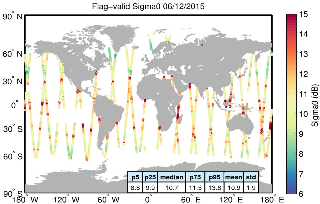
Figure 23. Geographical distribution of flag-valid sigma0 data over oceans and lakes for 06/12/2015. The statistical values shown in the table refer to the sigma0 in dB and are calculated over all measurements shown in the figure.
