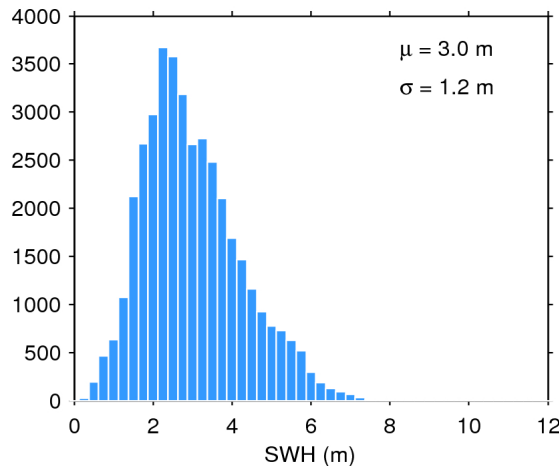
Figure 20. Histogram of science-valid SWH over oceans and lakes for 06/12/2015. The mean ( \mu ) and standard deviation ( \sigma ) are also shown. Note that values larger than 12 m are excluded from the histogram for the sake of readability but not from the computation of \mu and \sigma .
