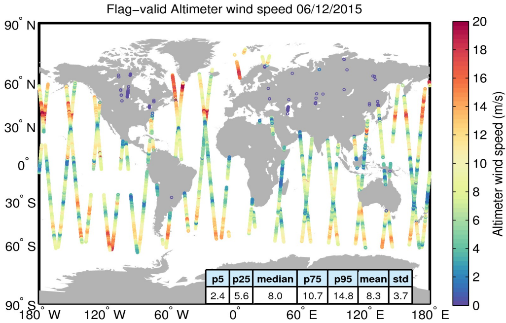
Figure 31. Geographical distribution of flag-valid wind data over oceans and lakes for 06/12/2015. The statistical values shown in the table refer to the wind in m/s and are calculated over all measurements shown in the figure.
