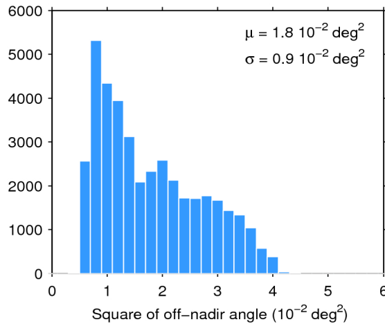
Figure 39. Histogram of flag-valid mispointing over oceans and lakes for 06/12/2015. The mean ( \mu ) and standard deviation ( \sigma ) are also shown. Note that values larger than 6 \cdot 10^{-2} \text{ deg}^2 are excluded from the histogram for the sake of readability but not from the computation of \mu and \sigma .
