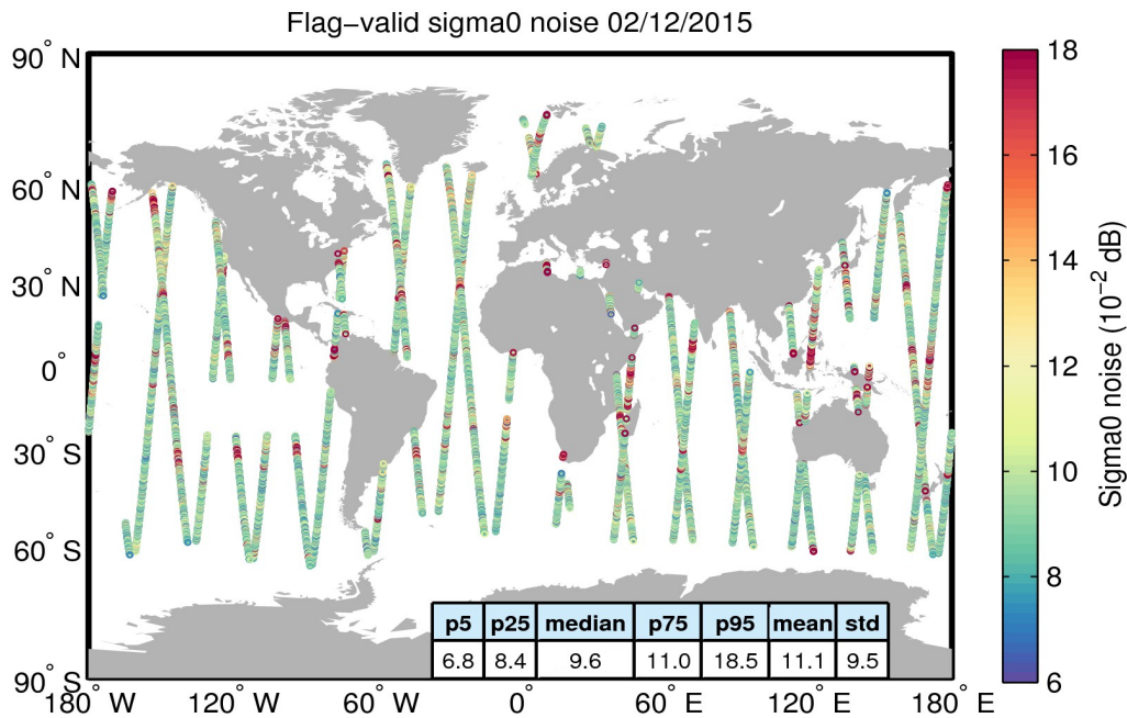
Figure 26. Geographical distribution of flag-valid 20-Hz sigma0 measurement noise over oceans and lakes for 02/12/2015. The statistical values shown in the table refer to the sigma0 noise and are calculated over all measurements shown in the figure.
