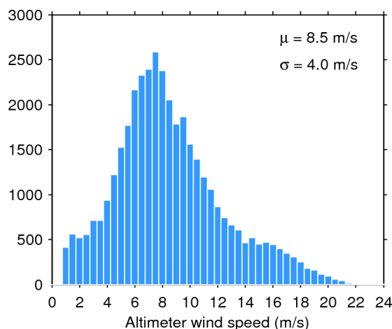
Figure 35. Histogram of science-valid wind over oceans and lakes for 02/12/2015. The mean ( \mu ) and standard deviation ( \sigma ) are also shown. Note that values larger than 24 m/s are excluded from the histogram for the sake of readability but not from the computation of \mu and \sigma .
