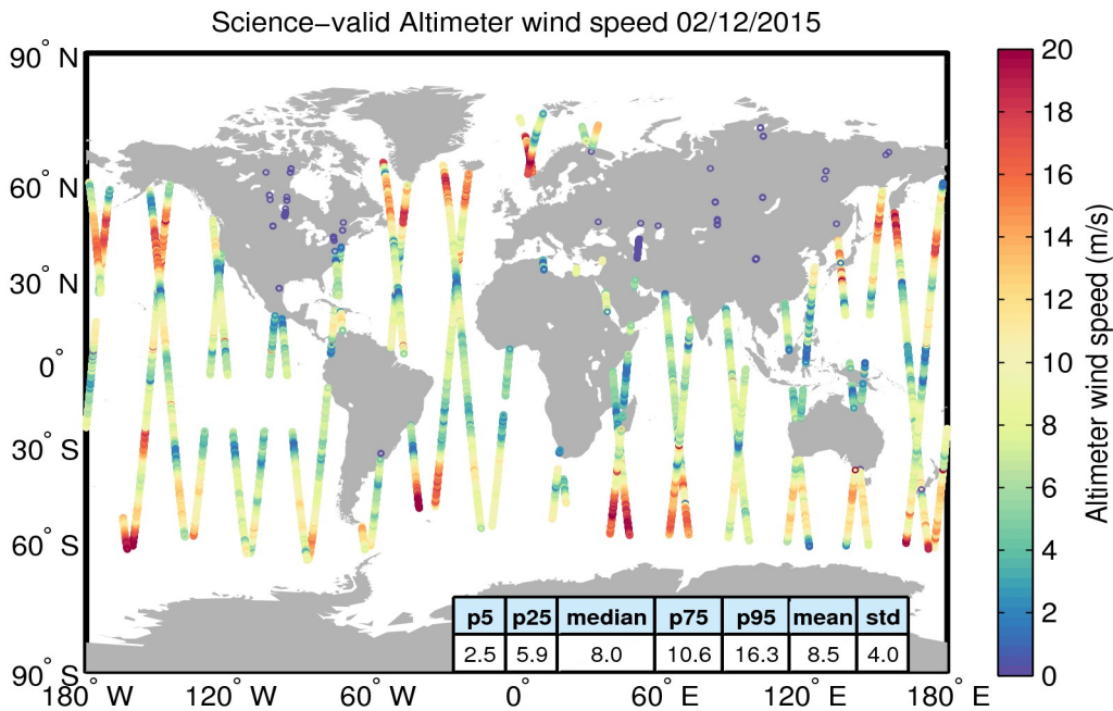
Figure 34. Geographical distribution of science-valid wind data over oceans and lakes for 02/12/2015. The statistical values shown in the table refer to the wind in m/s and are calculated over all measurements shown in the figure. Gray circles denote records that have been rejected based on the editing criteria described in Table 5.
