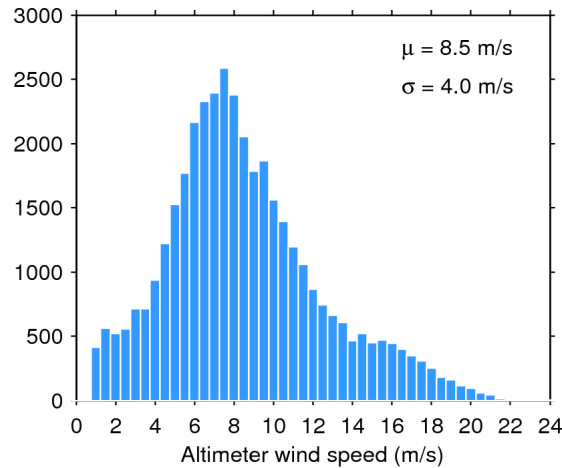
Figure 33. Histogram of flag-valid wind over oceans and lakes for 02/12/2015. The mean ( \mu ) and standard deviation ( \sigma ) are also shown. Note that values larger than 24 m/s are excluded from the histogram for the sake of readability but not from the computation of \mu and \sigma .
