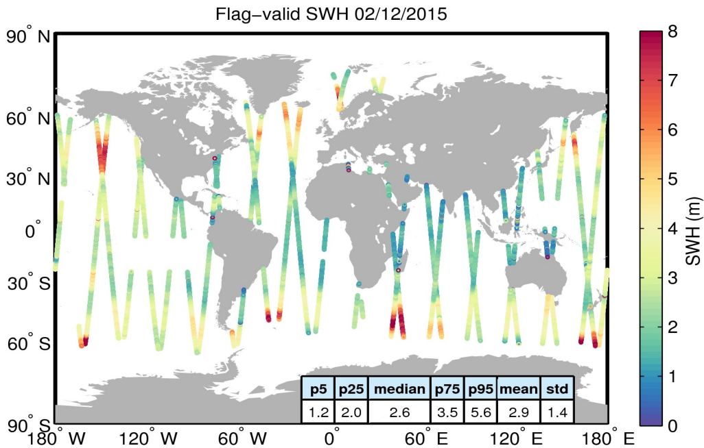
Figure 15. Geographical distribution of flag-valid SWH data over oceans and lakes for 02/12/2015. The statistical values shown in the table refer to the SWH in m and are calculated over all measurements shown in the figure.
