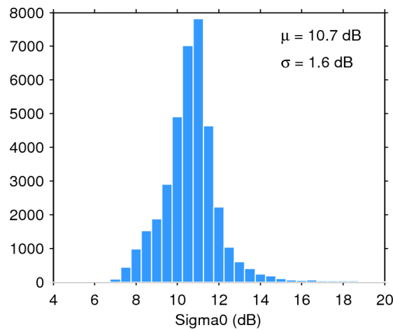
Figure 28. Histogram of science-valid sigma0 over oceans and lakes for 02/12/2015. The mean ( \mu ) and standard deviation ( \sigma ) are also shown. Note that values outside [4 20] dB are excluded from the histogram for the sake of readability but not from the computation of \mu and \sigma .
