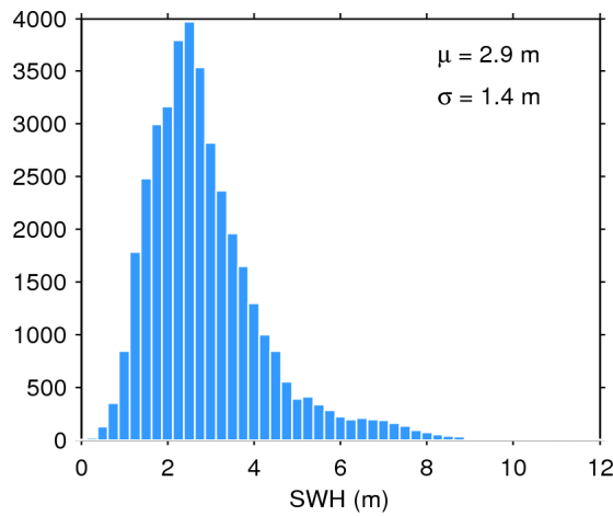
Figure 17. Histogram of flag-valid SWH over oceans and lakes for 02/12/2015. The mean ( \mu ) and standard deviation ( \sigma ) are also shown. Note that values larger than 12 m are excluded from the histogram for the sake of readability but not from the computation of \mu and \sigma .
