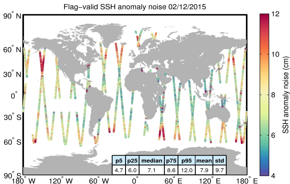
Figure 8. Geographical distribution of flag-valid 20-Hz SSH anomaly measurement noise over oceans and lakes for 02/12/2015. The statistical values shown in the table refer to the SSH anomaly noise and are calculated over all measurements shown in the figure.
