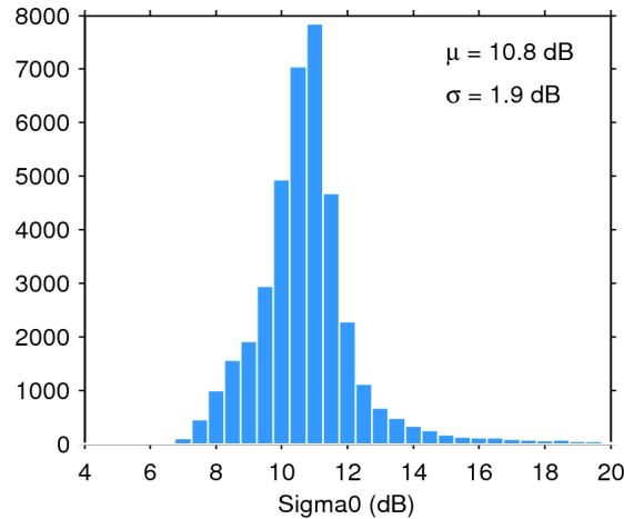
Figure 25. Histogram of flag-valid sigma0 over oceans and lakes for 02/12/2015. The mean ( \mu ) and standard deviation ( \sigma ) are also shown. Note that values outside [4 20] dB are excluded from the histogram for the sake of readability but not from the computation of \mu and \sigma .
