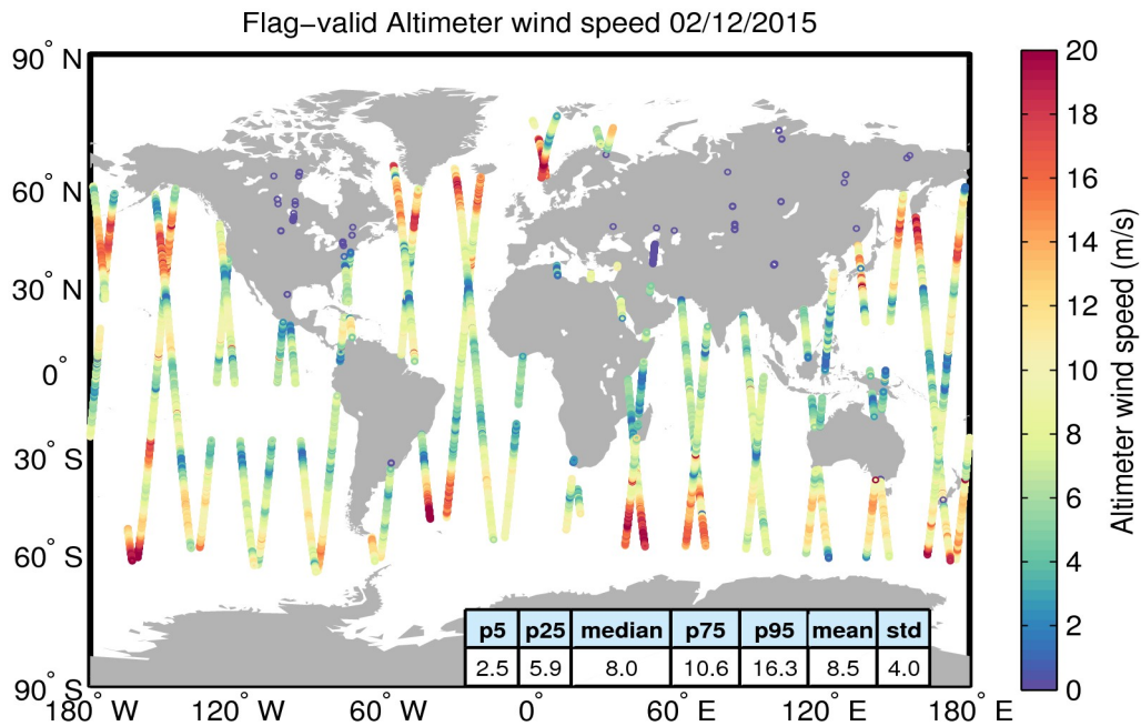
Figure 31. Geographical distribution of flag-valid wind data over oceans and lakes for 02/12/2015. The statistical values shown in the table refer to the wind in m/s and are calculated over all measurements shown in the figure.
