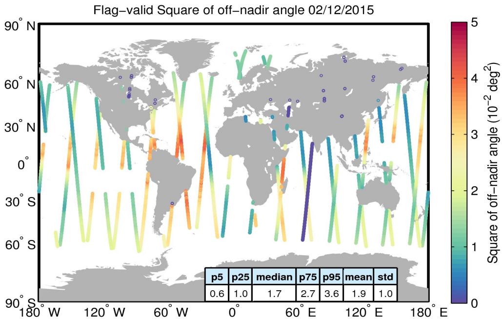
Figure 37. Geographical distribution of flag-valid mispointing data over oceans and lakes for 02/12/2015. The statistical values shown in the table refer to the mispointing in 10^{-2} deg 2 and are calculated over all measurements shown in the figure.
