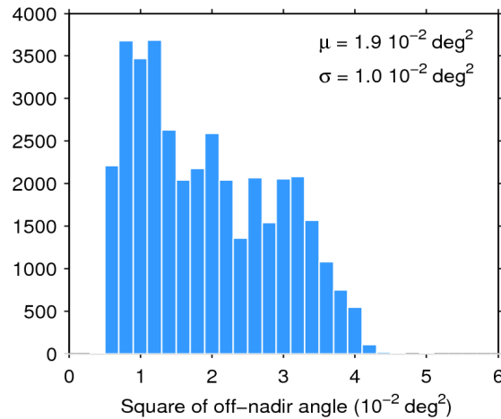
Figure 39. Histogram of flag-valid mispointing over oceans and lakes for 02/12/2015. The mean ( \mu ) and standard deviation ( \sigma ) are also shown. Note that values larger than 6 \cdot 10^{-2} \text{ deg}^2 are excluded from the histogram for the sake of readability but not from the computation of \mu and \sigma .
