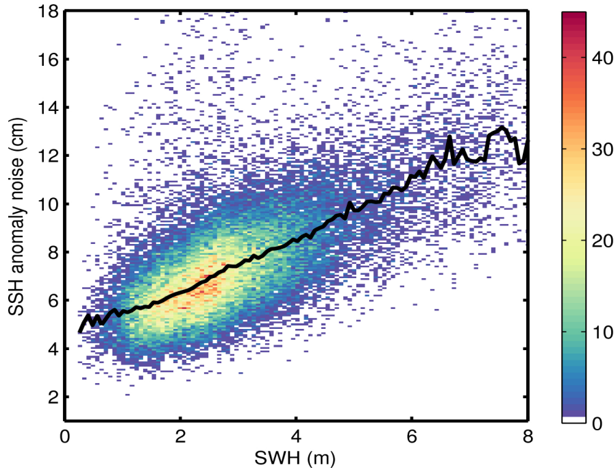
Figure 9. 2D histogram showing flag-valid SSH anomaly noise as a function of SWH for 02/12/2015. The black line denotes the median SSH anomaly noise as a function of SWH.
