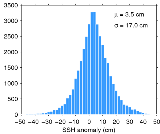
Figure 7. Histogram of flag-valid SSH anomaly over oceans and lakes for 02/12/2015. The mean ( \mu ) and standard deviation ( \sigma ) are also shown. Note that values outside [-50\ 50] cm are excluded from the histogram for the sake of readability but not from the computation of \mu and \sigma .
