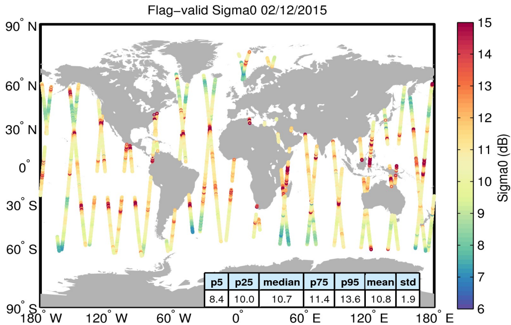
Figure 23. Geographical distribution of flag-valid sigma0 data over oceans and lakes for 02/12/2015. The statistical values shown in the table refer to the sigma0 in dB and are calculated over all measurements shown in the figure.
