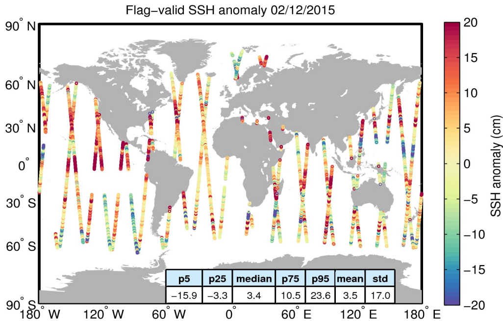
Figure 5. Geographical distribution of flag-valid 1-Hz SSH anomaly data over oceans and lakes for 02/12/2015. The statistical values shown in the table refer to the SSH anomaly in cm and are calculated over all measurements shown in the figure.
