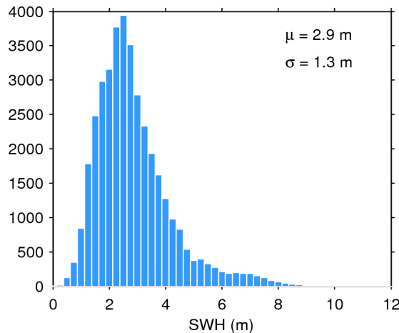
Figure 20. Histogram of science-valid SWH over oceans and lakes for 02/12/2015. The mean ( \mu ) and standard deviation ( \sigma ) are also shown. Note that values larger than 12 m are excluded from the histogram for the sake of readability but not from the computation of \mu and \sigma .
