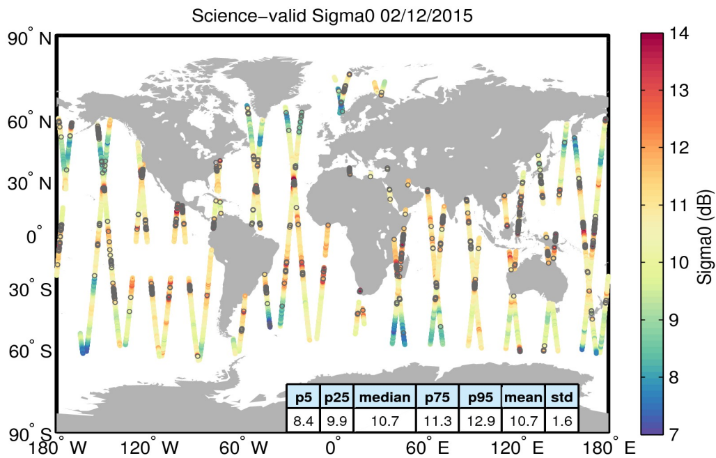
Figure 27. Geographical distribution of science-valid sigma0 data over oceans and lakes for 02/12/2015. The statistical values shown in the table refer to the sigma0 in dB and are calculated over all measurements shown in the figure. Gray circles denote records that have been rejected based on the editing criteria described in Table 4.
