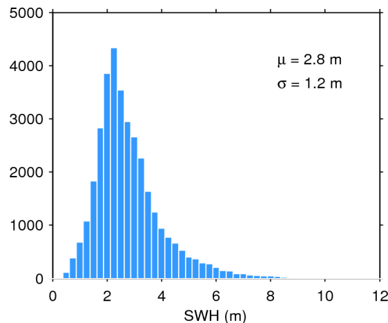
Figure 20. Histogram of science-valid SWH over oceans and lakes for 30/11/2015. The mean ( \mu ) and standard deviation ( \sigma ) are also shown. Note that values larger than 12 m are excluded from the histogram for the sake of readability but not from the computation of \mu and \sigma .
