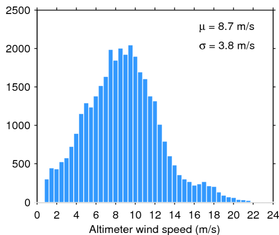
Figure 33. Histogram of flag-valid wind over oceans and lakes for 30/11/2015. The mean ( \mu ) and standard deviation ( \sigma ) are also shown. Note that values larger than 24 m/s are excluded from the histogram for the sake of readability but not from the computation of \mu and \sigma .
