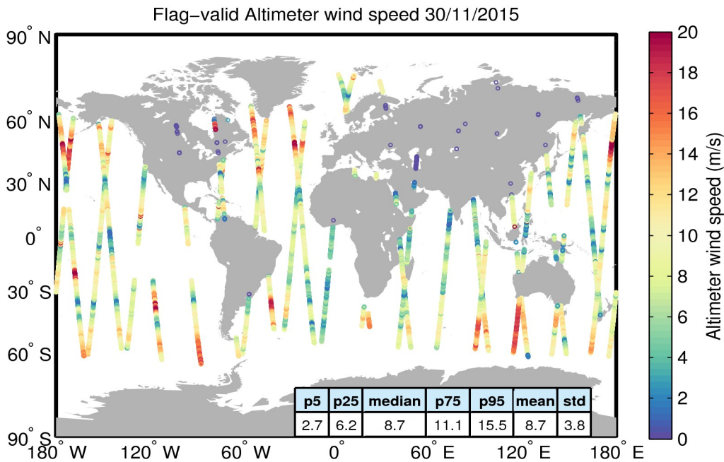
Figure 31. Geographical distribution of flag-valid wind data over oceans and lakes for 30/11/2015. The statistical values shown in the table refer to the wind in m/s and are calculated over all measurements shown in the figure.
