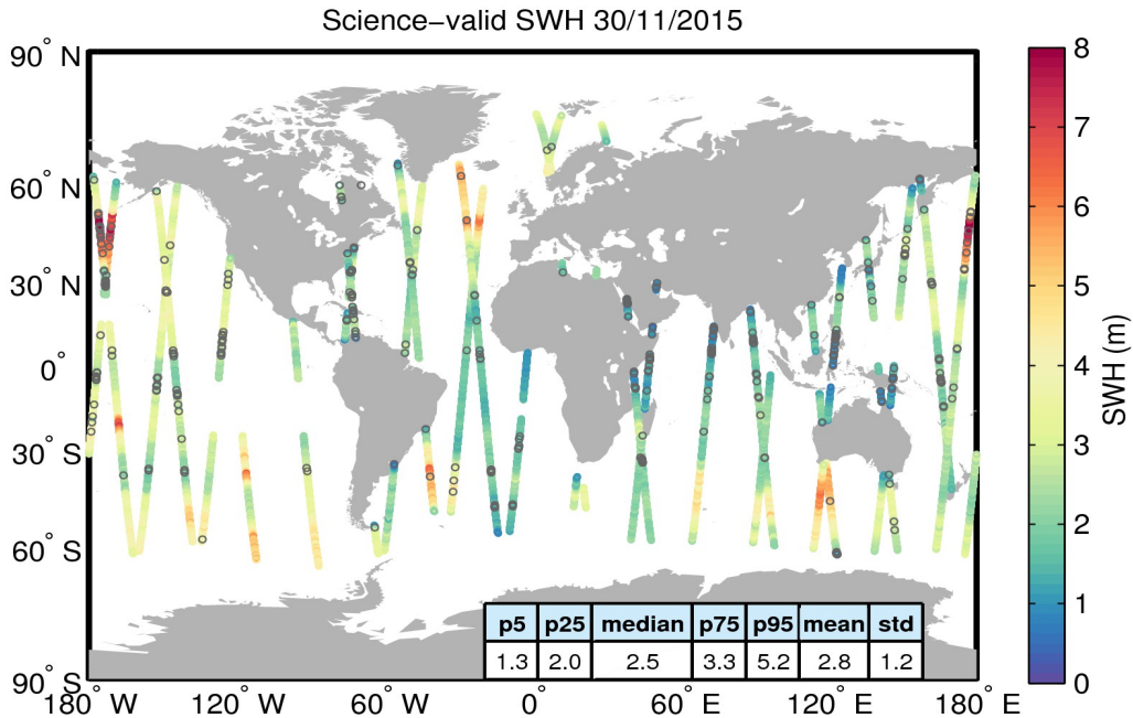
Figure 19. Geographical distribution of science-valid SWH data over oceans and lakes for 30/11/2015. The statistical values shown in the table refer to the SWH in m and are calculated over all measurements shown in the figure. Gray circles denote records that have been rejected based on the editing criteria described in Table 3.
