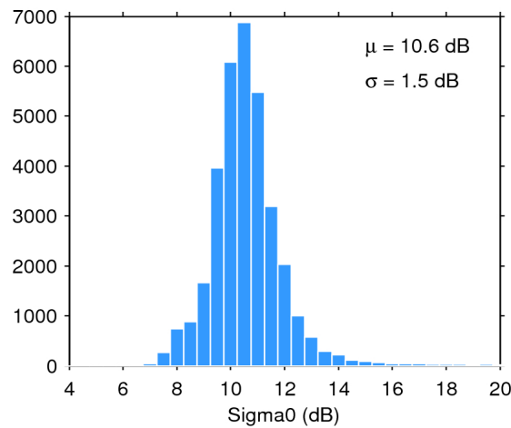
Figure 28. Histogram of science-valid sigma0 over oceans and lakes for 30/11/2015. The mean ( \mu ) and standard deviation ( \sigma ) are also shown. Note that values outside [4 20] dB are excluded from the histogram for the sake of readability but not from the computation of \mu and \sigma .
