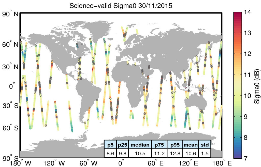
Figure 27. Geographical distribution of science-valid sigma0 data over oceans and lakes for 30/11/2015. The statistical values shown in the table refer to the sigma0 in dB and are calculated over all measurements shown in the figure. Gray circles denote records that have been rejected based on the editing criteria described in Table 4.
