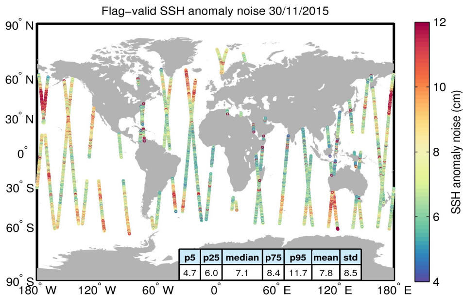
Figure 8. Geographical distribution of flag-valid 20-Hz SSH anomaly measurement noise over oceans and lakes for 30/11/2015. The statistical values shown in the table refer to the SSH anomaly noise and are calculated over all measurements shown in the figure.
