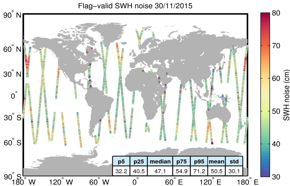
Figure 18. Geographical distribution of flag-valid 20-Hz SWH measurement noise over oceans and lakes for 30/11/2015. The statistical values shown in the figure refer to the SWH noise and are calculated over all measurements shown in the figure.
