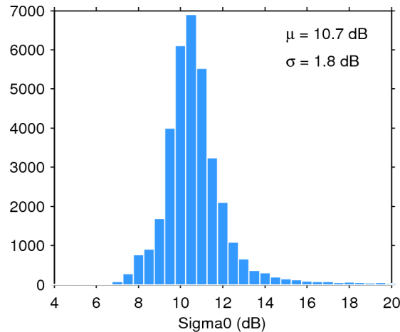
Figure 25. Histogram of flag-valid sigma0 over oceans and lakes for 30/11/2015. The mean ( \mu ) and standard deviation ( \sigma ) are also shown. Note that values outside [4 20] dB are excluded from the histogram for the sake of readability but not from the computation of \mu and \sigma .
