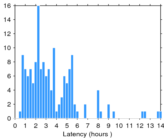
Figure 2. Histogram of the data latency for 30/11/2015. The y-axis denotes the number of files that are made available with a delay of x-hours with respect to the mean time of the records stored in the file.
