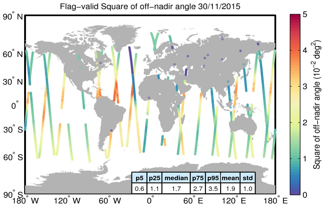
Figure 37. Geographical distribution of flag-valid mispointing data over oceans and lakes for 30/11/2015. The statistical values shown in the table refer to the mispointing in 10^{-2} \text{ deg}^2 and are calculated over all measurements shown in the figure.
