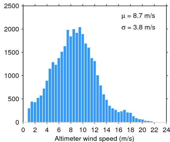
Figure 35. Histogram of science-valid wind over oceans and lakes for 30/11/2015. The mean ( \mu ) and standard deviation ( \sigma ) are also shown. Note that values larger than 24 m/s are excluded from the histogram for the sake of readability but not from the computation of \mu and \sigma .
