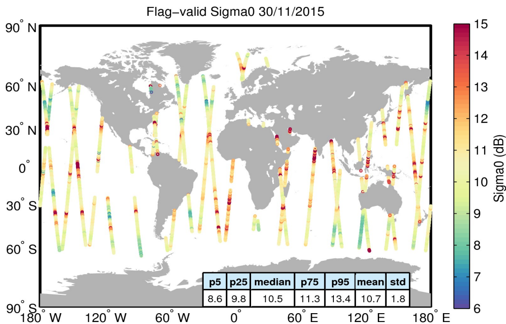
Figure 23. Geographical distribution of flag-valid sigma0 data over oceans and lakes for 30/11/2015. The statistical values shown in the table refer to the sigma0 in dB and are calculated over all measurements shown in the figure.
