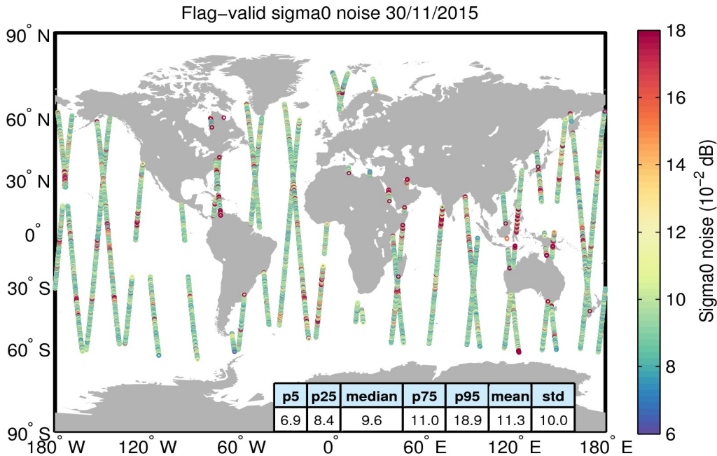
Figure 26. Geographical distribution of flag-valid 20-Hz sigma0 measurement noise over oceans and lakes for 30/11/2015. The statistical values shown in the table refer to the sigma0 noise and are calculated over all measurements shown in the figure.
