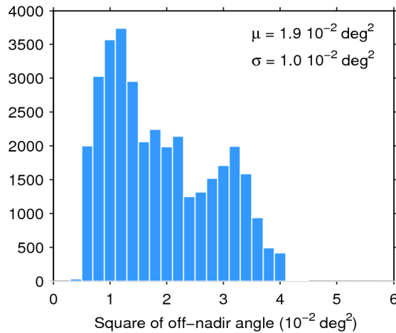
Figure 39. Histogram of flag-valid mispointing over oceans and lakes for 30/11/2015. The mean ( \mu ) and standard deviation ( \sigma ) are also shown. Note that values larger than 6 \cdot 10^{-2} \text{ deg}^2 are excluded from the histogram for the sake of readability but not from the computation of \mu and \sigma .
