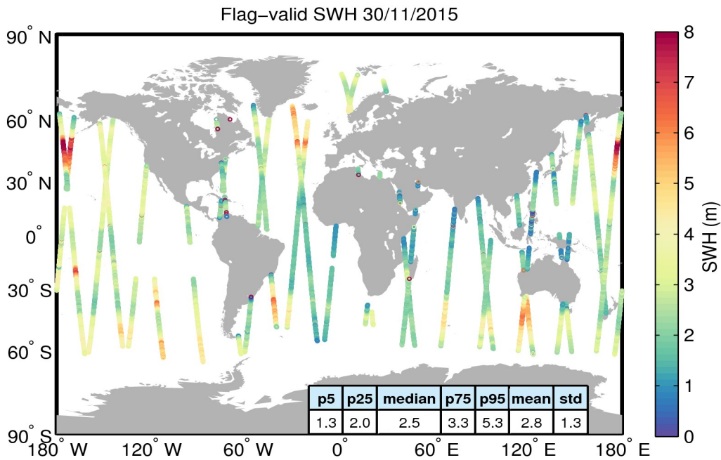
Figure 15. Geographical distribution of flag-valid SWH data over oceans and lakes for 30/11/2015. The statistical values shown in the table refer to the SWH in m and are calculated over all measurements shown in the figure.
