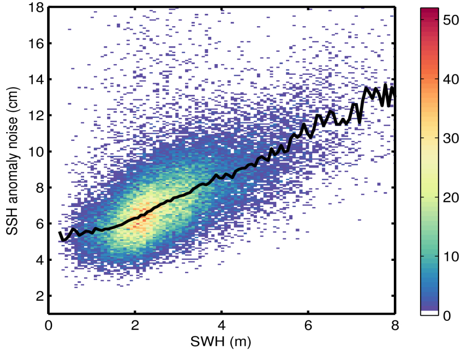
Figure 9. 2D histogram showing flag-valid SSH anomaly noise as a function of SWH for 30/11/2015. The black line denotes the median SSH anomaly noise as a function of SWH.
