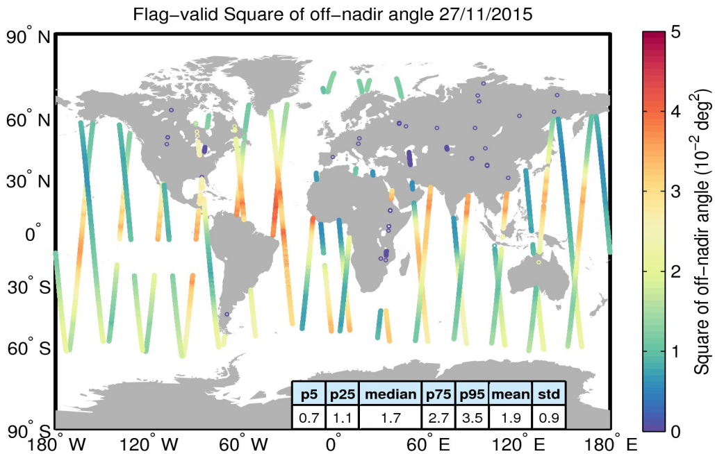
Figure 37. Geographical distribution of flag-valid mispointing data over oceans and lakes for 27/11/2015. The statistical values shown in the table refer to the mispointing in 10^{-2} \text{ deg}^2 and are calculated over all measurements shown in the figure.
