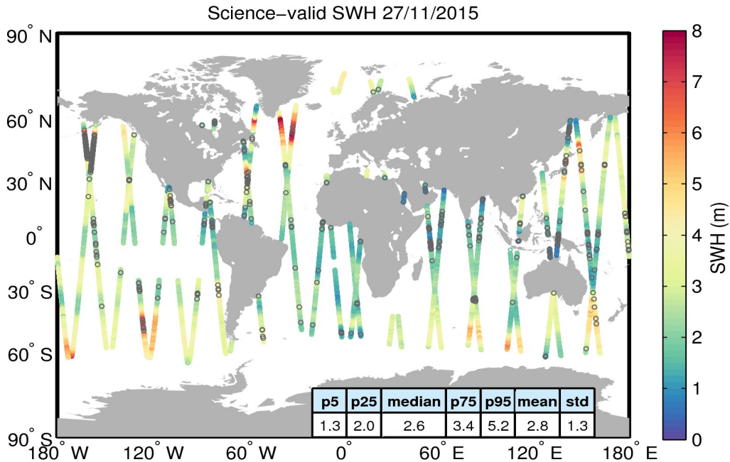
Figure 19. Geographical distribution of science-valid SWH data over oceans and lakes for 27/11/2015. The statistical values shown in the table refer to the SWH in m and are calculated over all measurements shown in the figure. Gray circles denote records that have been rejected based on the editing criteria described in Table 3.
