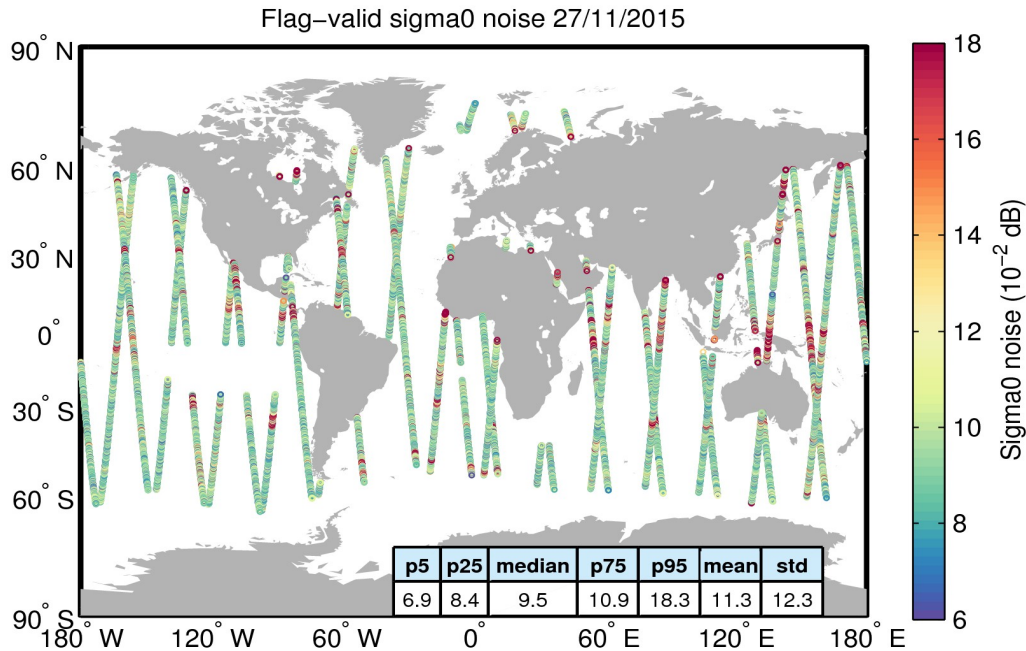
Figure 26. Geographical distribution of flag-valid 20-Hz sigma0 measurement noise over oceans and lakes for 27/11/2015. The statistical values shown in the table refer to the sigma0 noise and are calculated over all measurements shown in the figure.
