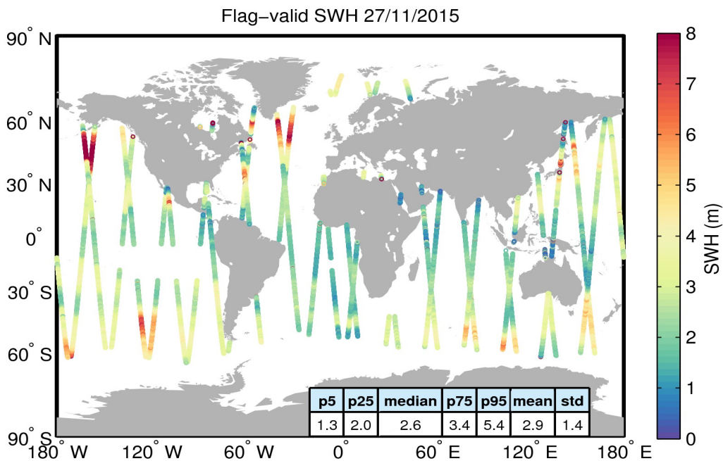
Figure 15. Geographical distribution of flag-valid SWH data over oceans and lakes for 27/11/2015. The statistical values shown in the table refer to the SWH in m and are calculated over all measurements shown in the figure.
