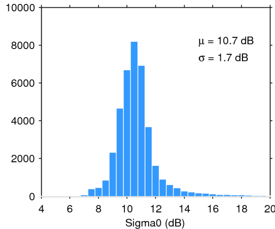
Figure 25. Histogram of flag-valid sigma0 over oceans and lakes for 27/11/2015. The mean ( \mu ) and standard deviation ( \sigma ) are also shown. Note that values outside [4 20] dB are excluded from the histogram for the sake of readability but not from the computation of \mu and \sigma .
