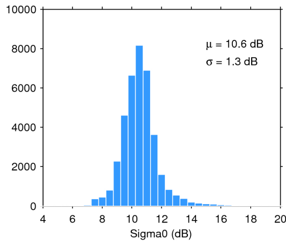
Figure 28. Histogram of science-valid sigma0 over oceans and lakes for 27/11/2015. The mean ( \mu ) and standard deviation ( \sigma ) are also shown. Note that values outside [4 20] dB are excluded from the histogram for the sake of readability but not from the computation of \mu and \sigma .
