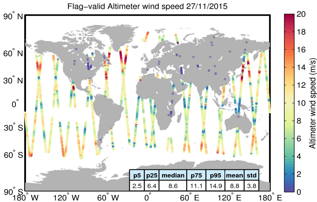
Figure 31. Geographical distribution of flag-valid wind data over oceans and lakes for 27/11/2015. The statistical values shown in the table refer to the wind in m/s and are calculated over all measurements shown in the figure.
