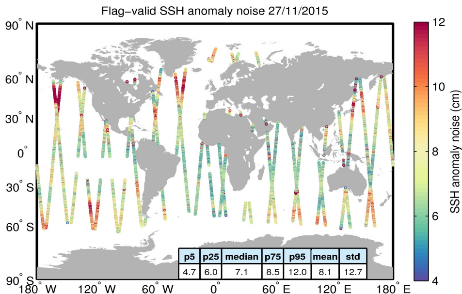
Figure 8. Geographical distribution of flag-valid 20-Hz SSH anomaly measurement noise over oceans and lakes for 27/11/2015. The statistical values shown in the table refer to the SSH anomaly noise and are calculated over all measurements shown in the figure.
