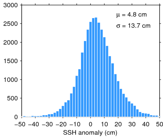
Figure 11. Histogram of science-valid SSH anomaly over oceans and lakes for 27/11/2015. The mean ( \mu ) and standard deviation ( \sigma ) are also shown. Note that values outside [-50 50] cm are excluded from the histogram for the sake of readability but not from the computation of \mu and \sigma .
