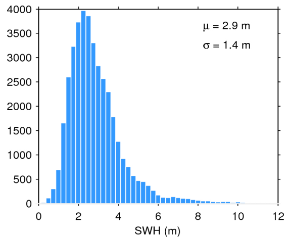
Figure 17. Histogram of flag-valid SWH over oceans and lakes for 27/11/2015. The mean ( \mu ) and standard deviation ( \sigma ) are also shown. Note that values larger than 12 m are excluded from the histogram for the sake of readability but not from the computation of \mu and \sigma .
