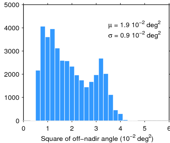
Figure 39. Histogram of flag-valid mispointing over oceans and lakes for 27/11/2015. The mean ( \mu ) and standard deviation ( \sigma ) are also shown. Note that values larger than 6 \cdot 10^{-2} \text{ deg}^2 are excluded from the histogram for the sake of readability but not from the computation of \mu and \sigma .
