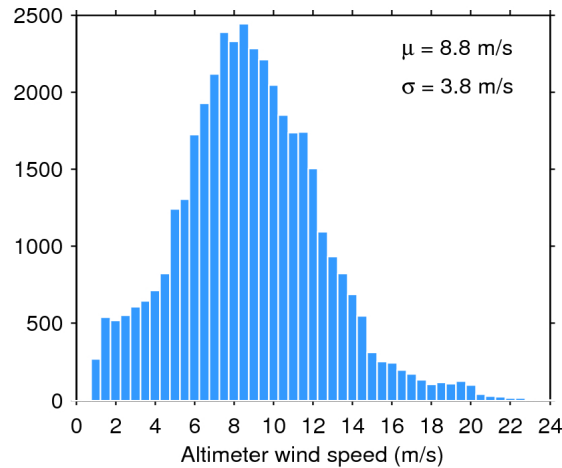
Figure 33. Histogram of flag-valid wind over oceans and lakes for 27/11/2015. The mean ( \mu ) and standard deviation ( \sigma ) are also shown. Note that values larger than 24 m/s are excluded from the histogram for the sake of readability but not from the computation of \mu and \sigma .
