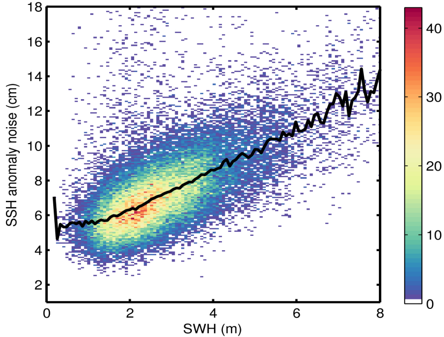
Figure 9. 2D histogram showing flag-valid SSH anomaly noise as a function of SWH for 27/11/2015. The black line denotes the median SSH anomaly noise as a function of SWH.
