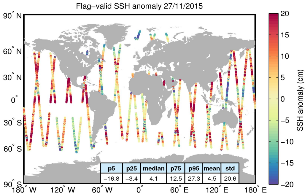
Figure 5. Geographical distribution of flag-valid 1-Hz SSH anomaly data over oceans and lakes for 27/11/2015. The statistical values shown in the table refer to the SSH anomaly in cm and are calculated over all measurements shown in the figure.
