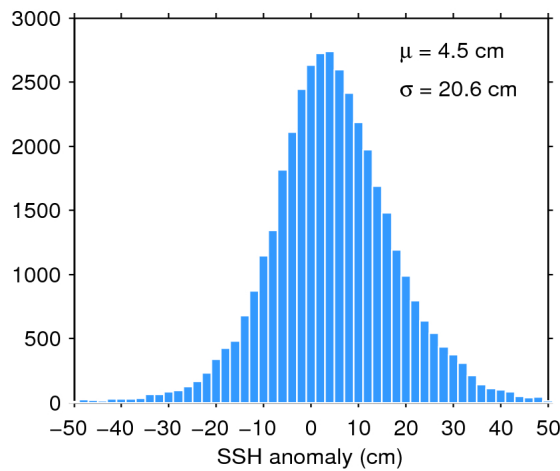
Figure 7. Histogram of flag-valid SSH anomaly over oceans and lakes for 27/11/2015. The mean ( \mu ) and standard deviation ( \sigma ) are also shown. Note that values outside [-50\ 50] cm are excluded from the histogram for the sake of readability but not from the computation of \mu and \sigma .
