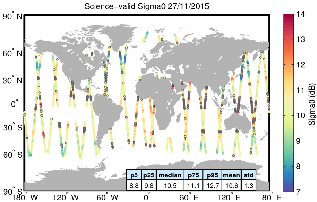
Figure 27. Geographical distribution of science-valid sigma0 data over oceans and lakes for 27/11/2015. The statistical values shown in the table refer to the sigma0 in dB and are calculated over all measurements shown in the figure. Gray circles denote records that have been rejected based on the editing criteria described in Table 4.
