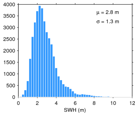
Figure 20. Histogram of science-valid SWH over oceans and lakes for 27/11/2015. The mean ( \mu ) and standard deviation ( \sigma ) are also shown. Note that values larger than 12 m are excluded from the histogram for the sake of readability but not from the computation of \mu and \sigma .
