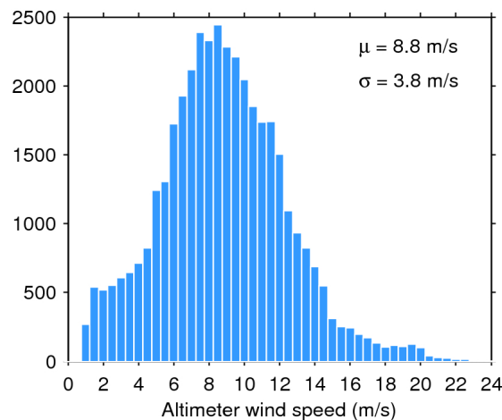
Figure 35. Histogram of science-valid wind over oceans and lakes for 27/11/2015. The mean ( \mu ) and standard deviation ( \sigma ) are also shown. Note that values larger than 24 m/s are excluded from the histogram for the sake of readability but not from the computation of \mu and \sigma .
