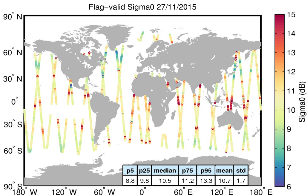
Figure 23. Geographical distribution of flag-valid sigma0 data over oceans and lakes for 27/11/2015. The statistical values shown in the table refer to the sigma0 in dB and are calculated over all measurements shown in the figure.
