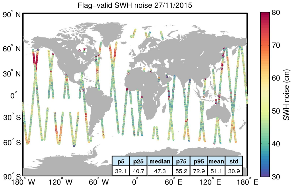
Figure 18. Geographical distribution of flag-valid 20-Hz SWH measurement noise over oceans and lakes for 27/11/2015. The statistical values shown in the figure refer to the SWH noise and are calculated over all measurements shown in the figure.
