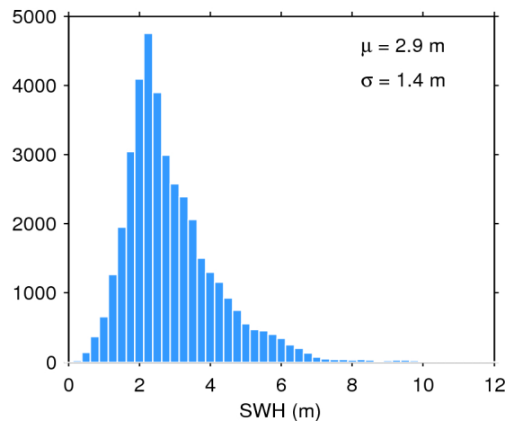
Figure 20. Histogram of science-valid SWH over oceans and lakes for 26/11/2015. The mean ( \mu ) and standard deviation ( \sigma ) are also shown. Note that values larger than 12 m are excluded from the histogram for the sake of readability but not from the computation of \mu and \sigma .
