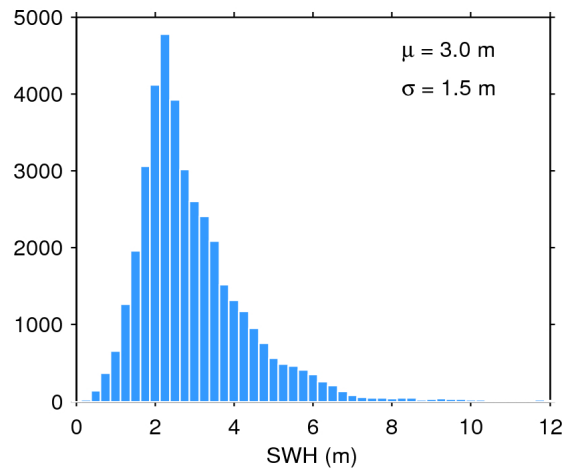
Figure 17. Histogram of flag-valid SWH over oceans and lakes for 26/11/2015. The mean ( \mu ) and standard deviation ( \sigma ) are also shown. Note that values larger than 12 m are excluded from the histogram for the sake of readability but not from the computation of \mu and \sigma .
