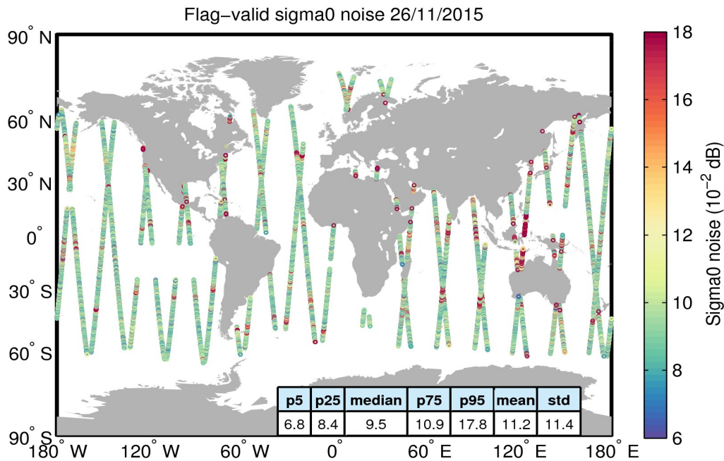
Figure 26. Geographical distribution of flag-valid 20-Hz sigma0 measurement noise over oceans and lakes for 26/11/2015. The statistical values shown in the table refer to the sigma0 noise and are calculated over all measurements shown in the figure.
