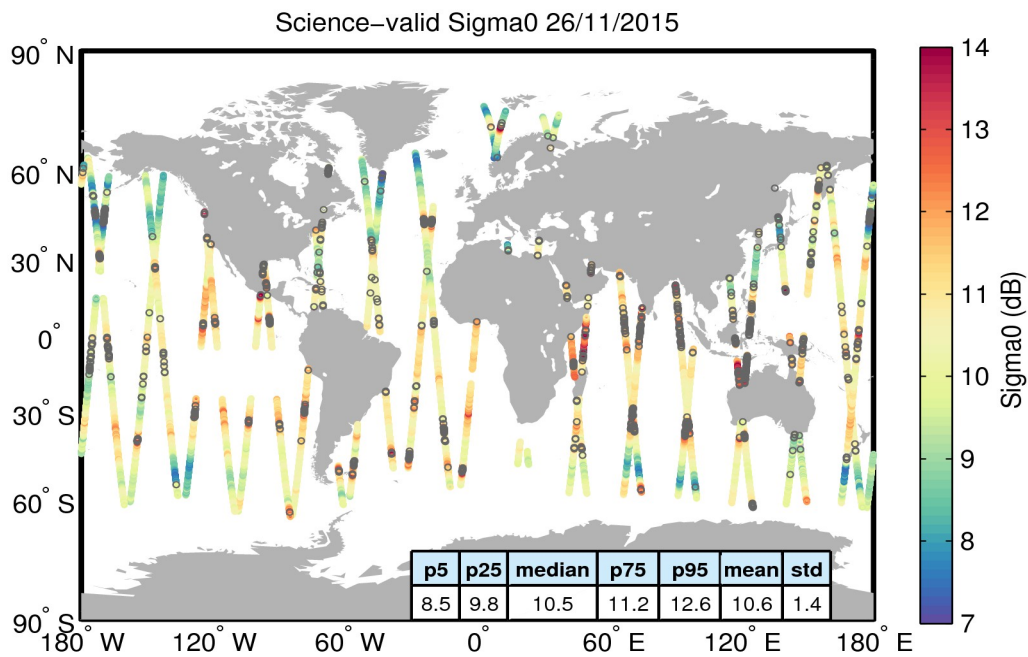
Figure 27. Geographical distribution of science-valid sigma0 data over oceans and lakes for 26/11/2015. The statistical values shown in the table refer to the sigma0 in dB and are calculated over all measurements shown in the figure. Gray circles denote records that have been rejected based on the editing criteria described in Table 4.
