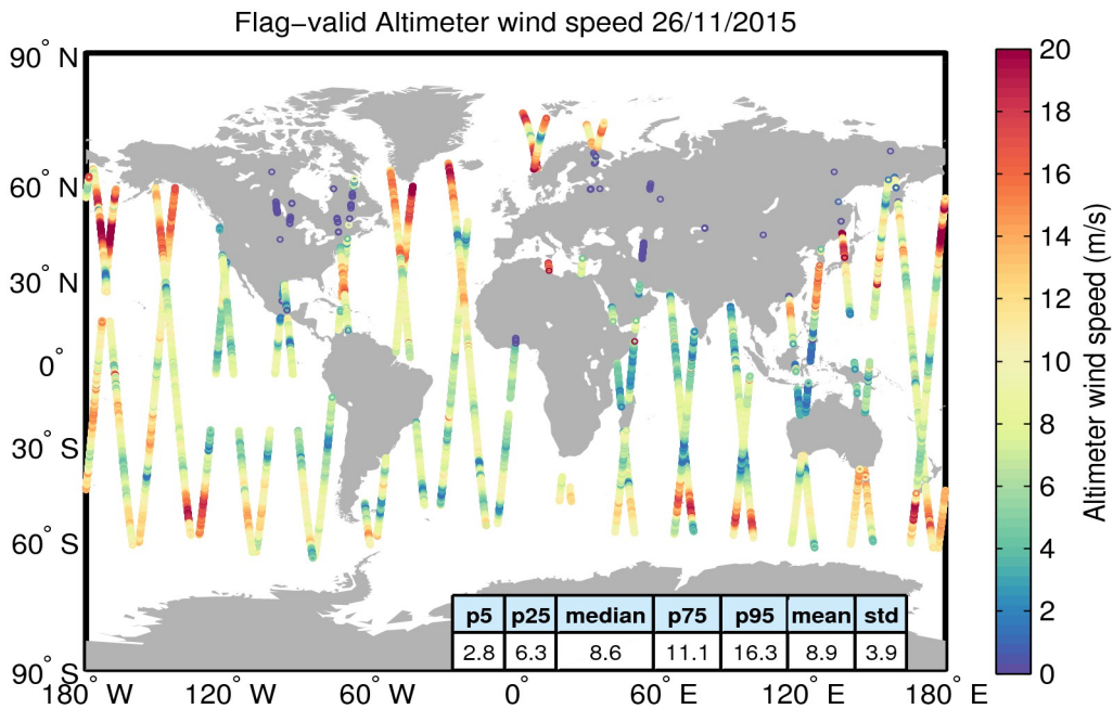
Figure 31. Geographical distribution of flag-valid wind data over oceans and lakes for 26/11/2015. The statistical values shown in the table refer to the wind in m/s and are calculated over all measurements shown in the figure.
