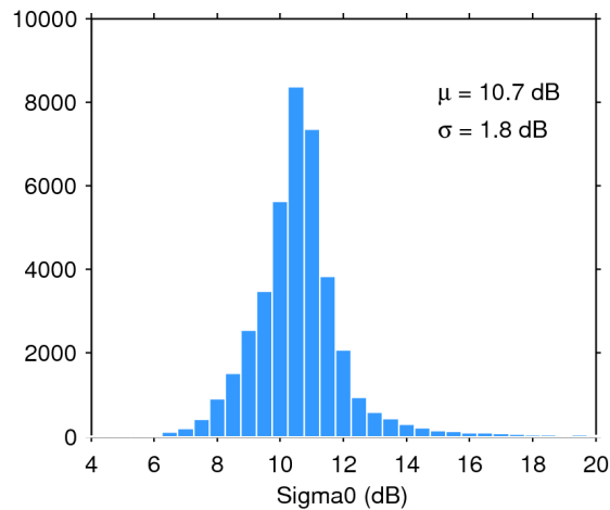
Figure 25. Histogram of flag-valid sigma0 over oceans and lakes for 26/11/2015. The mean ( \mu ) and standard deviation ( \sigma ) are also shown. Note that values outside [4 20] dB are excluded from the histogram for the sake of readability but not from the computation of \mu and \sigma .
