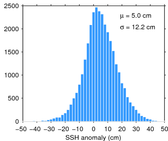
Figure 11. Histogram of science-valid SSH anomaly over oceans and lakes for 26/11/2015. The mean ( \mu ) and standard deviation ( \sigma ) are also shown. Note that values outside [-50 50] cm are excluded from the histogram for the sake of readability but not from the computation of \mu and \sigma .
