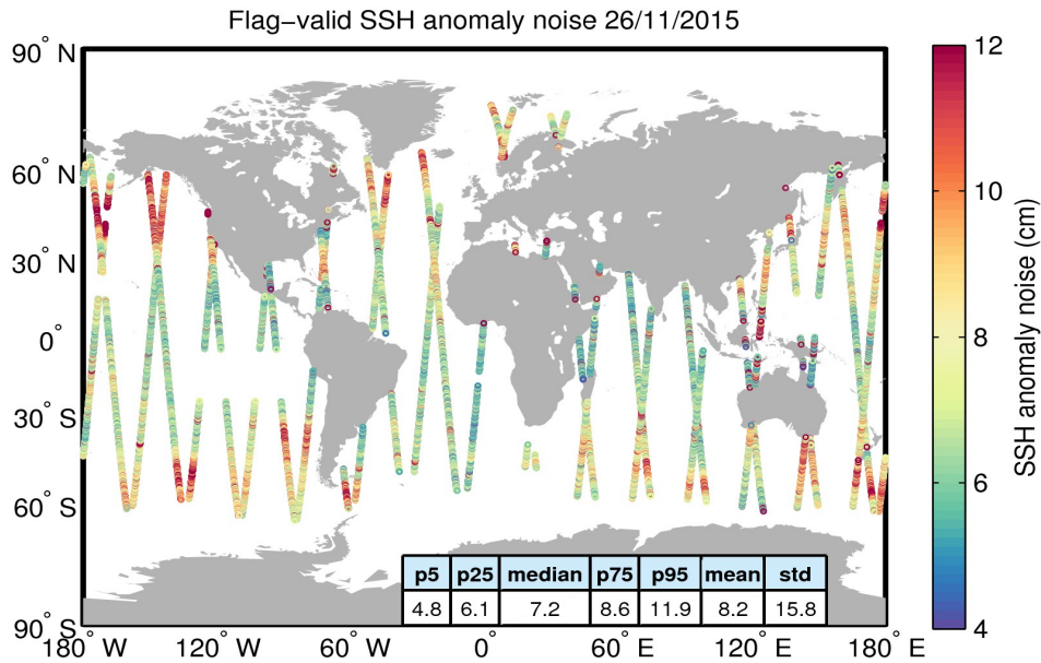
Figure 8. Geographical distribution of flag-valid 20-Hz SSH anomaly measurement noise over oceans and lakes for 26/11/2015. The statistical values shown in the table refer to the SSH anomaly noise and are calculated over all measurements shown in the figure.
