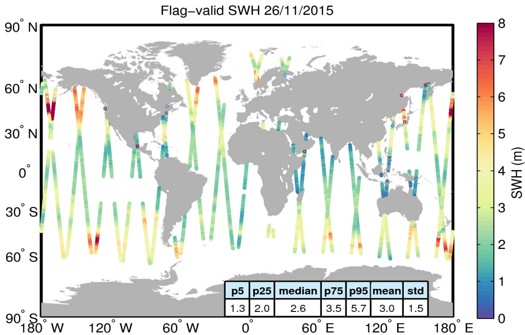
Figure 15. Geographical distribution of flag-valid SWH data over oceans and lakes for 26/11/2015. The statistical values shown in the table refer to the SWH in m and are calculated over all measurements shown in the figure.
