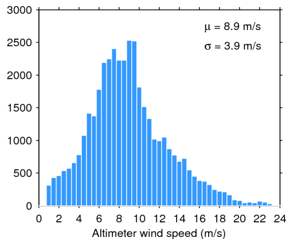
Figure 35. Histogram of science-valid wind over oceans and lakes for 26/11/2015. The mean ( \mu ) and standard deviation ( \sigma ) are also shown. Note that values larger than 24 m/s are excluded from the histogram for the sake of readability but not from the computation of \mu and \sigma .
