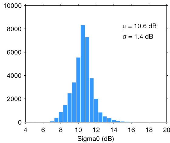
Figure 28. Histogram of science-valid sigma0 over oceans and lakes for 26/11/2015. The mean ( \mu ) and standard deviation ( \sigma ) are also shown. Note that values outside [4 20] dB are excluded from the histogram for the sake of readability but not from the computation of \mu and \sigma .
