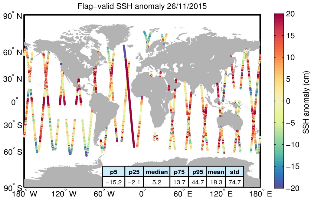
Figure 5. Geographical distribution of flag-valid 1-Hz SSH anomaly data over oceans and lakes for 26/11/2015. The statistical values shown in the table refer to the SSH anomaly in cm and are calculated over all measurements shown in the figure.
