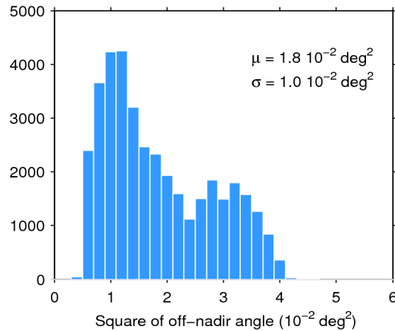
Figure 39. Histogram of flag-valid mispointing over oceans and lakes for 26/11/2015. The mean ( \mu ) and standard deviation ( \sigma ) are also shown. Note that values larger than 6 \cdot 10^{-2} \text{ deg}^2 are excluded from the histogram for the sake of readability but not from the computation of \mu and \sigma .
