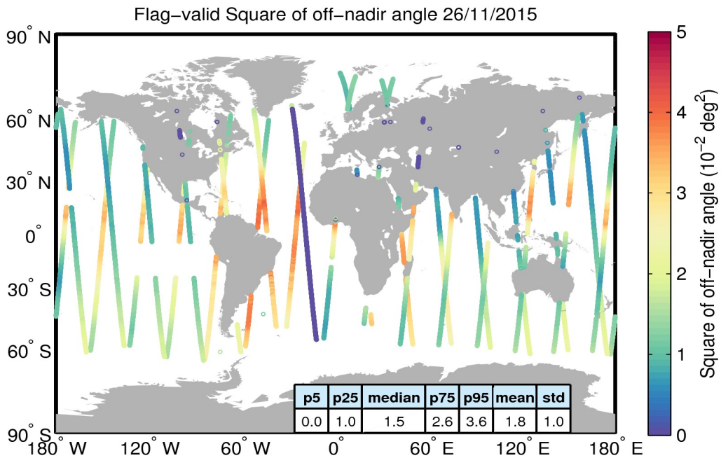
Figure 37. Geographical distribution of flag-valid mispointing data over oceans and lakes for 26/11/2015. The statistical values shown in the table refer to the mispointing in 10^{-2} \text{deg}^2 and are calculated over all measurements shown in the figure.
