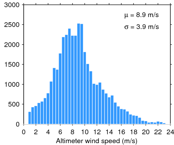
Figure 33. Histogram of flag-valid wind over oceans and lakes for 26/11/2015. The mean ( \mu ) and standard deviation ( \sigma ) are also shown. Note that values larger than 24 m/s are excluded from the histogram for the sake of readability but not from the computation of \mu and \sigma .
