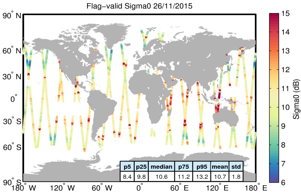
Figure 23. Geographical distribution of flag-valid sigma0 data over oceans and lakes for 26/11/2015. The statistical values shown in the table refer to the sigma0 in dB and are calculated over all measurements shown in the figure.
