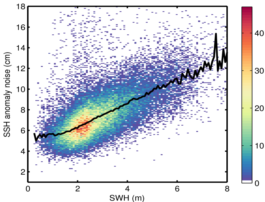
Figure 9. 2D histogram showing flag-valid SSH anomaly noise as a function of SWH for 26/11/2015. The black line denotes the median SSH anomaly noise as a function of SWH.
