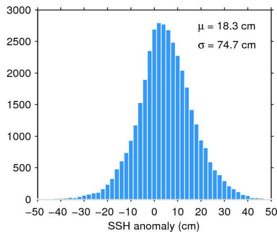
Figure 7. Histogram of flag-valid SSH anomaly over oceans and lakes for 26/11/2015. The mean ( \mu ) and standard deviation ( \sigma ) are also shown. Note that values outside [-50 50] cm are excluded from the histogram for the sake of readability but not from the computation of \mu and \sigma .
