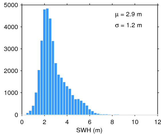
Figure 17. Histogram of flag-valid SWH over oceans and lakes for 25/11/2015. The mean ( \mu ) and standard deviation ( \sigma ) are also shown. Note that values larger than 12 m are excluded from the histogram for the sake of readability but not from the computation of \mu and \sigma .
