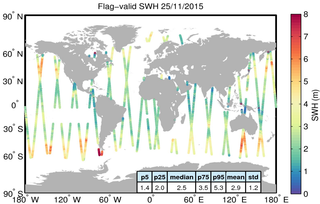
Figure 15. Geographical distribution of flag-valid SWH data over oceans and lakes for 25/11/2015. The statistical values shown in the table refer to the SWH in m and are calculated over all measurements shown in the figure.
