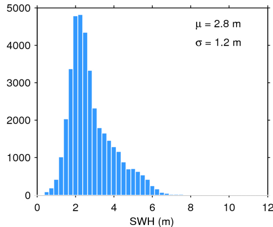
Figure 20. Histogram of science-valid SWH over oceans and lakes for 25/11/2015. The mean ( \mu ) and standard deviation ( \sigma ) are also shown. Note that values larger than 12 m are excluded from the histogram for the sake of readability but not from the computation of \mu and \sigma .
