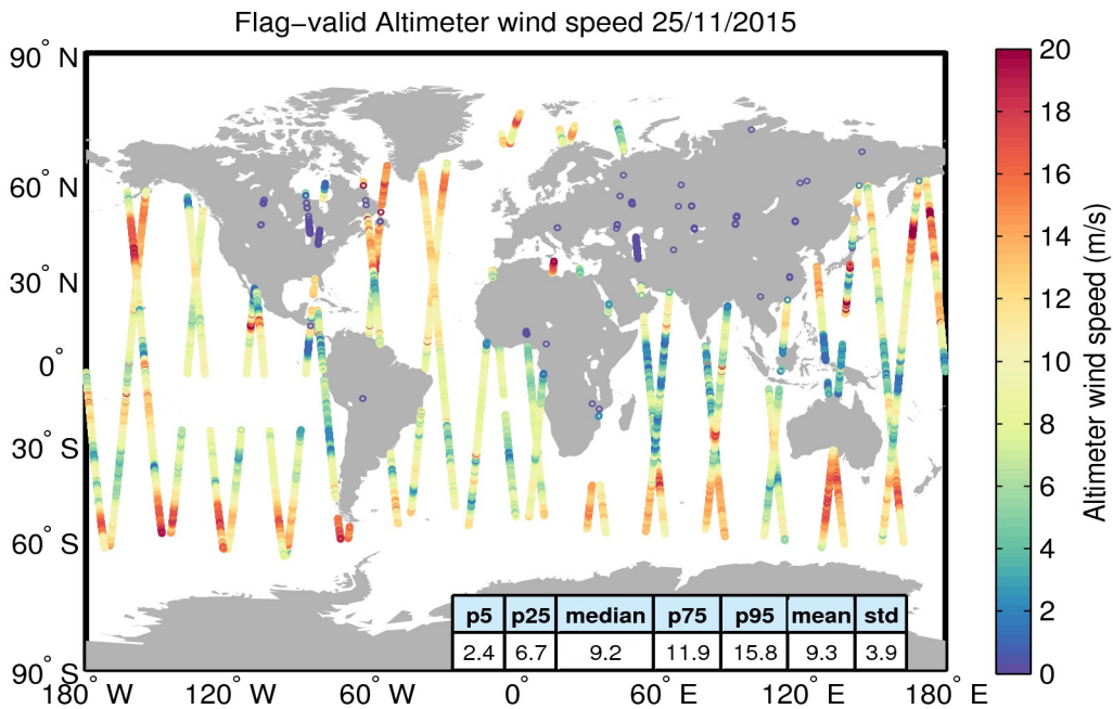
Figure 31. Geographical distribution of flag-valid wind data over oceans and lakes for 25/11/2015. The statistical values shown in the table refer to the wind in m/s and are calculated over all measurements shown in the figure.
