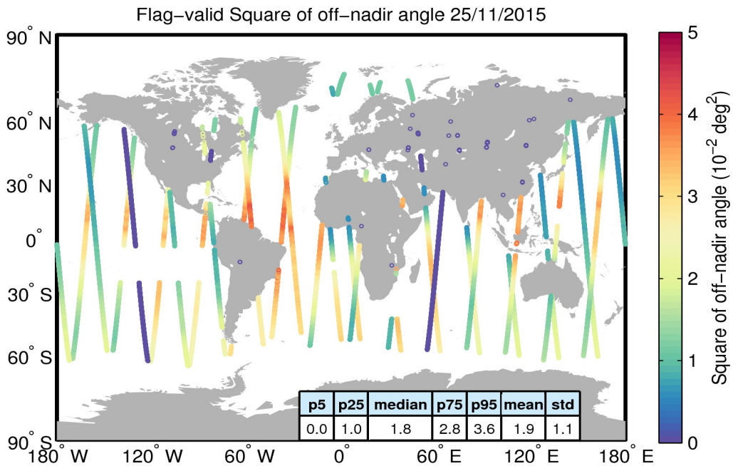
Figure 37. Geographical distribution of flag-valid mispointing data over oceans and lakes for 25/11/2015. The statistical values shown in the table refer to the mispointing in 10^{-2} \text{ deg}^2 and are calculated over all measurements shown in the figure.
