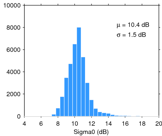
Figure 28. Histogram of science-valid sigma0 over oceans and lakes for 25/11/2015. The mean ( \mu ) and standard deviation ( \sigma ) are also shown. Note that values outside [4 20] dB are excluded from the histogram for the sake of readability but not from the computation of \mu and \sigma .
