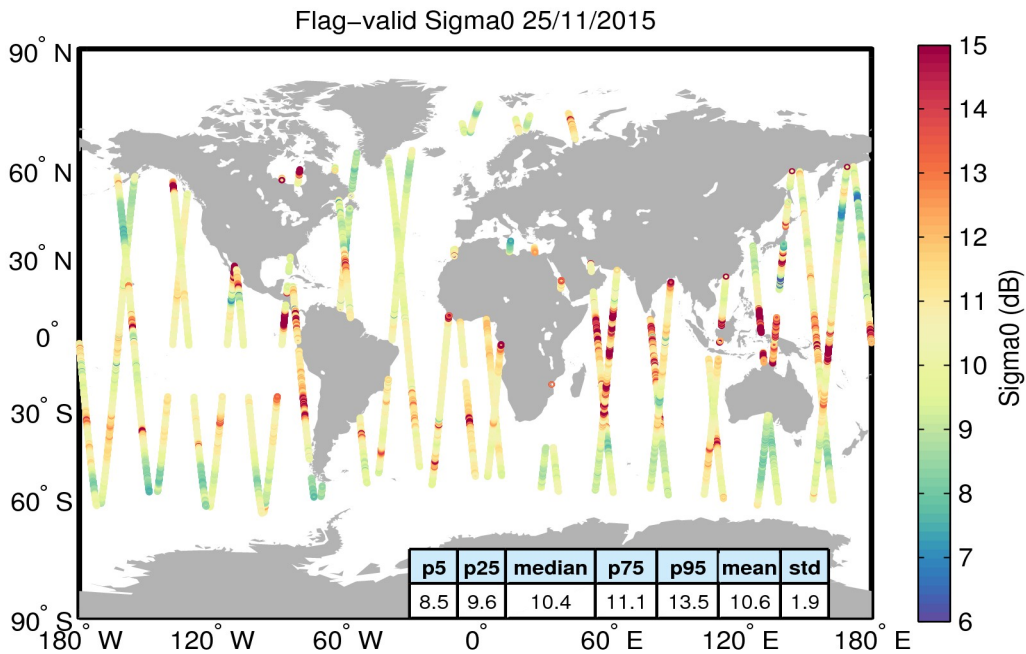
Figure 23. Geographical distribution of flag-valid sigma0 data over oceans and lakes for 25/11/2015. The statistical values shown in the table refer to the sigma0 in dB and are calculated over all measurements shown in the figure.
