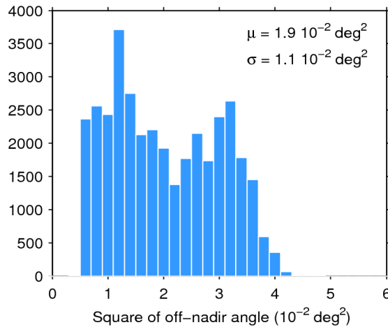
Figure 39. Histogram of flag-valid mispointing over oceans and lakes for 25/11/2015. The mean ( \mu ) and standard deviation ( \sigma ) are also shown. Note that values larger than 6 \cdot 10^{-2} \text{ deg}^2 are excluded from the histogram for the sake of readability but not from the computation of \mu and \sigma .
