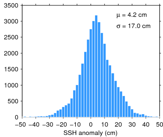
Figure 7. Histogram of flag-valid SSH anomaly over oceans and lakes for 25/11/2015. The mean ( \mu ) and standard deviation ( \sigma ) are also shown. Note that values outside [-50 50] cm are excluded from the histogram for the sake of readability but not from the computation of \mu and \sigma .
