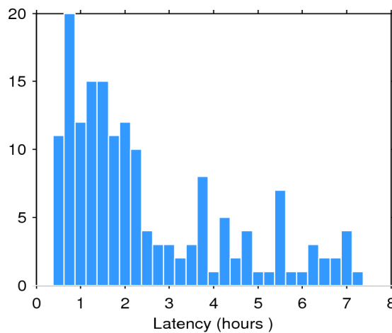
Figure 2. Histogram of the data latency for 25/11/2015. The y-axis denotes the number of files that are made available with a delay of x-hours with respect to the mean time of the records stored in the file.
