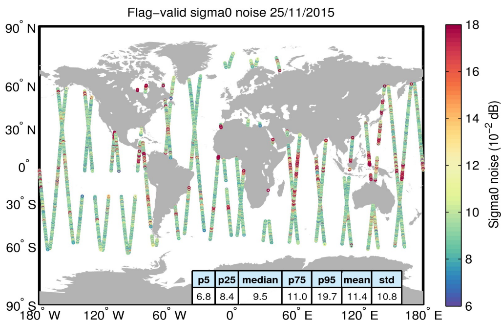
Figure 26. Geographical distribution of flag-valid 20-Hz sigma0 measurement noise over oceans and lakes for 25/11/2015. The statistical values shown in the table refer to the sigma0 noise and are calculated over all measurements shown in the figure.
