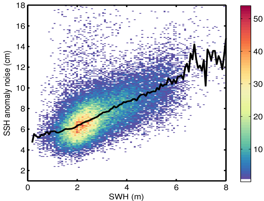
Figure 9. 2D histogram showing flag-valid SSH anomaly noise as a function of SWH for 25/11/2015. The black line denotes the median SSH anomaly noise as a function of SWH.
