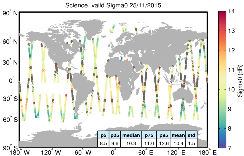
Figure 27. Geographical distribution of science-valid sigma0 data over oceans and lakes for 25/11/2015. The statistical values shown in the table refer to the sigma0 in dB and are calculated over all measurements shown in the figure. Gray circles denote records that have been rejected based on the editing criteria described in Table 4.
