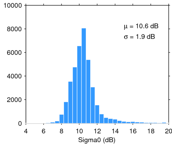
Figure 25. Histogram of flag-valid sigma0 over oceans and lakes for 25/11/2015. The mean ( \mu ) and standard deviation ( \sigma ) are also shown. Note that values outside [4 20] dB are excluded from the histogram for the sake of readability but not from the computation of \mu and \sigma .
