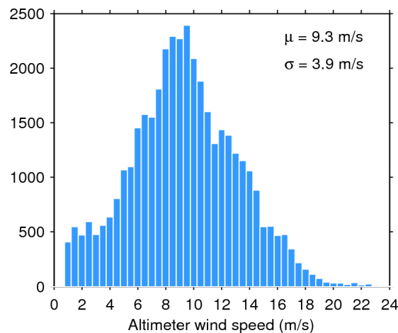
Figure 35. Histogram of science-valid wind over oceans and lakes for 25/11/2015. The mean ( \mu ) and standard deviation ( \sigma ) are also shown. Note that values larger than 24 m/s are excluded from the histogram for the sake of readability but not from the computation of \mu and \sigma .
