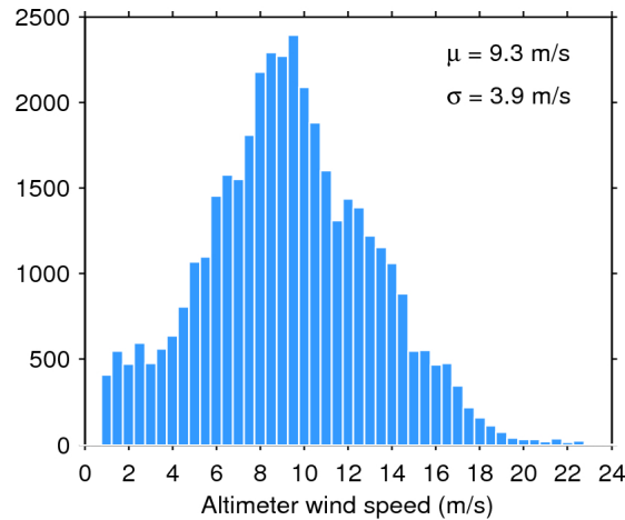
Figure 33. Histogram of flag-valid wind over oceans and lakes for 25/11/2015. The mean ( \mu ) and standard deviation ( \sigma ) are also shown. Note that values larger than 24 m/s are excluded from the histogram for the sake of readability but not from the computation of \mu and \sigma .
