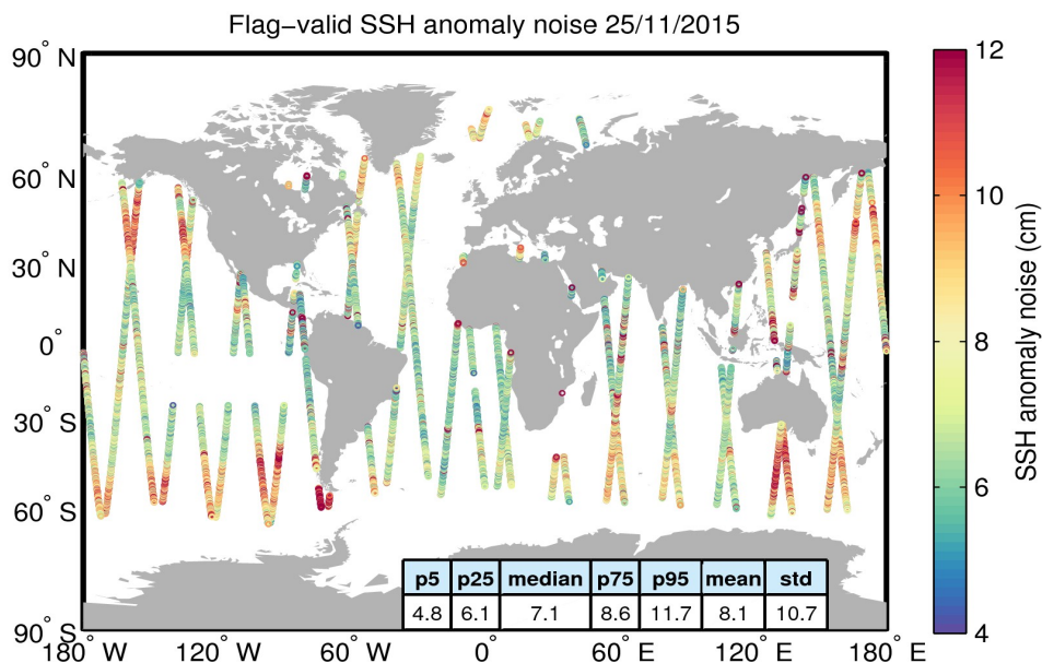
Figure 8. Geographical distribution of flag-valid 20-Hz SSH anomaly measurement noise over oceans and lakes for 25/11/2015. The statistical values shown in the table refer to the SSH anomaly noise and are calculated over all measurements shown in the figure.
