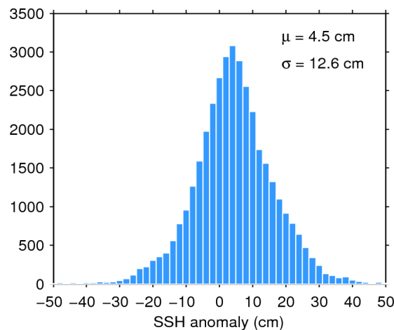
Figure 11. Histogram of science-valid SSH anomaly over oceans and lakes for 25/11/2015. The mean ( \mu ) and standard deviation ( \sigma ) are also shown. Note that values outside [-50 50] cm are excluded from the histogram for the sake of readability but not from the computation of \mu and \sigma .
