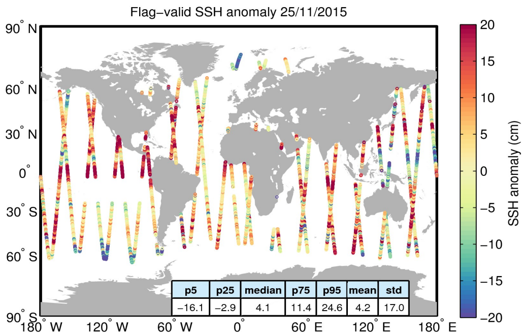
Figure 5. Geographical distribution of flag-valid 1-Hz SSH anomaly data over oceans and lakes for 25/11/2015. The statistical values shown in the table refer to the SSH anomaly in cm and are calculated over all measurements shown in the figure.
