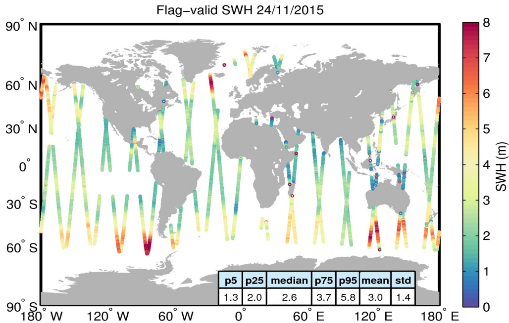
Figure 15. Geographical distribution of flag-valid SWH data over oceans and lakes for 24/11/2015. The statistical values shown in the table refer to the SWH in m and are calculated over all measurements shown in the figure.
