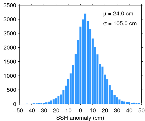
Figure 7. Histogram of flag-valid SSH anomaly over oceans and lakes for 24/11/2015. The mean ( \mu ) and standard deviation ( \sigma ) are also shown. Note that values outside [-50 50] cm are excluded from the histogram for the sake of readability but not from the computation of \mu and \sigma .
