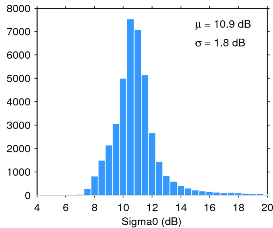
Figure 25. Histogram of flag-valid sigma0 over oceans and lakes for 24/11/2015. The mean ( \mu ) and standard deviation ( \sigma ) are also shown. Note that values outside [4 20] dB are excluded from the histogram for the sake of readability but not from the computation of \mu and \sigma .
