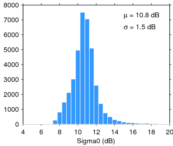
Figure 28. Histogram of science-valid sigma0 over oceans and lakes for 24/11/2015. The mean ( \mu ) and standard deviation ( \sigma ) are also shown. Note that values outside [4 20] dB are excluded from the histogram for the sake of readability but not from the computation of \mu and \sigma .
