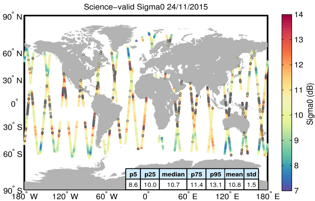
Figure 27. Geographical distribution of science-valid sigma0 data over oceans and lakes for 24/11/2015. The statistical values shown in the table refer to the sigma0 in dB and are calculated over all measurements shown in the figure. Gray circles denote records that have been rejected based on the editing criteria described in Table 4.
