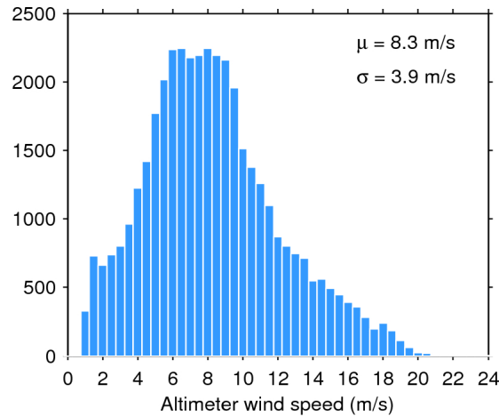
Figure 33. Histogram of flag-valid wind over oceans and lakes for 24/11/2015. The mean ( \mu ) and standard deviation ( \sigma ) are also shown. Note that values larger than 24 m/s are excluded from the histogram for the sake of readability but not from the computation of \mu and \sigma .
