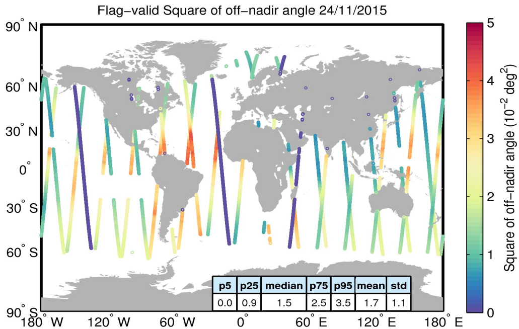
Figure 37. Geographical distribution of flag-valid mispointing data over oceans and lakes for 24/11/2015. The statistical values shown in the table refer to the mispointing in 10^{-2} \text{ deg}^2 and are calculated over all measurements shown in the figure.
