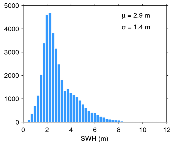
Figure 20. Histogram of science-valid SWH over oceans and lakes for 24/11/2015. The mean ( \mu ) and standard deviation ( \sigma ) are also shown. Note that values larger than 12 m are excluded from the histogram for the sake of readability but not from the computation of \mu and \sigma .
