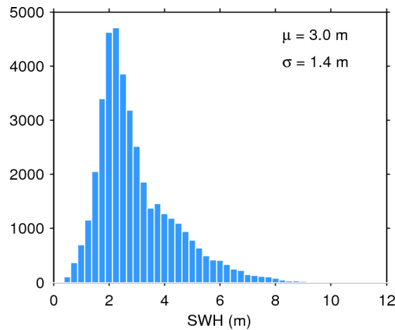
Figure 17. Histogram of flag-valid SWH over oceans and lakes for 24/11/2015. The mean ( \mu ) and standard deviation ( \sigma ) are also shown. Note that values larger than 12 m are excluded from the histogram for the sake of readability but not from the computation of \mu and \sigma .
