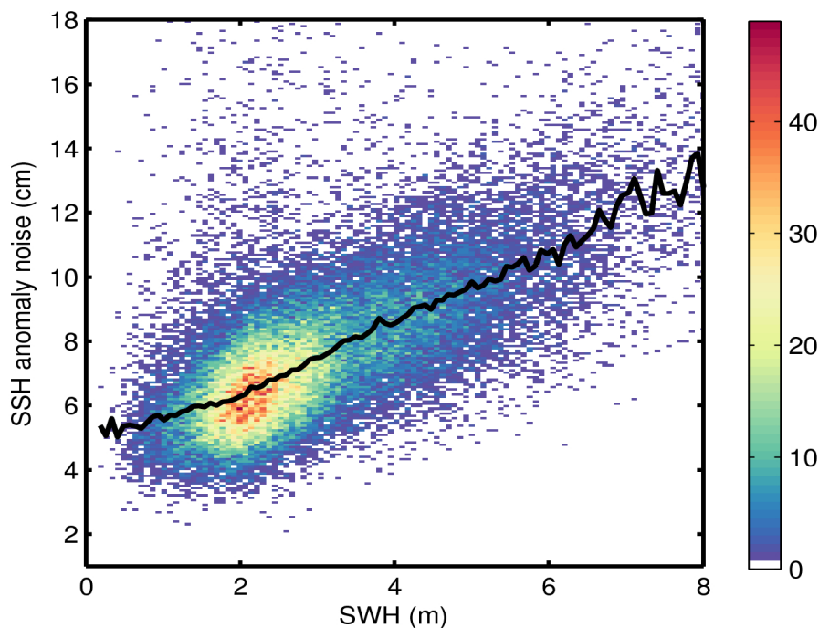
Figure 9. 2D histogram showing flag-valid SSH anomaly noise as a function of SWH for 24/11/2015. The black line denotes the median SSH anomaly noise as a function of SWH.
