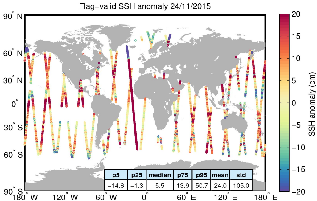
Figure 5. Geographical distribution of flag-valid 1-Hz SSH anomaly data over oceans and lakes for 24/11/2015. The statistical values shown in the table refer to the SSH anomaly in cm and are calculated over all measurements shown in the figure.
