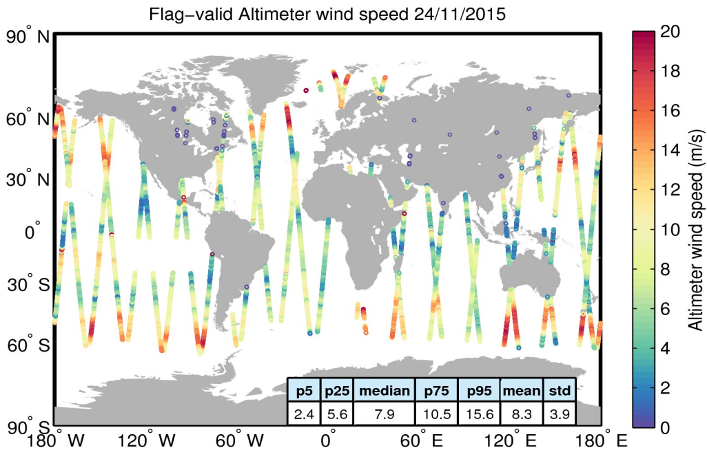
Figure 31. Geographical distribution of flag-valid wind data over oceans and lakes for 24/11/2015. The statistical values shown in the table refer to the wind in m/s and are calculated over all measurements shown in the figure.
