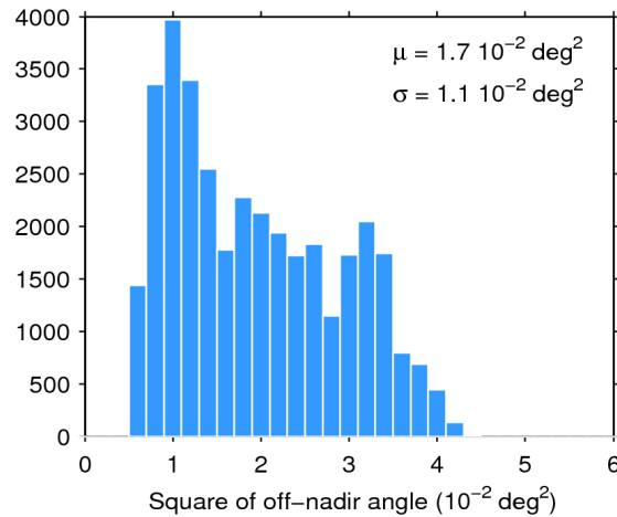
Figure 39. Histogram of flag-valid mispointing over oceans and lakes for 24/11/2015. The mean ( \mu ) and standard deviation ( \sigma ) are also shown. Note that values larger than 6 \cdot 10^{-2} \text{ deg}^2 are excluded from the histogram for the sake of readability but not from the computation of \mu and \sigma .
