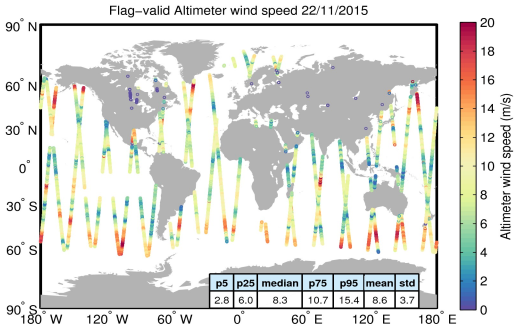
Figure 31. Geographical distribution of flag-valid wind data over oceans and lakes for 22/11/2015. The statistical values shown in the table refer to the wind in m/s and are calculated over all measurements shown in the figure.
