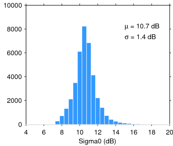
Figure 28. Histogram of science-valid sigma0 over oceans and lakes for 22/11/2015. The mean ( \mu ) and standard deviation ( \sigma ) are also shown. Note that values outside [4 20] dB are excluded from the histogram for the sake of readability but not from the computation of \mu and \sigma .
