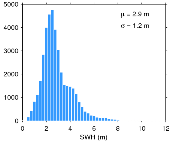
Figure 20. Histogram of science-valid SWH over oceans and lakes for 22/11/2015. The mean ( \mu ) and standard deviation ( \sigma ) are also shown. Note that values larger than 12 m are excluded from the histogram for the sake of readability but not from the computation of \mu and \sigma .
