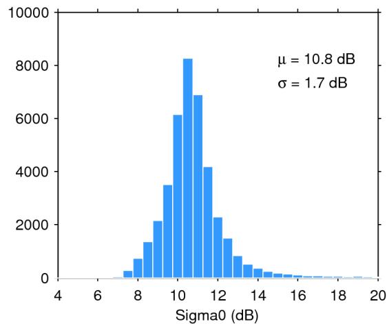
Figure 25. Histogram of flag-valid sigma0 over oceans and lakes for 22/11/2015. The mean ( \mu ) and standard deviation ( \sigma ) are also shown. Note that values outside [4 20] dB are excluded from the histogram for the sake of readability but not from the computation of \mu and \sigma .
