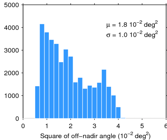
Figure 39. Histogram of flag-valid mispointing over oceans and lakes for 22/11/2015. The mean ( \mu ) and standard deviation ( \sigma ) are also shown. Note that values larger than 6 \cdot 10^{-2} \text{ deg}^2 are excluded from the histogram for the sake of readability but not from the computation of \mu and \sigma .
