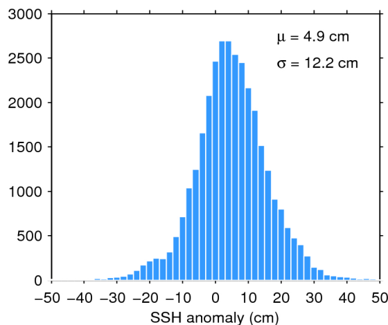
Figure 11. Histogram of science-valid SSH anomaly over oceans and lakes for 22/11/2015. The mean ( \mu ) and standard deviation ( \sigma ) are also shown. Note that values outside [-50 50] cm are excluded from the histogram for the sake of readability but not from the computation of \mu and \sigma .
