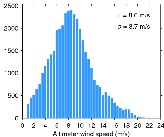
Figure 35. Histogram of science-valid wind over oceans and lakes for 22/11/2015. The mean ( \mu ) and standard deviation ( \sigma ) are also shown. Note that values larger than 24 m/s are excluded from the histogram for the sake of readability but not from the computation of \mu and \sigma .
