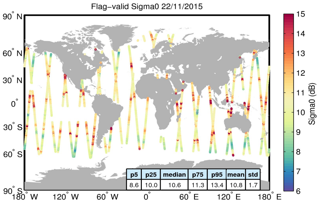
Figure 23. Geographical distribution of flag-valid sigma0 data over oceans and lakes for 22/11/2015. The statistical values shown in the table refer to the sigma0 in dB and are calculated over all measurements shown in the figure.
