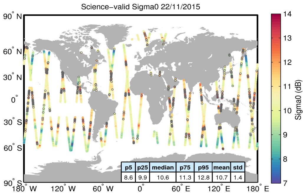
Figure 27. Geographical distribution of science-valid sigma0 data over oceans and lakes for 22/11/2015. The statistical values shown in the table refer to the sigma0 in dB and are calculated over all measurements shown in the figure. Gray circles denote records that have been rejected based on the editing criteria described in Table 4.
