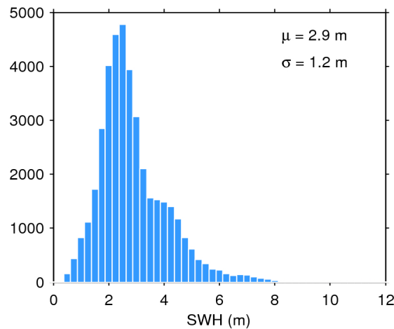
Figure 17. Histogram of flag-valid SWH over oceans and lakes for 22/11/2015. The mean ( \mu ) and standard deviation ( \sigma ) are also shown. Note that values larger than 12 m are excluded from the histogram for the sake of readability but not from the computation of \mu and \sigma .
