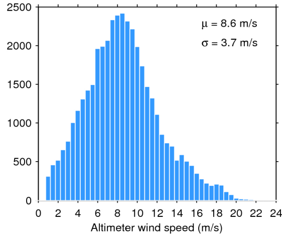
Figure 33. Histogram of flag-valid wind over oceans and lakes for 22/11/2015. The mean ( \mu ) and standard deviation ( \sigma ) are also shown. Note that values larger than 24 m/s are excluded from the histogram for the sake of readability but not from the computation of \mu and \sigma .
