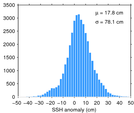
Figure 7. Histogram of flag-valid SSH anomaly over oceans and lakes for 22/11/2015. The mean ( \mu ) and standard deviation ( \sigma ) are also shown. Note that values outside [-50 50] cm are excluded from the histogram for the sake of readability but not from the computation of \mu and \sigma .
