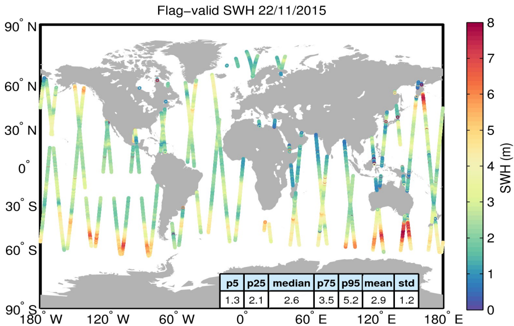
Figure 15. Geographical distribution of flag-valid SWH data over oceans and lakes for 22/11/2015. The statistical values shown in the table refer to the SWH in m and are calculated over all measurements shown in the figure.
