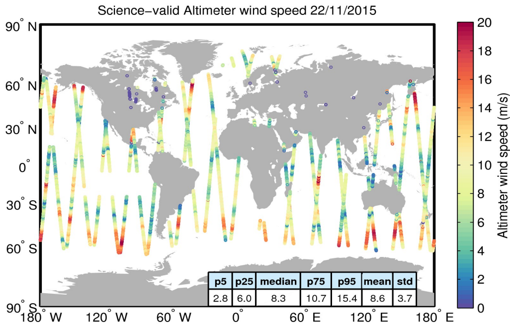
Figure 34. Geographical distribution of science-valid wind data over oceans and lakes for 22/11/2015. The statistical values shown in the table refer to the wind in m/s and are calculated over all measurements shown in the figure. Gray circles denote records that have been rejected based on the editing criteria described in Table 5.
