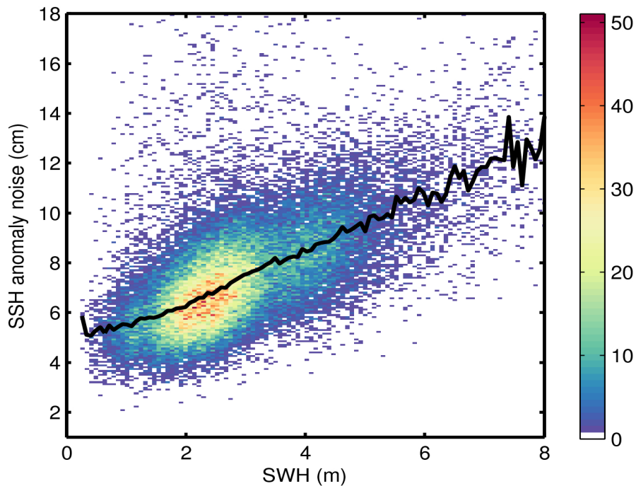
Figure 9. 2D histogram showing flag-valid SSH anomaly noise as a function of SWH for 22/11/2015. The black line denotes the median SSH anomaly noise as a function of SWH.
