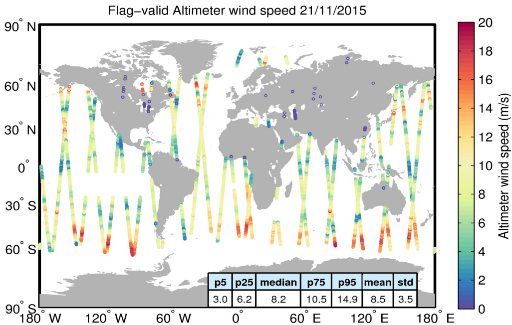
Figure 31. Geographical distribution of flag-valid wind data over oceans and lakes for 21/11/2015. The statistical values shown in the figure refer to the wind in m/s and are calculated over all measurements shown in the figure.
