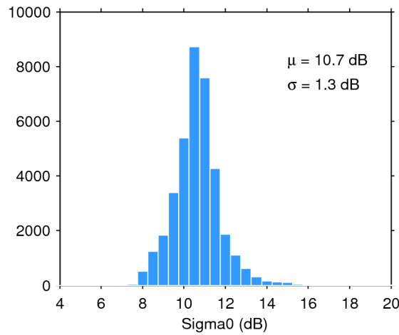
Figure 28. Histogram of science-valid sigma0 over oceans and lakes for 21/11/2015. The mean ( \mu ) and standard deviation ( \sigma ) are also shown. Note that values outside [4 20] dB are excluded from the histogram for the sake of readability but not from the computation of \mu and \sigma .
