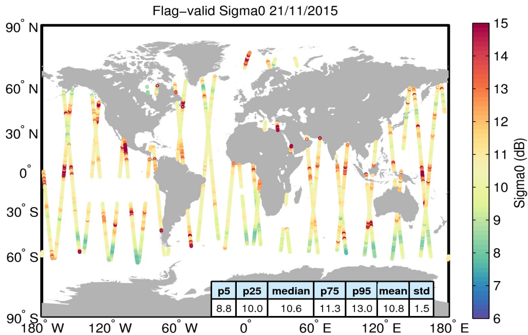
Figure 23. Geographical distribution of flag-valid sigma0 data over oceans and lakes for 21/11/2015. The statistical values shown in the table refer to the sigma0 in dB and are calculated over all measurements shown in the figure.
