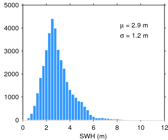
Figure 20. Histogram of science-valid SWH over oceans and lakes for 21/11/2015. The mean ( \mu ) and standard deviation ( \sigma ) are also shown. Note that values larger than 12 m are excluded from the histogram for the sake of readability but not from the computation of \mu and \sigma .
