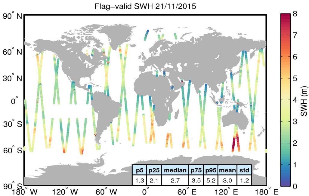
Figure 15. Geographical distribution of flag-valid SWH data over oceans and lakes for 21/11/2015. The statistical values shown in the table refer to the SWH in m and are calculated over all measurements shown in the figure.
