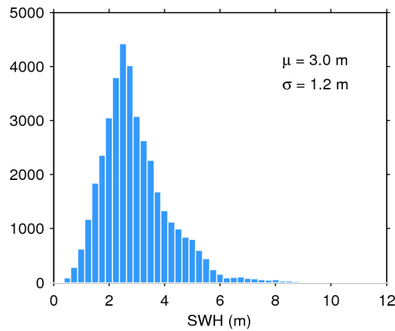
Figure 17. Histogram of flag-valid SWH over oceans and lakes for 21/11/2015. The mean ( \mu ) and standard deviation ( \sigma ) are also shown. Note that values larger than 12 m are excluded from the histogram for the sake of readability but not from the computation of \mu and \sigma .
