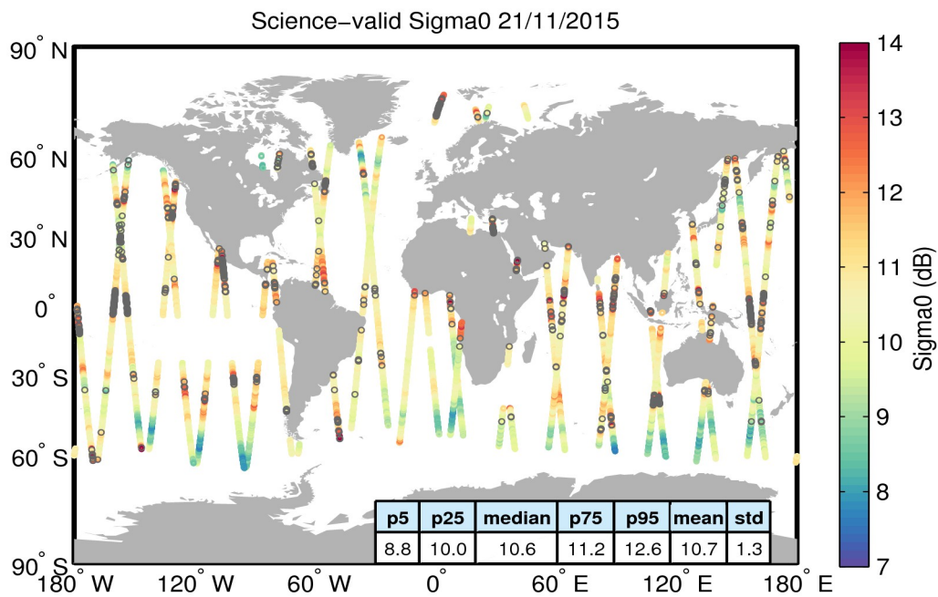
Figure 27. Geographical distribution of science-valid sigma0 data over oceans and lakes for 21/11/2015. The statistical values shown in the table refer to the sigma0 in dB and are calculated over all measurements shown in the figure. Gray circles denote records that have been rejected based on the editing criteria described in Table 4.
