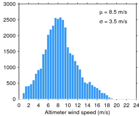
Figure 33. Histogram of flag-valid wind over oceans and lakes for 21/11/2015. The mean ( \mu ) and standard deviation ( \sigma ) are also shown. Note that values larger than 24 m/s are excluded from the histogram for the sake of readability but not from the computation of \mu and \sigma .
