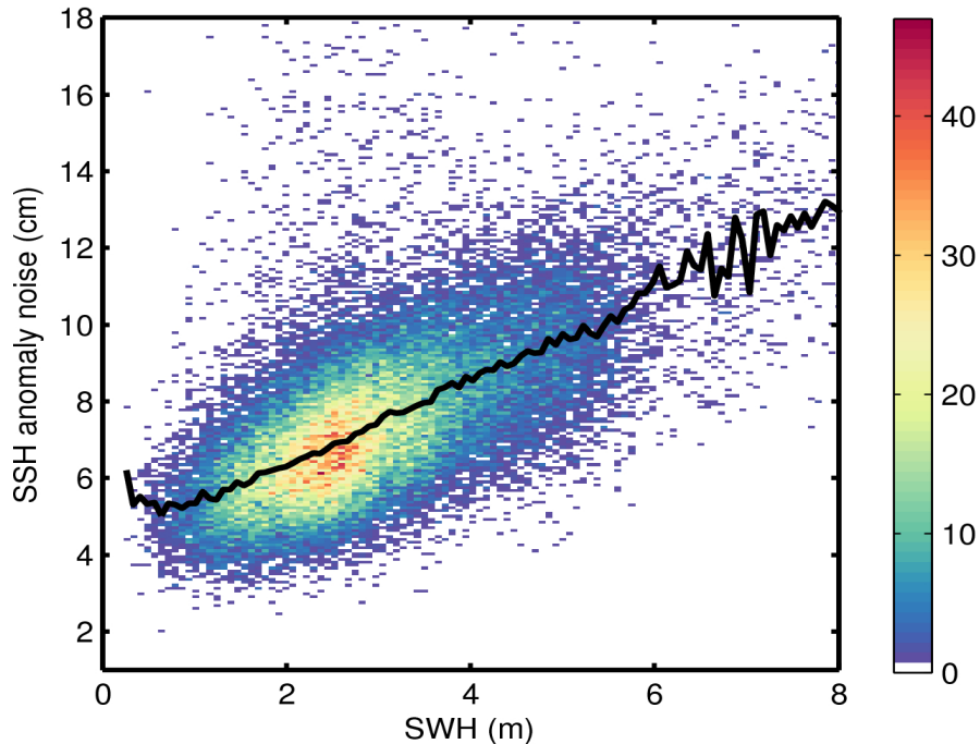
Figure 9. 2D histogram showing flag-valid SSH anomaly noise as a function of SWH for 21/11/2015. The black line denotes the median SSH anomaly noise as a function of SWH.
