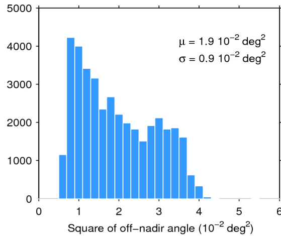
Figure 39. Histogram of flag-valid mispointing over oceans and lakes for 21/11/2015. The mean ( \mu ) and standard deviation ( \sigma ) are also shown. Note that values larger than 6 \cdot 10^{-2} \text{ deg}^2 are excluded from the histogram for the sake of readability but not from the computation of \mu and \sigma .
