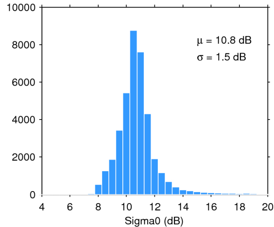
Figure 25. Histogram of flag-valid sigma0 over oceans and lakes for 21/11/2015. The mean ( \mu ) and standard deviation ( \sigma ) are also shown. Note that values outside [4 20] dB are excluded from the histogram for the sake of readability but not from the computation of \mu and \sigma .
