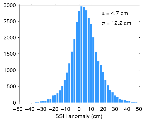
Figure 11. Histogram of science-valid SSH anomaly over oceans and lakes for 21/11/2015. The mean ( \mu ) and standard deviation ( \sigma ) are also shown. Note that values outside [-50 50] cm are excluded from the histogram for the sake of readability but not from the computation of \mu and \sigma .
