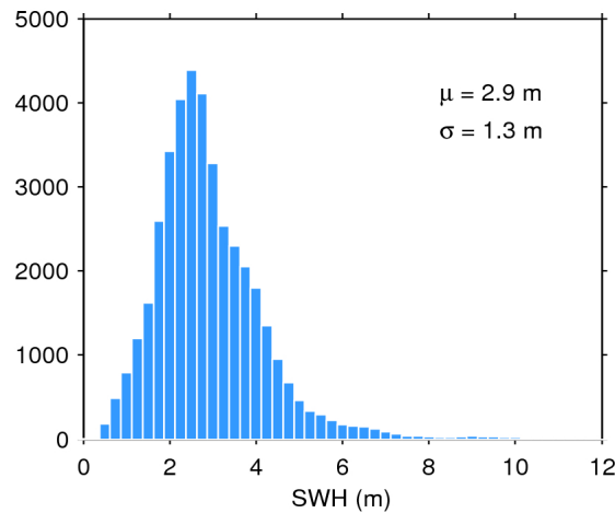
Figure 17. Histogram of flag-valid SWH over oceans and lakes for 20/11/2015. The mean ( \mu ) and standard deviation ( \sigma ) are also shown. Note that values larger than 12 m are excluded from the histogram for the sake of readability but not from the computation of \mu and \sigma .
