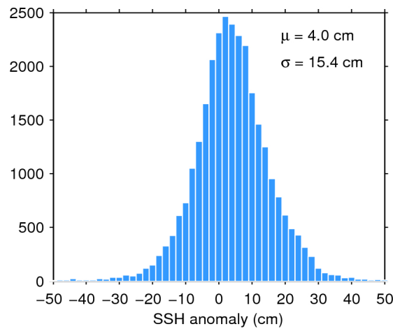
Figure 7. Histogram of flag-valid SSH anomaly over oceans and lakes for 20/11/2015. The mean ( \mu ) and standard deviation ( \sigma ) are also shown. Note that values outside [-50\ 50] cm are excluded from the histogram for the sake of readability but not from the computation of \mu and \sigma .
