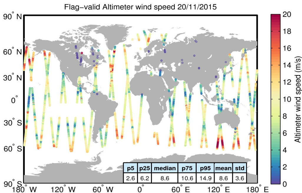
Figure 31. Geographical distribution of flag-valid wind data over oceans and lakes for 20/11/2015. The statistical values shown in the table refer to the wind in m/s and are calculated over all measurements shown in the figure.
