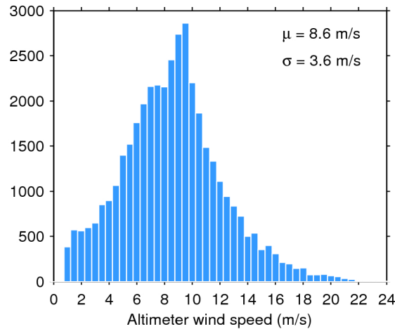
Figure 33. Histogram of flag-valid wind over oceans and lakes for 20/11/2015. The mean ( \mu ) and standard deviation ( \sigma ) are also shown. Note that values larger than 24 m/s are excluded from the histogram for the sake of readability but not from the computation of \mu and \sigma .
