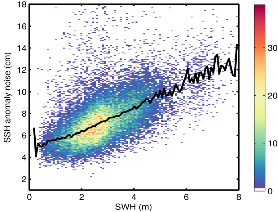
Figure 9. 2D histogram showing flag-valid SSH anomaly noise as a function of SWH for 20/11/2015. The black line denotes the median SSH anomaly noise as a function of SWH.
