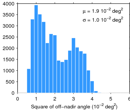
Figure 39. Histogram of flag-valid mispointing over oceans and lakes for 20/11/2015. The mean ( \mu ) and standard deviation ( \sigma ) are also shown. Note that values larger than 6 \cdot 10^{-2} \text{ deg}^2 are excluded from the histogram for the sake of readability but not from the computation of \mu and \sigma .
