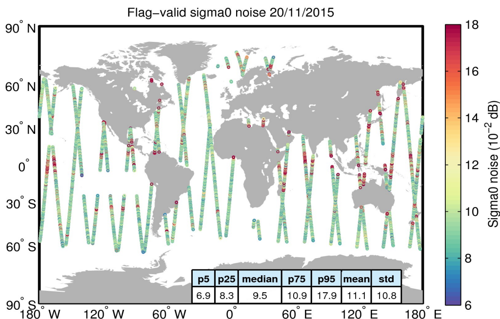
Figure 26. Geographical distribution of flag-valid 20-Hz sigma0 measurement noise over oceans and lakes for 20/11/2015. The statistical values shown in the table refer to the sigma0 noise and are calculated over all measurements shown in the figure.
