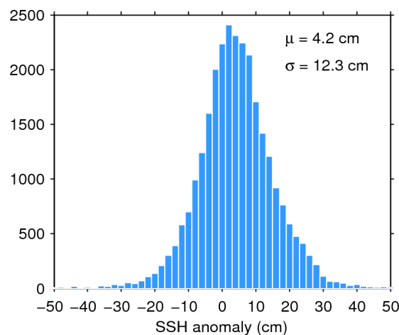
Figure 11. Histogram of science-valid SSH anomaly over oceans and lakes for 20/11/2015. The mean ( \mu ) and standard deviation ( \sigma ) are also shown. Note that values outside [-50 50] cm are excluded from the histogram for the sake of readability but not from the computation of \mu and \sigma .
