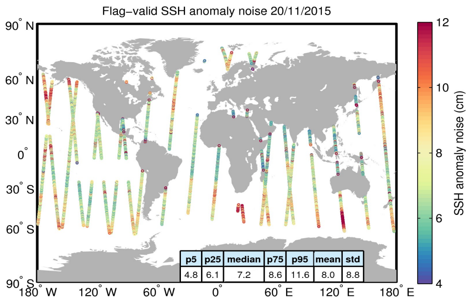
Figure 8. Geographical distribution of flag-valid 20-Hz SSH anomaly measurement noise over oceans and lakes for 20/11/2015. The statistical values shown in the table refer to the SSH anomaly noise and are calculated over all measurements shown in the figure.
