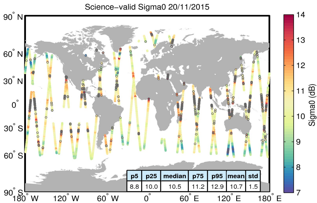
Figure 27. Geographical distribution of science-valid sigma0 data over oceans and lakes for 20/11/2015. The statistical values shown in the table refer to the sigma0 in dB and are calculated over all measurements shown in the figure. Gray circles denote records that have been rejected based on the editing criteria described in Table 4.
