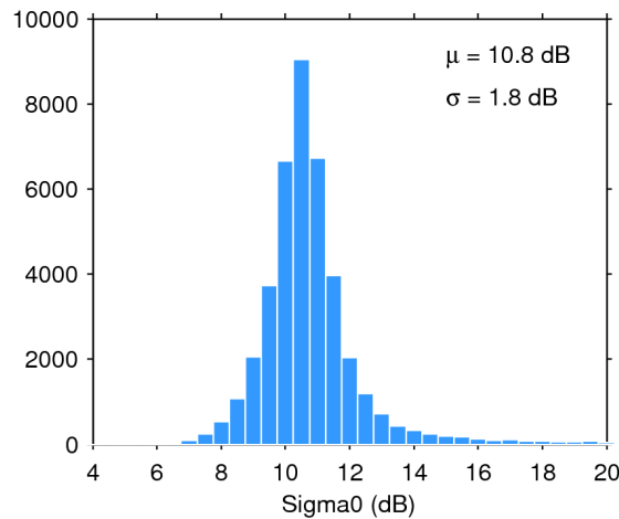
Figure 25. Histogram of flag-valid sigma0 over oceans and lakes for 20/11/2015. The mean ( \mu ) and standard deviation ( \sigma ) are also shown. Note that values outside [4 20] dB are excluded from the histogram for the sake of readability but not from the computation of \mu and \sigma .
