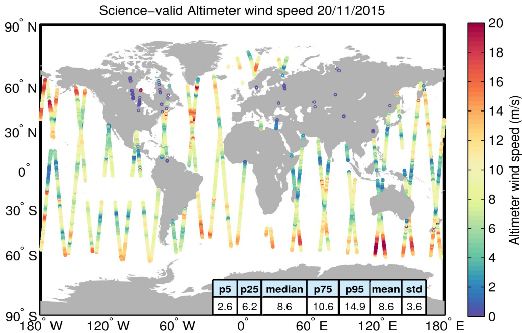
Figure 34. Geographical distribution of science-valid wind data over oceans and lakes for 20/11/2015. The statistical values shown in the table refer to the wind in m/s and are calculated over all measurements shown in the figure. Gray circles denote records that have been rejected based on the editing criteria described in Table 5.
