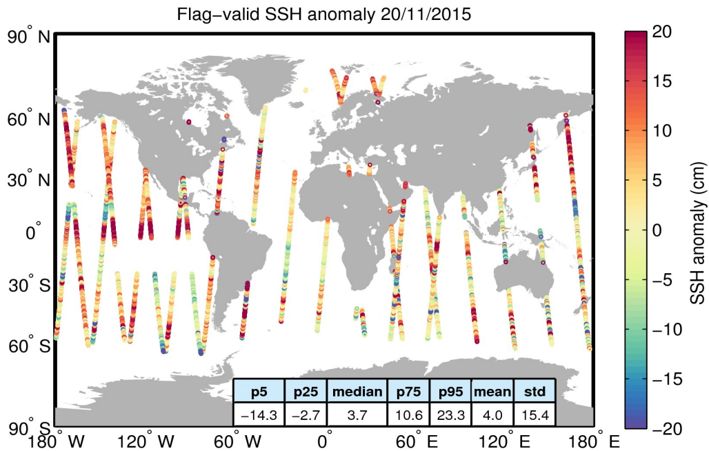
Figure 5. Geographical distribution of flag-valid 1-Hz SSH anomaly data over oceans and lakes for 20/11/2015. The statistical values shown in the table refer to the SSH anomaly in cm and are calculated over all measurements shown in the figure.
