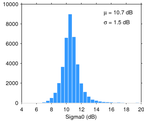
Figure 28. Histogram of science-valid sigma0 over oceans and lakes for 20/11/2015. The mean ( \mu ) and standard deviation ( \sigma ) are also shown. Note that values outside [4 20] dB are excluded from the histogram for the sake of readability but not from the computation of \mu and \sigma .
