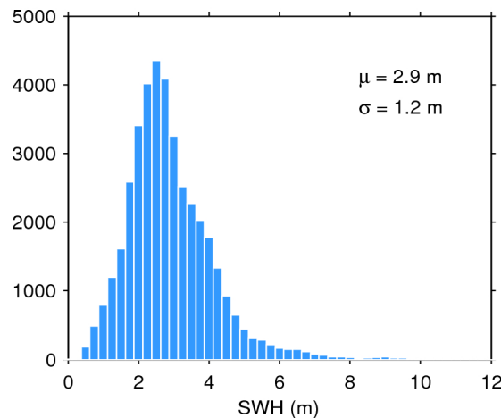
Figure 20. Histogram of science-valid SWH over oceans and lakes for 20/11/2015. The mean ( \mu ) and standard deviation ( \sigma ) are also shown. Note that values larger than 12 m are excluded from the histogram for the sake of readability but not from the computation of \mu and \sigma .
