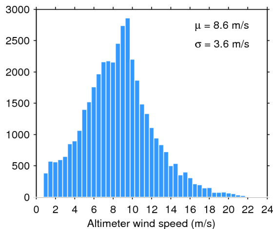
Figure 35. Histogram of science-valid wind over oceans and lakes for 20/11/2015. The mean ( \mu ) and standard deviation ( \sigma ) are also shown. Note that values larger than 24 m/s are excluded from the histogram for the sake of readability but not from the computation of \mu and \sigma .
