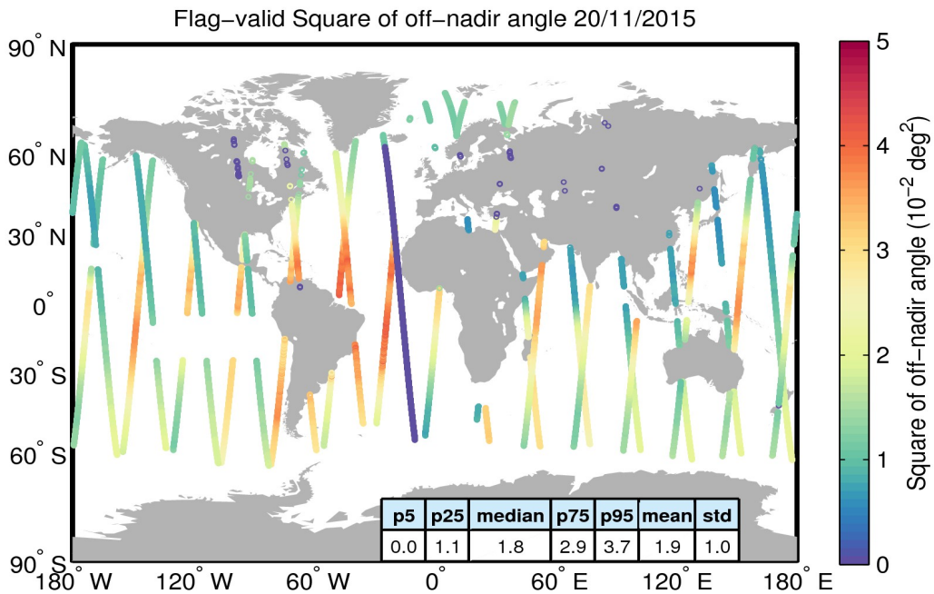
Figure 37. Geographical distribution of flag-valid mispointing data over oceans and lakes for 20/11/2015. The statistical values shown in the table refer to the mispointing in 10^{-2} deg 2 and are calculated over all measurements shown in the figure.
