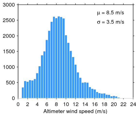
Figure 35. Histogram of science-valid wind over oceans and lakes for 18/11/2015. The mean ( \mu ) and standard deviation ( \sigma ) are also shown. Note that values larger than 24 m/s are excluded from the histogram for the sake of readability but not from the computation of \mu and \sigma .
