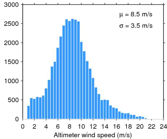
Figure 33. Histogram of flag-valid wind over oceans and lakes for 18/11/2015. The mean ( \mu ) and standard deviation ( \sigma ) are also shown. Note that values larger than 24 m/s are excluded from the histogram for the sake of readability but not from the computation of \mu and \sigma .
