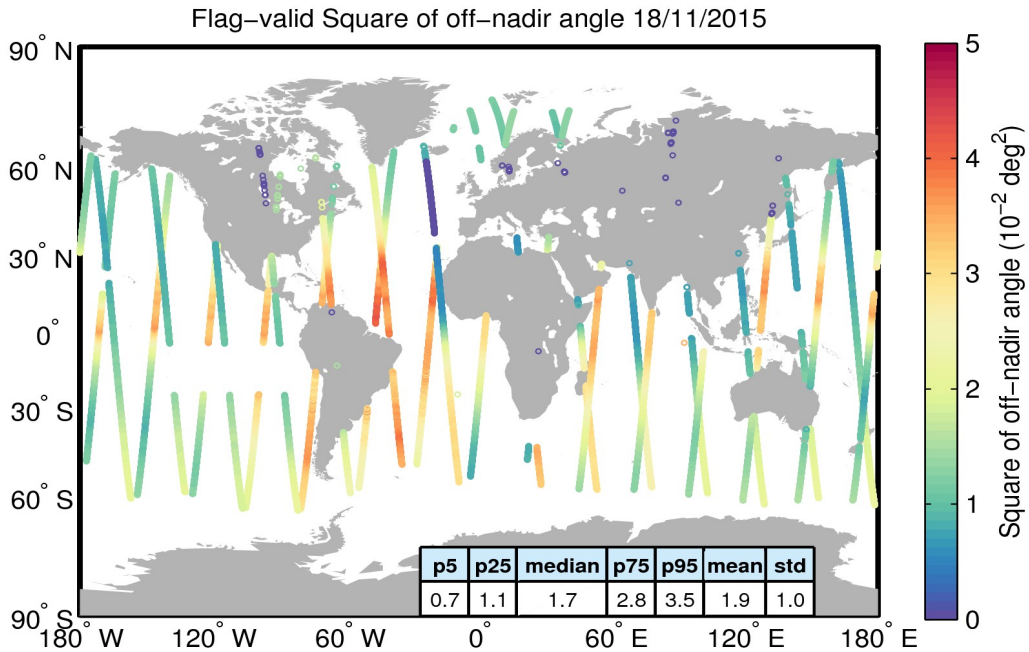
Figure 37. Geographical distribution of flag-valid mispointing data over oceans and lakes for 18/11/2015. The statistical values shown in the table refer to the mispointing in 10^{-2} deg 2 and are calculated over all measurements shown in the figure.
