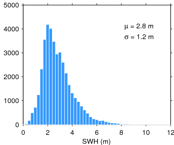
Figure 20. Histogram of science-valid SWH over oceans and lakes for 18/11/2015. The mean ( \mu ) and standard deviation ( \sigma ) are also shown. Note that values larger than 12 m are excluded from the histogram for the sake of readability but not from the computation of \mu and \sigma .
