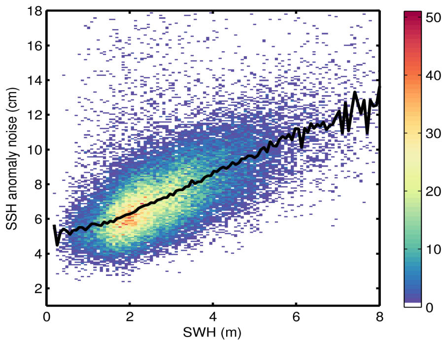
Figure 9. 2D histogram showing flag-valid SSH anomaly noise as a function of SWH for 18/11/2015. The black line denotes the median SSH anomaly noise as a function of SWH.
