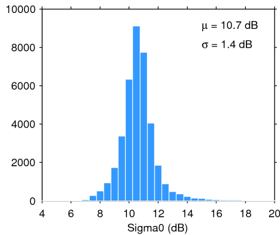
Figure 28. Histogram of science-valid sigma0 over oceans and lakes for 18/11/2015. The mean ( \mu ) and standard deviation ( \sigma ) are also shown. Note that values outside [4 20] dB are excluded from the histogram for the sake of readability but not from the computation of \mu and \sigma .
