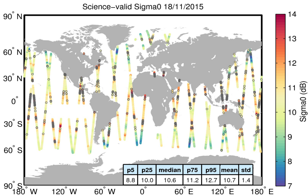
Figure 27. Geographical distribution of science-valid sigma0 data over oceans and lakes for 18/11/2015. The statistical values shown in the table refer to the sigma0 in dB and are calculated over all measurements shown in the figure. Gray circles denote records that have been rejected based on the editing criteria described in Table 4.
