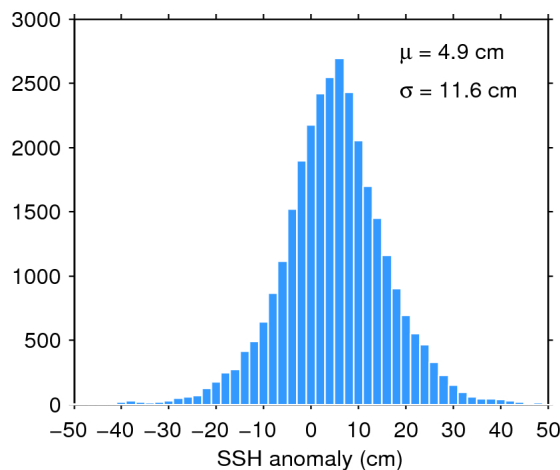
Figure 11. Histogram of science-valid SSH anomaly over oceans and lakes for 18/11/2015. The mean ( \mu ) and standard deviation ( \sigma ) are also shown. Note that values outside [-50 50] cm are excluded from the histogram for the sake of readability but not from the computation of \mu and \sigma .
