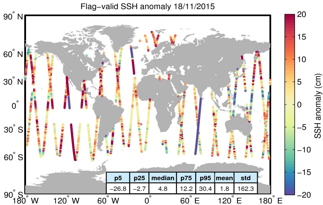
Figure 5. Geographical distribution of flag-valid 1-Hz SSH anomaly data over oceans and lakes for 18/11/2015. The statistical values shown in the table refer to the SSH anomaly in cm and are calculated over all measurements shown in the figure.
