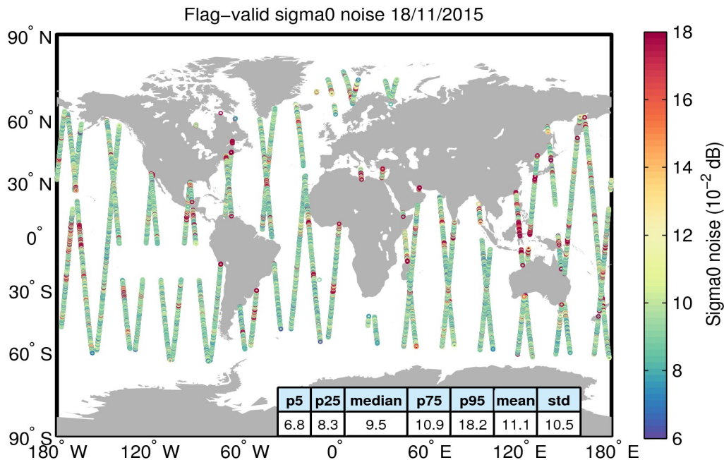
Figure 26. Geographical distribution of flag-valid 20-Hz sigma0 measurement noise over oceans and lakes for 18/11/2015. The statistical values shown in the table refer to the sigma0 noise and are calculated over all measurements shown in the figure.
