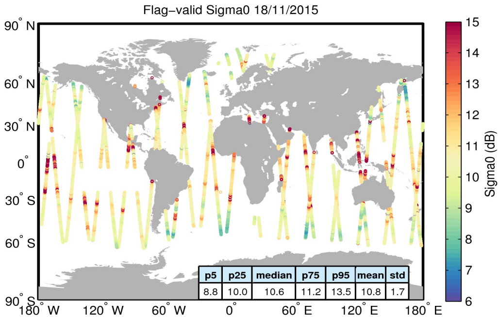
Figure 23. Geographical distribution of flag-valid sigma0 data over oceans and lakes for 18/11/2015. The statistical values shown in the table refer to the sigma0 in dB and are calculated over all measurements shown in the figure.
