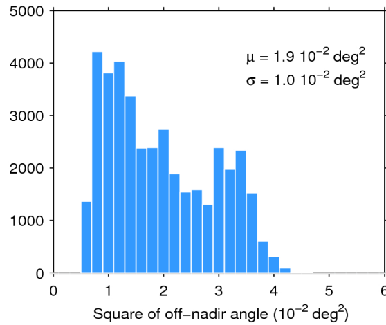
Figure 39. Histogram of flag-valid mispointing over oceans and lakes for 18/11/2015. The mean ( \mu ) and standard deviation ( \sigma ) are also shown. Note that values larger than 6 \cdot 10^{-2} \text{ deg}^2 are excluded from the histogram for the sake of readability but not from the computation of \mu and \sigma .
