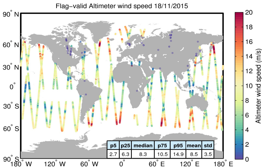
Figure 31. Geographical distribution of flag-valid wind data over oceans and lakes for 18/11/2015. The statistical values shown in the table refer to the wind in m/s and are calculated over all measurements shown in the figure.
