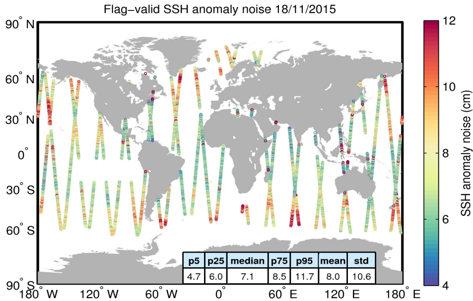
Figure 8. Geographical distribution of flag-valid 20-Hz SSH anomaly measurement noise over oceans and lakes for 18/11/2015. The statistical values shown in the table refer to the SSH anomaly noise and are calculated over all measurements shown in the figure.
