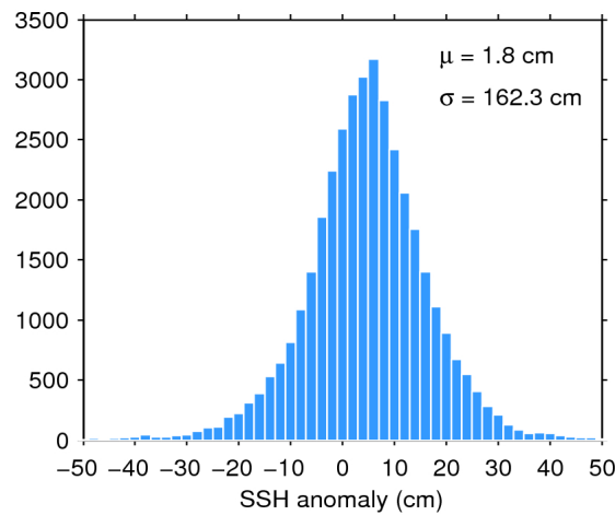
Figure 7. Histogram of flag-valid SSH anomaly over oceans and lakes for 18/11/2015. The mean ( \mu ) and standard deviation ( \sigma ) are also shown. Note that values outside [-50 50] cm are excluded from the histogram for the sake of readability but not from the computation of \mu and \sigma .
