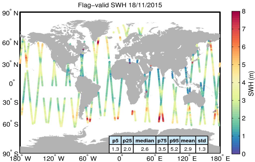
Figure 15. Geographical distribution of flag-valid SWH data over oceans and lakes for 18/11/2015. The statistical values shown in the table refer to the SWH in m and are calculated over all measurements shown in the figure.
