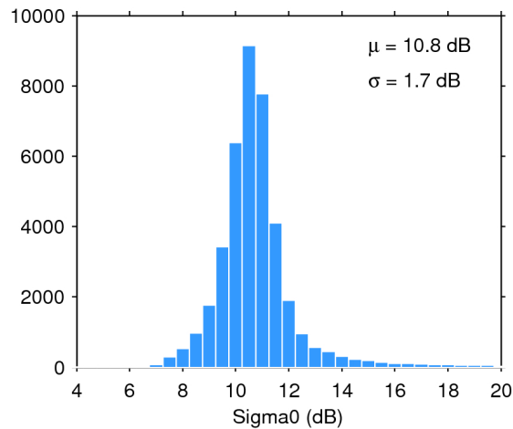
Figure 25. Histogram of flag-valid sigma0 over oceans and lakes for 18/11/2015. The mean ( \mu ) and standard deviation ( \sigma ) are also shown. Note that values outside [4 20] dB are excluded from the histogram for the sake of readability but not from the computation of \mu and \sigma .
