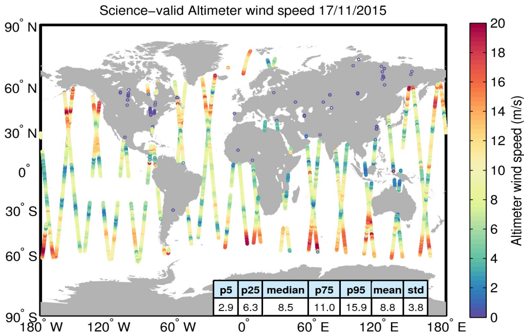
Figure 34. Geographical distribution of science-valid wind data over oceans and lakes for 17/11/2015. The statistical values shown in the table refer to the wind in m/s and are calculated over all measurements shown in the figure. Gray circles denote records that have been rejected based on the editing criteria described in Table 5.
