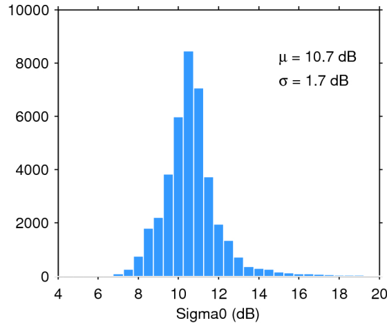
Figure 25. Histogram of flag-valid sigma0 over oceans and lakes for 17/11/2015. The mean ( \mu ) and standard deviation ( \sigma ) are also shown. Note that values outside [4 20] dB are excluded from the histogram for the sake of readability but not from the computation of \mu and \sigma .
