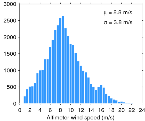
Figure 33. Histogram of flag-valid wind over oceans and lakes for 17/11/2015. The mean ( \mu ) and standard deviation ( \sigma ) are also shown. Note that values larger than 24 m/s are excluded from the histogram for the sake of readability but not from the computation of \mu and \sigma .
