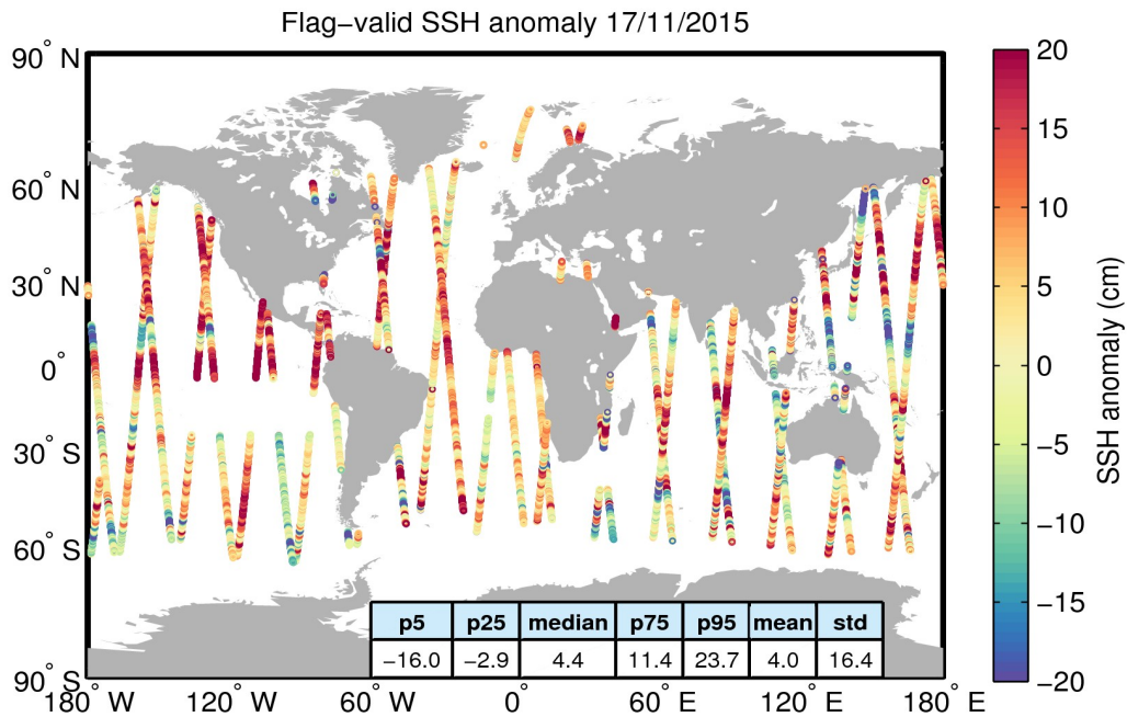
Figure 5. Geographical distribution of flag-valid 1-Hz SSH anomaly data over oceans and lakes for 17/11/2015. The statistical values shown in the table refer to the SSH anomaly in cm and are calculated over all measurements shown in the figure.
