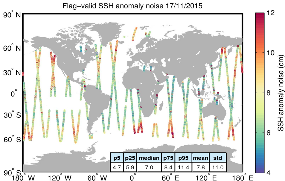
Figure 8. Geographical distribution of flag-valid 20-Hz SSH anomaly measurement noise over oceans and lakes for 17/11/2015. The statistical values shown in the table refer to the SSH anomaly noise and are calculated over all measurements shown in the figure.
