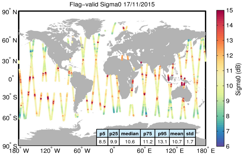
Figure 23. Geographical distribution of flag-valid sigma0 data over oceans and lakes for 17/11/2015. The statistical values shown in the table refer to the sigma0 in dB and are calculated over all measurements shown in the figure.
