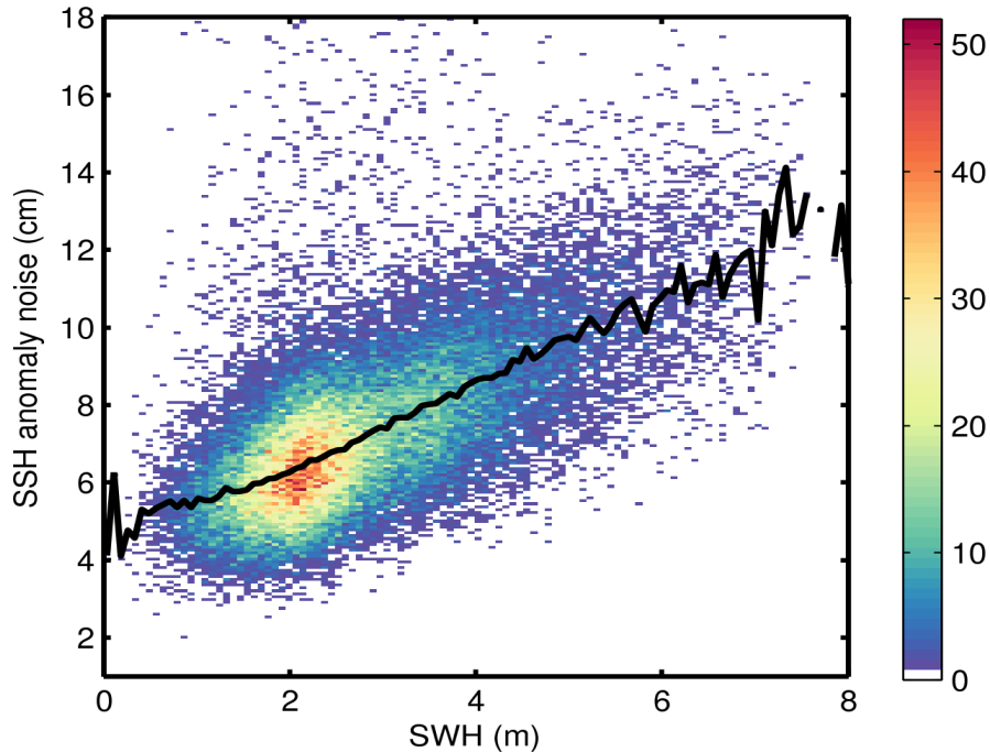
Figure 9. 2D histogram showing flag-valid SSH anomaly noise as a function of SWH for 17/11/2015. The black line denotes the median SSH anomaly noise as a function of SWH.
