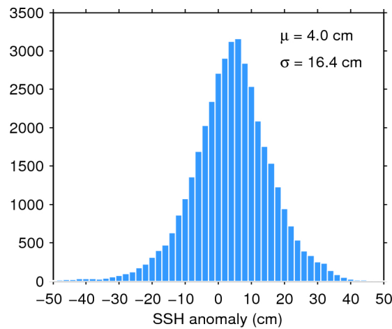
Figure 7. Histogram of flag-valid SSH anomaly over oceans and lakes for 17/11/2015. The mean ( \mu ) and standard deviation ( \sigma ) are also shown. Note that values outside [-50\ 50] cm are excluded from the histogram for the sake of readability but not from the computation of \mu and \sigma .
