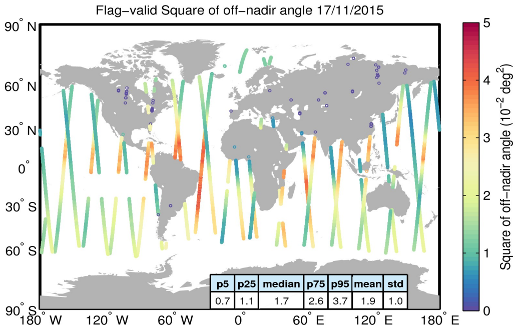
Figure 37. Geographical distribution of flag-valid mispointing data over oceans and lakes for 17/11/2015. The statistical values shown in the table refer to the mispointing in 10^{-2} deg 2 and are calculated over all measurements shown in the figure.
