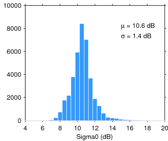
Figure 28. Histogram of science-valid sigma0 over oceans and lakes for 17/11/2015. The mean ( \mu ) and standard deviation ( \sigma ) are also shown. Note that values outside [4 20] dB are excluded from the histogram for the sake of readability but not from the computation of \mu and \sigma .
