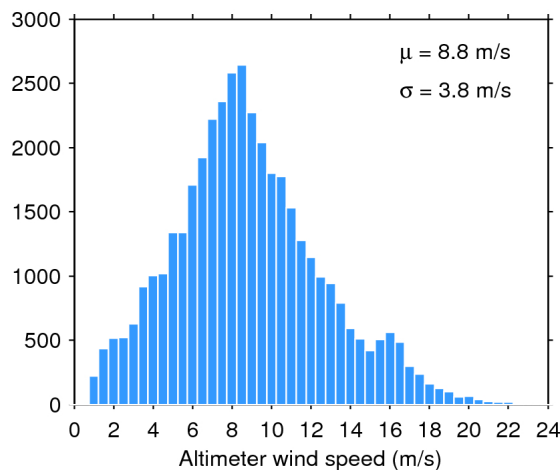
Figure 35. Histogram of science-valid wind over oceans and lakes for 17/11/2015. The mean ( \mu ) and standard deviation ( \sigma ) are also shown. Note that values larger than 24 m/s are excluded from the histogram for the sake of readability but not from the computation of \mu and \sigma .
