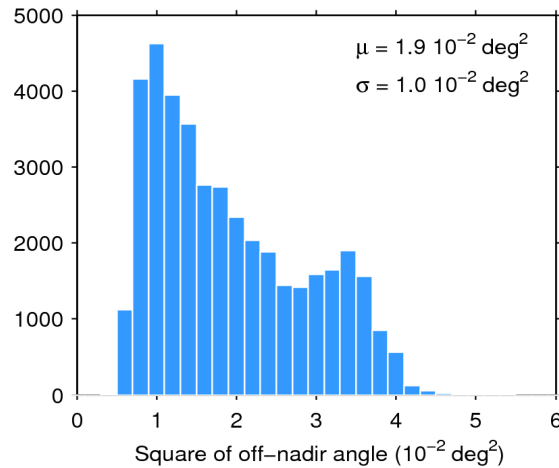
Figure 39. Histogram of flag-valid mispointing over oceans and lakes for 17/11/2015. The mean ( \mu ) and standard deviation ( \sigma ) are also shown. Note that values larger than 6 \cdot 10^{-2} \text{ deg}^2 are excluded from the histogram for the sake of readability but not from the computation of \mu and \sigma .
