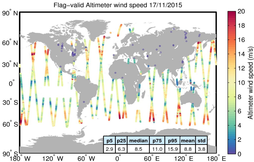
Figure 31. Geographical distribution of flag-valid wind data over oceans and lakes for 17/11/2015. The statistical values shown in the table refer to the wind in m/s and are calculated over all measurements shown in the figure.
