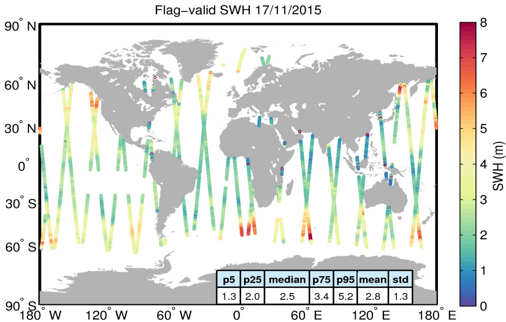
Figure 15. Geographical distribution of flag-valid SWH data over oceans and lakes for 17/11/2015. The statistical values shown in the table refer to the SWH in m and are calculated over all measurements shown in the figure.
