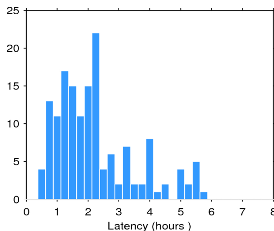
Figure 2. Histogram of the data latency for 17/11/2015. The y-axis denotes the number of files that are made available with a delay of x-hours with respect to the mean time of the records stored in the file.
