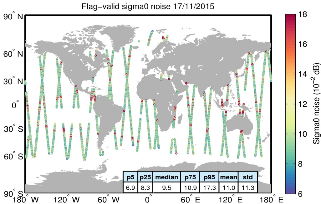
Figure 26. Geographical distribution of flag-valid 20-Hz sigma0 measurement noise over oceans and lakes for 17/11/2015. The statistical values shown in the table refer to the sigma0 noise and are calculated over all measurements shown in the figure.
