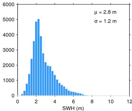
Figure 20. Histogram of science-valid SWH over oceans and lakes for 17/11/2015. The mean ( \mu ) and standard deviation ( \sigma ) are also shown. Note that values larger than 12 m are excluded from the histogram for the sake of readability but not from the computation of \mu and \sigma .
