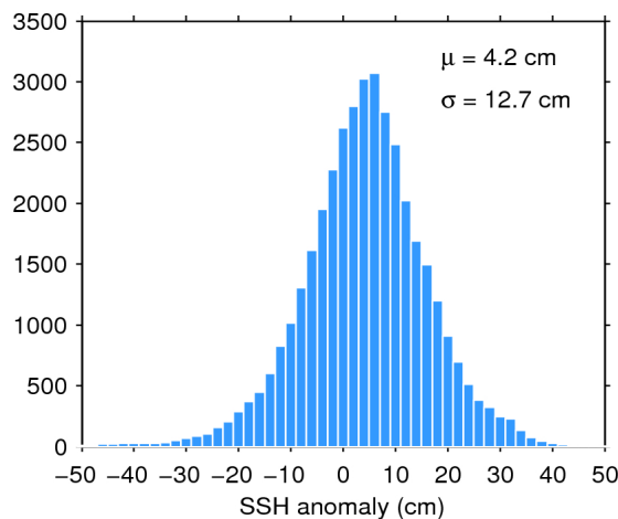
Figure 11. Histogram of science-valid SSH anomaly over oceans and lakes for 17/11/2015. The mean ( \mu ) and standard deviation ( \sigma ) are also shown. Note that values outside [-50 50] cm are excluded from the histogram for the sake of readability but not from the computation of \mu and \sigma .
