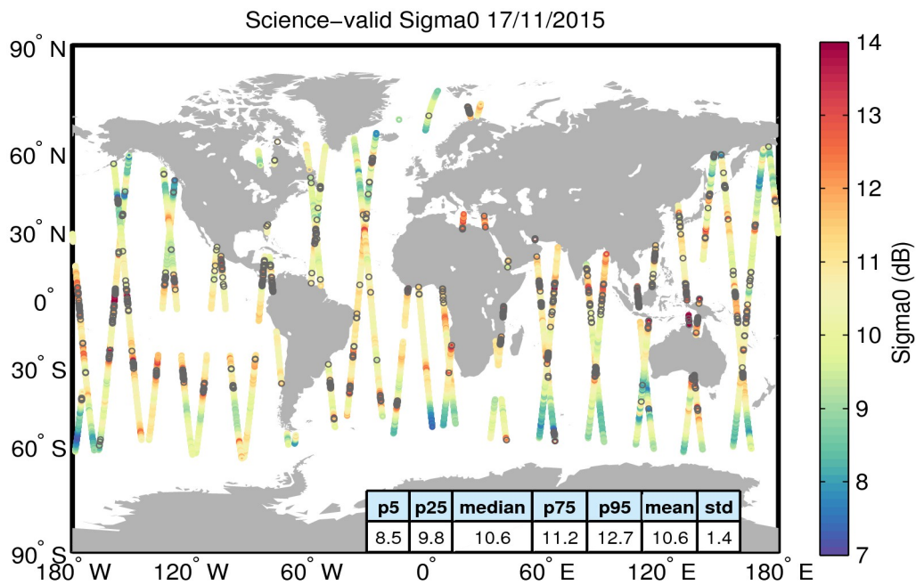
Figure 27. Geographical distribution of science-valid sigma0 data over oceans and lakes for 17/11/2015. The statistical values shown in the table refer to the sigma0 in dB and are calculated over all measurements shown in the figure. Gray circles denote records that have been rejected based on the editing criteria described in Table 4.
