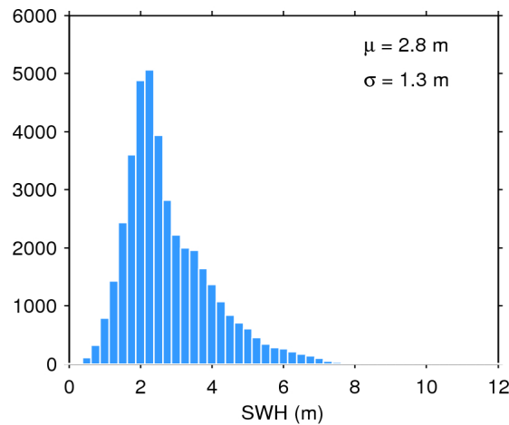
Figure 17. Histogram of flag-valid SWH over oceans and lakes for 17/11/2015. The mean ( \mu ) and standard deviation ( \sigma ) are also shown. Note that values larger than 12 m are excluded from the histogram for the sake of readability but not from the computation of \mu and \sigma .
