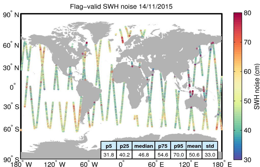
Figure 18. Geographical distribution of flag-valid 20-Hz SWH measurement noise over oceans and lakes for 14/11/2015. The statistical values shown in the figure refer to the SWH noise and are calculated over all measurements shown in the figure.
