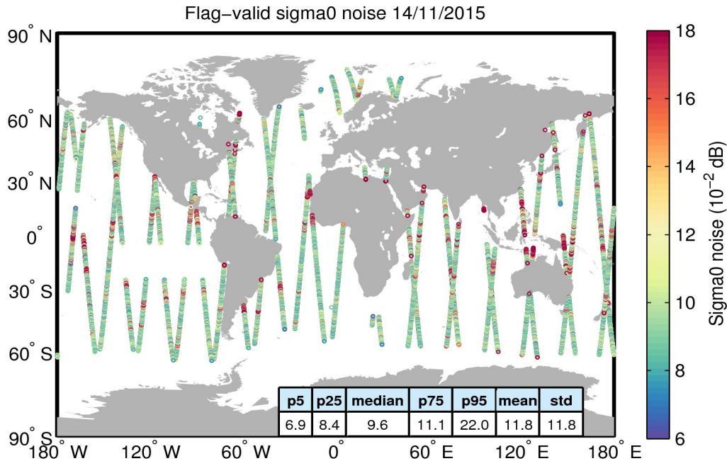
Figure 26. Geographical distribution of flag-valid 20-Hz sigma0 measurement noise over oceans and lakes for 14/11/2015. The statistical values shown in the table refer to the sigma0 noise and are calculated over all measurements shown in the figure.
