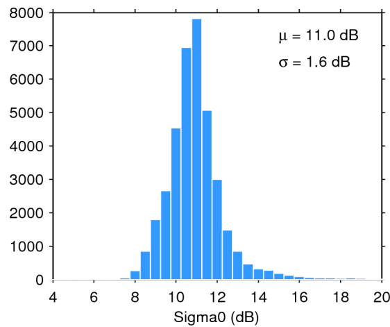
Figure 28. Histogram of science-valid sigma0 over oceans and lakes for 14/11/2015. The mean ( \mu ) and standard deviation ( \sigma ) are also shown. Note that values outside [4 20] dB are excluded from the histogram for the sake of readability but not from the computation of \mu and \sigma .
