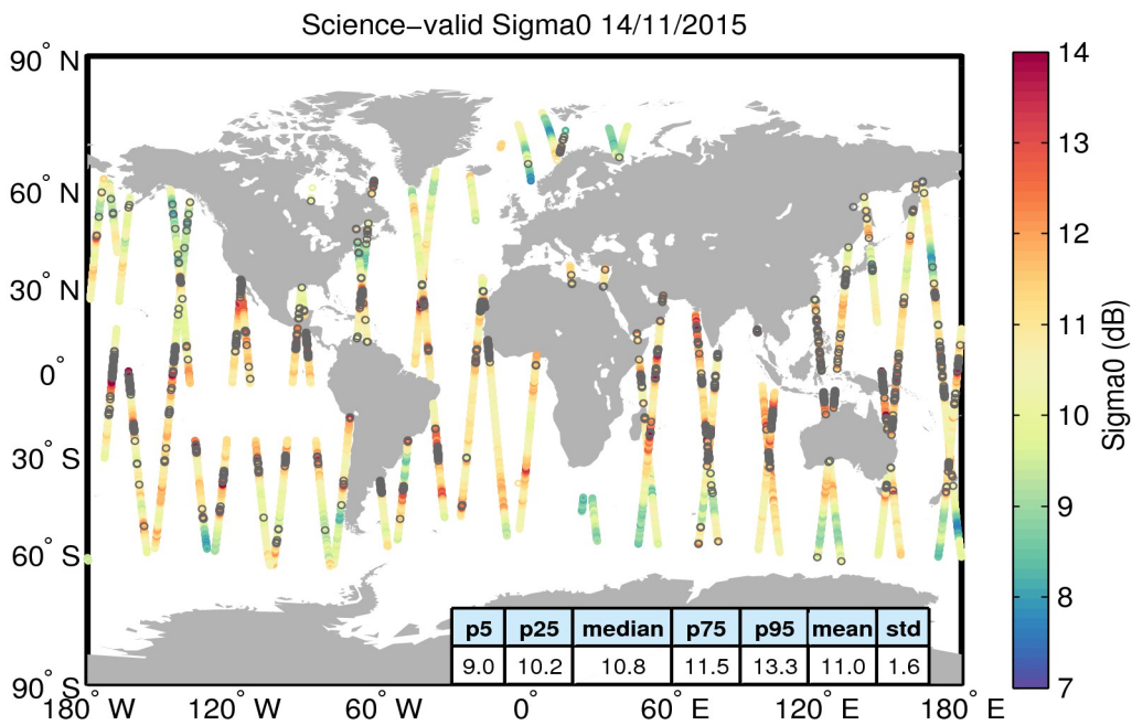
Figure 27. Geographical distribution of science-valid sigma0 data over oceans and lakes for 14/11/2015. The statistical values shown in the table refer to the sigma0 in dB and are calculated over all measurements shown in the figure. Gray circles denote records that have been rejected based on the editing criteria described in Table 4.
