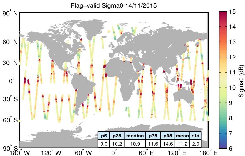
Figure 23. Geographical distribution of flag-valid sigma0 data over oceans and lakes for 14/11/2015. The statistical values shown in the table refer to the sigma0 in dB and are calculated over all measurements shown in the figure.
