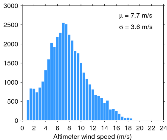
Figure 35. Histogram of science-valid wind over oceans and lakes for 14/11/2015. The mean ( \mu ) and standard deviation ( \sigma ) are also shown. Note that values larger than 24 m/s are excluded from the histogram for the sake of readability but not from the computation of \mu and \sigma .
