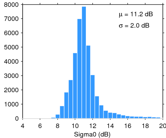
Figure 25. Histogram of flag-valid sigma0 over oceans and lakes for 14/11/2015. The mean ( \mu ) and standard deviation ( \sigma ) are also shown. Note that values outside [4 20] dB are excluded from the histogram for the sake of readability but not from the computation of \mu and \sigma .
