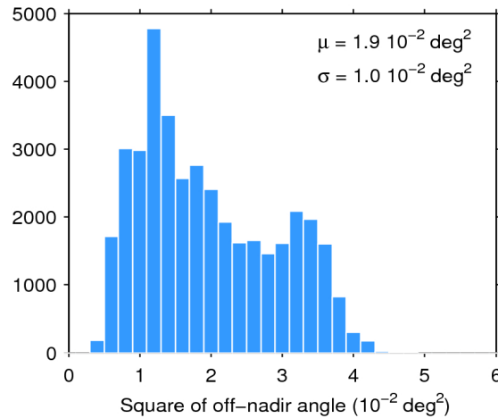
Figure 39. Histogram of flag-valid mispointing over oceans and lakes for 14/11/2015. The mean ( \mu ) and standard deviation ( \sigma ) are also shown. Note that values larger than 6 \cdot 10^{-2} \text{ deg}^2 are excluded from the histogram for the sake of readability but not from the computation of \mu and \sigma .
