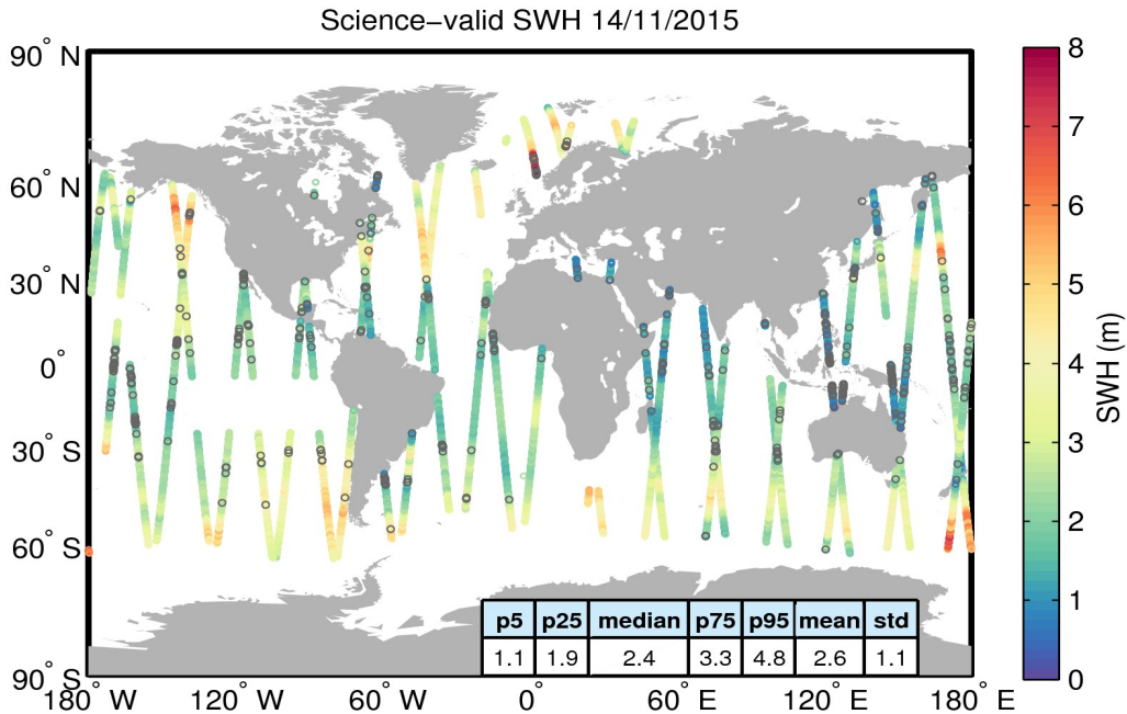
Figure 19. Geographical distribution of science-valid SWH data over oceans and lakes for 14/11/2015. The statistical values shown in the table refer to the SWH in m and are calculated over all measurements shown in the figure. Gray circles denote records that have been rejected based on the editing criteria described in Table 3.
