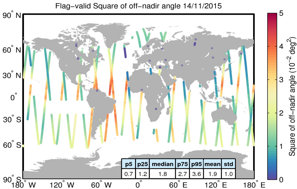
Figure 37. Geographical distribution of flag-valid mispointing data over oceans and lakes for 14/11/2015. The statistical values shown in the table refer to the mispointing in 10^{-2} \text{deg}^2 and are calculated over all measurements shown in the figure.
