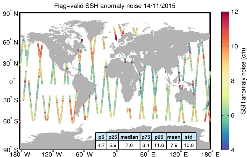
Figure 8. Geographical distribution of flag-valid 20-Hz SSH anomaly measurement noise over oceans and lakes for 14/11/2015. The statistical values shown in the table refer to the SSH anomaly noise and are calculated over all measurements shown in the figure.
