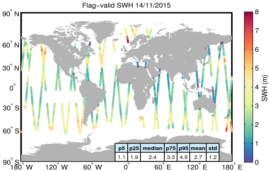
Figure 15. Geographical distribution of flag-valid SWH data over oceans and lakes for 14/11/2015. The statistical values shown in the table refer to the SWH in m and are calculated over all measurements shown in the figure.
