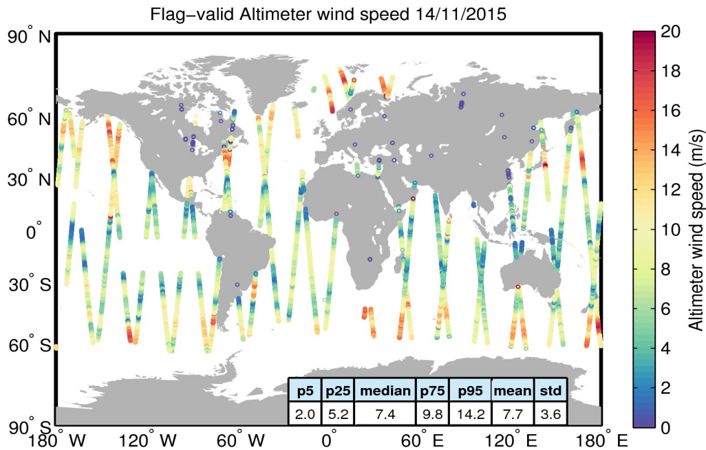
Figure 31. Geographical distribution of flag-valid wind data over oceans and lakes for 14/11/2015. The statistical values shown in the table refer to the wind in m/s and are calculated over all measurements shown in the figure.
