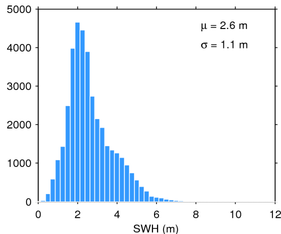
Figure 20. Histogram of science-valid SWH over oceans and lakes for 14/11/2015. The mean ( \mu ) and standard deviation ( \sigma ) are also shown. Note that values larger than 12 m are excluded from the histogram for the sake of readability but not from the computation of \mu and \sigma .
