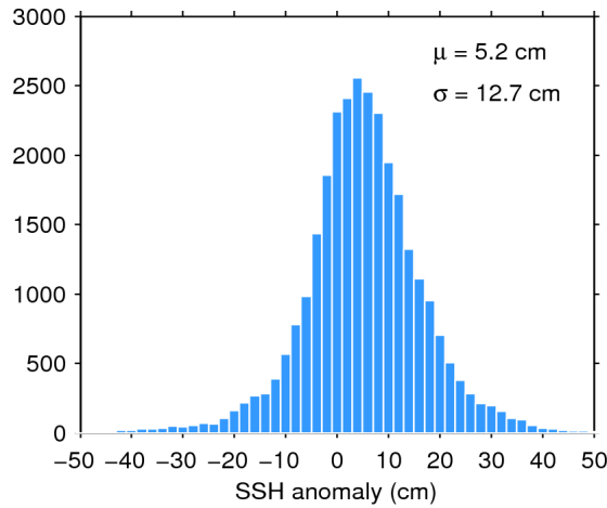
Figure 11. Histogram of science-valid SSH anomaly over oceans and lakes for 14/11/2015. The mean ( \mu ) and standard deviation ( \sigma ) are also shown. Note that values outside [-50 50] cm are excluded from the histogram for the sake of readability but not from the computation of \mu and \sigma .
