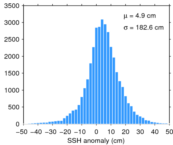
Figure 7. Histogram of flag-valid SSH anomaly over oceans and lakes for 14/11/2015. The mean ( \mu ) and standard deviation ( \sigma ) are also shown. Note that values outside [-50\ 50] cm are excluded from the histogram for the sake of readability but not from the computation of \mu and \sigma .
