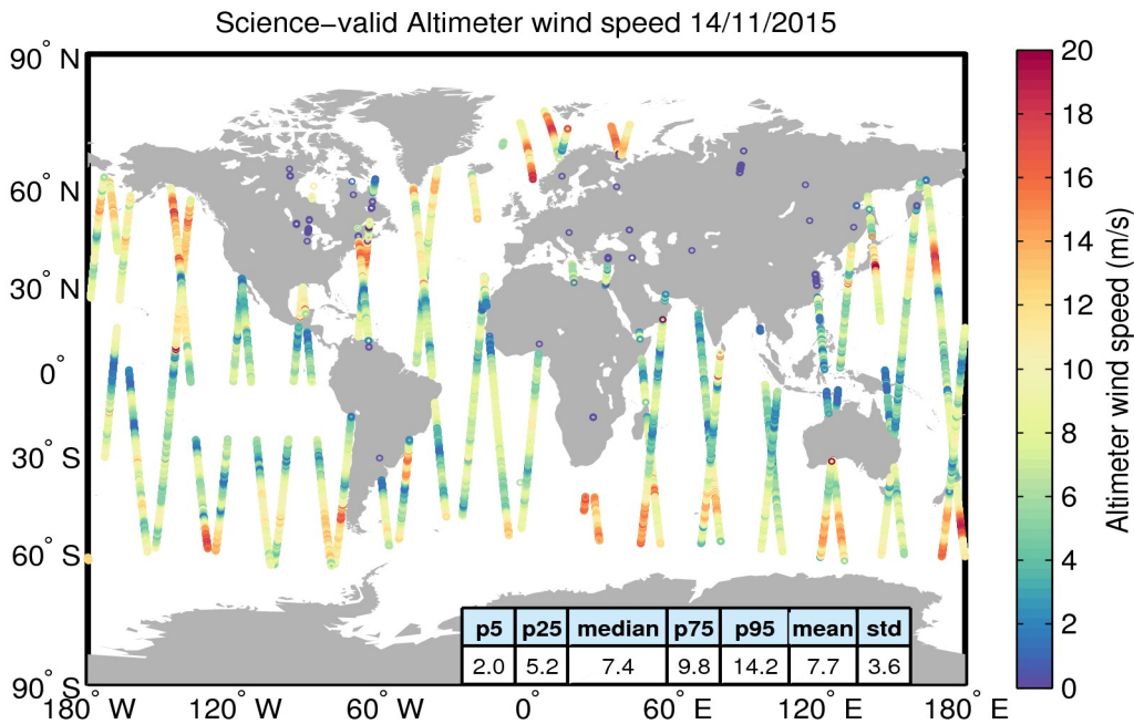
Figure 34. Geographical distribution of science-valid wind data over oceans and lakes for 14/11/2015. The statistical values shown in the table refer to the wind in m/s and are calculated over all measurements shown in the figure. Gray circles denote records that have been rejected based on the editing criteria described in Table 5.
