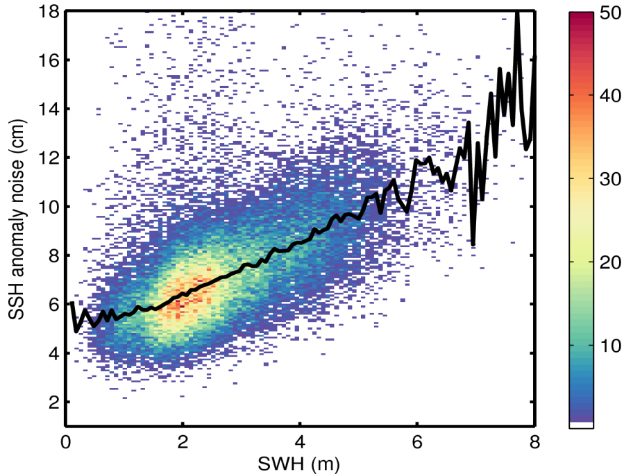
Figure 9. 2D histogram showing flag-valid SSH anomaly noise as a function of SWH for 14/11/2015. The black line denotes the median SSH anomaly noise as a function of SWH.
