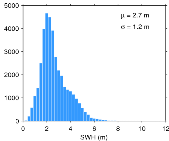
Figure 17. Histogram of flag-valid SWH over oceans and lakes for 14/11/2015. The mean ( \mu ) and standard deviation ( \sigma ) are also shown. Note that values larger than 12 m are excluded from the histogram for the sake of readability but not from the computation of \mu and \sigma .
