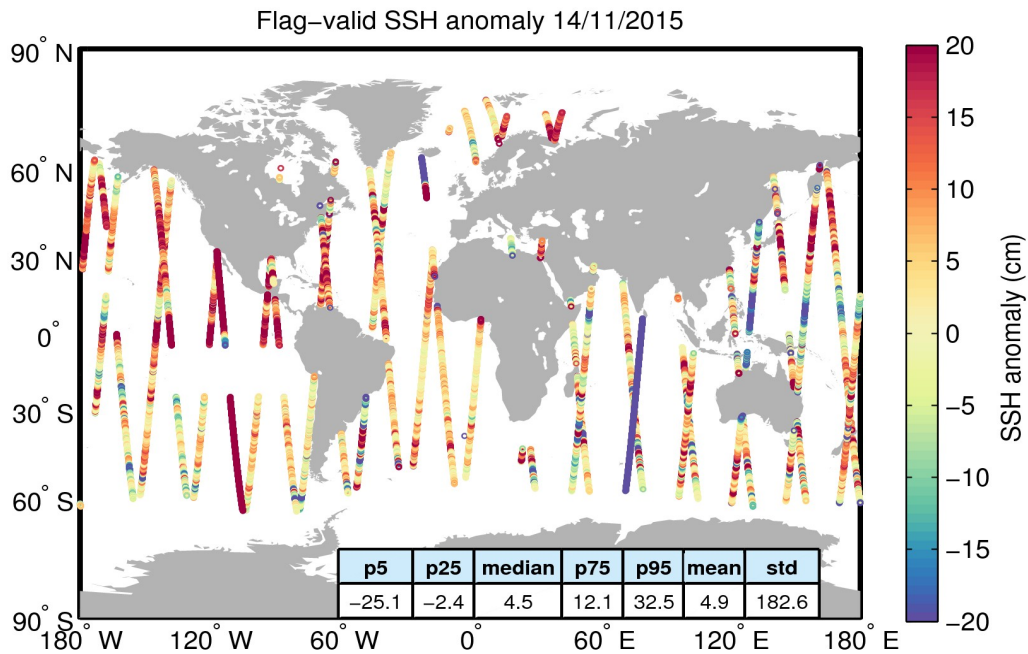
Figure 5. Geographical distribution of flag-valid 1-Hz SSH anomaly data over oceans and lakes for 14/11/2015. The statistical values shown in the table refer to the SSH anomaly in cm and are calculated over all measurements shown in the figure.
