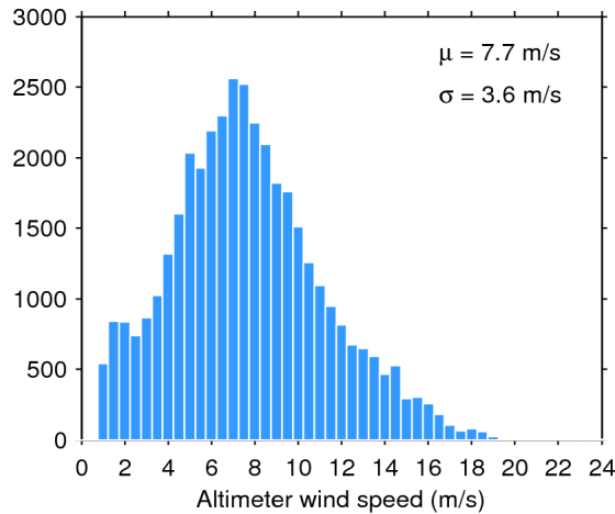
Figure 33. Histogram of flag-valid wind over oceans and lakes for 14/11/2015. The mean ( \mu ) and standard deviation ( \sigma ) are also shown. Note that values larger than 24 m/s are excluded from the histogram for the sake of readability but not from the computation of \mu and \sigma .
