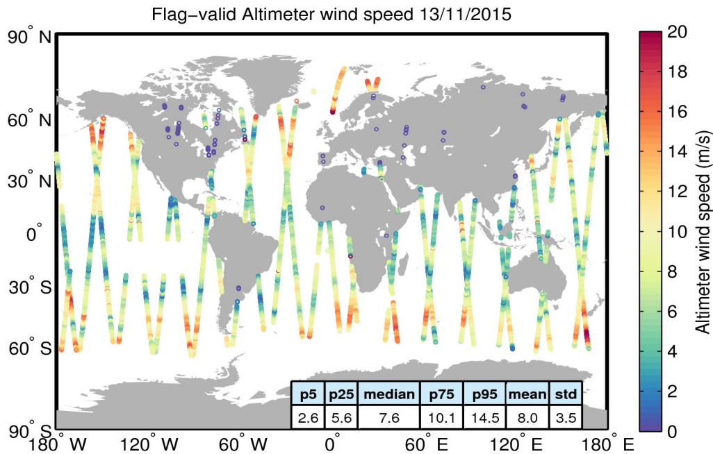
Figure 31. Geographical distribution of flag-valid wind data over oceans and lakes for 13/11/2015. The statistical values shown in the table refer to the wind in m/s and are calculated over all measurements shown in the figure.
