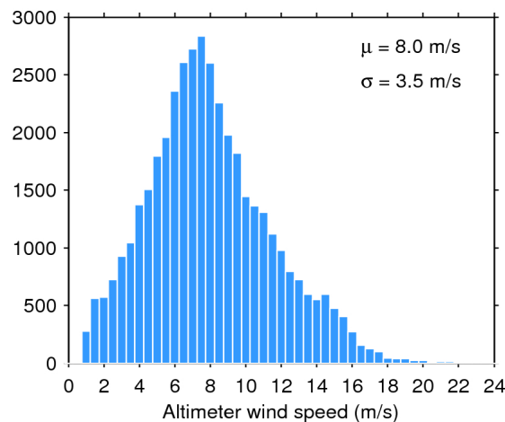
Figure 35. Histogram of science-valid wind over oceans and lakes for 13/11/2015. The mean ( \mu ) and standard deviation ( \sigma ) are also shown. Note that values larger than 24 m/s are excluded from the histogram for the sake of readability but not from the computation of \mu and \sigma .
