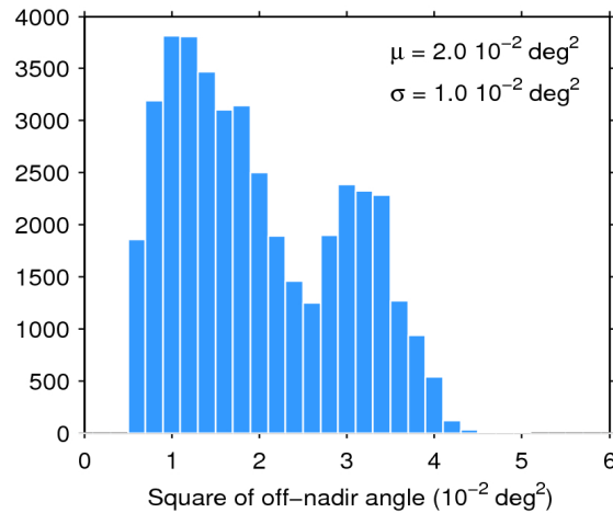
Figure 39. Histogram of flag-valid mispointing over oceans and lakes for 13/11/2015. The mean ( \mu ) and standard deviation ( \sigma ) are also shown. Note that values larger than 6 \cdot 10^{-2} \text{ deg}^2 are excluded from the histogram for the sake of readability but not from the computation of \mu and \sigma .
