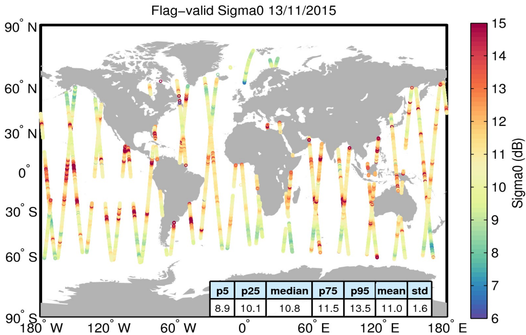
Figure 23. Geographical distribution of flag-valid sigma0 data over oceans and lakes for 13/11/2015. The statistical values shown in the table refer to the sigma0 in dB and are calculated over all measurements shown in the figure.
