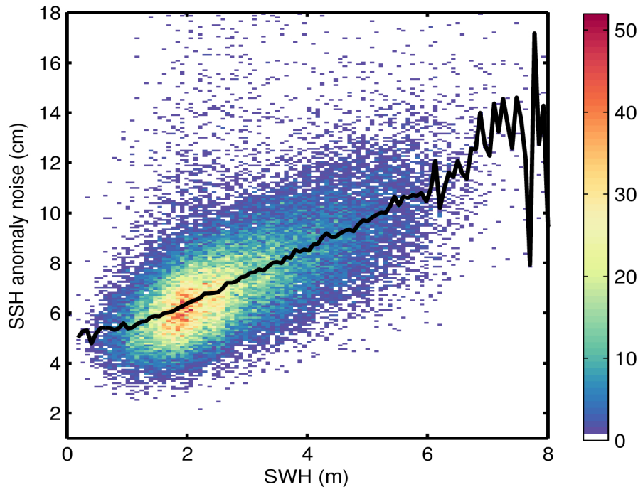
Figure 9. 2D histogram showing flag-valid SSH anomaly noise as a function of SWH for 13/11/2015. The black line denotes the median SSH anomaly noise as a function of SWH.
