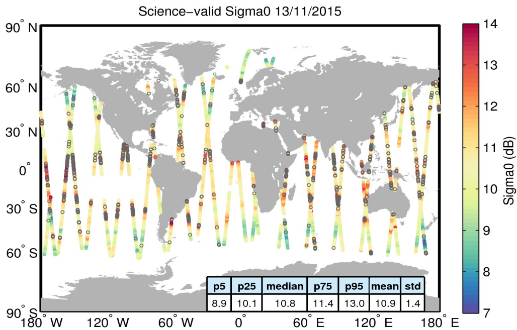
Figure 27. Geographical distribution of science-valid sigma0 data over oceans and lakes for 13/11/2015. The statistical values shown in the table refer to the sigma0 in dB and are calculated over all measurements shown in the figure. Gray circles denote records that have been rejected based on the editing criteria described in Table 4.
