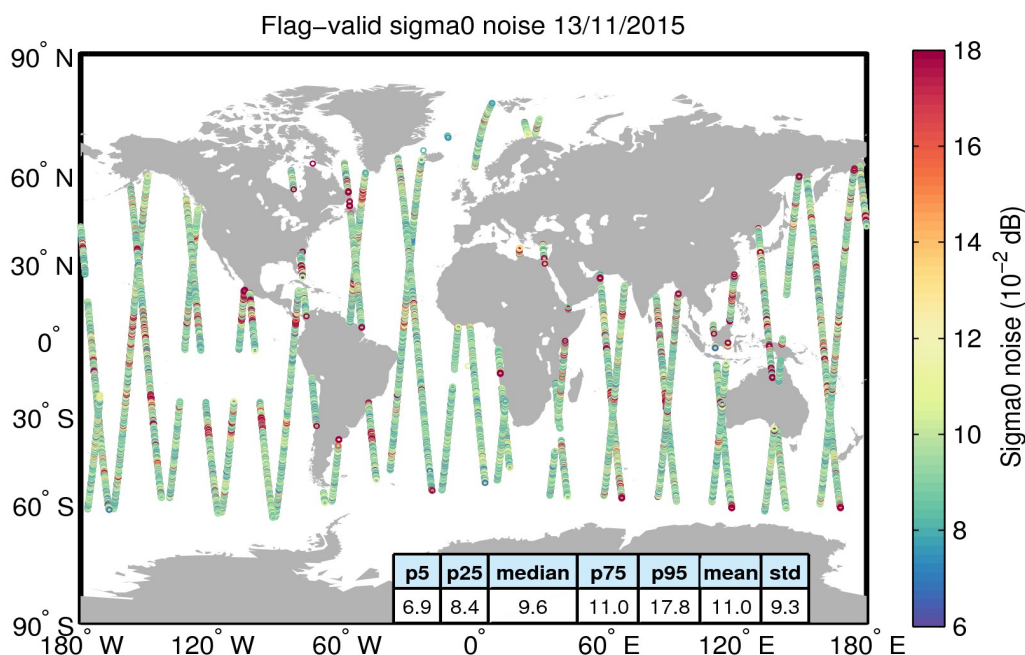
Figure 26. Geographical distribution of flag-valid 20-Hz sigma0 measurement noise over oceans and lakes for 13/11/2015. The statistical values shown in the table refer to the sigma0 noise and are calculated over all measurements shown in the figure.
