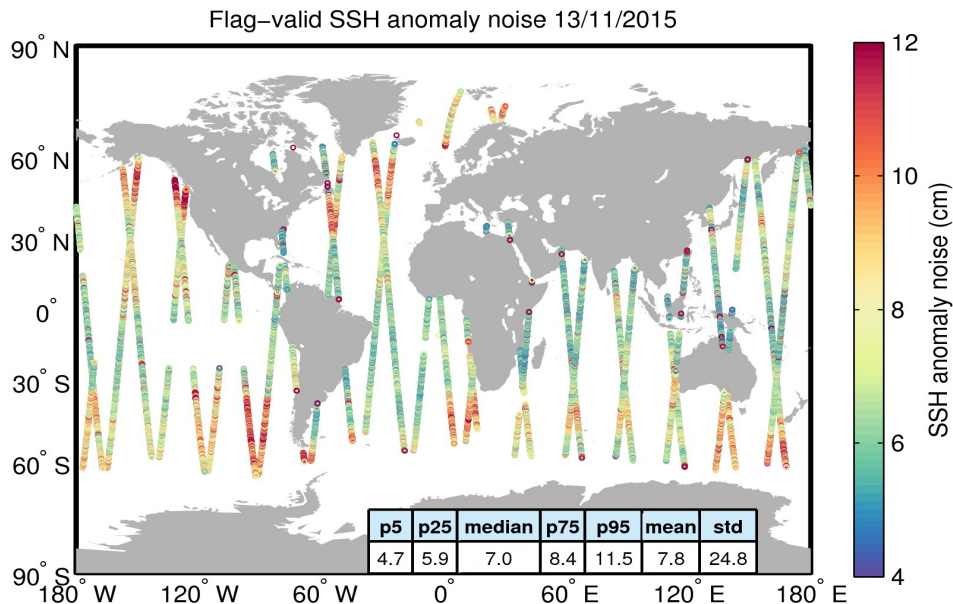
Figure 8. Geographical distribution of flag-valid 20-Hz SSH anomaly measurement noise over oceans and lakes for 13/11/2015. The statistical values shown in the table refer to the SSH anomaly noise and are calculated over all measurements shown in the figure.
