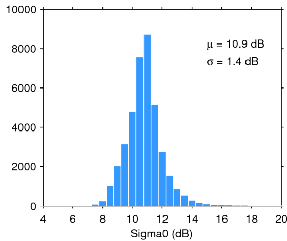
Figure 28. Histogram of science-valid sigma0 over oceans and lakes for 13/11/2015. The mean ( \mu ) and standard deviation ( \sigma ) are also shown. Note that values outside [4 20] dB are excluded from the histogram for the sake of readability but not from the computation of \mu and \sigma .
