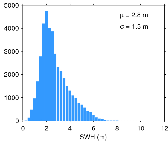
Figure 17. Histogram of flag-valid SWH over oceans and lakes for 13/11/2015. The mean ( \mu ) and standard deviation ( \sigma ) are also shown. Note that values larger than 12 m are excluded from the histogram for the sake of readability but not from the computation of \mu and \sigma .
