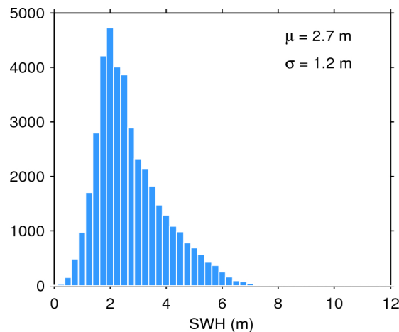
Figure 20. Histogram of science-valid SWH over oceans and lakes for 13/11/2015. The mean ( \mu ) and standard deviation ( \sigma ) are also shown. Note that values larger than 12 m are excluded from the histogram for the sake of readability but not from the computation of \mu and \sigma .
