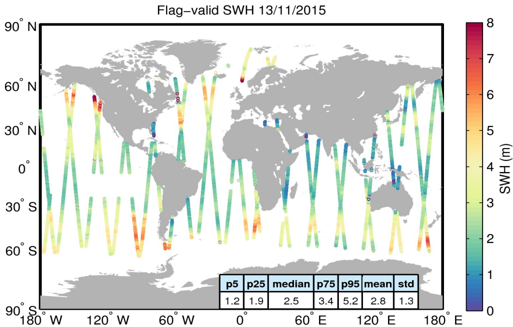
Figure 15. Geographical distribution of flag-valid SWH data over oceans and lakes for 13/11/2015. The statistical values shown in the table refer to the SWH in m and are calculated over all measurements shown in the figure.
