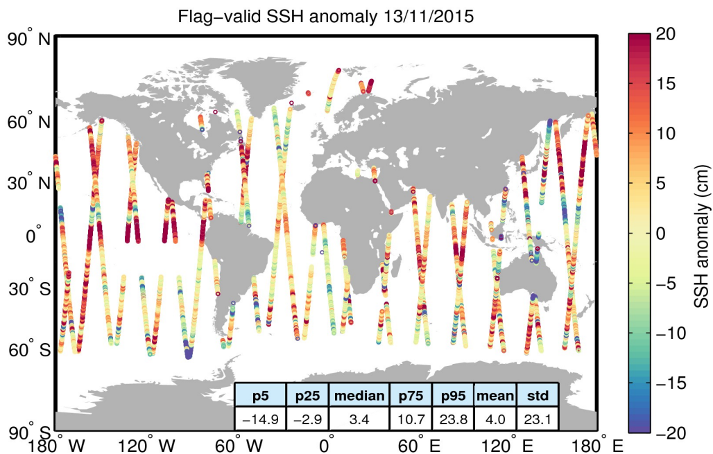
Figure 5. Geographical distribution of flag-valid 1-Hz SSH anomaly data over oceans and lakes for 13/11/2015. The statistical values shown in the table refer to the SSH anomaly in cm and are calculated over all measurements shown in the figure.
