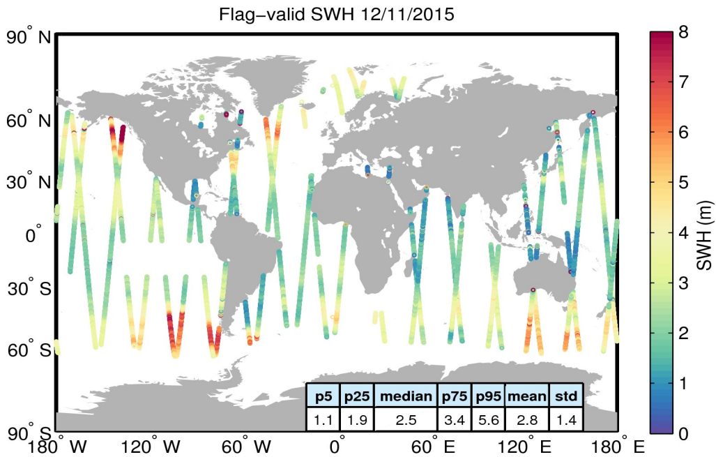
Figure 15. Geographical distribution of flag-valid SWH data over oceans and lakes for 12/11/2015. The statistical values shown in the table refer to the SWH in m and are calculated over all measurements shown in the figure.
