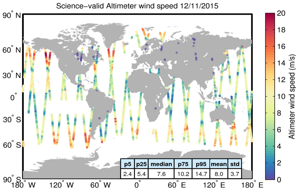
Figure 34. Geographical distribution of science-valid wind data over oceans and lakes for 12/11/2015. The statistical values shown in the table refer to the wind in m/s and are calculated over all measurements shown in the figure. Gray circles denote records that have been rejected based on the editing criteria described in Table 5.
