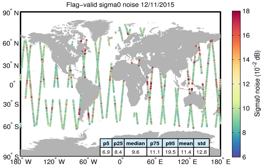
Figure 26. Geographical distribution of flag-valid 20-Hz sigma0 measurement noise over oceans and lakes for 12/11/2015. The statistical values shown in the table refer to the sigma0 noise and are calculated over all measurements shown in the figure.
