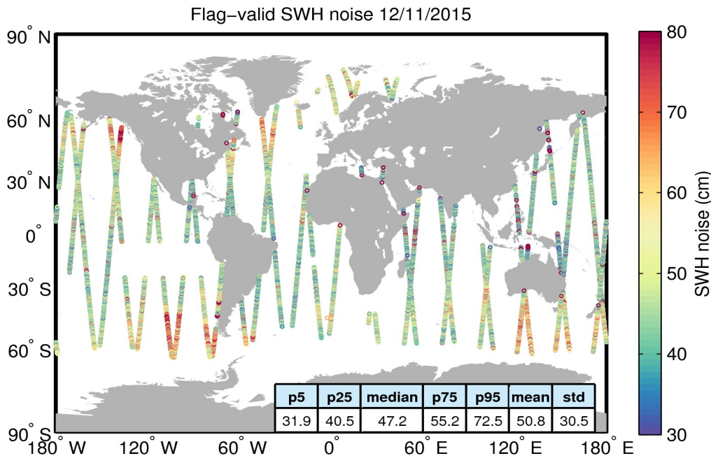
Figure 18. Geographical distribution of flag-valid 20-Hz SWH measurement noise over oceans and lakes for 12/11/2015. The statistical values shown in the figure refer to the SWH noise and are calculated over all measurements shown in the figure.
