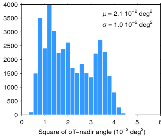
Figure 39. Histogram of flag-valid mispointing over oceans and lakes for 12/11/2015. The mean ( \mu ) and standard deviation ( \sigma ) are also shown. Note that values larger than 6 \cdot 10^{-2} \text{ deg}^2 are excluded from the histogram for the sake of readability but not from the computation of \mu and \sigma .
