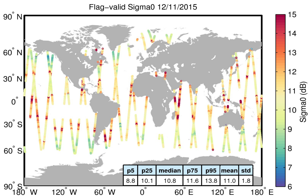
Figure 23. Geographical distribution of flag-valid sigma0 data over oceans and lakes for 12/11/2015. The statistical values shown in the table refer to the sigma0 in dB and are calculated over all measurements shown in the figure.
