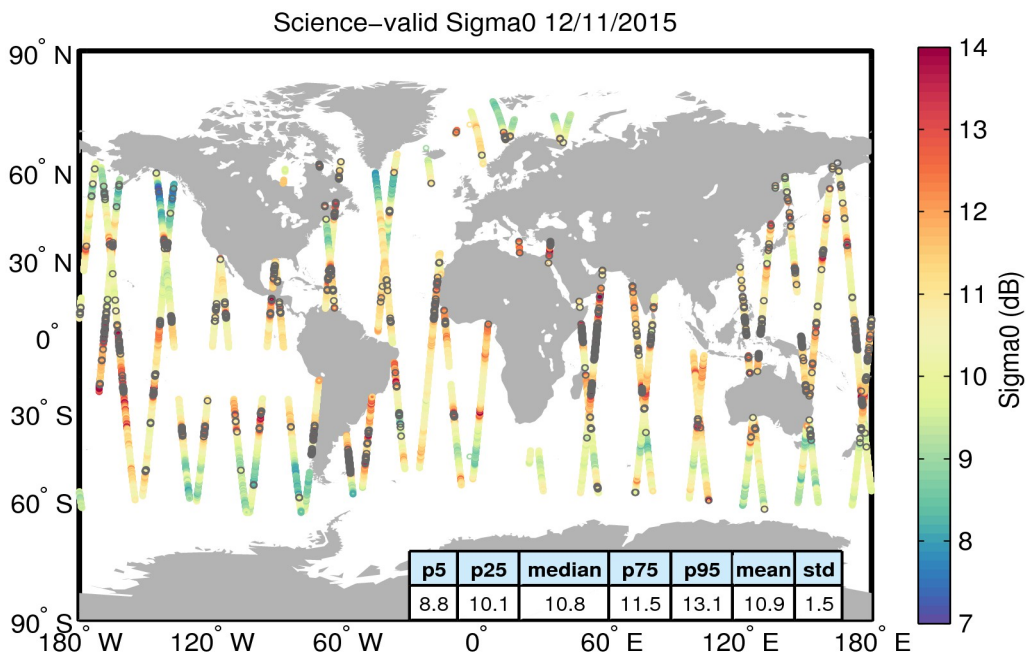
Figure 27. Geographical distribution of science-valid sigma0 data over oceans and lakes for 12/11/2015. The statistical values shown in the table refer to the sigma0 in dB and are calculated over all measurements shown in the figure. Gray circles denote records that have been rejected based on the editing criteria described in Table 4.
