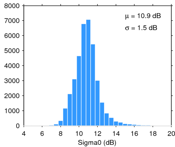
Figure 28. Histogram of science-valid sigma0 over oceans and lakes for 12/11/2015. The mean ( \mu ) and standard deviation ( \sigma ) are also shown. Note that values outside [4 20] dB are excluded from the histogram for the sake of readability but not from the computation of \mu and \sigma .
