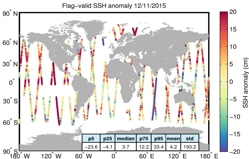
Figure 5. Geographical distribution of flag-valid 1-Hz SSH anomaly data over oceans and lakes for 12/11/2015. The statistical values shown in the table refer to the SSH anomaly in cm and are calculated over all measurements shown in the figure.
