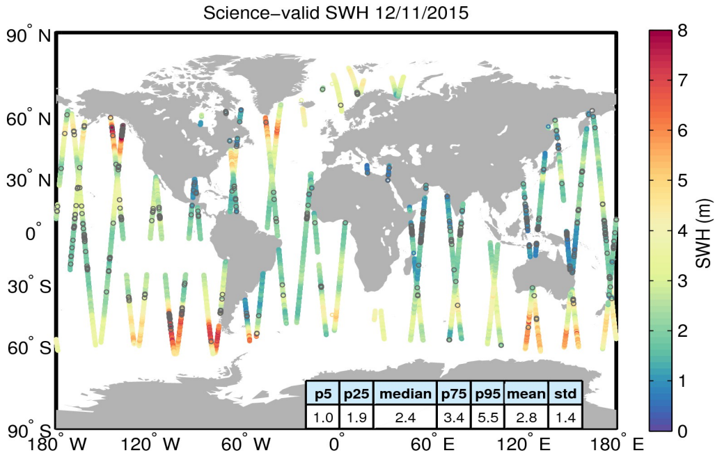
Figure 19. Geographical distribution of science-valid SWH data over oceans and lakes for 12/11/2015. The statistical values shown in the table refer to the SWH in m and are calculated over all measurements shown in the figure. Gray circles denote records that have been rejected based on the editing criteria described in Table 3.
