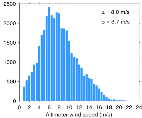
Figure 33. Histogram of flag-valid wind over oceans and lakes for 12/11/2015. The mean ( \mu ) and standard deviation ( \sigma ) are also shown. Note that values larger than 24 m/s are excluded from the histogram for the sake of readability but not from the computation of \mu and \sigma .
