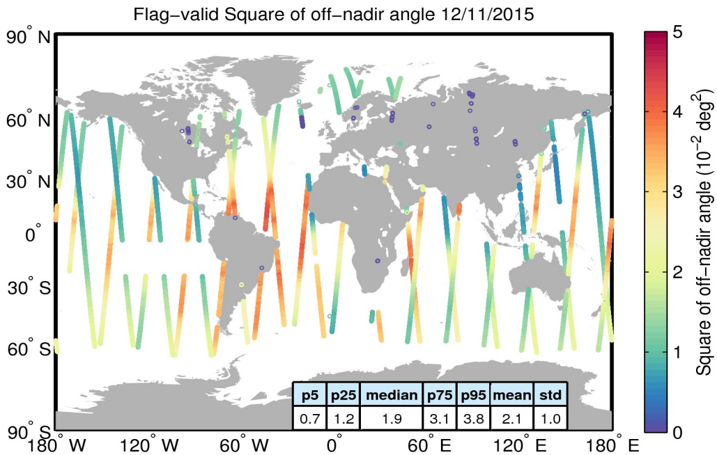
Figure 37. Geographical distribution of flag-valid mispointing data over oceans and lakes for 12/11/2015. The statistical values shown in the table refer to the mispointing in 10^{-2} deg 2 and are calculated over all measurements shown in the figure.
