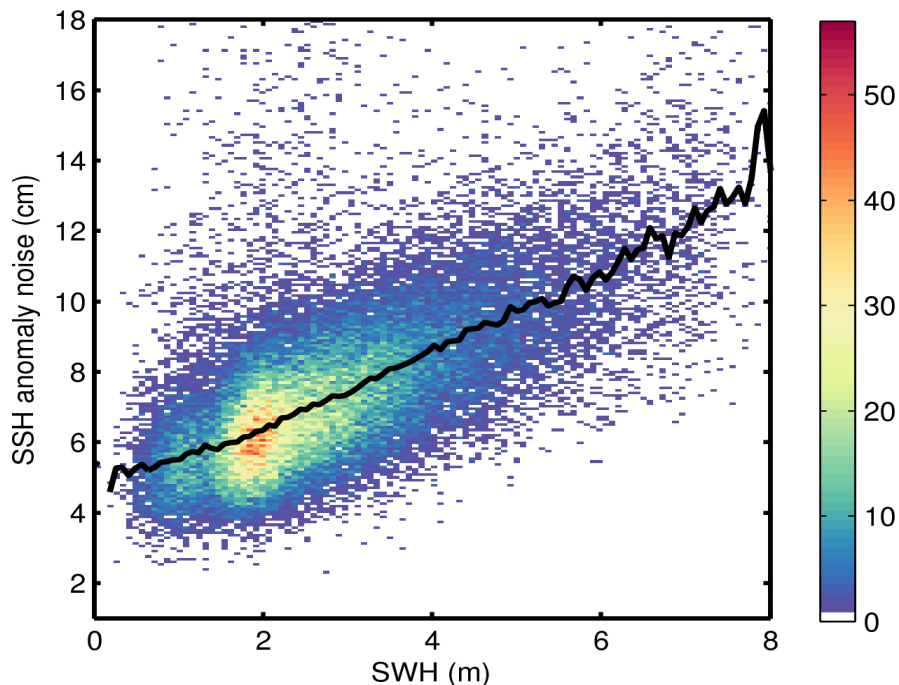
Figure 9. 2D histogram showing flag-valid SSH anomaly noise as a function of SWH for 12/11/2015. The black line denotes the median SSH anomaly noise as a function of SWH.
