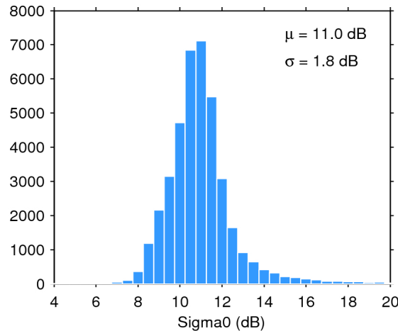
Figure 25. Histogram of flag-valid sigma0 over oceans and lakes for 12/11/2015. The mean ( \mu ) and standard deviation ( \sigma ) are also shown. Note that values outside [4 20] dB are excluded from the histogram for the sake of readability but not from the computation of \mu and \sigma .
