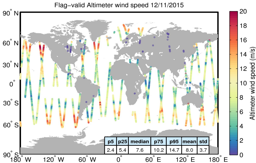
Figure 31. Geographical distribution of flag-valid wind data over oceans and lakes for 12/11/2015. The statistical values shown in the table refer to the wind in m/s and are calculated over all measurements shown in the figure.
