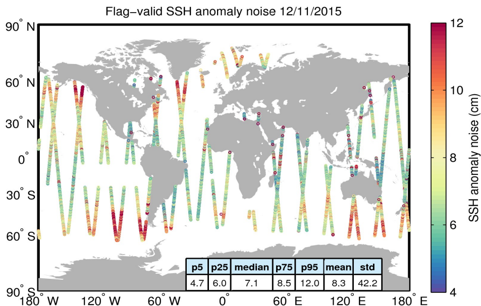
Figure 8. Geographical distribution of flag-valid 20-Hz SSH anomaly measurement noise over oceans and lakes for 12/11/2015. The statistical values shown in the table refer to the SSH anomaly noise and are calculated over all measurements shown in the figure.
