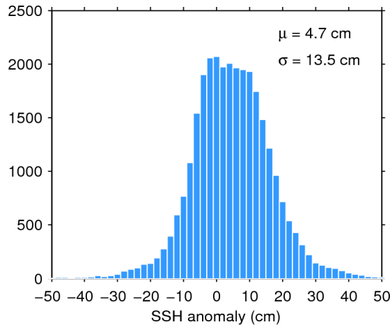
Figure 11. Histogram of science-valid SSH anomaly over oceans and lakes for 12/11/2015. The mean ( \mu ) and standard deviation ( \sigma ) are also shown. Note that values outside [-50 50] cm are excluded from the histogram for the sake of readability but not from the computation of \mu and \sigma .
