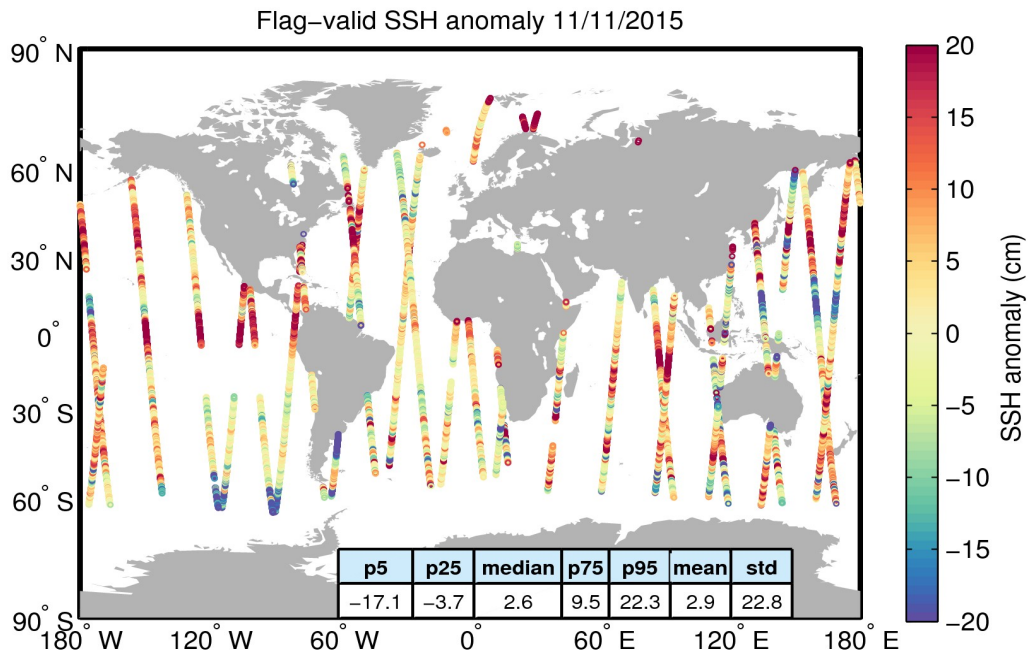
Figure 5. Geographical distribution of flag-valid 1-Hz SSH anomaly data over oceans and lakes for 11/11/2015. The statistical values shown in the table refer to the SSH anomaly in cm and are calculated over all measurements shown in the figure.
