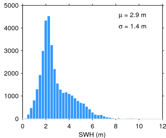
Figure 20. Histogram of science-valid SWH over oceans and lakes for 11/11/2015. The mean ( \mu ) and standard deviation ( \sigma ) are also shown. Note that values larger than 12 m are excluded from the histogram for the sake of readability but not from the computation of \mu and \sigma .
