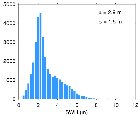
Figure 17. Histogram of flag-valid SWH over oceans and lakes for 11/11/2015. The mean ( \mu ) and standard deviation ( \sigma ) are also shown. Note that values larger than 12 m are excluded from the histogram for the sake of readability but not from the computation of \mu and \sigma .
