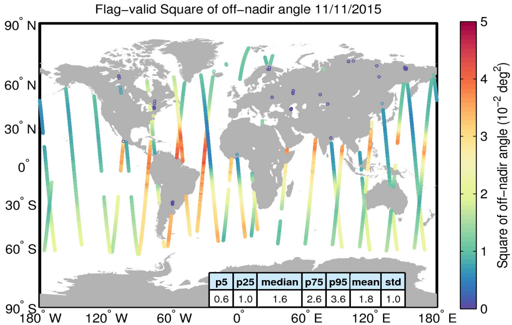
Figure 37. Geographical distribution of flag-valid mispointing data over oceans and lakes for 11/11/2015. The statistical values shown in the table refer to the mispointing in 10^{-2} \text{ deg}^2 and are calculated over all measurements shown in the figure.
