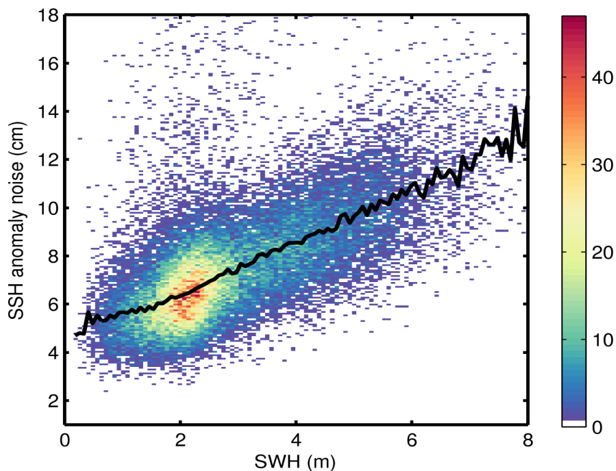
Figure 9. 2D histogram showing flag-valid SSH anomaly noise as a function of SWH for 11/11/2015. The black line denotes the median SSH anomaly noise as a function of SWH.
