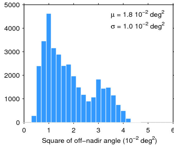
Figure 39. Histogram of flag-valid mispointing over oceans and lakes for 11/11/2015. The mean ( \mu ) and standard deviation ( \sigma ) are also shown. Note that values larger than 6 \cdot 10^{-2} \text{ deg}^2 are excluded from the histogram for the sake of readability but not from the computation of \mu and \sigma .
