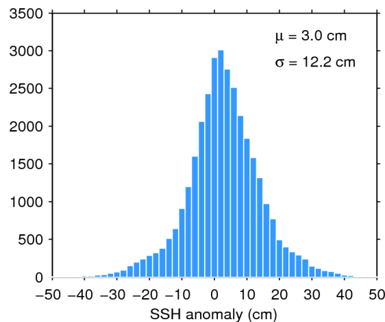
Figure 11. Histogram of science-valid SSH anomaly over oceans and lakes for 11/11/2015. The mean ( \mu ) and standard deviation ( \sigma ) are also shown. Note that values outside [-50 50] cm are excluded from the histogram for the sake of readability but not from the computation of \mu and \sigma .
