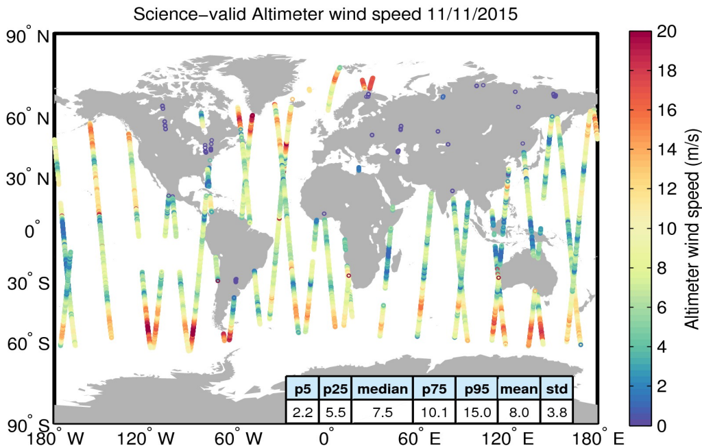
Figure 34. Geographical distribution of science-valid wind data over oceans and lakes for 11/11/2015. The statistical values shown in the table refer to the wind in m/s and are calculated over all measurements shown in the figure. Gray circles denote records that have been rejected based on the editing criteria described in Table 5.
