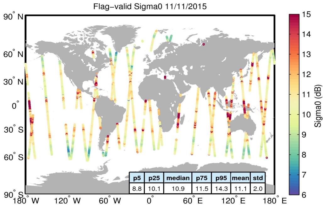
Figure 23. Geographical distribution of flag-valid sigma0 data over oceans and lakes for 11/11/2015. The statistical values shown in the table refer to the sigma0 in dB and are calculated over all measurements shown in the figure.
