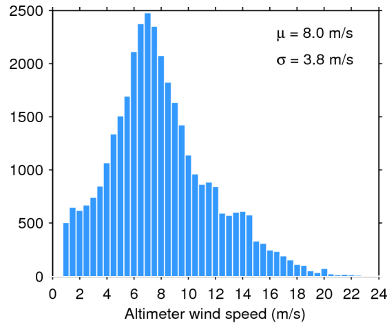
Figure 33. Histogram of flag-valid wind over oceans and lakes for 11/11/2015. The mean ( \mu ) and standard deviation ( \sigma ) are also shown. Note that values larger than 24 m/s are excluded from the histogram for the sake of readability but not from the computation of \mu and \sigma .
