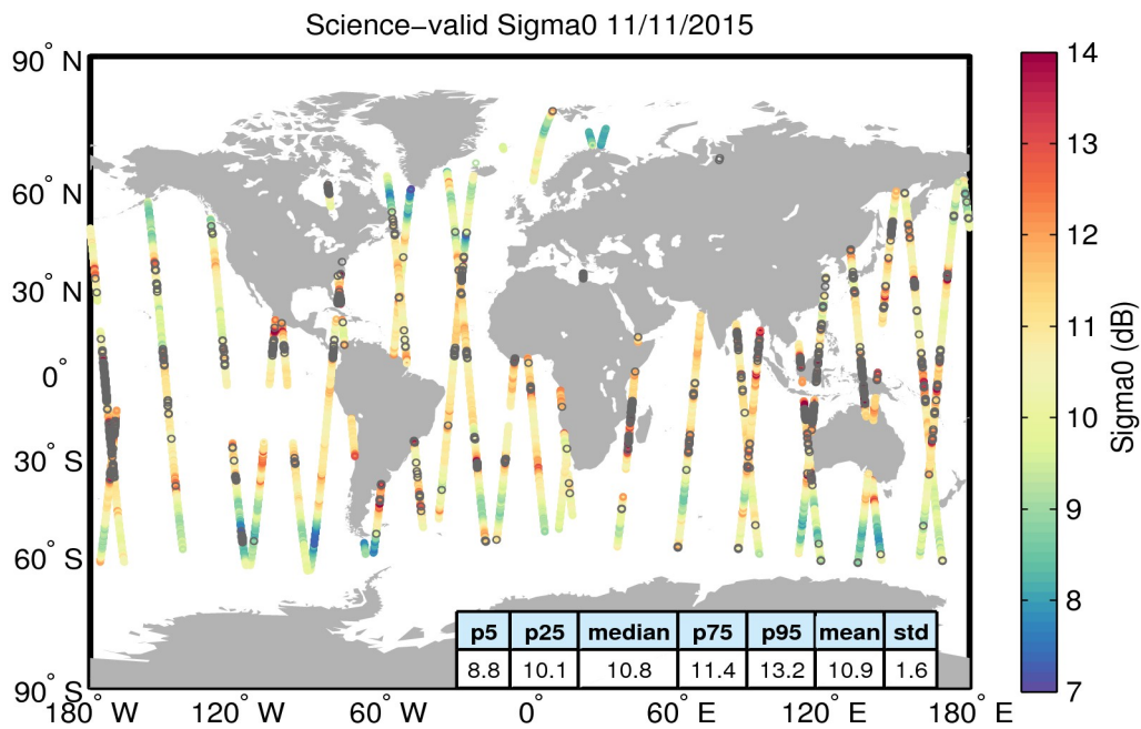
Figure 27. Geographical distribution of science-valid sigma0 data over oceans and lakes for 11/11/2015. The statistical values shown in the table refer to the sigma0 in dB and are calculated over all measurements shown in the figure. Gray circles denote records that have been rejected based on the editing criteria described in Table 4.
