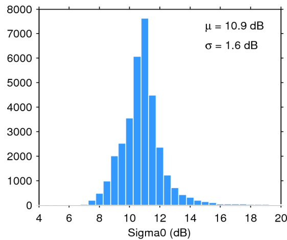
Figure 28. Histogram of science-valid sigma0 over oceans and lakes for 11/11/2015. The mean ( \mu ) and standard deviation ( \sigma ) are also shown. Note that values outside [4 20] dB are excluded from the histogram for the sake of readability but not from the computation of \mu and \sigma .
