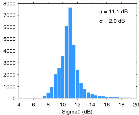
Figure 25. Histogram of flag-valid sigma0 over oceans and lakes for 11/11/2015. The mean ( \mu ) and standard deviation ( \sigma ) are also shown. Note that values outside [4 20] dB are excluded from the histogram for the sake of readability but not from the computation of \mu and \sigma .
