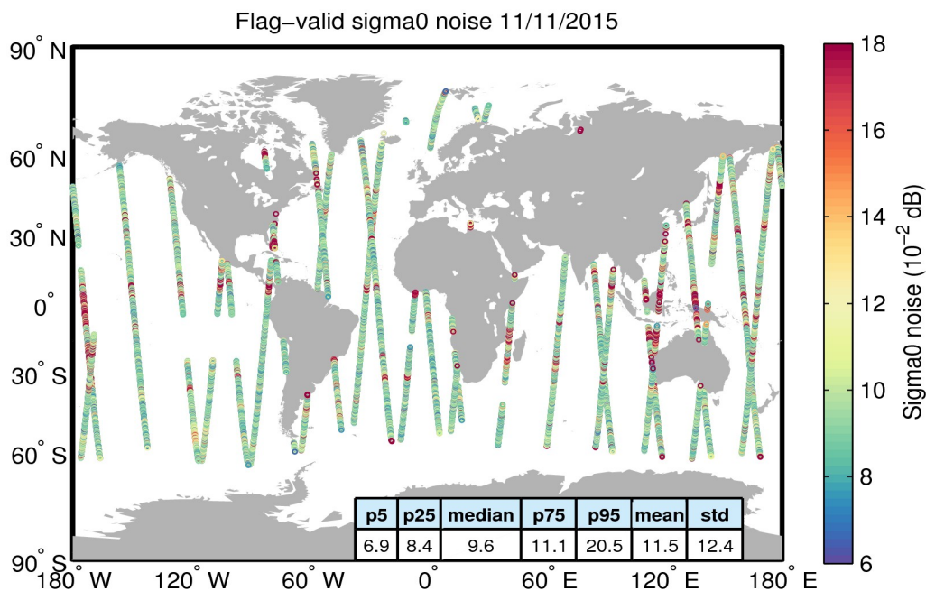
Figure 26. Geographical distribution of flag-valid 20-Hz sigma0 measurement noise over oceans and lakes for 11/11/2015. The statistical values shown in the table refer to the sigma0 noise and are calculated over all measurements shown in the figure.
