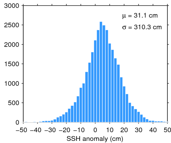
Figure 7. Histogram of flag-valid SSH anomaly over oceans and lakes for 10/11/2015. The mean ( \mu ) and standard deviation ( \sigma ) are also shown. Note that values outside [-50\ 50] cm are excluded from the histogram for the sake of readability but not from the computation of \mu and \sigma .
