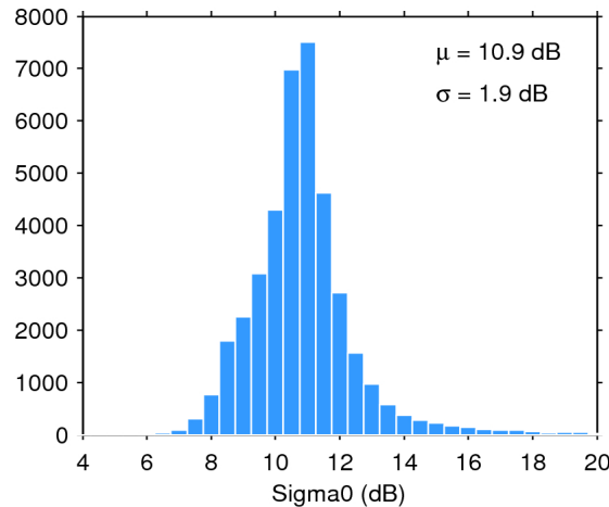
Figure 25. Histogram of flag-valid sigma0 over oceans and lakes for 10/11/2015. The mean ( \mu ) and standard deviation ( \sigma ) are also shown. Note that values outside [4 20] dB are excluded from the histogram for the sake of readability but not from the computation of \mu and \sigma .
