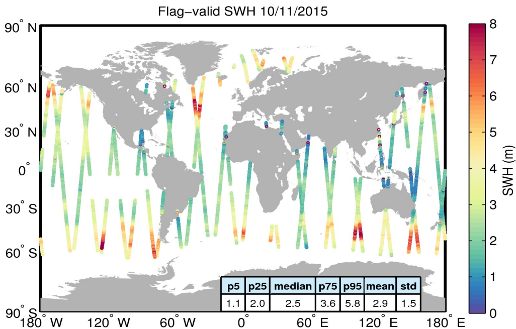
Figure 15. Geographical distribution of flag-valid SWH data over oceans and lakes for 10/11/2015. The statistical values shown in the table refer to the SWH in m and are calculated over all measurements shown in the figure.
