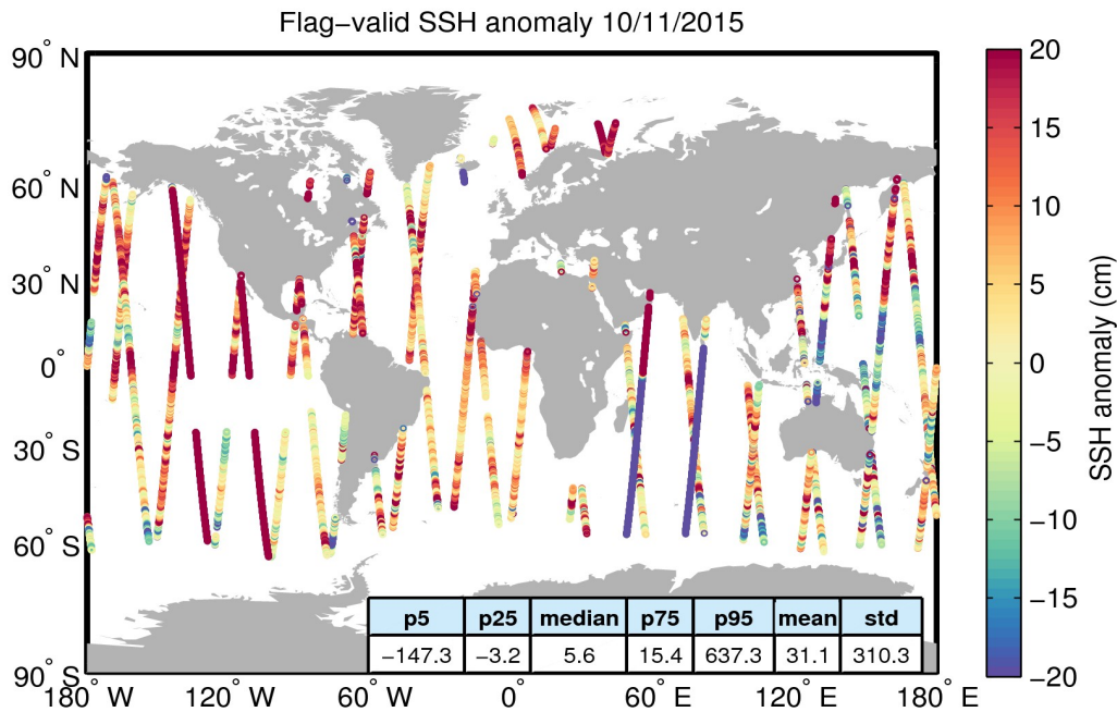
Figure 5. Geographical distribution of flag-valid 1-Hz SSH anomaly data over oceans and lakes for 10/11/2015. The statistical values shown in the table refer to the SSH anomaly in cm and are calculated over all measurements shown in the figure.
