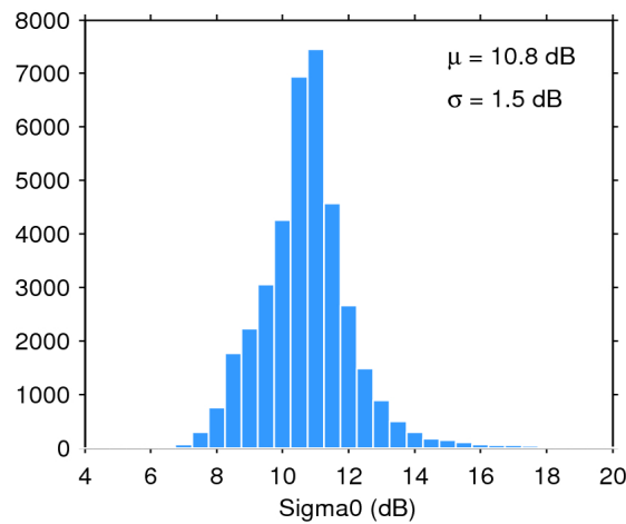
Figure 28. Histogram of science-valid sigma0 over oceans and lakes for 10/11/2015. The mean ( \mu ) and standard deviation ( \sigma ) are also shown. Note that values outside [4 20] dB are excluded from the histogram for the sake of readability but not from the computation of \mu and \sigma .
