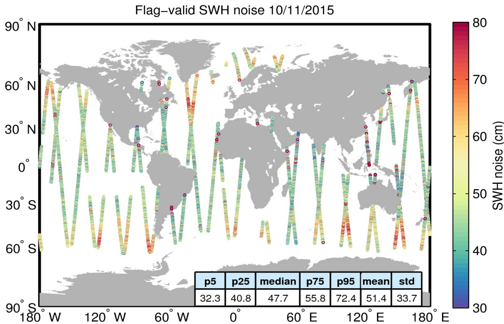
Figure 18. Geographical distribution of flag-valid 20-Hz SWH measurement noise over oceans and lakes for 10/11/2015. The statistical values shown in the figure refer to the SWH noise and are calculated over all measurements shown in the figure.
