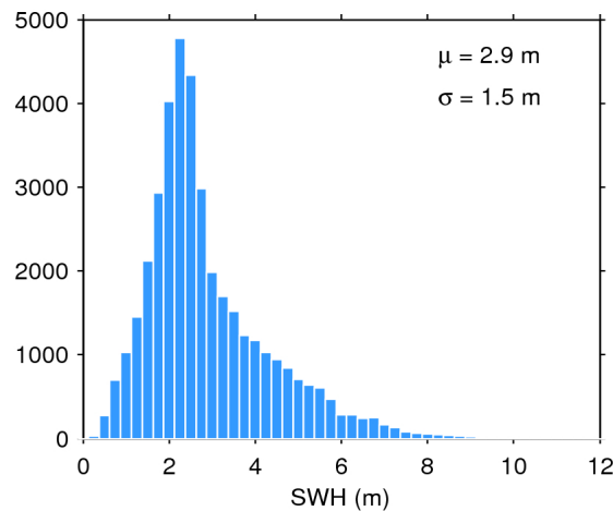
Figure 17. Histogram of flag-valid SWH over oceans and lakes for 10/11/2015. The mean ( \mu ) and standard deviation ( \sigma ) are also shown. Note that values larger than 12 m are excluded from the histogram for the sake of readability but not from the computation of \mu and \sigma .
