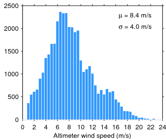
Figure 35. Histogram of science-valid wind over oceans and lakes for 10/11/2015. The mean ( \mu ) and standard deviation ( \sigma ) are also shown. Note that values larger than 24 m/s are excluded from the histogram for the sake of readability but not from the computation of \mu and \sigma .
