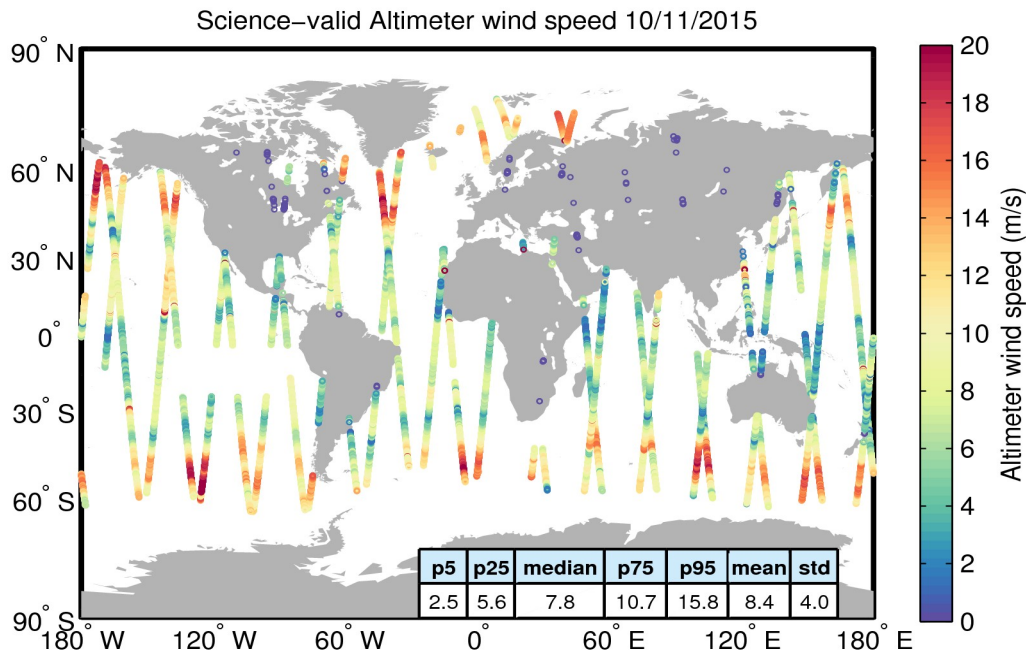
Figure 34. Geographical distribution of science-valid wind data over oceans and lakes for 10/11/2015. The statistical values shown in the table refer to the wind in m/s and are calculated over all measurements shown in the figure. Gray circles denote records that have been rejected based on the editing criteria described in Table 5.
