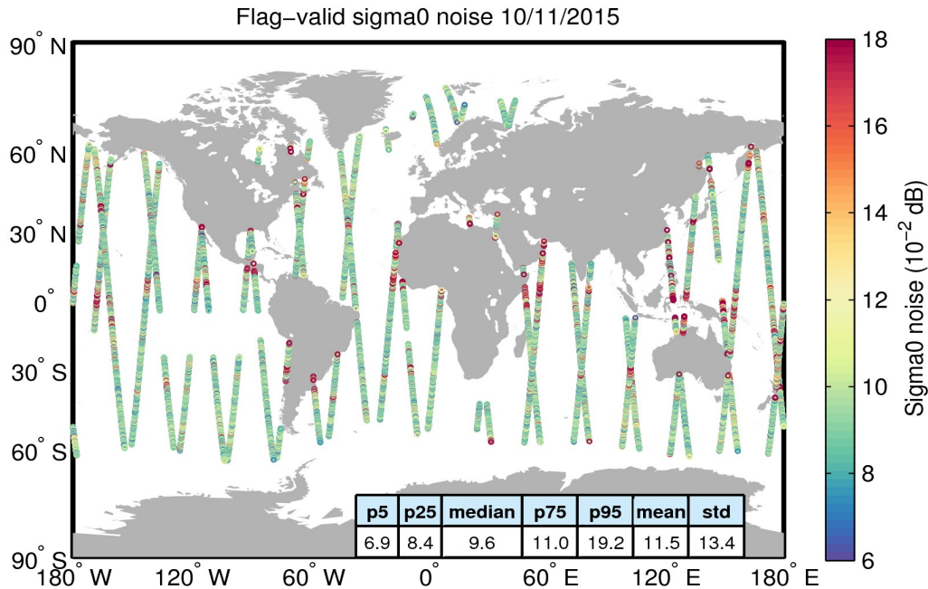
Figure 26. Geographical distribution of flag-valid 20-Hz sigma0 measurement noise over oceans and lakes for 10/11/2015. The statistical values shown in the table refer to the sigma0 noise and are calculated over all measurements shown in the figure.
