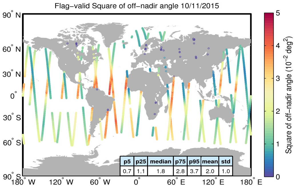
Figure 37. Geographical distribution of flag-valid mispointing data over oceans and lakes for 10/11/2015. The statistical values shown in the table refer to the mispointing in 10^{-2} deg 2 and are calculated over all measurements shown in the figure.
