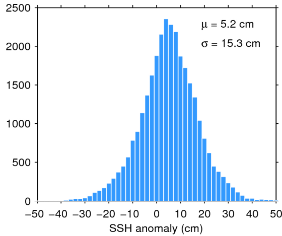
Figure 11. Histogram of science-valid SSH anomaly over oceans and lakes for 10/11/2015. The mean ( \mu ) and standard deviation ( \sigma ) are also shown. Note that values outside [-50 50] cm are excluded from the histogram for the sake of readability but not from the computation of \mu and \sigma .
