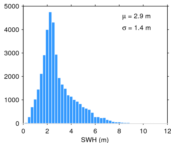
Figure 20. Histogram of science-valid SWH over oceans and lakes for 10/11/2015. The mean ( \mu ) and standard deviation ( \sigma ) are also shown. Note that values larger than 12 m are excluded from the histogram for the sake of readability but not from the computation of \mu and \sigma .
