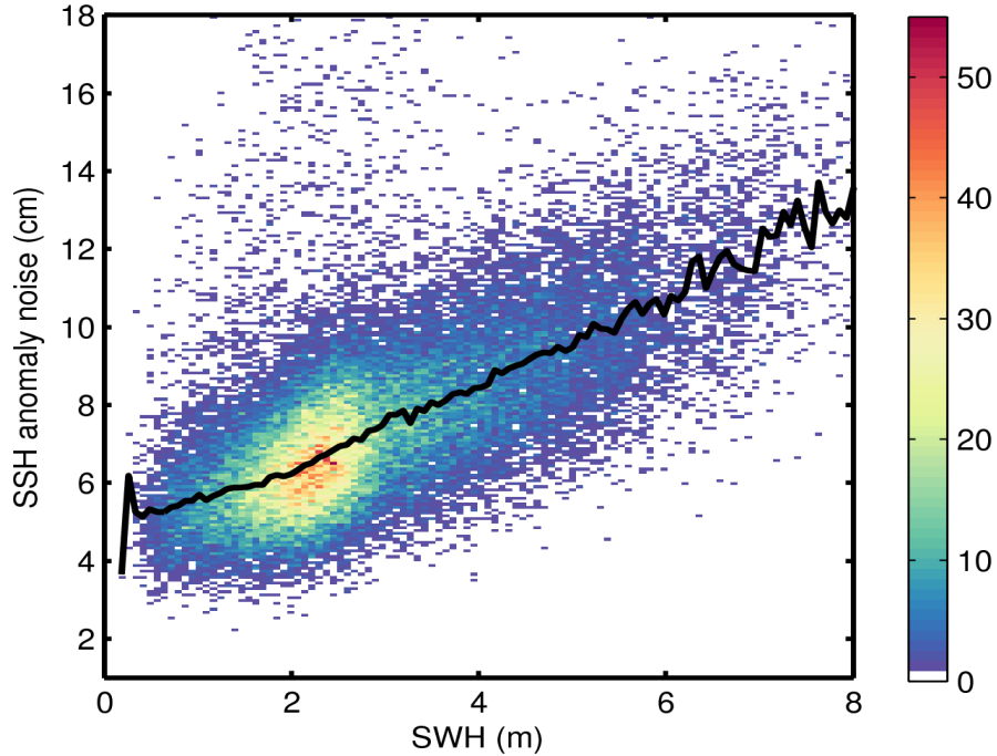
Figure 9. 2D histogram showing flag-valid SSH anomaly noise as a function of SWH for 10/11/2015. The black line denotes the median SSH anomaly noise as a function of SWH.
