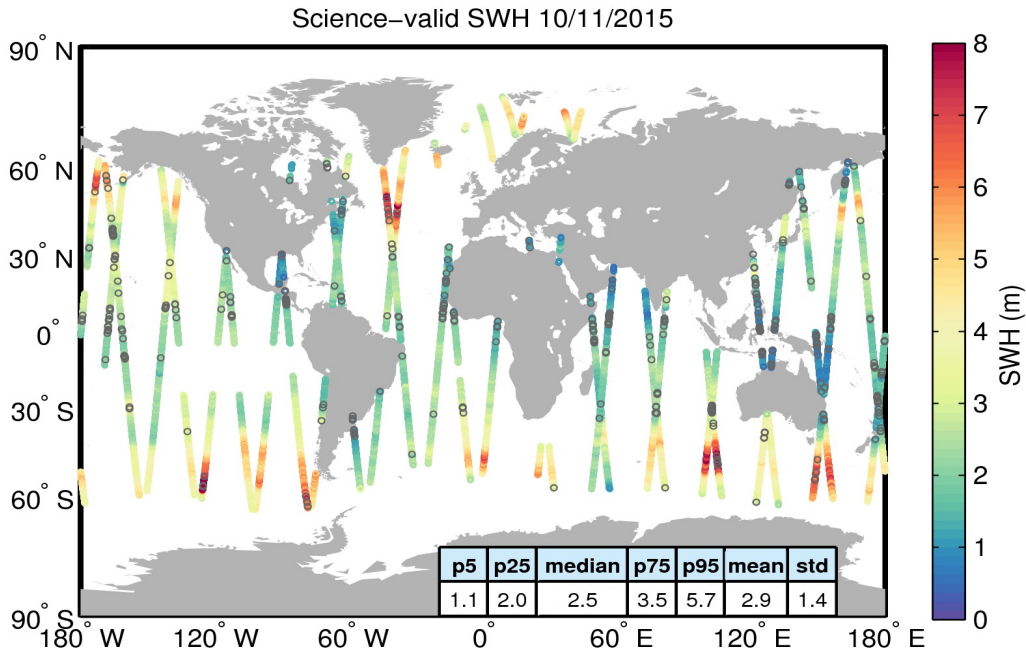
Figure 19. Geographical distribution of science-valid SWH data over oceans and lakes for 10/11/2015. The statistical values shown in the table refer to the SWH in m and are calculated over all measurements shown in the figure. Gray circles denote records that have been rejected based on the editing criteria described in Table 3.
