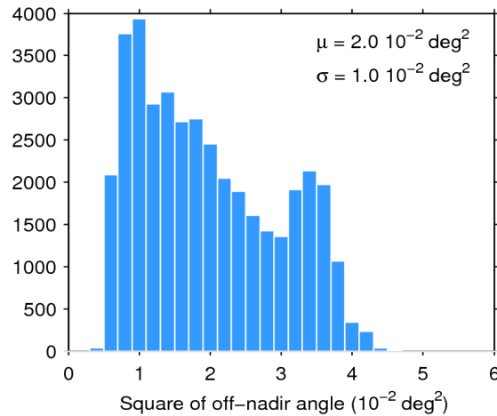
Figure 39. Histogram of flag-valid mispointing over oceans and lakes for 10/11/2015. The mean ( \mu ) and standard deviation ( \sigma ) are also shown. Note that values larger than 6 \cdot 10^{-2} \text{ deg}^2 are excluded from the histogram for the sake of readability but not from the computation of \mu and \sigma .
