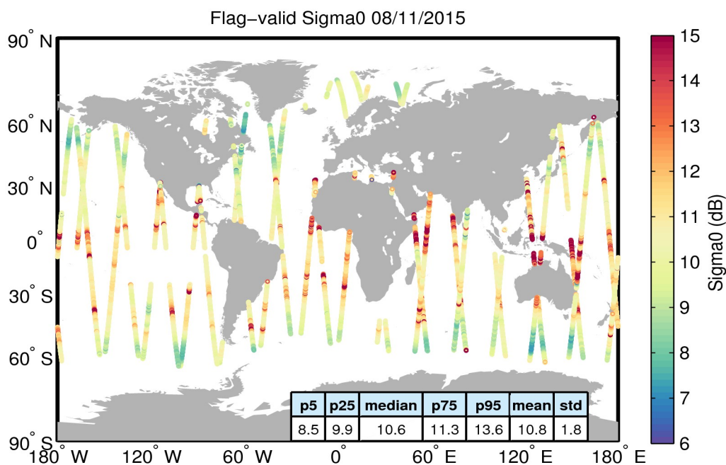
Figure 23. Geographical distribution of flag-valid sigma0 data over oceans and lakes for 08/11/2015. The statistical values shown in the table refer to the sigma0 in dB and are calculated over all measurements shown in the figure.
