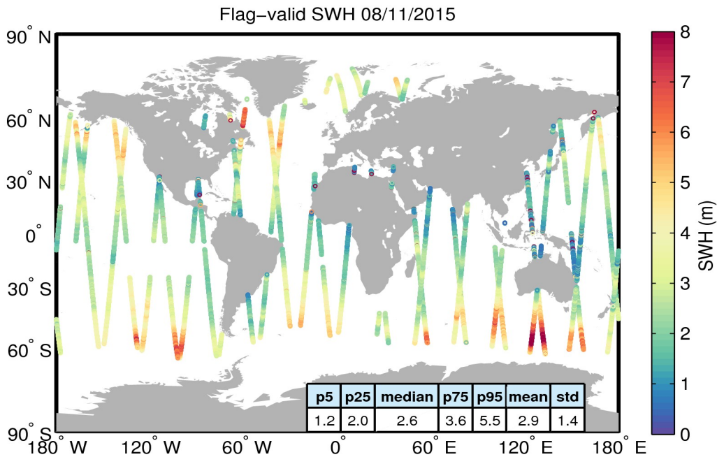
Figure 15. Geographical distribution of flag-valid SWH data over oceans and lakes for 08/11/2015. The statistical values shown in the table refer to the SWH in m and are calculated over all measurements shown in the figure.
