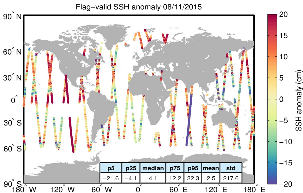
Figure 5. Geographical distribution of flag-valid 1-Hz SSH anomaly data over oceans and lakes for 08/11/2015. The statistical values shown in the table refer to the SSH anomaly in cm and are calculated over all measurements shown in the figure.
