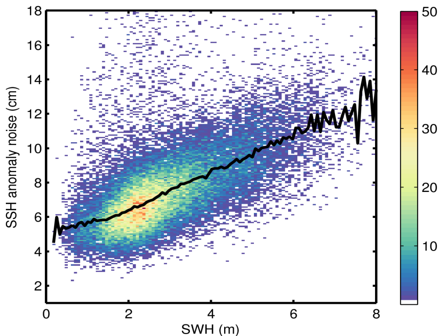
Figure 9. 2D histogram showing flag-valid SSH anomaly noise as a function of SWH for 08/11/2015. The black line denotes the median SSH anomaly noise as a function of SWH.
