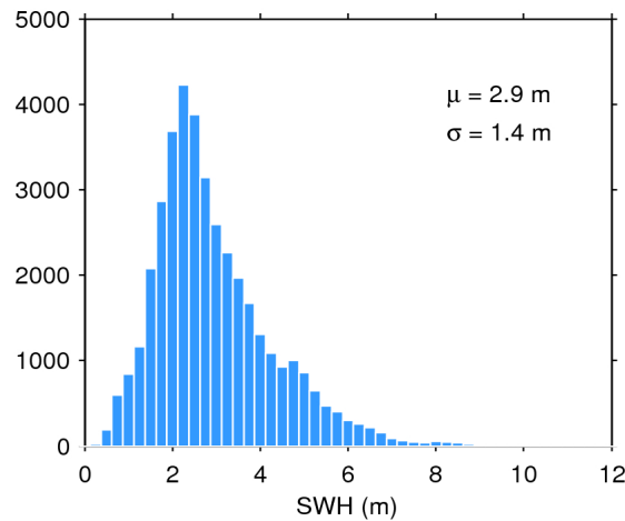
Figure 17. Histogram of flag-valid SWH over oceans and lakes for 08/11/2015. The mean ( \mu ) and standard deviation ( \sigma ) are also shown. Note that values larger than 12 m are excluded from the histogram for the sake of readability but not from the computation of \mu and \sigma .
