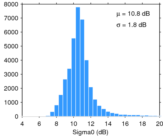
Figure 25. Histogram of flag-valid sigma0 over oceans and lakes for 08/11/2015. The mean ( \mu ) and standard deviation ( \sigma ) are also shown. Note that values outside [4 20] dB are excluded from the histogram for the sake of readability but not from the computation of \mu and \sigma .
