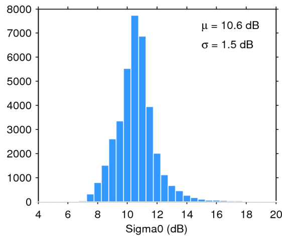
Figure 28. Histogram of science-valid sigma0 over oceans and lakes for 08/11/2015. The mean ( \mu ) and standard deviation ( \sigma ) are also shown. Note that values outside [4 20] dB are excluded from the histogram for the sake of readability but not from the computation of \mu and \sigma .
