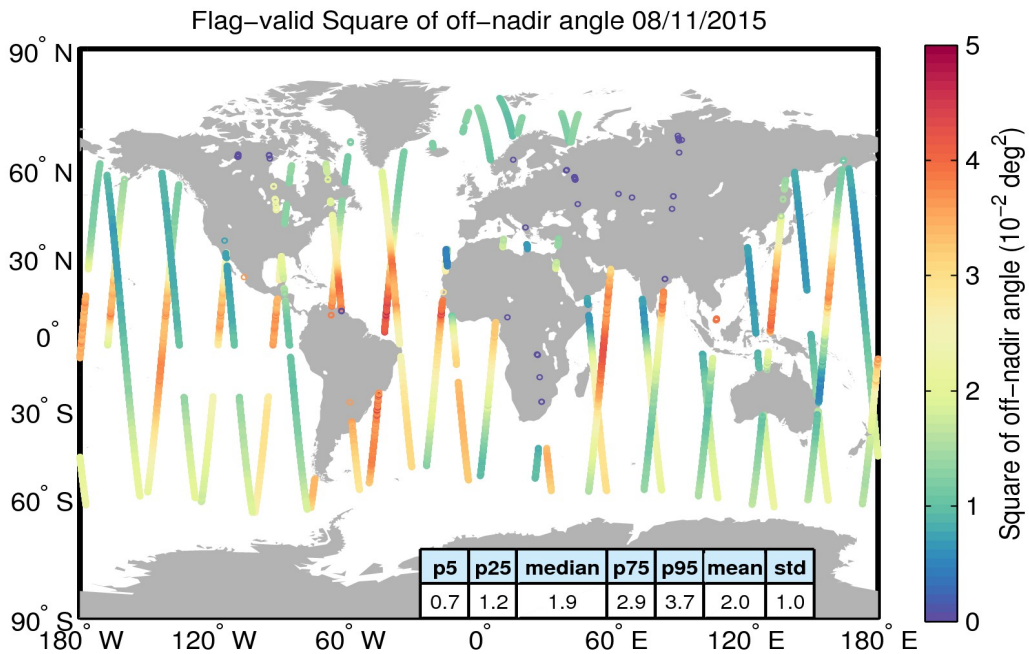
Figure 37. Geographical distribution of flag-valid mispointing data over oceans and lakes for 08/11/2015. The statistical values shown in the table refer to the mispointing in 10^{-2} \text{ deg}^2 and are calculated over all measurements shown in the figure.
