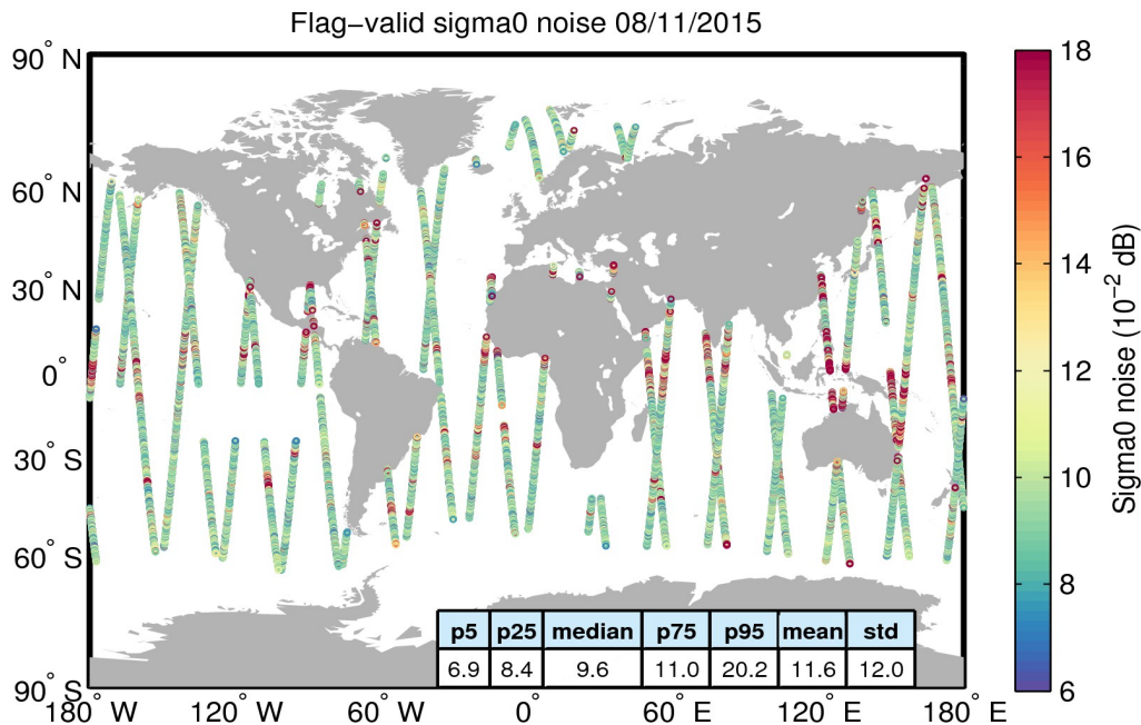
Figure 26. Geographical distribution of flag-valid 20-Hz sigma0 measurement noise over oceans and lakes for 08/11/2015. The statistical values shown in the table refer to the sigma0 noise and are calculated over all measurements shown in the figure.
