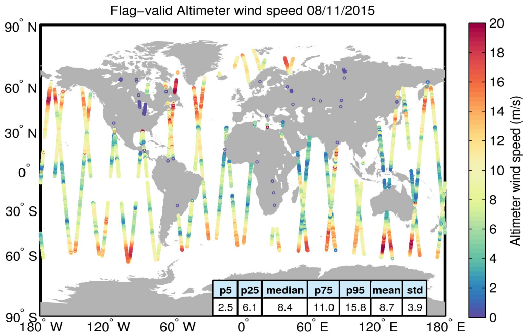
Figure 31. Geographical distribution of flag-valid wind data over oceans and lakes for 08/11/2015. The statistical values shown in the table refer to the wind in m/s and are calculated over all measurements shown in the figure.
