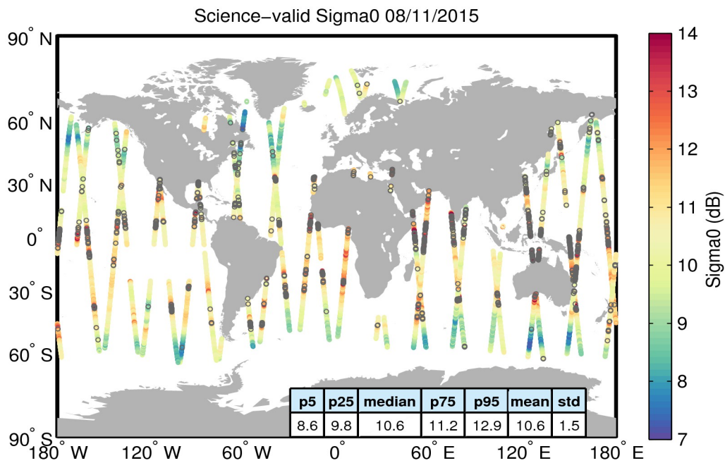
Figure 27. Geographical distribution of science-valid sigma0 data over oceans and lakes for 08/11/2015. The statistical values shown in the table refer to the sigma0 in dB and are calculated over all measurements shown in the figure. Gray circles denote records that have been rejected based on the editing criteria described in Table 4.
