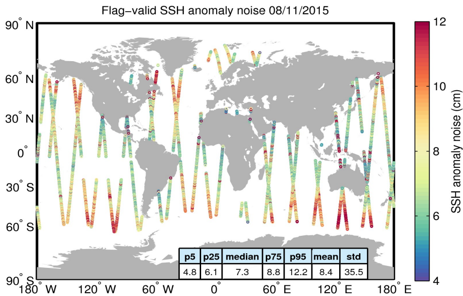
Figure 8. Geographical distribution of flag-valid 20-Hz SSH anomaly measurement noise over oceans and lakes for 08/11/2015. The statistical values shown in the table refer to the SSH anomaly noise and are calculated over all measurements shown in the figure.
