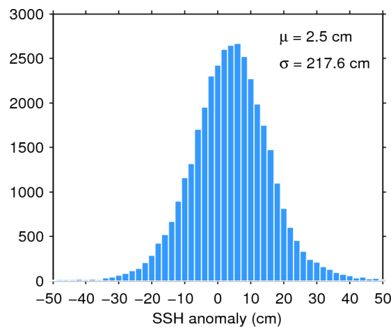
Figure 7. Histogram of flag-valid SSH anomaly over oceans and lakes for 08/11/2015. The mean ( \mu ) and standard deviation ( \sigma ) are also shown. Note that values outside [-50\ 50] cm are excluded from the histogram for the sake of readability but not from the computation of \mu and \sigma .
