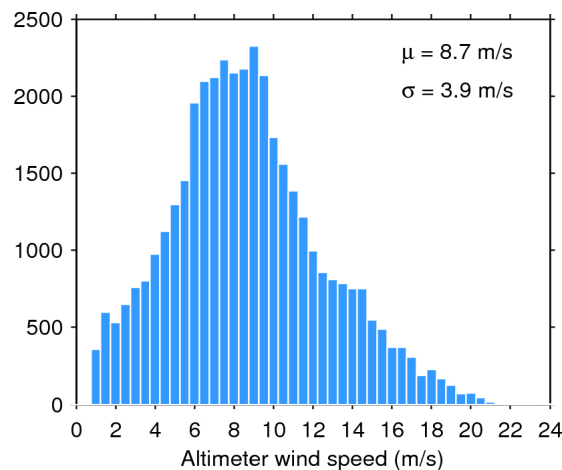
Figure 35. Histogram of science-valid wind over oceans and lakes for 08/11/2015. The mean ( \mu ) and standard deviation ( \sigma ) are also shown. Note that values larger than 24 m/s are excluded from the histogram for the sake of readability but not from the computation of \mu and \sigma .
