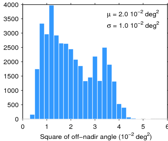
Figure 39. Histogram of flag-valid mispointing over oceans and lakes for 08/11/2015. The mean ( \mu ) and standard deviation ( \sigma ) are also shown. Note that values larger than 6 \cdot 10^{-2} \text{ deg}^2 are excluded from the histogram for the sake of readability but not from the computation of \mu and \sigma .
