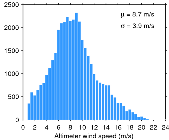
Figure 33. Histogram of flag-valid wind over oceans and lakes for 08/11/2015. The mean ( \mu ) and standard deviation ( \sigma ) are also shown. Note that values larger than 24 m/s are excluded from the histogram for the sake of readability but not from the computation of \mu and \sigma .
