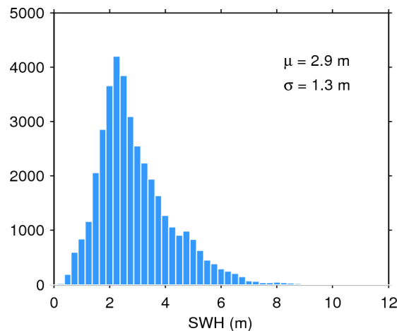
Figure 20. Histogram of science-valid SWH over oceans and lakes for 08/11/2015. The mean ( \mu ) and standard deviation ( \sigma ) are also shown. Note that values larger than 12 m are excluded from the histogram for the sake of readability but not from the computation of \mu and \sigma .
