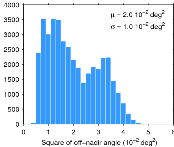
Figure 39. Histogram of flag-valid mispointing over oceans and lakes for 07/11/2015. The mean ( \mu ) and standard deviation ( \sigma ) are also shown. Note that values larger than 6 \cdot 10^{-2} \text{ deg}^2 are excluded from the histogram for the sake of readability but not from the computation of \mu and \sigma .
