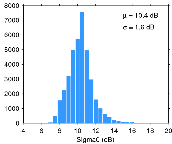
Figure 28. Histogram of science-valid sigma0 over oceans and lakes for 07/11/2015. The mean ( \mu ) and standard deviation ( \sigma ) are also shown. Note that values outside [4 20] dB are excluded from the histogram for the sake of readability but not from the computation of \mu and \sigma .
