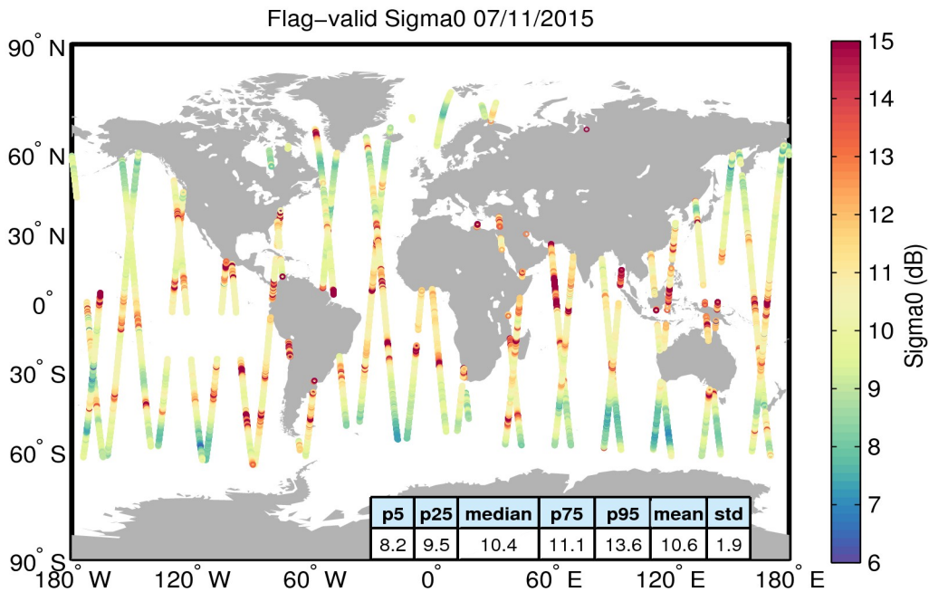
Figure 23. Geographical distribution of flag-valid sigma0 data over oceans and lakes for 07/11/2015. The statistical values shown in the table refer to the sigma0 in dB and are calculated over all measurements shown in the figure.
