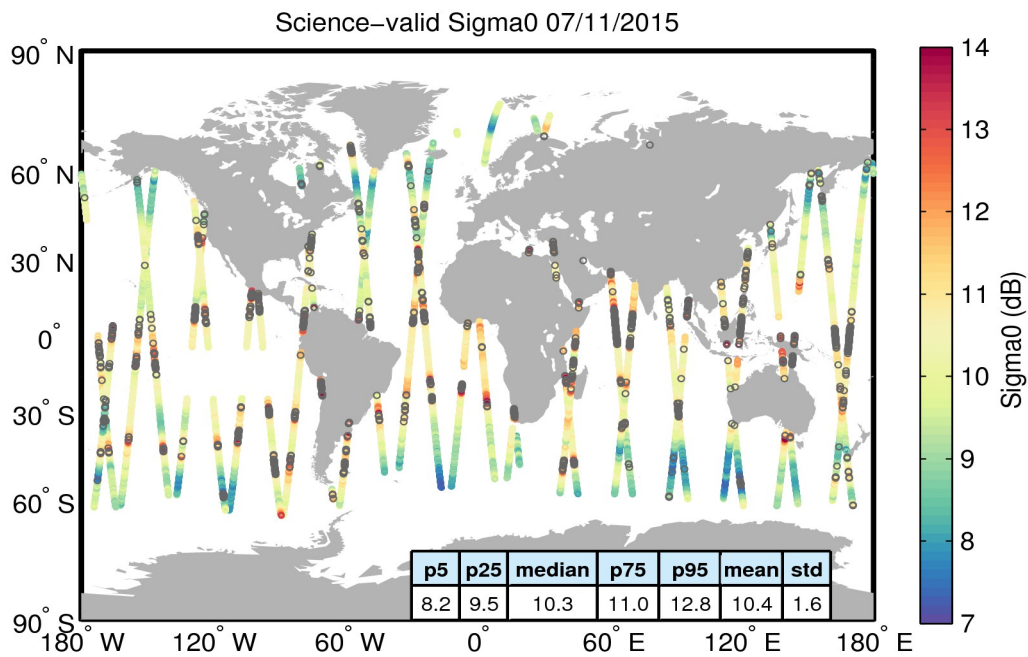
Figure 27. Geographical distribution of science-valid sigma0 data over oceans and lakes for 07/11/2015. The statistical values shown in the table refer to the sigma0 in dB and are calculated over all measurements shown in the figure. Gray circles denote records that have been rejected based on the editing criteria described in Table 4.
