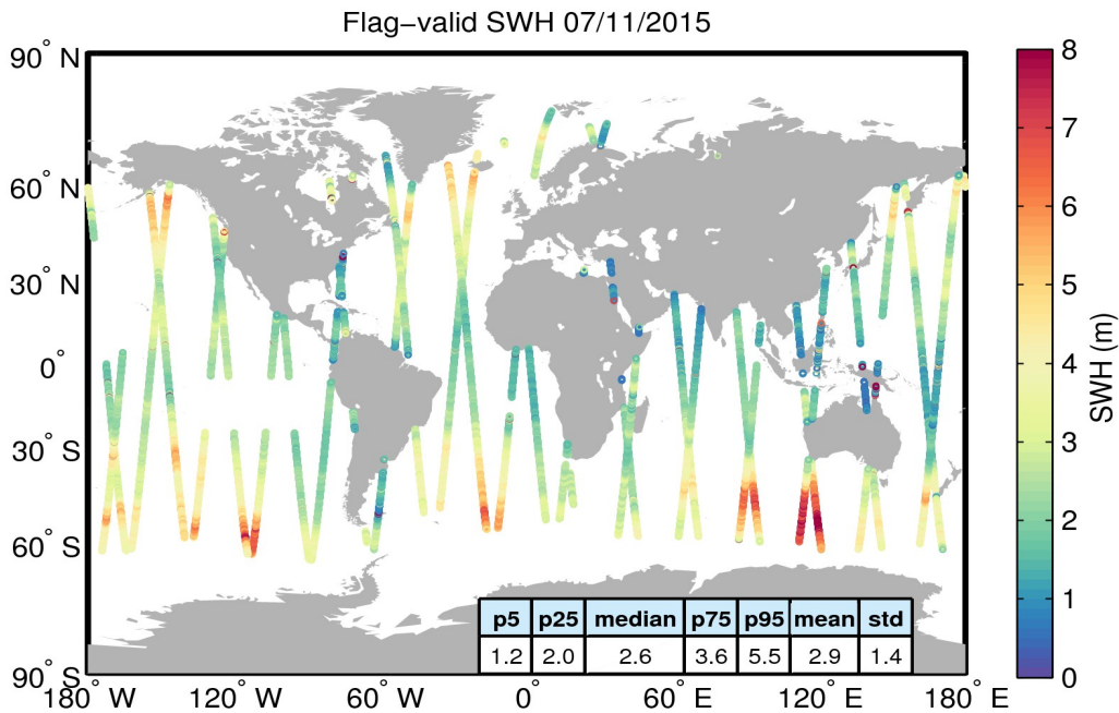
Figure 15. Geographical distribution of flag-valid SWH data over oceans and lakes for 07/11/2015. The statistical values shown in the table refer to the SWH in m and are calculated over all measurements shown in the figure.
