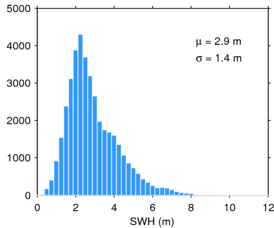
Figure 17. Histogram of flag-valid SWH over oceans and lakes for 07/11/2015. The mean ( \mu ) and standard deviation ( \sigma ) are also shown. Note that values larger than 12 m are excluded from the histogram for the sake of readability but not from the computation of \mu and \sigma .
