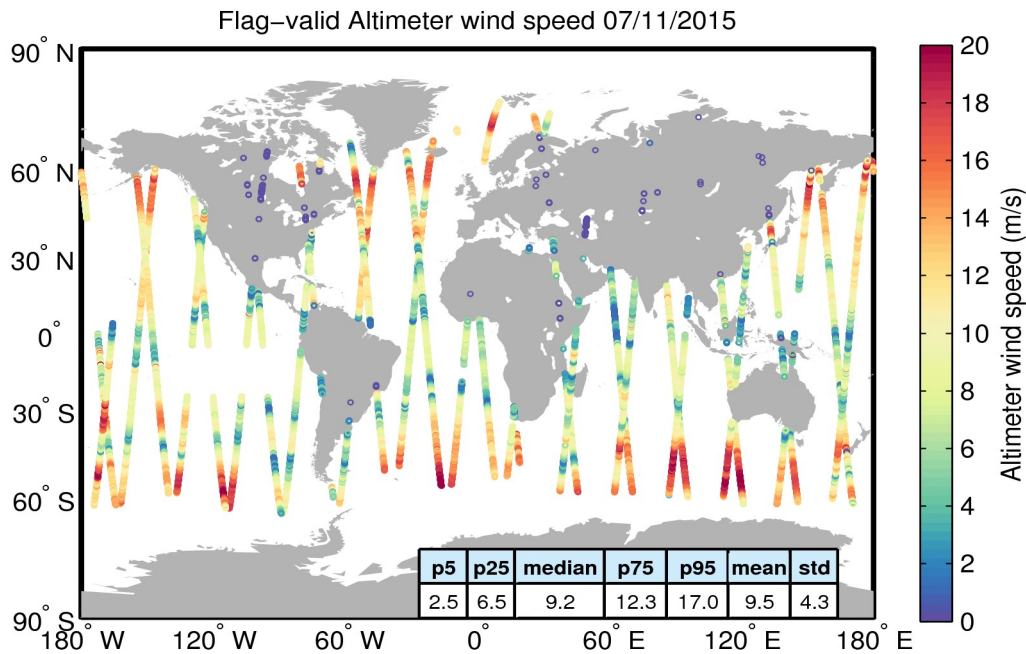
Figure 31. Geographical distribution of flag-valid wind data over oceans and lakes for 07/11/2015. The statistical values shown in the table refer to the wind in m/s and are calculated over all measurements shown in the figure.
