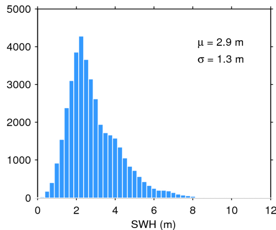
Figure 20. Histogram of science-valid SWH over oceans and lakes for 07/11/2015. The mean ( \mu ) and standard deviation ( \sigma ) are also shown. Note that values larger than 12 m are excluded from the histogram for the sake of readability but not from the computation of \mu and \sigma .
