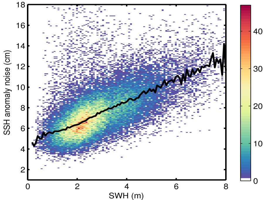
Figure 9. 2D histogram showing flag-valid SSH anomaly noise as a function of SWH for 07/11/2015. The black line denotes the median SSH anomaly noise as a function of SWH.
