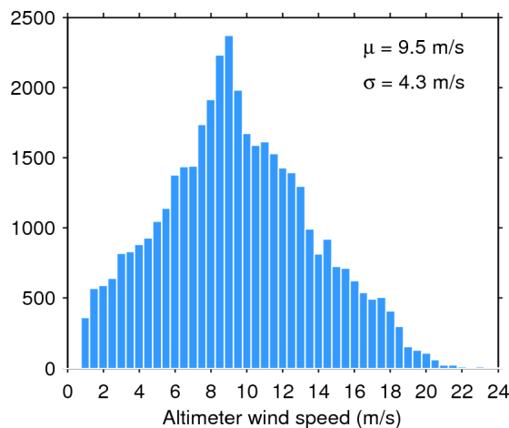
Figure 35. Histogram of science-valid wind over oceans and lakes for 07/11/2015. The mean ( \mu ) and standard deviation ( \sigma ) are also shown. Note that values larger than 24 m/s are excluded from the histogram for the sake of readability but not from the computation of \mu and \sigma .
