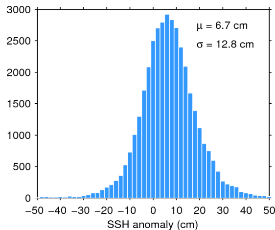
Figure 11. Histogram of science-valid SSH anomaly over oceans and lakes for 07/11/2015. The mean ( \mu ) and standard deviation ( \sigma ) are also shown. Note that values outside [-50 50] cm are excluded from the histogram for the sake of readability but not from the computation of \mu and \sigma .
