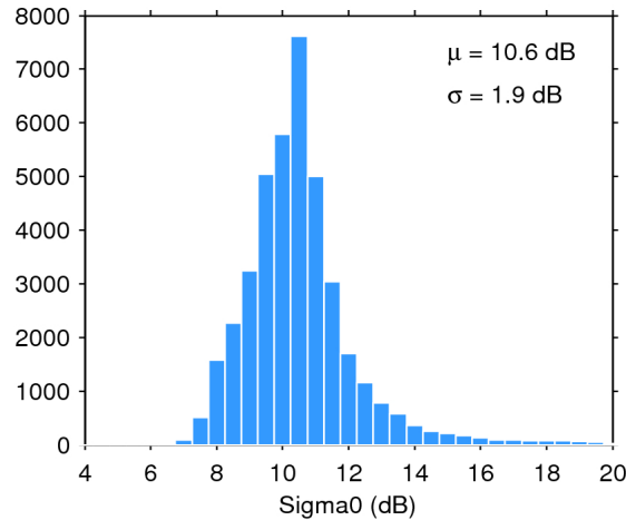
Figure 25. Histogram of flag-valid sigma0 over oceans and lakes for 07/11/2015. The mean ( \mu ) and standard deviation ( \sigma ) are also shown. Note that values outside [4 20] dB are excluded from the histogram for the sake of readability but not from the computation of \mu and \sigma .
