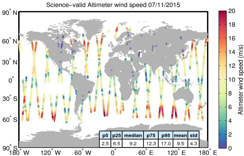
Figure 34. Geographical distribution of science-valid wind data over oceans and lakes for 07/11/2015. The statistical values shown in the table refer to the wind in m/s and are calculated over all measurements shown in the figure. Gray circles denote records that have been rejected based on the editing criteria described in Table 5.
