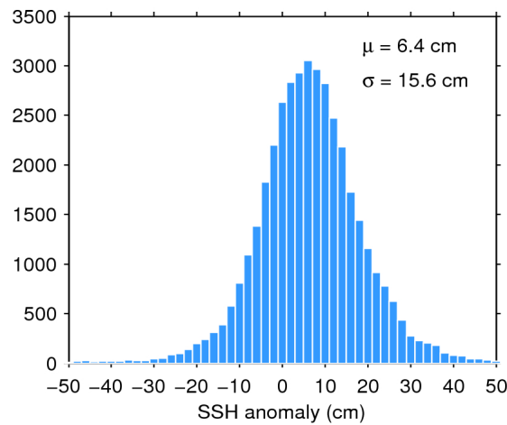
Figure 7. Histogram of flag-valid SSH anomaly over oceans and lakes for 07/11/2015. The mean ( \mu ) and standard deviation ( \sigma ) are also shown. Note that values outside [-50 50] cm are excluded from the histogram for the sake of readability but not from the computation of \mu and \sigma .
