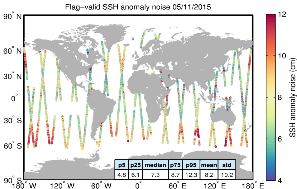
Figure 8. Geographical distribution of flag-valid 20-Hz SSH anomaly measurement noise over oceans and lakes for 05/11/2015. The statistical values shown in the table refer to the SSH anomaly noise and are calculated over all measurements shown in the figure.
