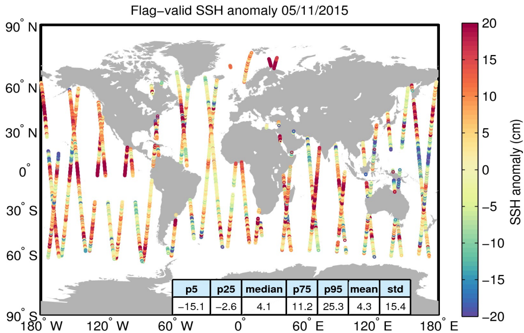
Figure 5. Geographical distribution of flag-valid 1-Hz SSH anomaly data over oceans and lakes for 05/11/2015. The statistical values shown in the table refer to the SSH anomaly in cm and are calculated over all measurements shown in the figure.
