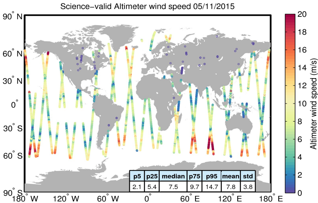
Figure 34. Geographical distribution of science-valid wind data over oceans and lakes for 05/11/2015. The statistical values shown in the table refer to the wind in m/s and are calculated over all measurements shown in the figure. Gray circles denote records that have been rejected based on the editing criteria described in Table 5.
