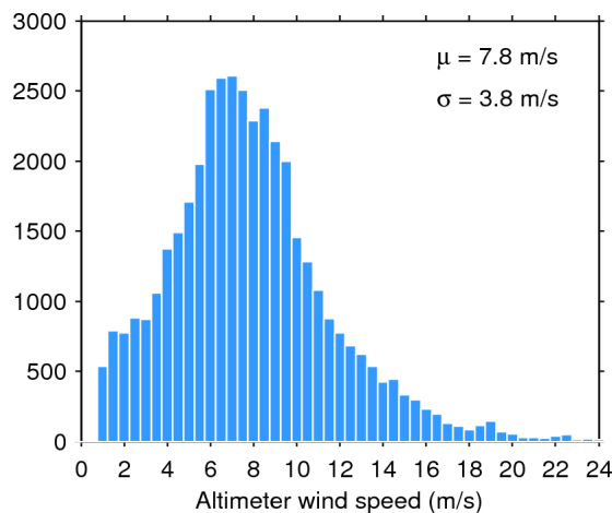
Figure 35. Histogram of science-valid wind over oceans and lakes for 05/11/2015. The mean ( \mu ) and standard deviation ( \sigma ) are also shown. Note that values larger than 24 m/s are excluded from the histogram for the sake of readability but not from the computation of \mu and \sigma .
