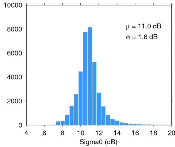
Figure 28. Histogram of science-valid sigma0 over oceans and lakes for 05/11/2015. The mean ( \mu ) and standard deviation ( \sigma ) are also shown. Note that values outside [4 20] dB are excluded from the histogram for the sake of readability but not from the computation of \mu and \sigma .
