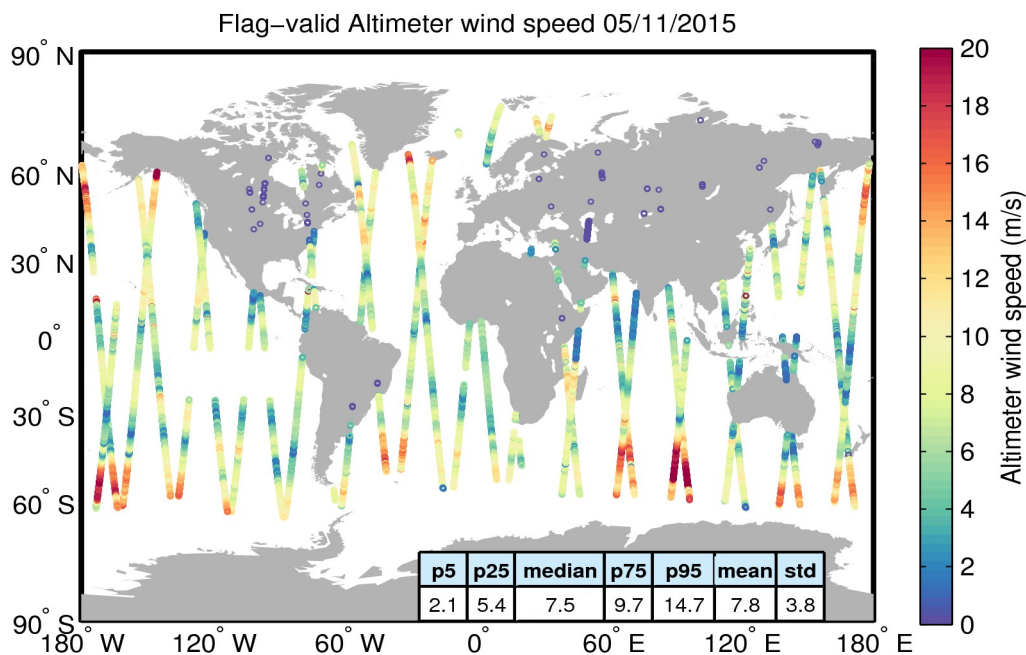
Figure 31. Geographical distribution of flag-valid wind data over oceans and lakes for 05/11/2015. The statistical values shown in the table refer to the wind in m/s and are calculated over all measurements shown in the figure.
