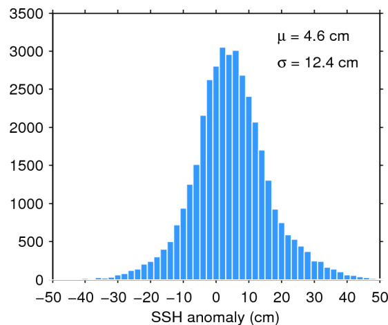
Figure 11. Histogram of science-valid SSH anomaly over oceans and lakes for 05/11/2015. The mean ( \mu ) and standard deviation ( \sigma ) are also shown. Note that values outside [-50 50] cm are excluded from the histogram for the sake of readability but not from the computation of \mu and \sigma .
