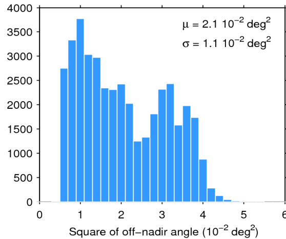
Figure 39. Histogram of flag-valid mispointing over oceans and lakes for 05/11/2015. The mean ( \mu ) and standard deviation ( \sigma ) are also shown. Note that values larger than 6 \cdot 10^{-2} \text{ deg}^2 are excluded from the histogram for the sake of readability but not from the computation of \mu and \sigma .
