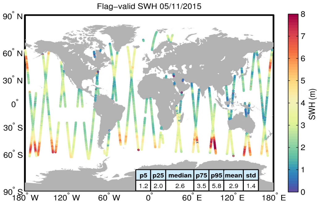
Figure 15. Geographical distribution of flag-valid SWH data over oceans and lakes for 05/11/2015. The statistical values shown in the table refer to the SWH in m and are calculated over all measurements shown in the figure.
