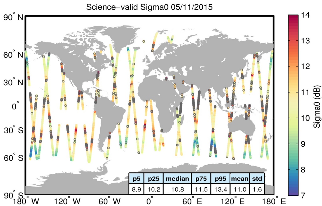
Figure 27. Geographical distribution of science-valid sigma0 data over oceans and lakes for 05/11/2015. The statistical values shown in the table refer to the sigma0 in dB and are calculated over all measurements shown in the figure. Gray circles denote records that have been rejected based on the editing criteria described in Table 4.
