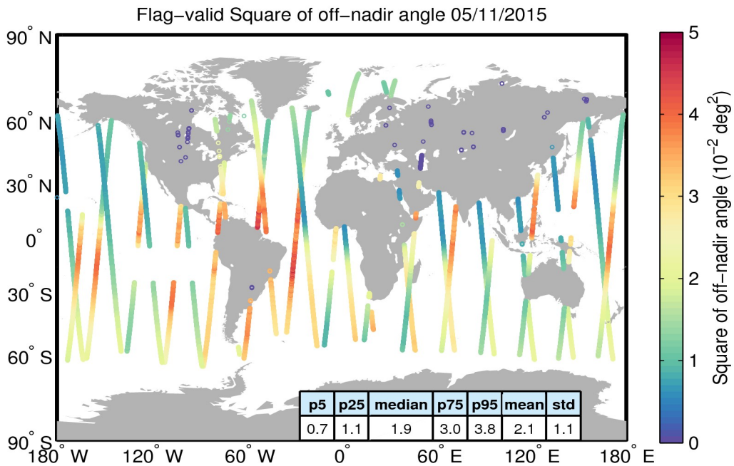
Figure 37. Geographical distribution of flag-valid mispointing data over oceans and lakes for 05/11/2015. The statistical values shown in the table refer to the mispointing in 10^{-2} \text{deg}^2 and are calculated over all measurements shown in the figure.
