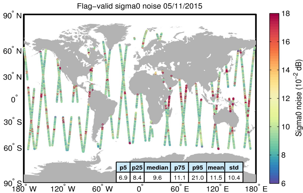
Figure 26. Geographical distribution of flag-valid 20-Hz sigma0 measurement noise over oceans and lakes for 05/11/2015. The statistical values shown in the table refer to the sigma0 noise and are calculated over all measurements shown in the figure.
