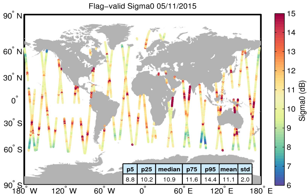
Figure 23. Geographical distribution of flag-valid sigma0 data over oceans and lakes for 05/11/2015. The statistical values shown in the table refer to the sigma0 in dB and are calculated over all measurements shown in the figure.
