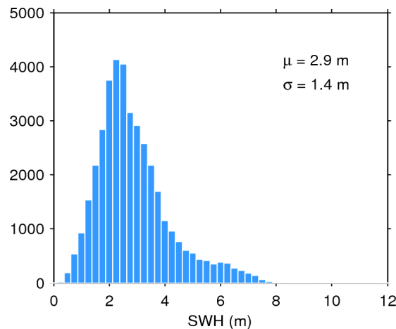
Figure 20. Histogram of science-valid SWH over oceans and lakes for 05/11/2015. The mean ( \mu ) and standard deviation ( \sigma ) are also shown. Note that values larger than 12 m are excluded from the histogram for the sake of readability but not from the computation of \mu and \sigma .
