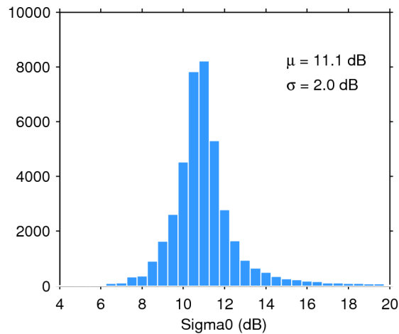
Figure 25. Histogram of flag-valid sigma0 over oceans and lakes for 05/11/2015. The mean ( \mu ) and standard deviation ( \sigma ) are also shown. Note that values outside [4 20] dB are excluded from the histogram for the sake of readability but not from the computation of \mu and \sigma .
