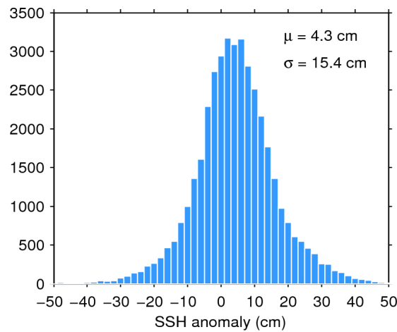
Figure 7. Histogram of flag-valid SSH anomaly over oceans and lakes for 05/11/2015. The mean ( \mu ) and standard deviation ( \sigma ) are also shown. Note that values outside [-50\ 50] cm are excluded from the histogram for the sake of readability but not from the computation of \mu and \sigma .
