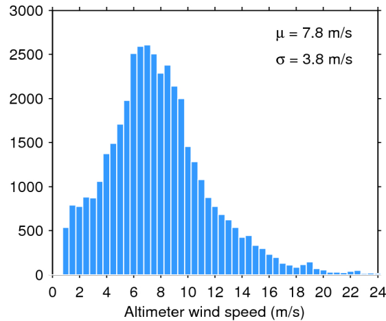
Figure 33. Histogram of flag-valid wind over oceans and lakes for 05/11/2015. The mean ( \mu ) and standard deviation ( \sigma ) are also shown. Note that values larger than 24 m/s are excluded from the histogram for the sake of readability but not from the computation of \mu and \sigma .
