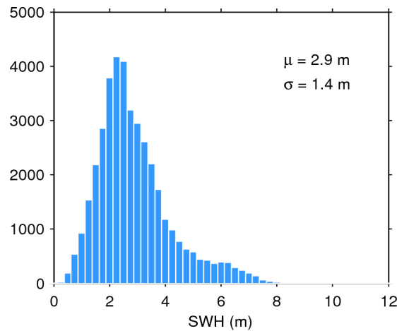
Figure 17. Histogram of flag-valid SWH over oceans and lakes for 05/11/2015. The mean ( \mu ) and standard deviation ( \sigma ) are also shown. Note that values larger than 12 m are excluded from the histogram for the sake of readability but not from the computation of \mu and \sigma .
