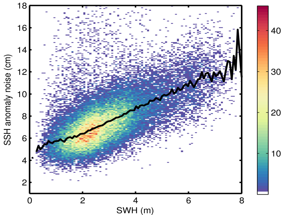
Figure 9. 2D histogram showing flag-valid SSH anomaly noise as a function of SWH for 05/11/2015. The black line denotes the median SSH anomaly noise as a function of SWH.
