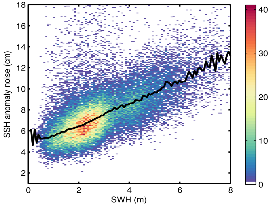
Figure 9. 2D histogram showing flag-valid SSH anomaly noise as a function of SWH for 04/11/2015. The black line denotes the median SSH anomaly noise as a function of SWH.
