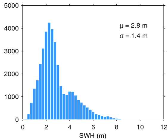
Figure 20. Histogram of science-valid SWH over oceans and lakes for 04/11/2015. The mean ( \mu ) and standard deviation ( \sigma ) are also shown. Note that values larger than 12 m are excluded from the histogram for the sake of readability but not from the computation of \mu and \sigma .
