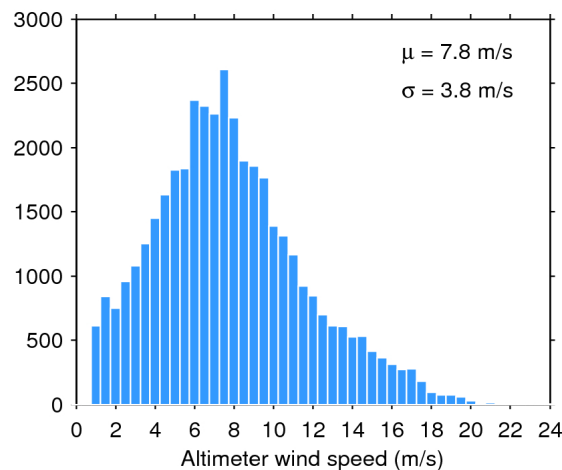
Figure 35. Histogram of science-valid wind over oceans and lakes for 04/11/2015. The mean ( \mu ) and standard deviation ( \sigma ) are also shown. Note that values larger than 24 m/s are excluded from the histogram for the sake of readability but not from the computation of \mu and \sigma .
