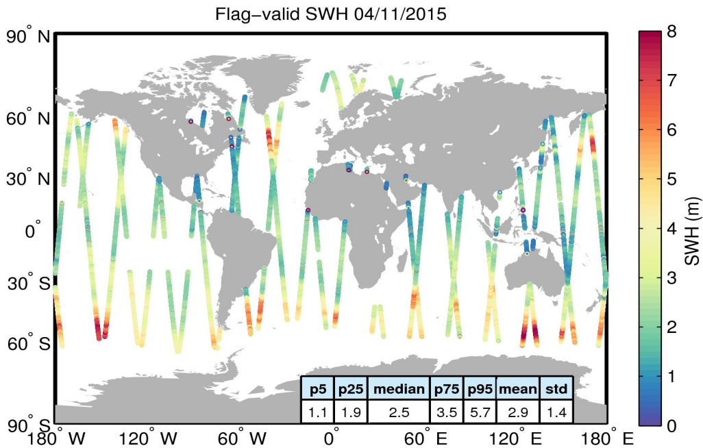
Figure 15. Geographical distribution of flag-valid SWH data over oceans and lakes for 04/11/2015. The statistical values shown in the table refer to the SWH in m and are calculated over all measurements shown in the figure.
