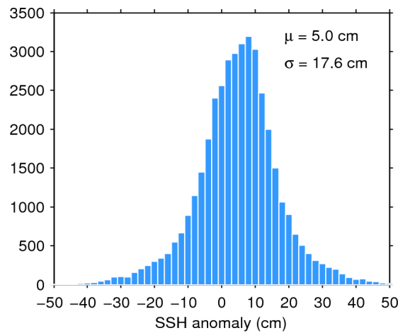
Figure 7. Histogram of flag-valid SSH anomaly over oceans and lakes for 04/11/2015. The mean ( \mu ) and standard deviation ( \sigma ) are also shown. Note that values outside [-50\ 50] cm are excluded from the histogram for the sake of readability but not from the computation of \mu and \sigma .
