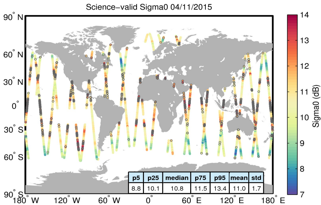
Figure 27. Geographical distribution of science-valid sigma0 data over oceans and lakes for 04/11/2015. The statistical values shown in the table refer to the sigma0 in dB and are calculated over all measurements shown in the figure. Gray circles denote records that have been rejected based on the editing criteria described in Table 4.
