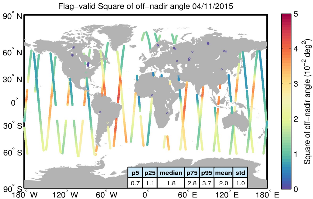
Figure 37. Geographical distribution of flag-valid mispointing data over oceans and lakes for 04/11/2015. The statistical values shown in the table refer to the mispointing in 10^{-2} deg 2 and are calculated over all measurements shown in the figure.
