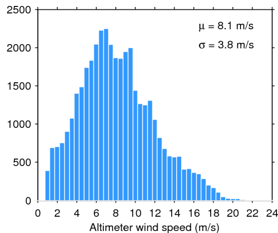
Figure 35. Histogram of science-valid wind over oceans and lakes for 03/11/2015. The mean ( \mu ) and standard deviation ( \sigma ) are also shown. Note that values larger than 24 m/s are excluded from the histogram for the sake of readability but not from the computation of \mu and \sigma .
