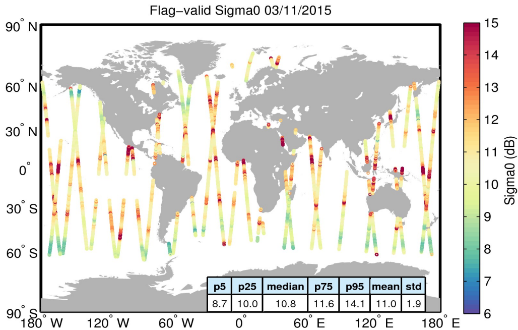
Figure 23. Geographical distribution of flag-valid sigma0 data over oceans and lakes for 03/11/2015. The statistical values shown in the table refer to the sigma0 in dB and are calculated over all measurements shown in the figure.
