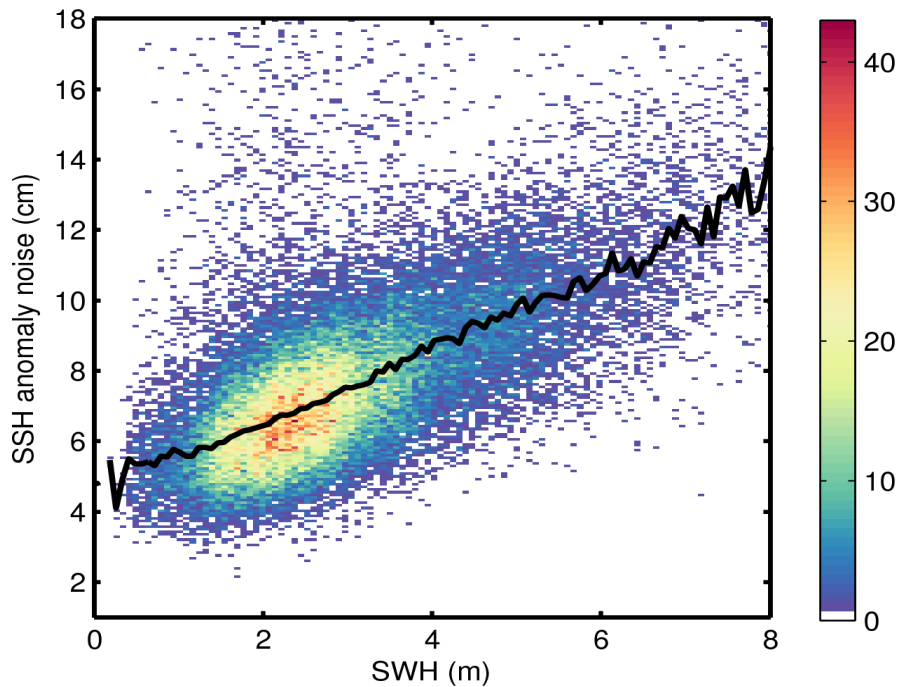
Figure 9. 2D histogram showing flag-valid SSH anomaly noise as a function of SWH for 03/11/2015. The black line denotes the median SSH anomaly noise as a function of SWH.
