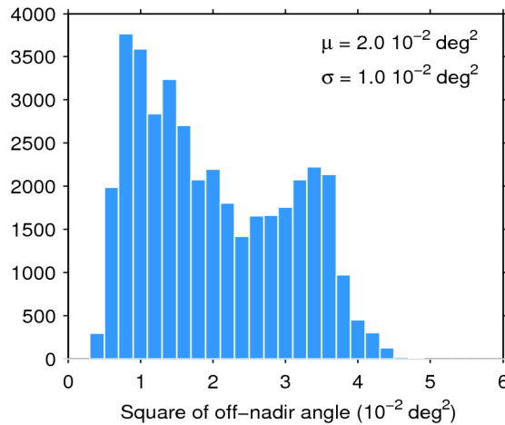
Figure 39. Histogram of flag-valid mispointing over oceans and lakes for 03/11/2015. The mean ( \mu ) and standard deviation ( \sigma ) are also shown. Note that values larger than 6 \cdot 10^{-2} \text{ deg}^2 are excluded from the histogram for the sake of readability but not from the computation of \mu and \sigma .
