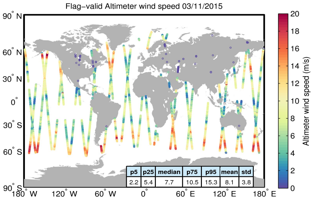
Figure 31. Geographical distribution of flag-valid wind data over oceans and lakes for 03/11/2015. The statistical values shown in the table refer to the wind in m/s and are calculated over all measurements shown in the figure.
