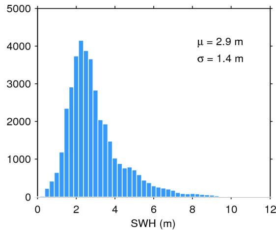
Figure 17. Histogram of flag-valid SWH over oceans and lakes for 03/11/2015. The mean ( \mu ) and standard deviation ( \sigma ) are also shown. Note that values larger than 12 m are excluded from the histogram for the sake of readability but not from the computation of \mu and \sigma .
