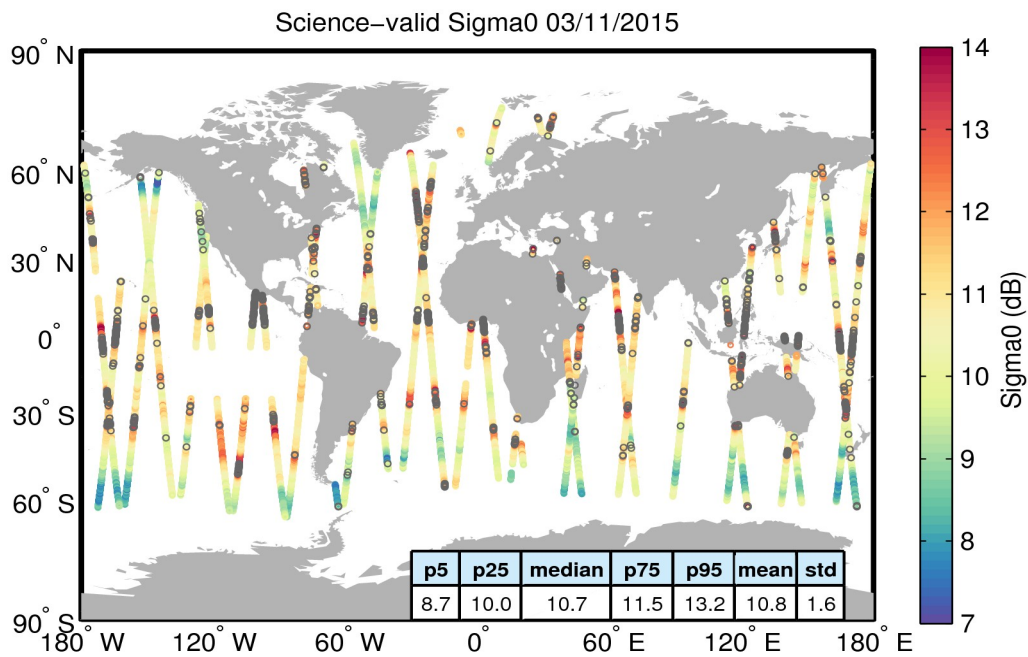
Figure 27. Geographical distribution of science-valid sigma0 data over oceans and lakes for 03/11/2015. The statistical values shown in the table refer to the sigma0 in dB and are calculated over all measurements shown in the figure. Gray circles denote records that have been rejected based on the editing criteria described in Table 4.
