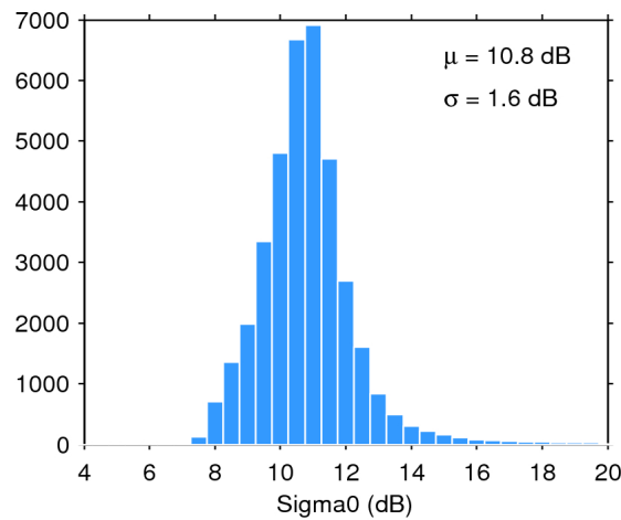
Figure 28. Histogram of science-valid sigma0 over oceans and lakes for 03/11/2015. The mean ( \mu ) and standard deviation ( \sigma ) are also shown. Note that values outside [4 20] dB are excluded from the histogram for the sake of readability but not from the computation of \mu and \sigma .
