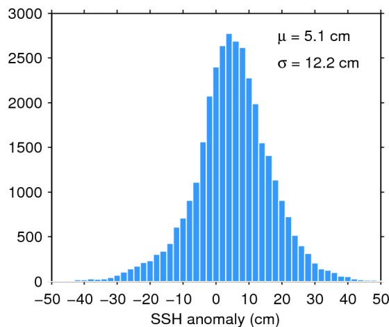
Figure 11. Histogram of science-valid SSH anomaly over oceans and lakes for 03/11/2015. The mean ( \mu ) and standard deviation ( \sigma ) are also shown. Note that values outside [-50 50] cm are excluded from the histogram for the sake of readability but not from the computation of \mu and \sigma .
