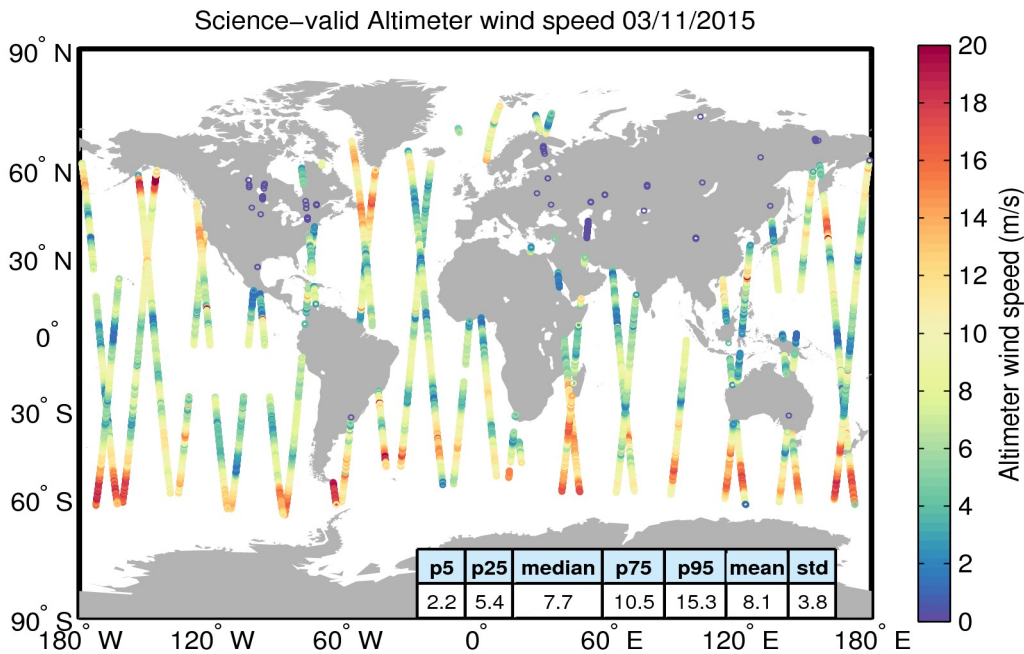
Figure 34. Geographical distribution of science-valid wind data over oceans and lakes for 03/11/2015. The statistical values shown in the table refer to the wind in m/s and are calculated over all measurements shown in the figure. Gray circles denote records that have been rejected based on the editing criteria described in Table 5.
