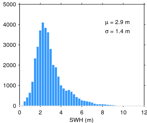
Figure 20. Histogram of science-valid SWH over oceans and lakes for 03/11/2015. The mean ( \mu ) and standard deviation ( \sigma ) are also shown. Note that values larger than 12 m are excluded from the histogram for the sake of readability but not from the computation of \mu and \sigma .
