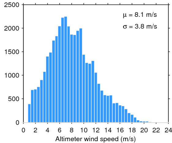
Figure 33. Histogram of flag-valid wind over oceans and lakes for 03/11/2015. The mean ( \mu ) and standard deviation ( \sigma ) are also shown. Note that values larger than 24 m/s are excluded from the histogram for the sake of readability but not from the computation of \mu and \sigma .
