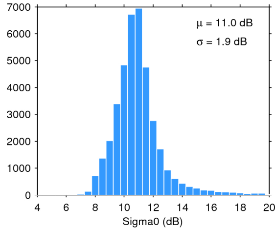
Figure 25. Histogram of flag-valid sigma0 over oceans and lakes for 03/11/2015. The mean ( \mu ) and standard deviation ( \sigma ) are also shown. Note that values outside [4 20] dB are excluded from the histogram for the sake of readability but not from the computation of \mu and \sigma .
