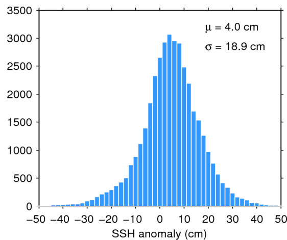
Figure 7. Histogram of flag-valid SSH anomaly over oceans and lakes for 03/11/2015. The mean ( \mu ) and standard deviation ( \sigma ) are also shown. Note that values outside [-50 \ 50] cm are excluded from the histogram for the sake of readability but not from the computation of \mu and \sigma .
