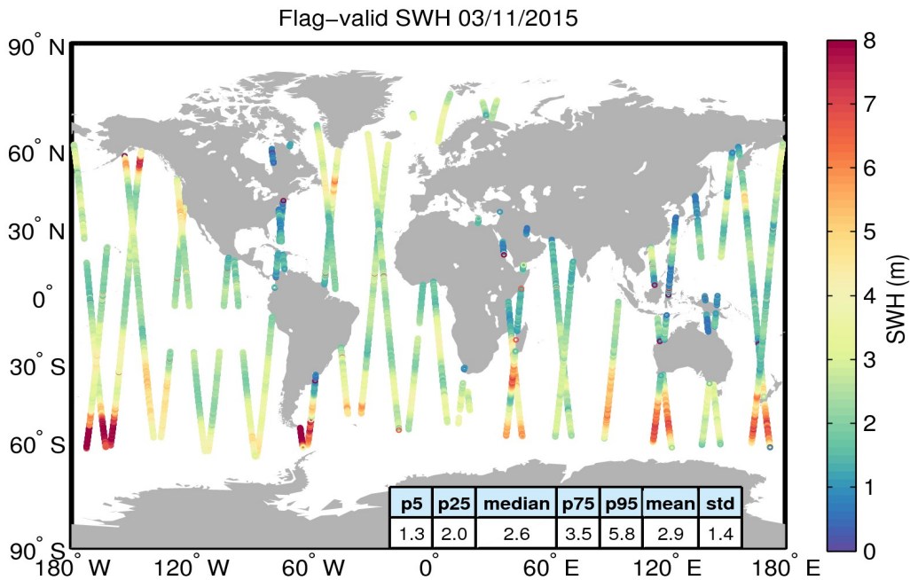
Figure 15. Geographical distribution of flag-valid SWH data over oceans and lakes for 03/11/2015. The statistical values shown in the table refer to the SWH in m and are calculated over all measurements shown in the figure.
