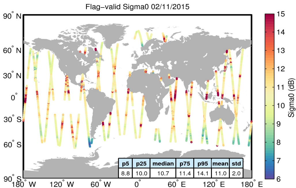
Figure 23. Geographical distribution of flag-valid sigma0 data over oceans and lakes for 02/11/2015. The statistical values shown in the table refer to the sigma0 in dB and are calculated over all measurements shown in the figure.
