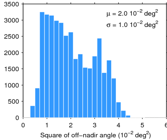
Figure 39. Histogram of flag-valid mispointing over oceans and lakes for 02/11/2015. The mean ( \mu ) and standard deviation ( \sigma ) are also shown. Note that values larger than 6 \cdot 10^{-2} \text{ deg}^2 are excluded from the histogram for the sake of readability but not from the computation of \mu and \sigma .
