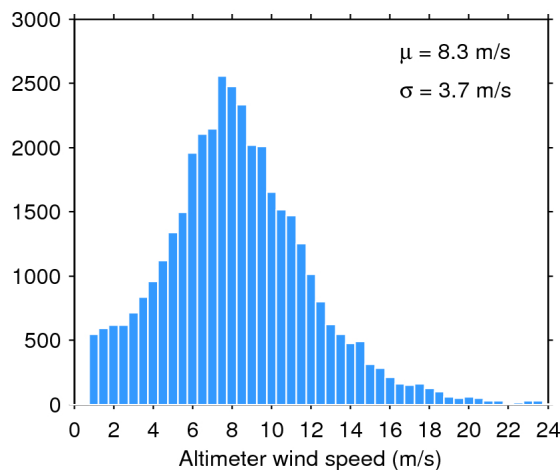
Figure 35. Histogram of science-valid wind over oceans and lakes for 02/11/2015. The mean ( \mu ) and standard deviation ( \sigma ) are also shown. Note that values larger than 24 m/s are excluded from the histogram for the sake of readability but not from the computation of \mu and \sigma .
