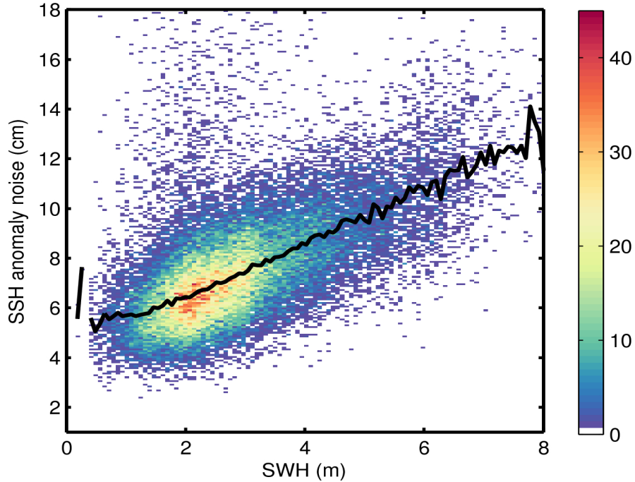
Figure 9. 2D histogram showing flag-valid SSH anomaly noise as a function of SWH for 02/11/2015. The black line denotes the median SSH anomaly noise as a function of SWH.
