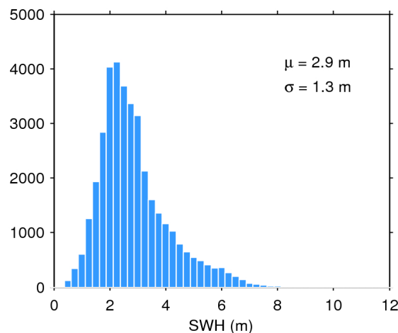
Figure 20. Histogram of science-valid SWH over oceans and lakes for 02/11/2015. The mean ( \mu ) and standard deviation ( \sigma ) are also shown. Note that values larger than 12 m are excluded from the histogram for the sake of readability but not from the computation of \mu and \sigma .
