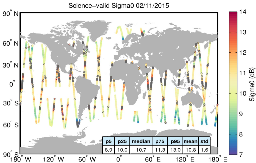
Figure 27. Geographical distribution of science-valid sigma0 data over oceans and lakes for 02/11/2015. The statistical values shown in the table refer to the sigma0 in dB and are calculated over all measurements shown in the figure. Gray circles denote records that have been rejected based on the editing criteria described in Table 4.
