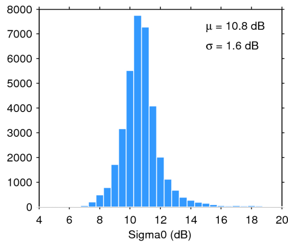
Figure 28. Histogram of science-valid sigma0 over oceans and lakes for 02/11/2015. The mean ( \mu ) and standard deviation ( \sigma ) are also shown. Note that values outside [4 20] dB are excluded from the histogram for the sake of readability but not from the computation of \mu and \sigma .
