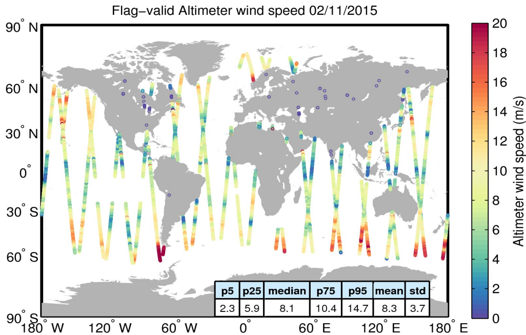
Figure 31. Geographical distribution of flag-valid wind data over oceans and lakes for 02/11/2015. The statistical values shown in the table refer to the wind in m/s and are calculated over all measurements shown in the figure.
