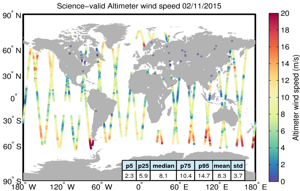
Figure 34. Geographical distribution of science-valid wind data over oceans and lakes for 02/11/2015. The statistical values shown in the table refer to the wind in m/s and are calculated over all measurements shown in the figure. Gray circles denote records that have been rejected based on the editing criteria described in Table 5.
