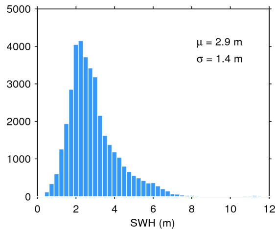
Figure 17. Histogram of flag-valid SWH over oceans and lakes for 02/11/2015. The mean ( \mu ) and standard deviation ( \sigma ) are also shown. Note that values larger than 12 m are excluded from the histogram for the sake of readability but not from the computation of \mu and \sigma .
