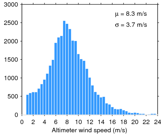
Figure 33. Histogram of flag-valid wind over oceans and lakes for 02/11/2015. The mean ( \mu ) and standard deviation ( \sigma ) are also shown. Note that values larger than 24 m/s are excluded from the histogram for the sake of readability but not from the computation of \mu and \sigma .
