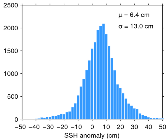
Figure 11. Histogram of science-valid SSH anomaly over oceans and lakes for 02/11/2015. The mean ( \mu ) and standard deviation ( \sigma ) are also shown. Note that values outside [-50 50] cm are excluded from the histogram for the sake of readability but not from the computation of \mu and \sigma .
