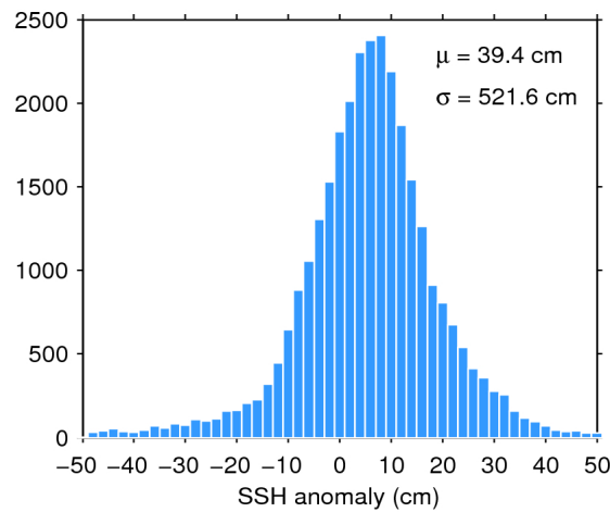
Figure 7. Histogram of flag-valid SSH anomaly over oceans and lakes for 02/11/2015. The mean ( \mu ) and standard deviation ( \sigma ) are also shown. Note that values outside [-50\ 50] cm are excluded from the histogram for the sake of readability but not from the computation of \mu and \sigma .
