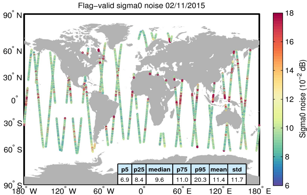
Figure 26. Geographical distribution of flag-valid 20-Hz sigma0 measurement noise over oceans and lakes for 02/11/2015. The statistical values shown in the table refer to the sigma0 noise and are calculated over all measurements shown in the figure.
