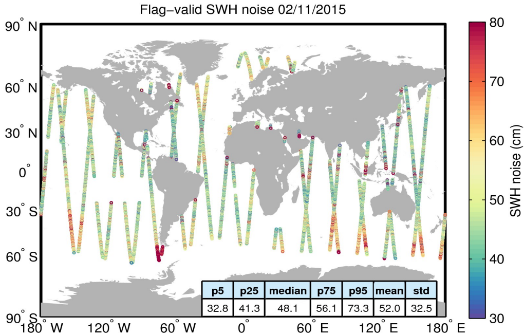
Figure 18. Geographical distribution of flag-valid 20-Hz SWH measurement noise over oceans and lakes for 02/11/2015. The statistical values shown in the figure refer to the SWH noise and are calculated over all measurements shown in the figure.
