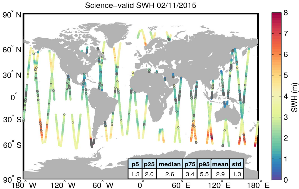
Figure 19. Geographical distribution of science-valid SWH data over oceans and lakes for 02/11/2015. The statistical values shown in the table refer to the SWH in m and are calculated over all measurements shown in the figure. Gray circles denote records that have been rejected based on the editing criteria described in Table 3.
