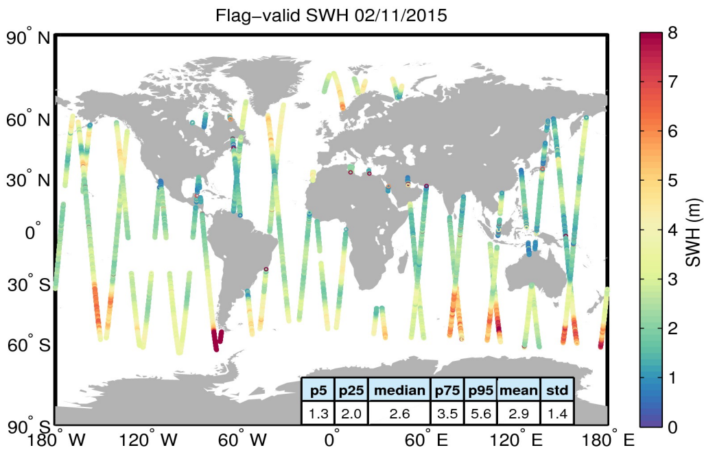
Figure 15. Geographical distribution of flag-valid SWH data over oceans and lakes for 02/11/2015. The statistical values shown in the table refer to the SWH in m and are calculated over all measurements shown in the figure.
