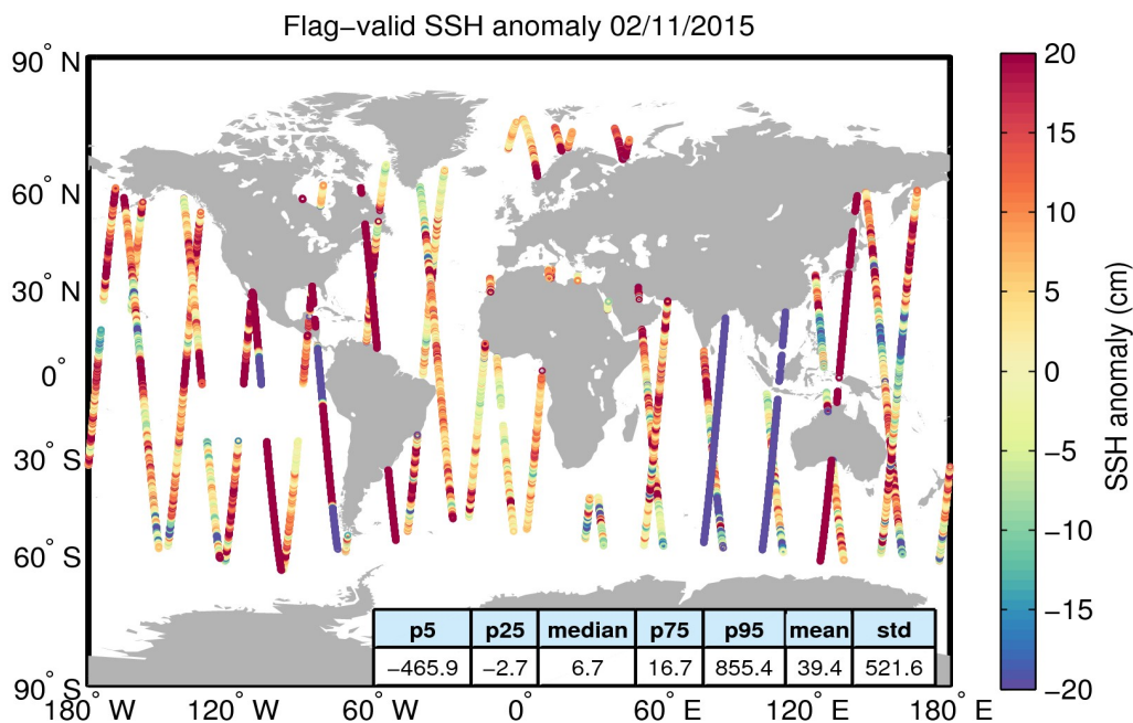
Figure 5. Geographical distribution of flag-valid 1-Hz SSH anomaly data over oceans and lakes for 02/11/2015. The statistical values shown in the table refer to the SSH anomaly in cm and are calculated over all measurements shown in the figure.
