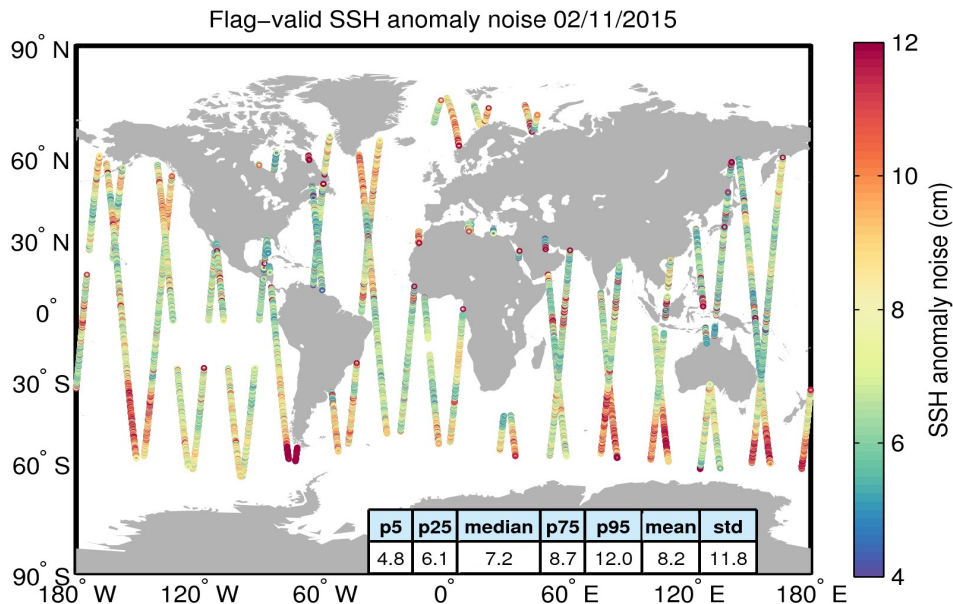
Figure 8. Geographical distribution of flag-valid 20-Hz SSH anomaly measurement noise over oceans and lakes for 02/11/2015. The statistical values shown in the table refer to the SSH anomaly noise and are calculated over all measurements shown in the figure.
