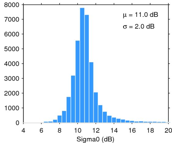
Figure 25. Histogram of flag-valid sigma0 over oceans and lakes for 02/11/2015. The mean ( \mu ) and standard deviation ( \sigma ) are also shown. Note that values outside [4 20] dB are excluded from the histogram for the sake of readability but not from the computation of \mu and \sigma .
