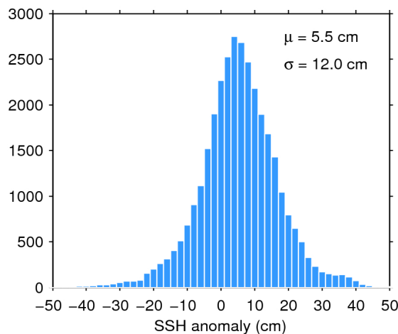
Figure 11. Histogram of science-valid SSH anomaly over oceans and lakes for 01/11/2015. The mean ( \mu ) and standard deviation ( \sigma ) are also shown. Note that values outside [-50 50] cm are excluded from the histogram for the sake of readability but not from the computation of \mu and \sigma .
