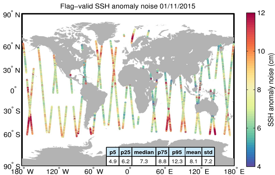
Figure 8. Geographical distribution of flag-valid 20-Hz SSH anomaly measurement noise over oceans and lakes for 01/11/2015. The statistical values shown in the table refer to the SSH anomaly noise and are calculated over all measurements shown in the figure.
