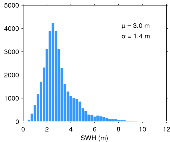
Figure 17. Histogram of flag-valid SWH over oceans and lakes for 01/11/2015. The mean ( \mu ) and standard deviation ( \sigma ) are also shown. Note that values larger than 12 m are excluded from the histogram for the sake of readability but not from the computation of \mu and \sigma .
