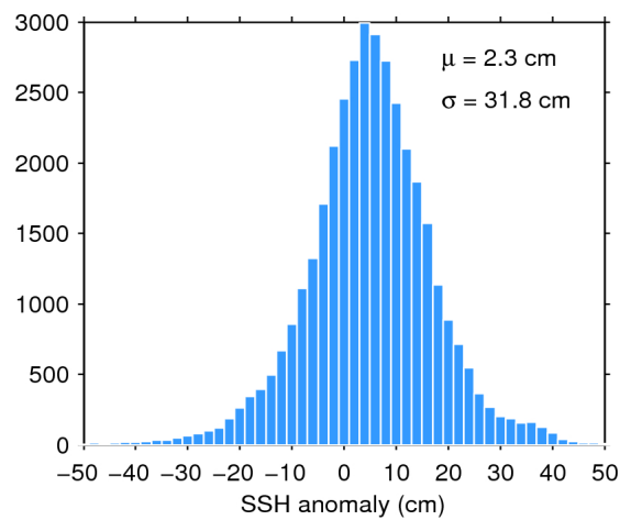
Figure 7. Histogram of flag-valid SSH anomaly over oceans and lakes for 01/11/2015. The mean ( \mu ) and standard deviation ( \sigma ) are also shown. Note that values outside [-50 50] cm are excluded from the histogram for the sake of readability but not from the computation of \mu and \sigma .
