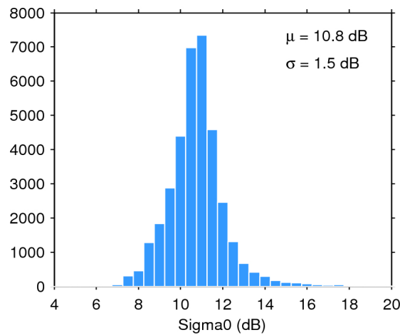
Figure 28. Histogram of science-valid sigma0 over oceans and lakes for 01/11/2015. The mean ( \mu ) and standard deviation ( \sigma ) are also shown. Note that values outside [4 20] dB are excluded from the histogram for the sake of readability but not from the computation of \mu and \sigma .
