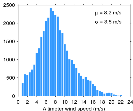
Figure 35. Histogram of science-valid wind over oceans and lakes for 01/11/2015. The mean ( \mu ) and standard deviation ( \sigma ) are also shown. Note that values larger than 24 m/s are excluded from the histogram for the sake of readability but not from the computation of \mu and \sigma .
