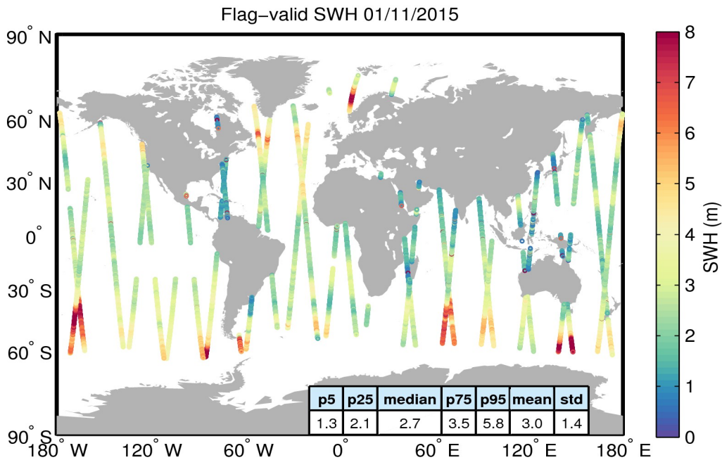
Figure 15. Geographical distribution of flag-valid SWH data over oceans and lakes for 01/11/2015. The statistical values shown in the table refer to the SWH in m and are calculated over all measurements shown in the figure.
