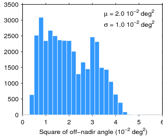
Figure 39. Histogram of flag-valid mispointing over oceans and lakes for 01/11/2015. The mean ( \mu ) and standard deviation ( \sigma ) are also shown. Note that values larger than 6 \cdot 10^{-2} \text{ deg}^2 are excluded from the histogram for the sake of readability but not from the computation of \mu and \sigma .
