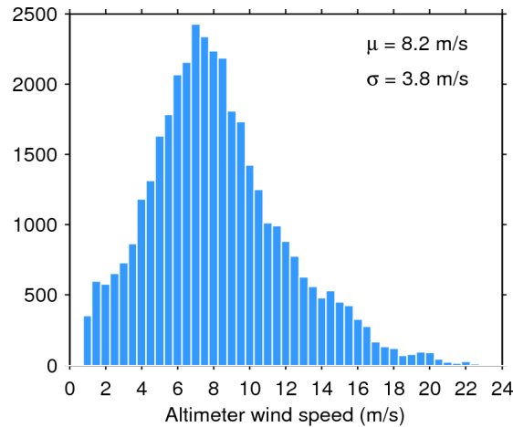
Figure 33. Histogram of flag-valid wind over oceans and lakes for 01/11/2015. The mean ( \mu ) and standard deviation ( \sigma ) are also shown. Note that values larger than 24 m/s are excluded from the histogram for the sake of readability but not from the computation of \mu and \sigma .
