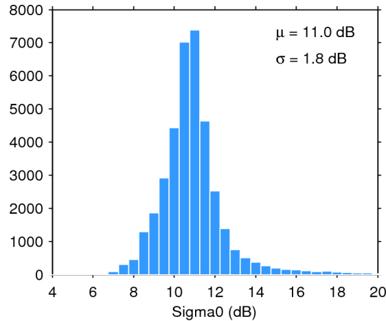
Figure 25. Histogram of flag-valid sigma0 over oceans and lakes for 01/11/2015. The mean ( \mu ) and standard deviation ( \sigma ) are also shown. Note that values outside [4 20] dB are excluded from the histogram for the sake of readability but not from the computation of \mu and \sigma .
