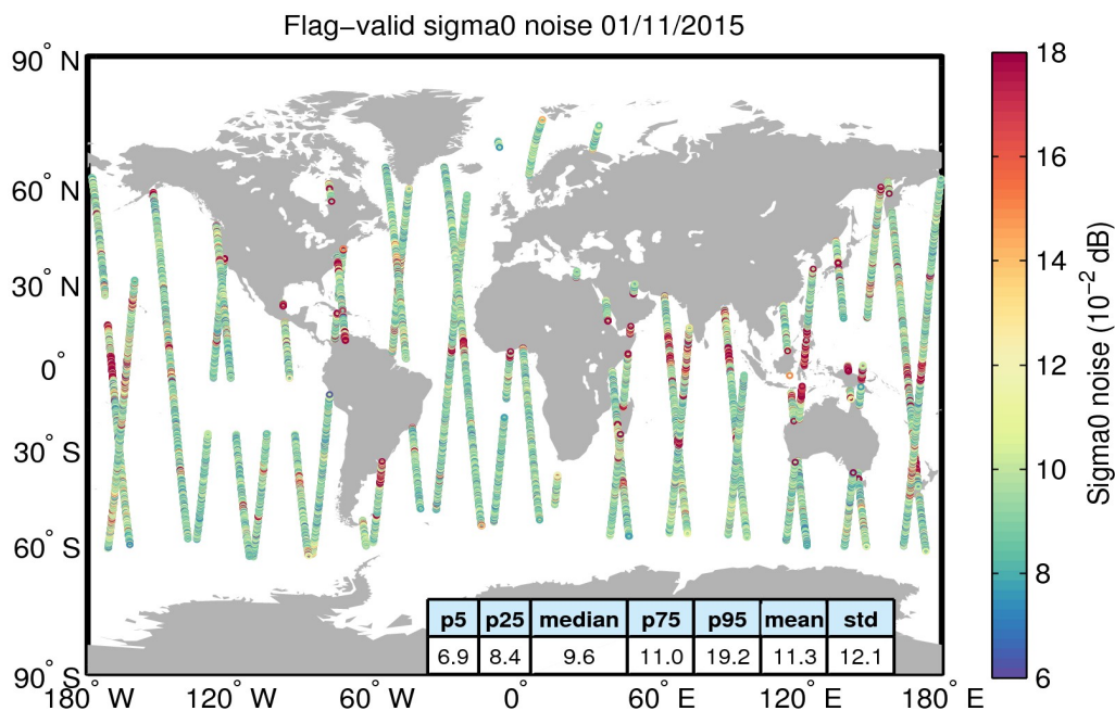
Figure 26. Geographical distribution of flag-valid 20-Hz sigma0 measurement noise over oceans and lakes for 01/11/2015. The statistical values shown in the table refer to the sigma0 noise and are calculated over all measurements shown in the figure.
