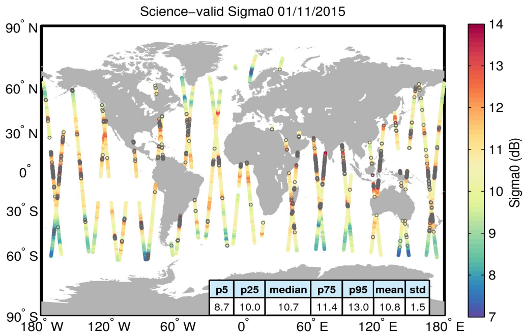
Figure 27. Geographical distribution of science-valid sigma0 data over oceans and lakes for 01/11/2015. The statistical values shown in the table refer to the sigma0 in dB and are calculated over all measurements shown in the figure. Gray circles denote records that have been rejected based on the editing criteria described in Table 4.
