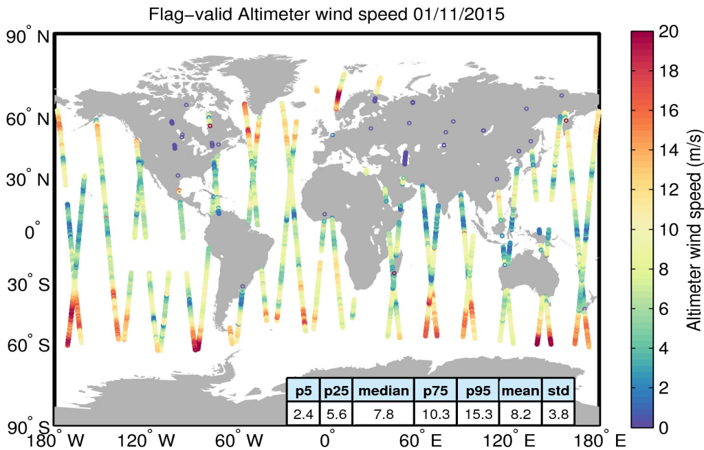
Figure 31. Geographical distribution of flag-valid wind data over oceans and lakes for 01/11/2015. The statistical values shown in the table refer to the wind in m/s and are calculated over all measurements shown in the figure.
