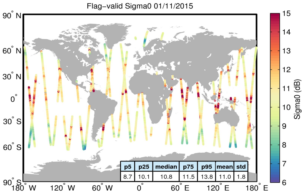
Figure 23. Geographical distribution of flag-valid sigma0 data over oceans and lakes for 01/11/2015. The statistical values shown in the table refer to the sigma0 in dB and are calculated over all measurements shown in the figure.
