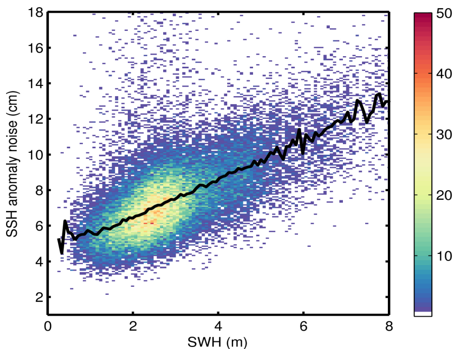
Figure 9. 2D histogram showing flag-valid SSH anomaly noise as a function of SWH for 01/11/2015. The black line denotes the median SSH anomaly noise as a function of SWH.
