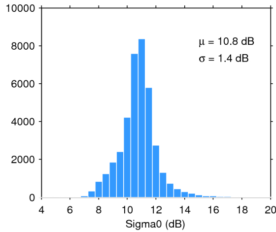
Figure 28. Histogram of science-valid sigma0 over oceans and lakes for 31/10/2015. The mean ( \mu ) and standard deviation ( \sigma ) are also shown. Note that values outside [4 20] dB are excluded from the histogram for the sake of readability but not from the computation of \mu and \sigma .
