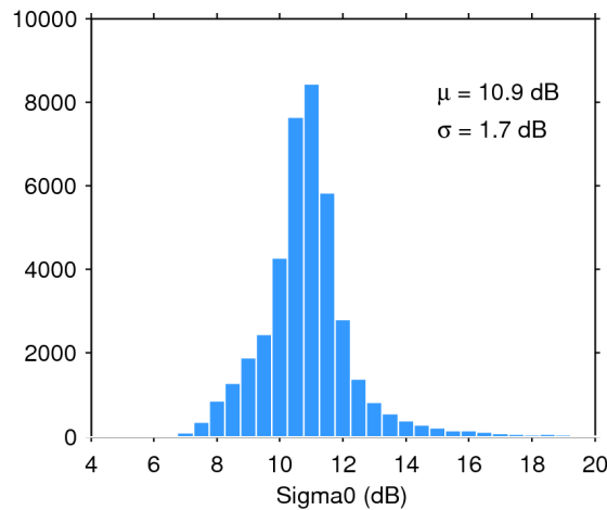
Figure 25. Histogram of flag-valid sigma0 over oceans and lakes for 31/10/2015. The mean ( \mu ) and standard deviation ( \sigma ) are also shown. Note that values outside [4 20] dB are excluded from the histogram for the sake of readability but not from the computation of \mu and \sigma .
