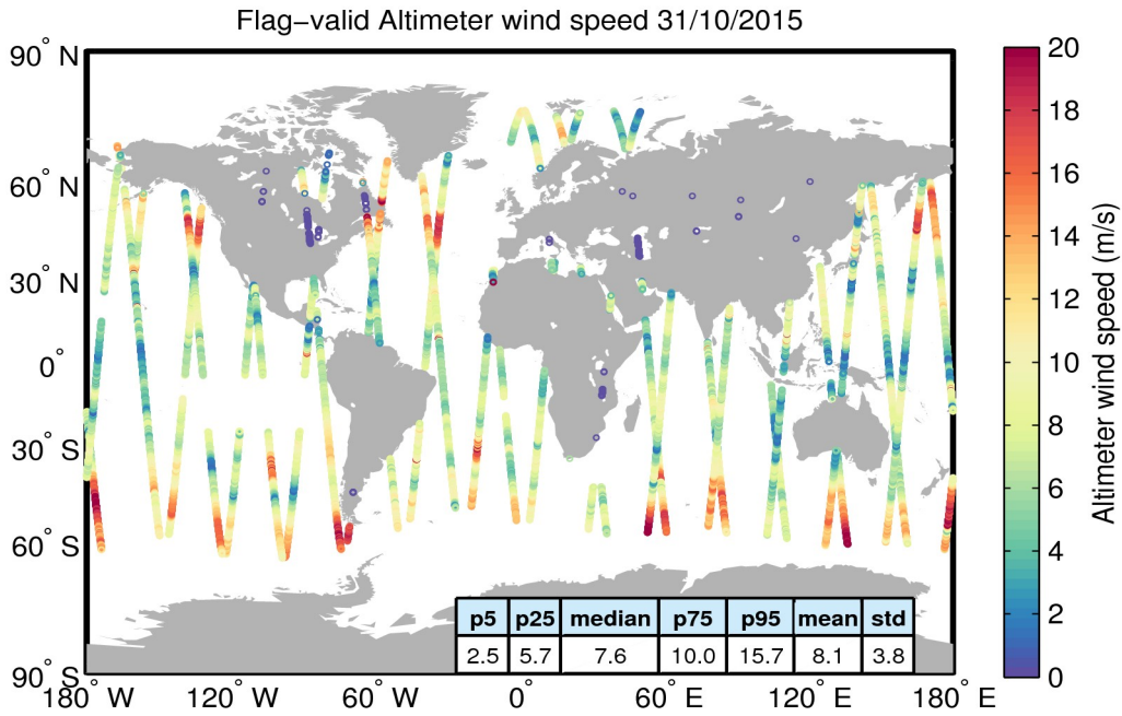
Figure 31. Geographical distribution of flag-valid wind data over oceans and lakes for 31/10/2015. The statistical values shown in the table refer to the wind in m/s and are calculated over all measurements shown in the figure.
