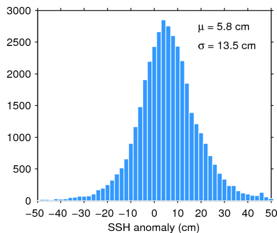
Figure 11. Histogram of science-valid SSH anomaly over oceans and lakes for 31/10/2015. The mean ( \mu ) and standard deviation ( \sigma ) are also shown. Note that values outside [-50 50] cm are excluded from the histogram for the sake of readability but not from the computation of \mu and \sigma .
