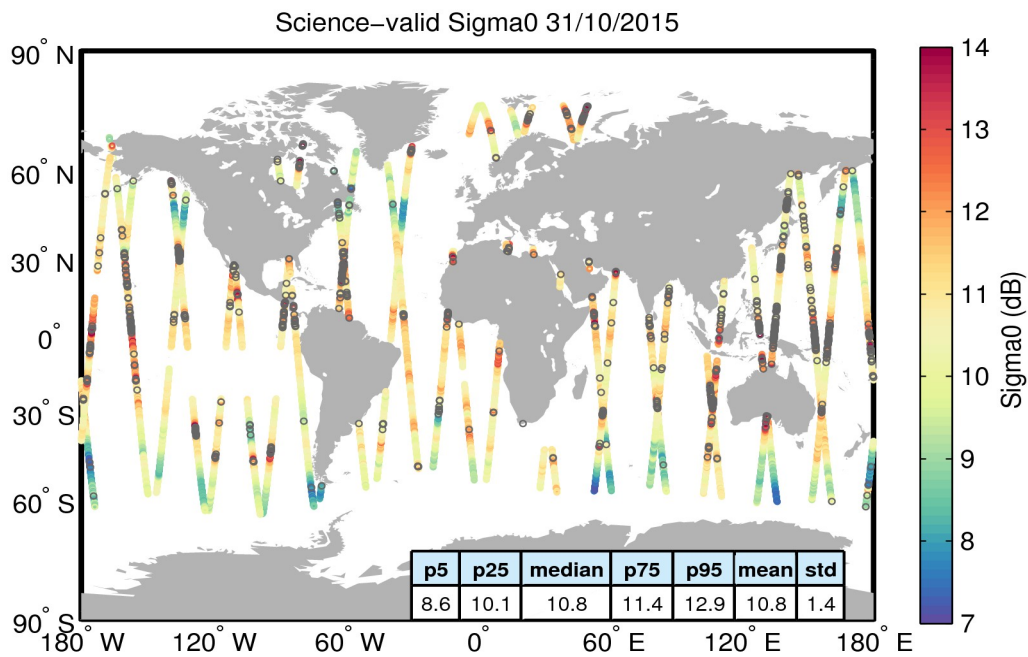
Figure 27. Geographical distribution of science-valid sigma0 data over oceans and lakes for 31/10/2015. The statistical values shown in the table refer to the sigma0 in dB and are calculated over all measurements shown in the figure. Gray circles denote records that have been rejected based on the editing criteria described in Table 4.
