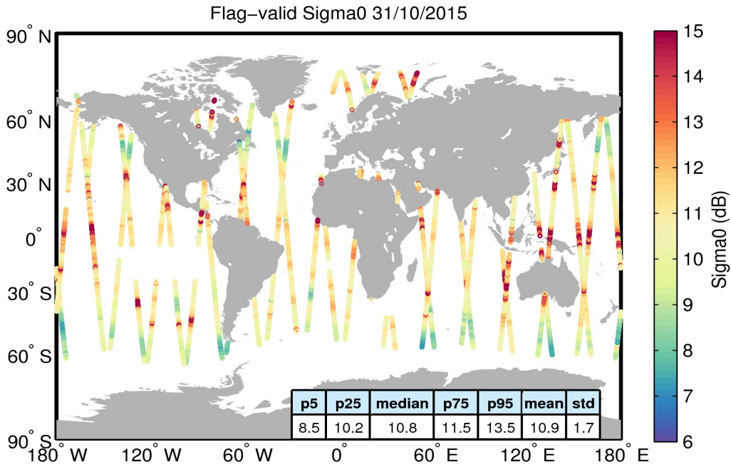
Figure 23. Geographical distribution of flag-valid sigma0 data over oceans and lakes for 31/10/2015. The statistical values shown in the table refer to the sigma0 in dB and are calculated over all measurements shown in the figure.
