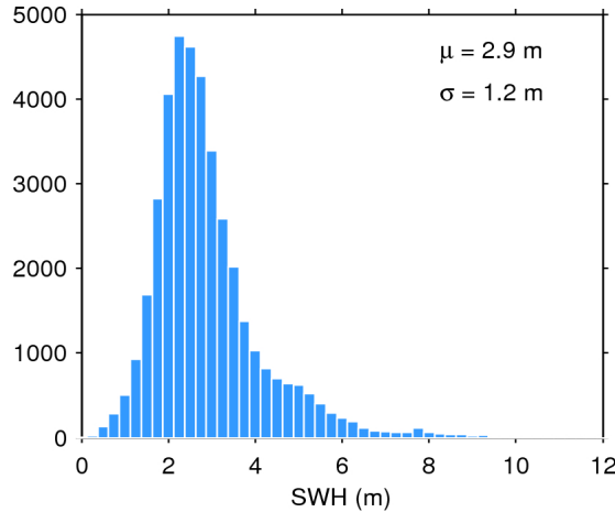
Figure 20. Histogram of science-valid SWH over oceans and lakes for 31/10/2015. The mean ( \mu ) and standard deviation ( \sigma ) are also shown. Note that values larger than 12 m are excluded from the histogram for the sake of readability but not from the computation of \mu and \sigma .
