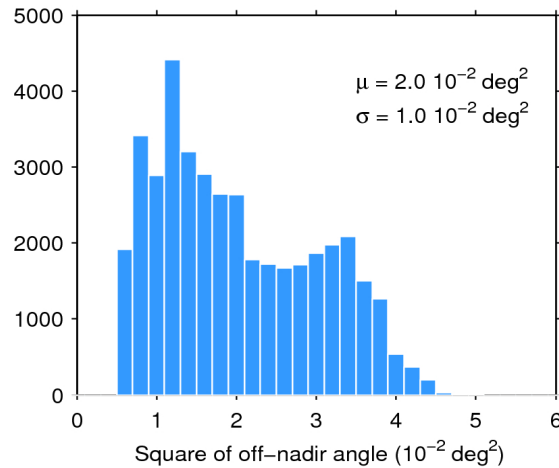
Figure 39. Histogram of flag-valid mispointing over oceans and lakes for 31/10/2015. The mean ( \mu ) and standard deviation ( \sigma ) are also shown. Note that values larger than 6 \cdot 10^{-2} \text{ deg}^2 are excluded from the histogram for the sake of readability but not from the computation of \mu and \sigma .
