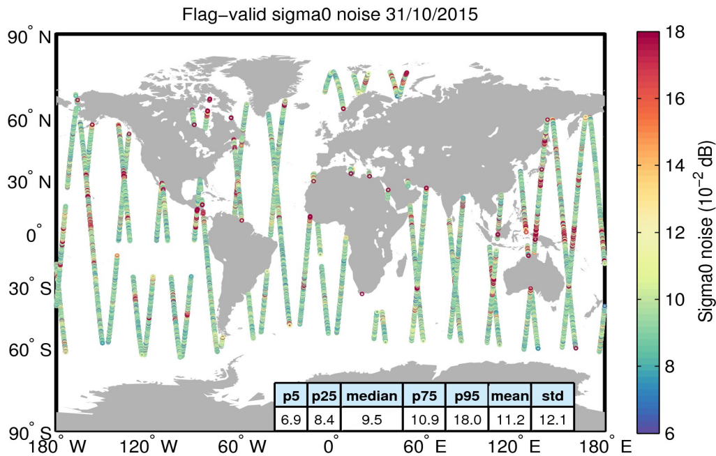
Figure 26. Geographical distribution of flag-valid 20-Hz sigma0 measurement noise over oceans and lakes for 31/10/2015. The statistical values shown in the table refer to the sigma0 noise and are calculated over all measurements shown in the figure.
