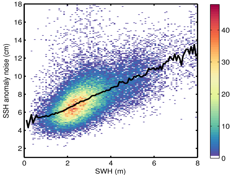
Figure 9. 2D histogram showing flag-valid SSH anomaly noise as a function of SWH for 31/10/2015. The black line denotes the median SSH anomaly noise as a function of SWH.
