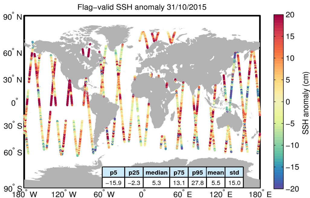
Figure 5. Geographical distribution of flag-valid 1-Hz SSH anomaly data over oceans and lakes for 31/10/2015. The statistical values shown in the table refer to the SSH anomaly in cm and are calculated over all measurements shown in the figure.
