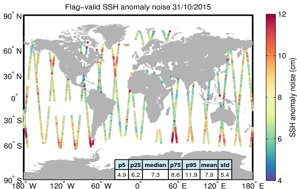
Figure 8. Geographical distribution of flag-valid 20-Hz SSH anomaly measurement noise over oceans and lakes for 31/10/2015. The statistical values shown in the table refer to the SSH anomaly noise and are calculated over all measurements shown in the figure.
