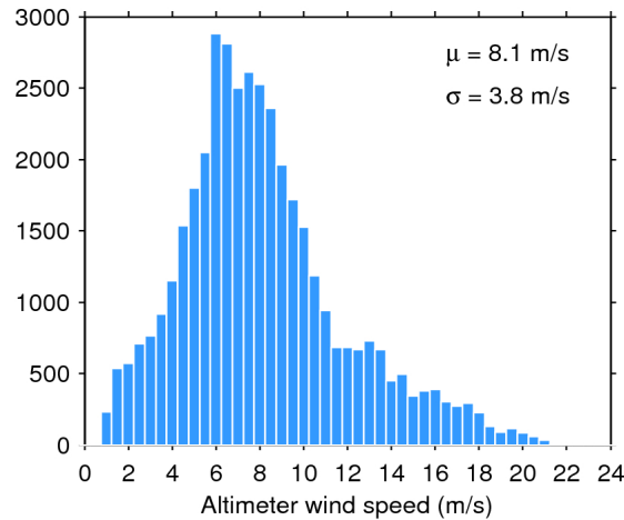
Figure 33. Histogram of flag-valid wind over oceans and lakes for 31/10/2015. The mean ( \mu ) and standard deviation ( \sigma ) are also shown. Note that values larger than 24 m/s are excluded from the histogram for the sake of readability but not from the computation of \mu and \sigma .
