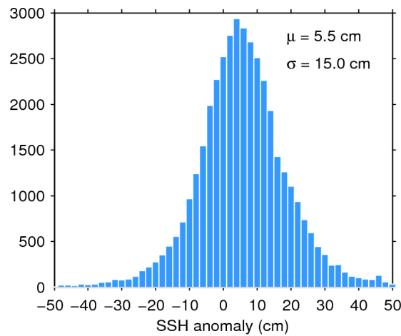
Figure 7. Histogram of flag-valid SSH anomaly over oceans and lakes for 31/10/2015. The mean ( \mu ) and standard deviation ( \sigma ) are also shown. Note that values outside [-50\ 50] cm are excluded from the histogram for the sake of readability but not from the computation of \mu and \sigma .
