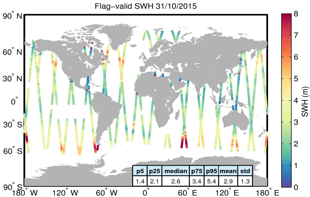
Figure 15. Geographical distribution of flag-valid SWH data over oceans and lakes for 31/10/2015. The statistical values shown in the table refer to the SWH in m and are calculated over all measurements shown in the figure.
