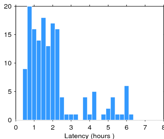
Figure 2. Histogram of the data latency for 31/10/2015. The y-axis denotes the number of files that are made available with a delay of x-hours with respect to the mean time of the records stored in the file.
