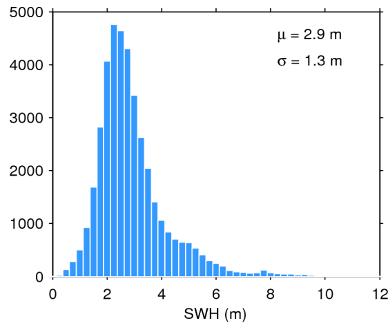
Figure 17. Histogram of flag-valid SWH over oceans and lakes for 31/10/2015. The mean ( \mu ) and standard deviation ( \sigma ) are also shown. Note that values larger than 12 m are excluded from the histogram for the sake of readability but not from the computation of \mu and \sigma .
