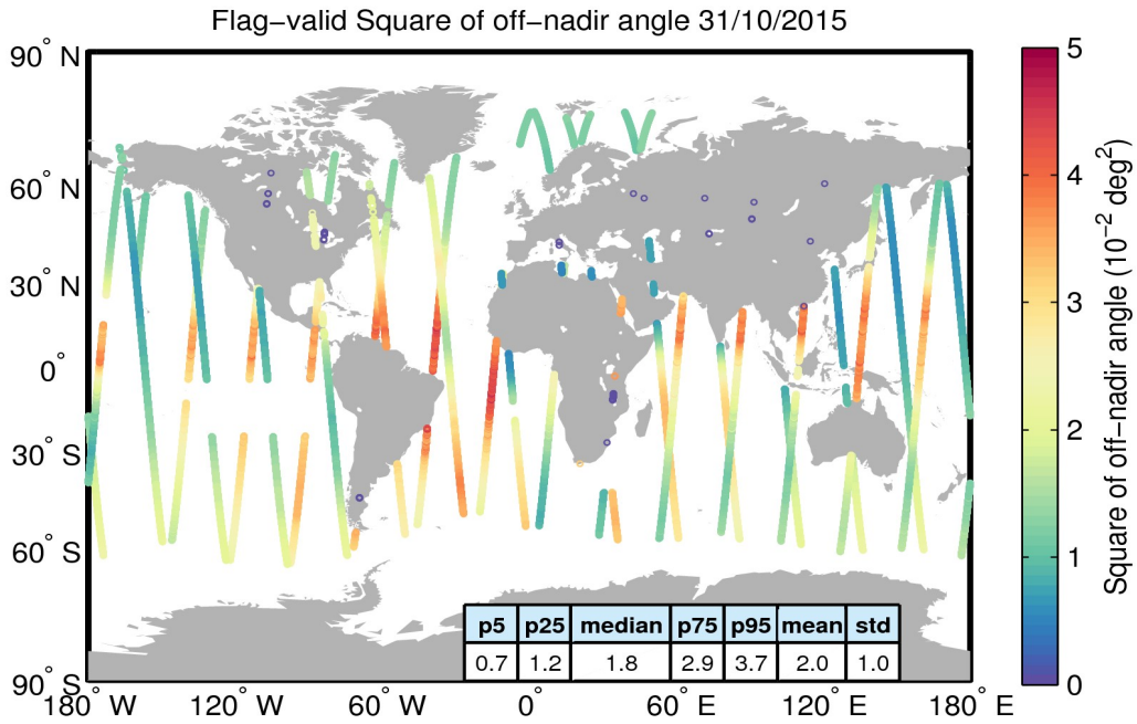
Figure 37. Geographical distribution of flag-valid mispointing data over oceans and lakes for 31/10/2015. The statistical values shown in the table refer to the mispointing in 10^{-2} deg 2 and are calculated over all measurements shown in the figure.
