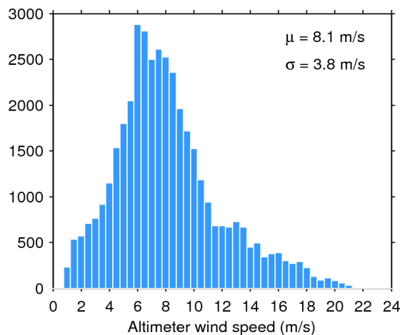
Figure 35. Histogram of science-valid wind over oceans and lakes for 31/10/2015. The mean ( \mu ) and standard deviation ( \sigma ) are also shown. Note that values larger than 24 m/s are excluded from the histogram for the sake of readability but not from the computation of \mu and \sigma .
