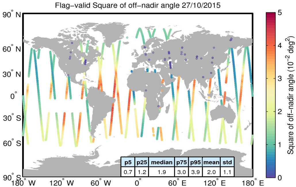
Figure 37. Geographical distribution of flag-valid mispointing data over oceans and lakes for 27/10/2015. The statistical values shown in the table refer to the mispointing in 10^{-2} \text{ deg}^2 and are calculated over all measurements shown in the figure.
