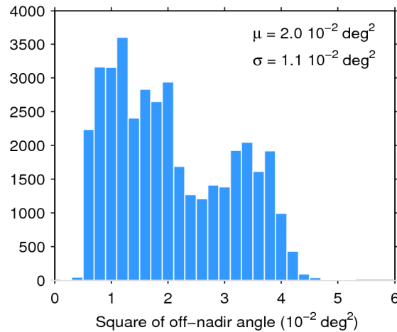
Figure 39. Histogram of flag-valid mispointing over oceans and lakes for 27/10/2015. The mean ( \mu ) and standard deviation ( \sigma ) are also shown. Note that values larger than 6 \cdot 10^{-2} \text{ deg}^2 are excluded from the histogram for the sake of readability but not from the computation of \mu and \sigma .
