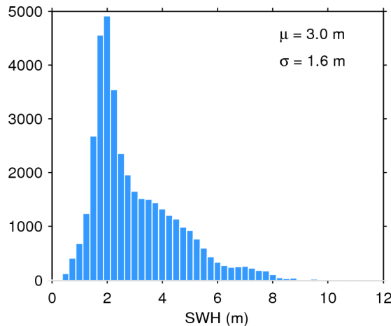
Figure 20. Histogram of science-valid SWH over oceans and lakes for 27/10/2015. The mean ( \mu ) and standard deviation ( \sigma ) are also shown. Note that values larger than 12 m are excluded from the histogram for the sake of readability but not from the computation of \mu and \sigma .
