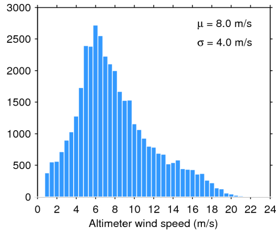
Figure 33. Histogram of flag-valid wind over oceans and lakes for 27/10/2015. The mean ( \mu ) and standard deviation ( \sigma ) are also shown. Note that values larger than 24 m/s are excluded from the histogram for the sake of readability but not from the computation of \mu and \sigma .
