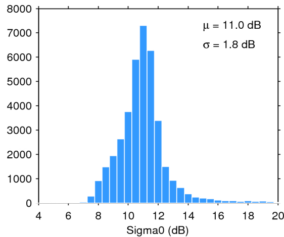
Figure 25. Histogram of flag-valid sigma0 over oceans and lakes for 27/10/2015. The mean ( \mu ) and standard deviation ( \sigma ) are also shown. Note that values outside [4 20] dB are excluded from the histogram for the sake of readability but not from the computation of \mu and \sigma .
