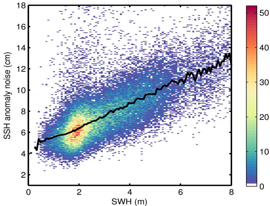
Figure 9. 2D histogram showing flag-valid SSH anomaly noise as a function of SWH for 27/10/2015. The black line denotes the median SSH anomaly noise as a function of SWH.
