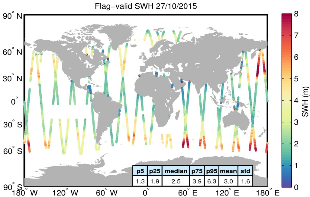
Figure 15. Geographical distribution of flag-valid SWH data over oceans and lakes for 27/10/2015. The statistical values shown in the table refer to the SWH in m and are calculated over all measurements shown in the figure.
