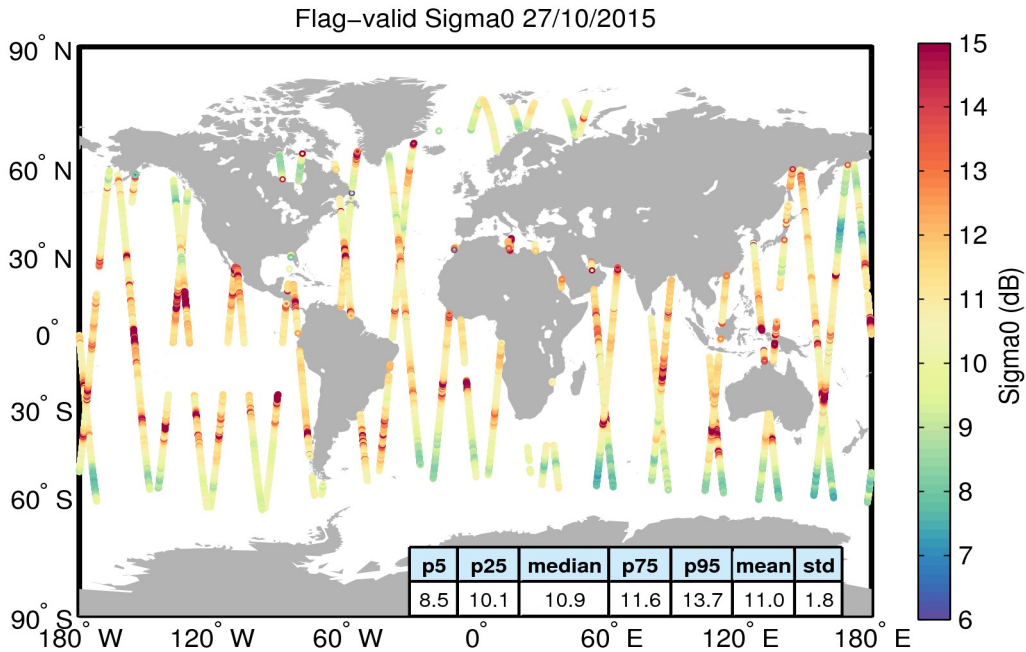
Figure 23. Geographical distribution of flag-valid sigma0 data over oceans and lakes for 27/10/2015. The statistical values shown in the table refer to the sigma0 in dB and are calculated over all measurements shown in the figure.
