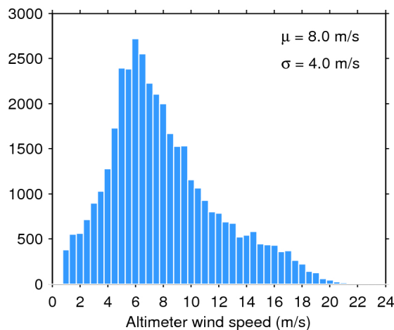
Figure 35. Histogram of science-valid wind over oceans and lakes for 27/10/2015. The mean ( \mu ) and standard deviation ( \sigma ) are also shown. Note that values larger than 24 m/s are excluded from the histogram for the sake of readability but not from the computation of \mu and \sigma .
