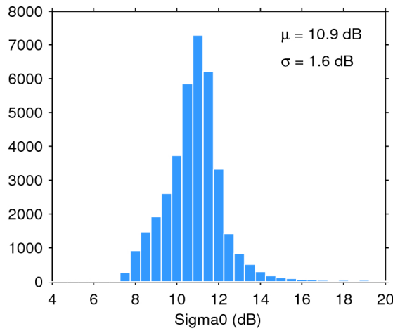
Figure 28. Histogram of science-valid sigma0 over oceans and lakes for 27/10/2015. The mean ( \mu ) and standard deviation ( \sigma ) are also shown. Note that values outside [4 20] dB are excluded from the histogram for the sake of readability but not from the computation of \mu and \sigma .
