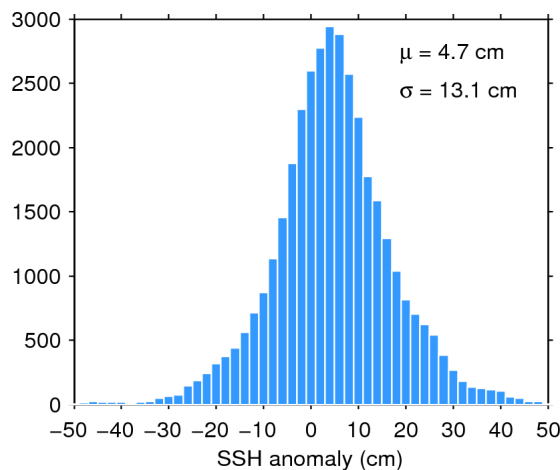
Figure 11. Histogram of science-valid SSH anomaly over oceans and lakes for 27/10/2015. The mean ( \mu ) and standard deviation ( \sigma ) are also shown. Note that values outside [-50 50] cm are excluded from the histogram for the sake of readability but not from the computation of \mu and \sigma .
