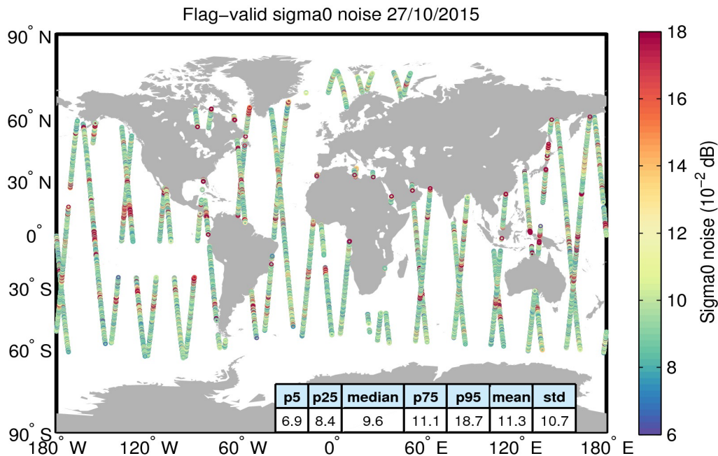
Figure 26. Geographical distribution of flag-valid 20-Hz sigma0 measurement noise over oceans and lakes for 27/10/2015. The statistical values shown in the table refer to the sigma0 noise and are calculated over all measurements shown in the figure.
