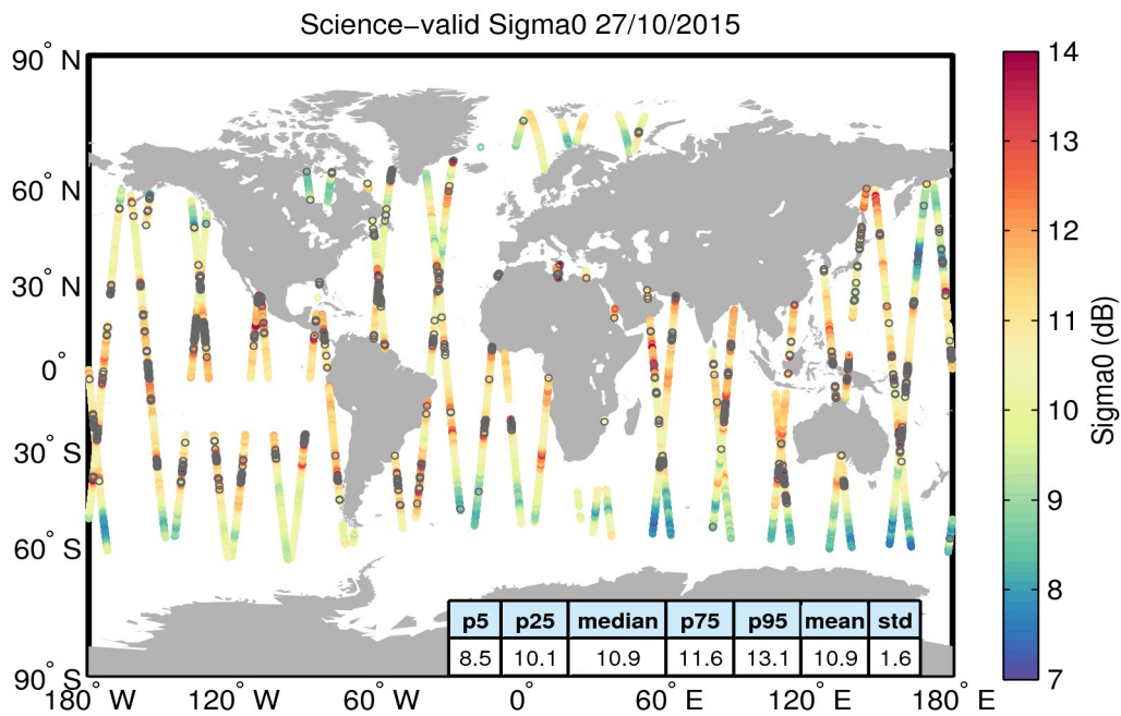
Figure 27. Geographical distribution of science-valid sigma0 data over oceans and lakes for 27/10/2015. The statistical values shown in the table refer to the sigma0 in dB and are calculated over all measurements shown in the figure. Gray circles denote records that have been rejected based on the editing criteria described in Table 4.
