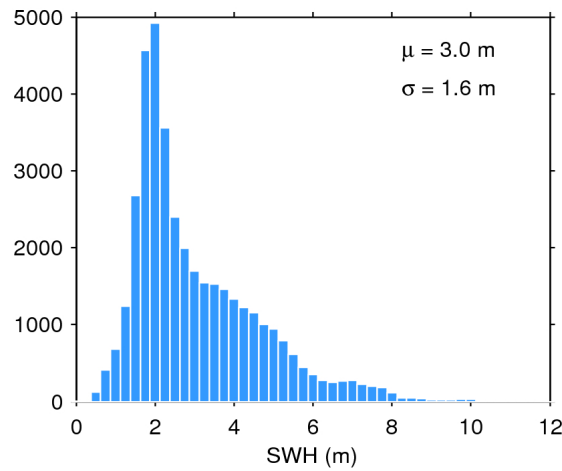
Figure 17. Histogram of flag-valid SWH over oceans and lakes for 27/10/2015. The mean ( \mu ) and standard deviation ( \sigma ) are also shown. Note that values larger than 12 m are excluded from the histogram for the sake of readability but not from the computation of \mu and \sigma .
