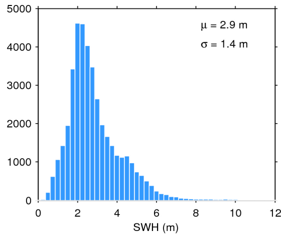
Figure 17. Histogram of flag-valid SWH over oceans and lakes for 24/10/2015. The mean ( \mu ) and standard deviation ( \sigma ) are also shown. Note that values larger than 12 m are excluded from the histogram for the sake of readability but not from the computation of \mu and \sigma .
