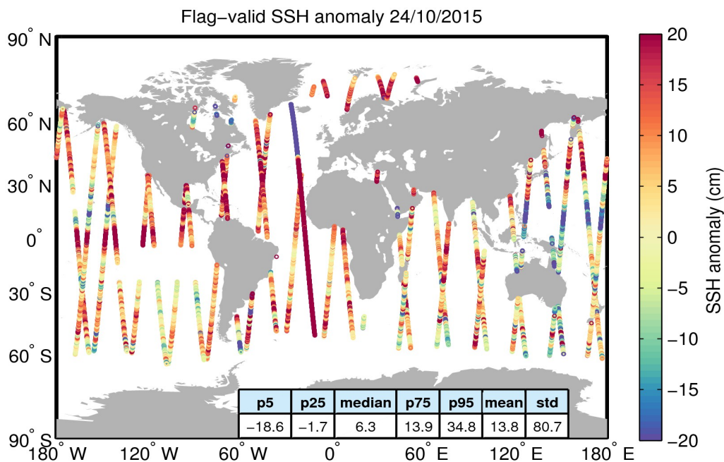
Figure 5. Geographical distribution of flag-valid 1-Hz SSH anomaly data over oceans and lakes for 24/10/2015. The statistical values shown in the table refer to the SSH anomaly in cm and are calculated over all measurements shown in the figure.
