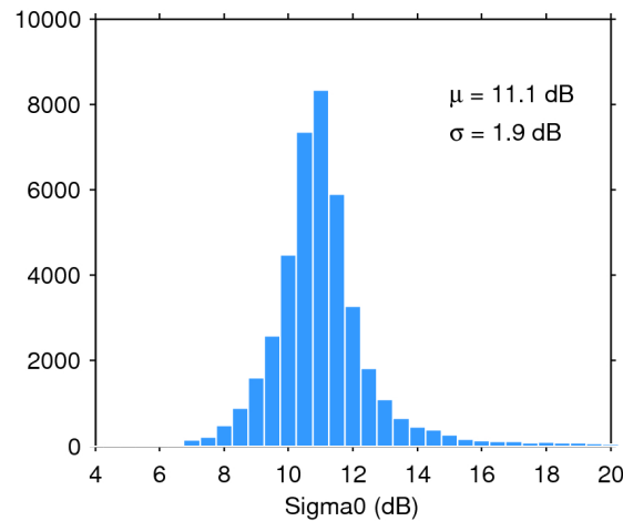
Figure 25. Histogram of flag-valid sigma0 over oceans and lakes for 24/10/2015. The mean ( \mu ) and standard deviation ( \sigma ) are also shown. Note that values outside [4 20] dB are excluded from the histogram for the sake of readability but not from the computation of \mu and \sigma .
