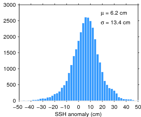
Figure 11. Histogram of science-valid SSH anomaly over oceans and lakes for 24/10/2015. The mean ( \mu ) and standard deviation ( \sigma ) are also shown. Note that values outside [-50 50] cm are excluded from the histogram for the sake of readability but not from the computation of \mu and \sigma .
