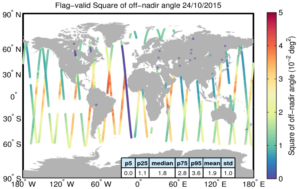
Figure 37. Geographical distribution of flag-valid mispointing data over oceans and lakes for 24/10/2015. The statistical values shown in the table refer to the mispointing in 10^{-2} deg 2 and are calculated over all measurements shown in the figure.
