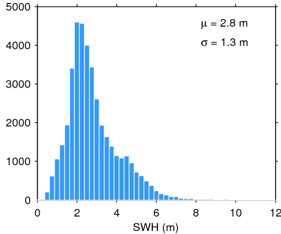
Figure 20. Histogram of science-valid SWH over oceans and lakes for 24/10/2015. The mean ( \mu ) and standard deviation ( \sigma ) are also shown. Note that values larger than 12 m are excluded from the histogram for the sake of readability but not from the computation of \mu and \sigma .
