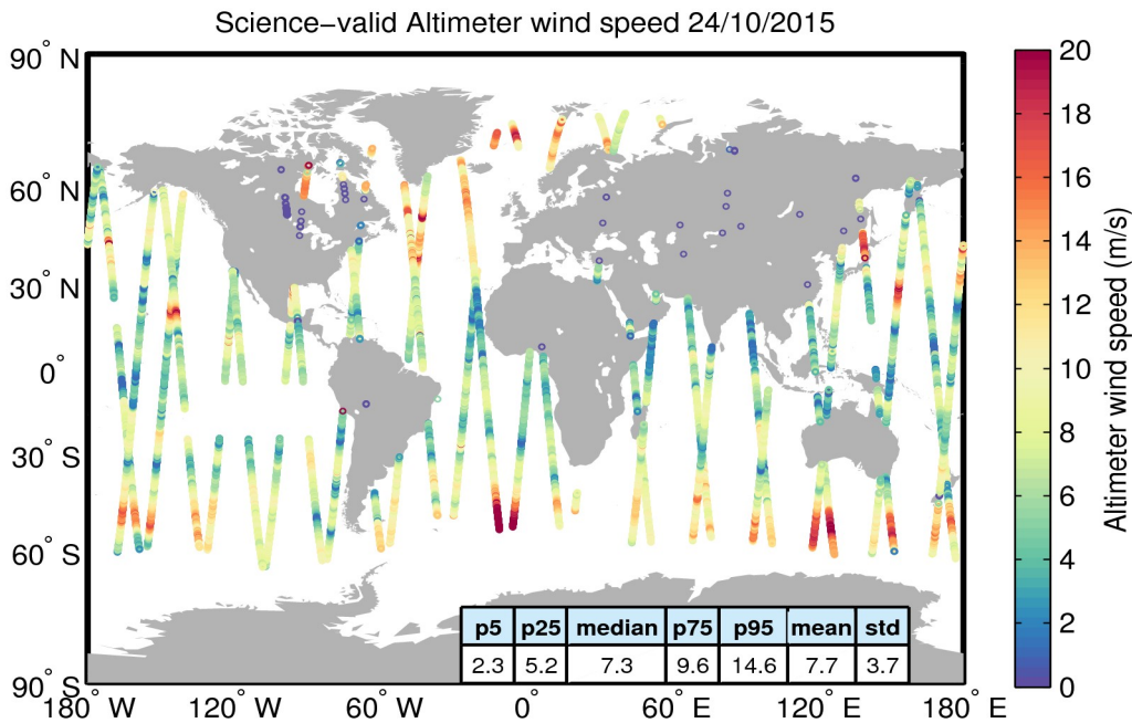
Figure 34. Geographical distribution of science-valid wind data over oceans and lakes for 24/10/2015. The statistical values shown in the table refer to the wind in m/s and are calculated over all measurements shown in the figure. Gray circles denote records that have been rejected based on the editing criteria described in Table 5.
