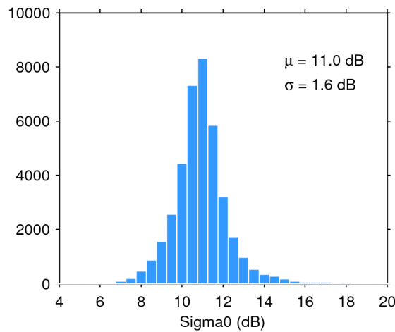
Figure 28. Histogram of science-valid sigma0 over oceans and lakes for 24/10/2015. The mean ( \mu ) and standard deviation ( \sigma ) are also shown. Note that values outside [4 20] dB are excluded from the histogram for the sake of readability but not from the computation of \mu and \sigma .
