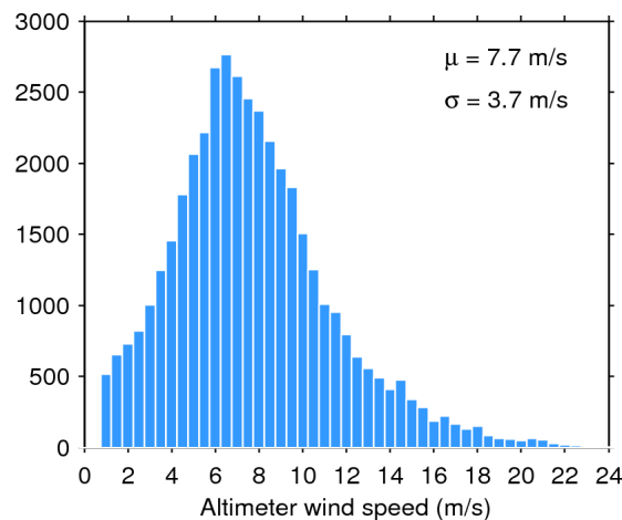
Figure 35. Histogram of science-valid wind over oceans and lakes for 24/10/2015. The mean ( \mu ) and standard deviation ( \sigma ) are also shown. Note that values larger than 24 m/s are excluded from the histogram for the sake of readability but not from the computation of \mu and \sigma .
