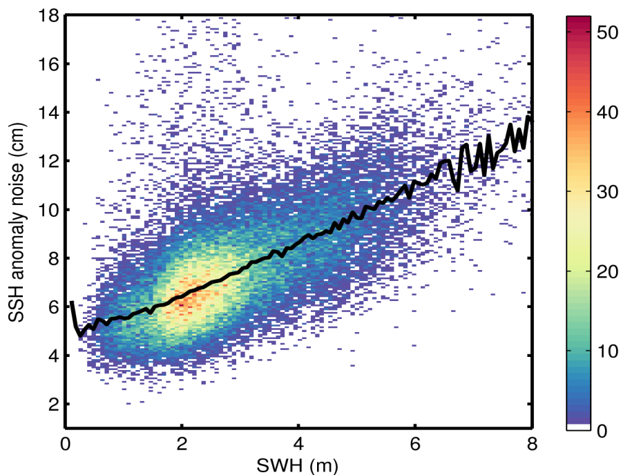
Figure 9. 2D histogram showing flag-valid SSH anomaly noise as a function of SWH for 24/10/2015. The black line denotes the median SSH anomaly noise as a function of SWH.
