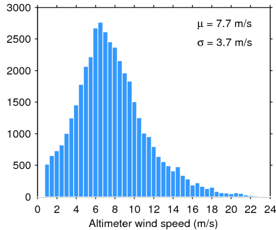
Figure 33. Histogram of flag-valid wind over oceans and lakes for 24/10/2015. The mean ( \mu ) and standard deviation ( \sigma ) are also shown. Note that values larger than 24 m/s are excluded from the histogram for the sake of readability but not from the computation of \mu and \sigma .
