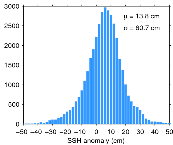
Figure 7. Histogram of flag-valid SSH anomaly over oceans and lakes for 24/10/2015. The mean ( \mu ) and standard deviation ( \sigma ) are also shown. Note that values outside [-50\ 50] cm are excluded from the histogram for the sake of readability but not from the computation of \mu and \sigma .
