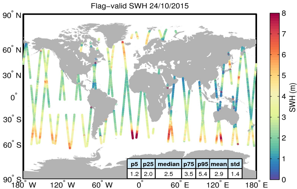
Figure 15. Geographical distribution of flag-valid SWH data over oceans and lakes for 24/10/2015. The statistical values shown in the table refer to the SWH in m and are calculated over all measurements shown in the figure.
