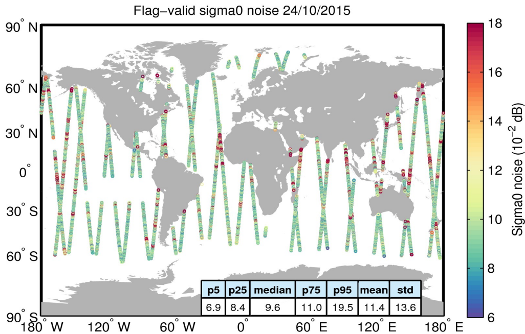
Figure 26. Geographical distribution of flag-valid 20-Hz sigma0 measurement noise over oceans and lakes for 24/10/2015. The statistical values shown in the table refer to the sigma0 noise and are calculated over all measurements shown in the figure.
