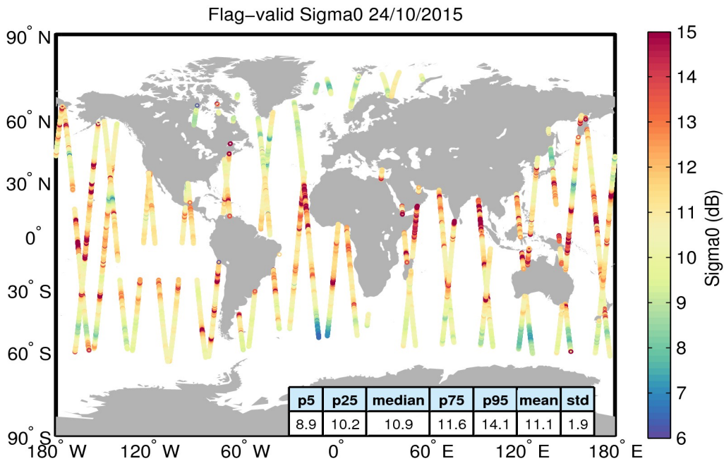
Figure 23. Geographical distribution of flag-valid sigma0 data over oceans and lakes for 24/10/2015. The statistical values shown in the table refer to the sigma0 in dB and are calculated over all measurements shown in the figure.
