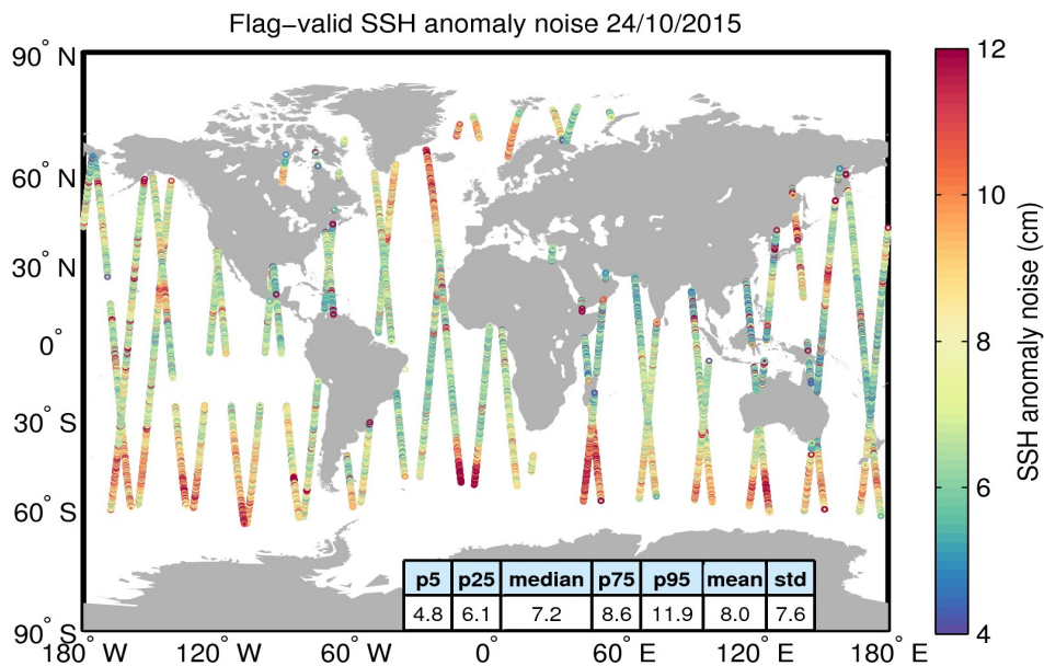
Figure 8. Geographical distribution of flag-valid 20-Hz SSH anomaly measurement noise over oceans and lakes for 24/10/2015. The statistical values shown in the table refer to the SSH anomaly noise and are calculated over all measurements shown in the figure.
