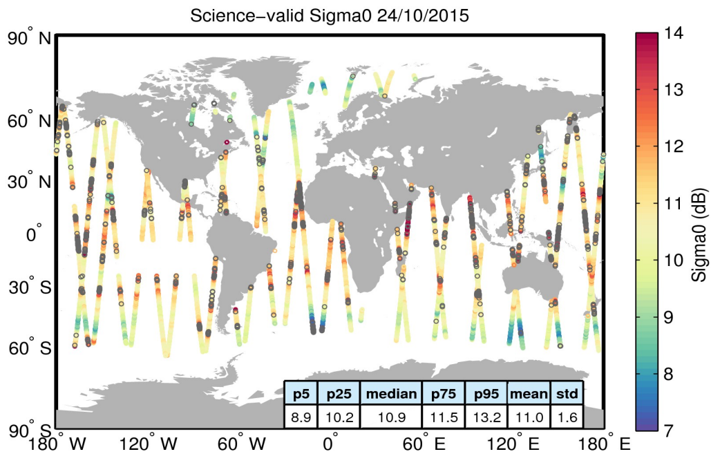
Figure 27. Geographical distribution of science-valid sigma0 data over oceans and lakes for 24/10/2015. The statistical values shown in the table refer to the sigma0 in dB and are calculated over all measurements shown in the figure. Gray circles denote records that have been rejected based on the editing criteria described in Table 4.
