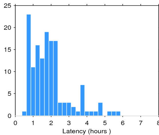
Figure 2. Histogram of the data latency for 24/10/2015. The y-axis denotes the number of files that are made available with a delay of x-hours with respect to the mean time of the records stored in the file.
