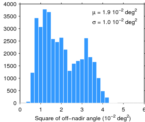
Figure 39. Histogram of flag-valid mispointing over oceans and lakes for 24/10/2015. The mean ( \mu ) and standard deviation ( \sigma ) are also shown. Note that values larger than 6 \cdot 10^{-2} \text{ deg}^2 are excluded from the histogram for the sake of readability but not from the computation of \mu and \sigma .
