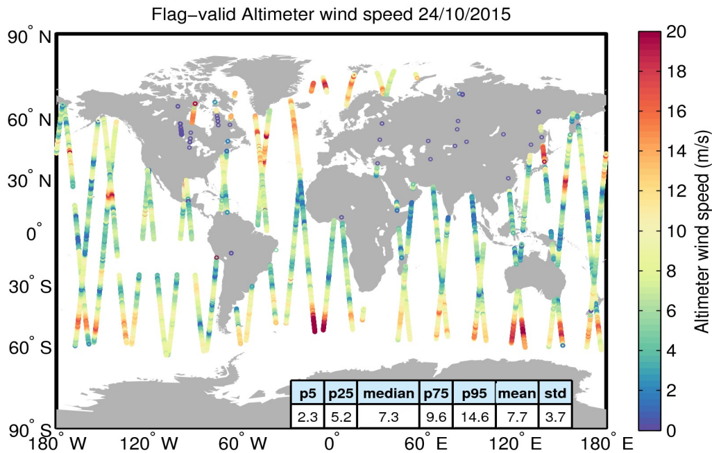
Figure 31. Geographical distribution of flag-valid wind data over oceans and lakes for 24/10/2015. The statistical values shown in the table refer to the wind in m/s and are calculated over all measurements shown in the figure.
