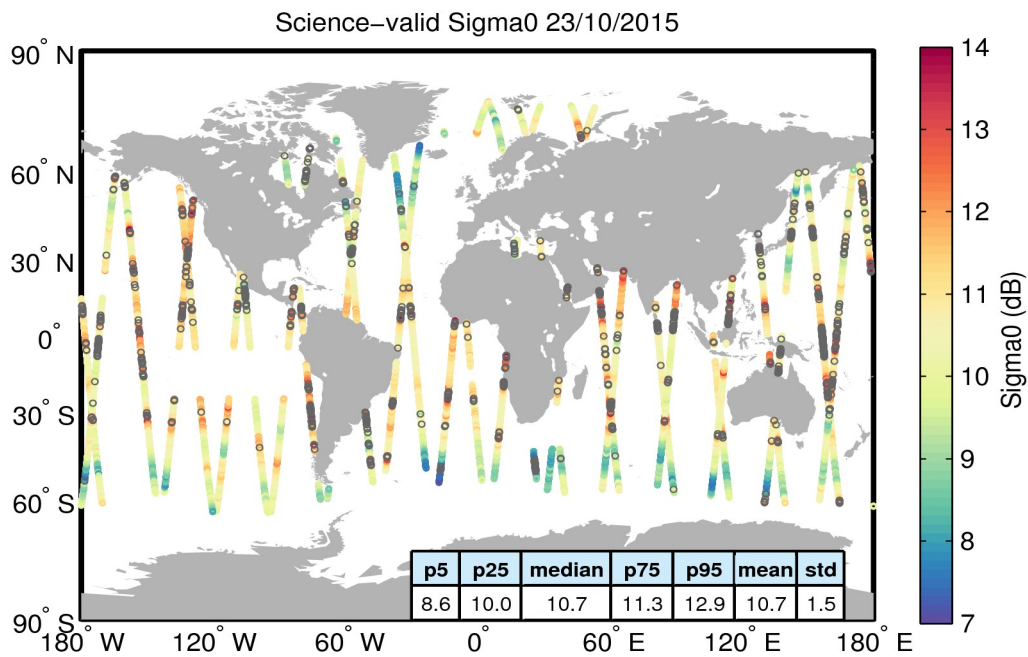
Figure 27. Geographical distribution of science-valid sigma0 data over oceans and lakes for 23/10/2015. The statistical values shown in the table refer to the sigma0 in dB and are calculated over all measurements shown in the figure. Gray circles denote records that have been rejected based on the editing criteria described in Table 4.
