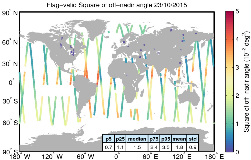
Figure 37. Geographical distribution of flag-valid mispointing data over oceans and lakes for 23/10/2015. The statistical values shown in the table refer to the mispointing in 10^{-2} \text{deg}^2 and are calculated over all measurements shown in the figure.
