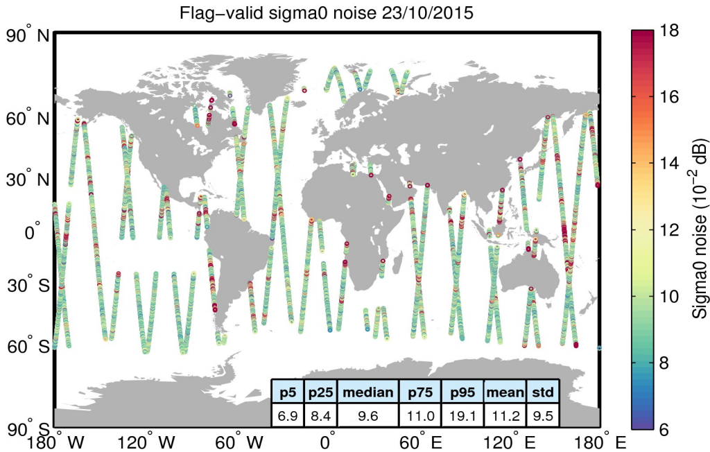
Figure 26. Geographical distribution of flag-valid 20-Hz sigma0 measurement noise over oceans and lakes for 23/10/2015. The statistical values shown in the table refer to the sigma0 noise and are calculated over all measurements shown in the figure.
