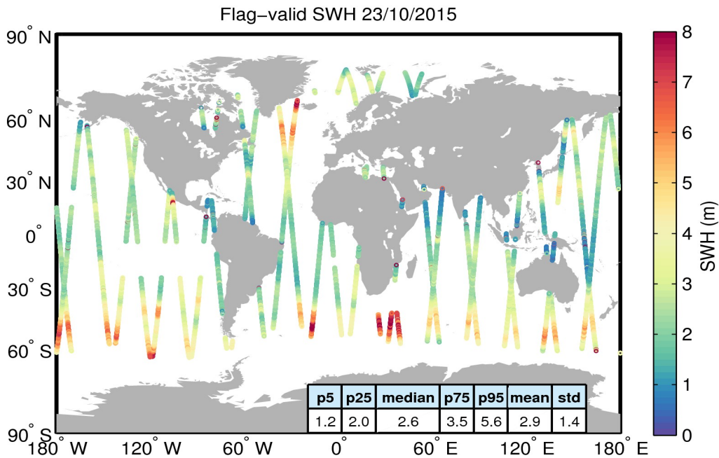
Figure 15. Geographical distribution of flag-valid SWH data over oceans and lakes for 23/10/2015. The statistical values shown in the table refer to the SWH in m and are calculated over all measurements shown in the figure.
