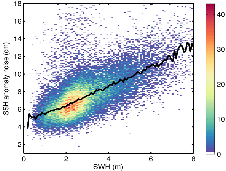
Figure 9. 2D histogram showing flag-valid SSH anomaly noise as a function of SWH for 23/10/2015. The black line denotes the median SSH anomaly noise as a function of SWH.
