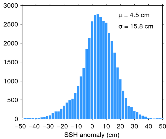
Figure 7. Histogram of flag-valid SSH anomaly over oceans and lakes for 23/10/2015. The mean ( \mu ) and standard deviation ( \sigma ) are also shown. Note that values outside [-50\ 50] cm are excluded from the histogram for the sake of readability but not from the computation of \mu and \sigma .
