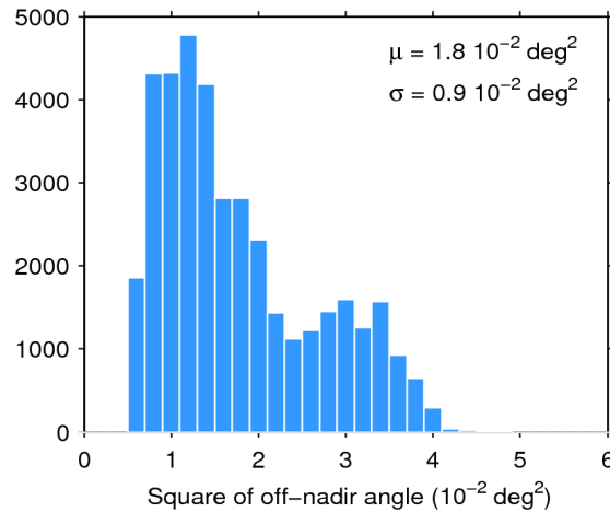
Figure 39. Histogram of flag-valid mispointing over oceans and lakes for 23/10/2015. The mean ( \mu ) and standard deviation ( \sigma ) are also shown. Note that values larger than 6 \cdot 10^{-2} \text{ deg}^2 are excluded from the histogram for the sake of readability but not from the computation of \mu and \sigma .
