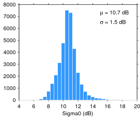
Figure 28. Histogram of science-valid sigma0 over oceans and lakes for 23/10/2015. The mean ( \mu ) and standard deviation ( \sigma ) are also shown. Note that values outside [4 20] dB are excluded from the histogram for the sake of readability but not from the computation of \mu and \sigma .
