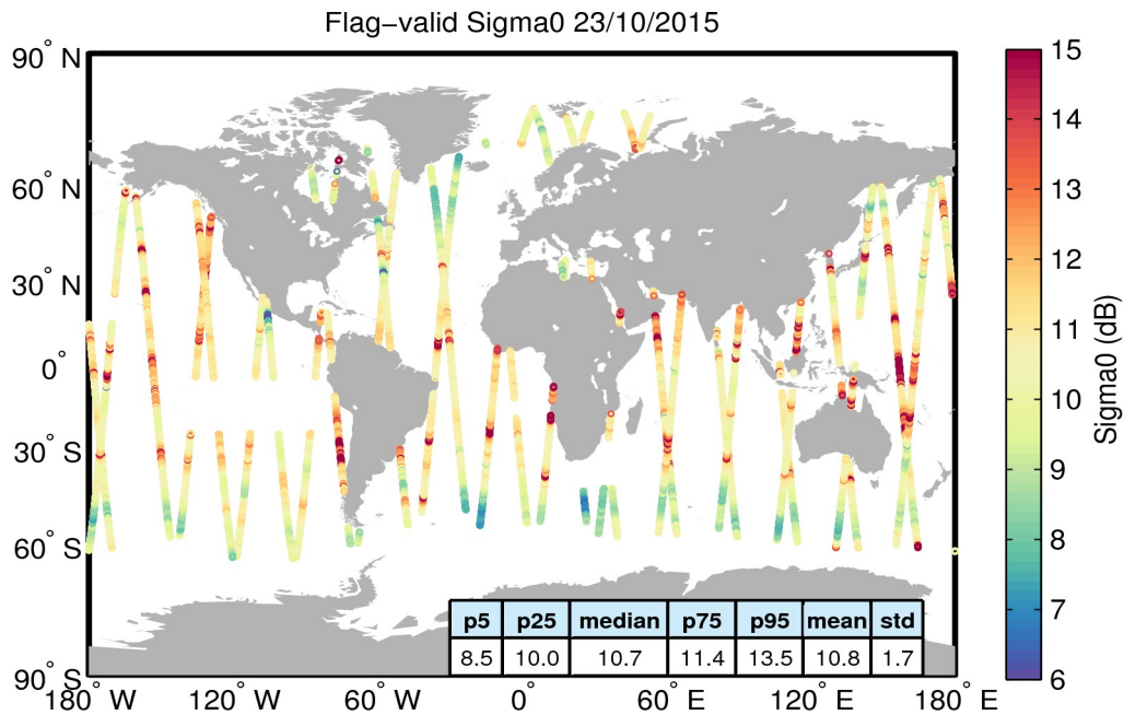
Figure 23. Geographical distribution of flag-valid sigma0 data over oceans and lakes for 23/10/2015. The statistical values shown in the table refer to the sigma0 in dB and are calculated over all measurements shown in the figure.
