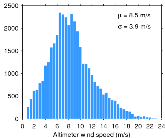
Figure 35. Histogram of science-valid wind over oceans and lakes for 23/10/2015. The mean ( \mu ) and standard deviation ( \sigma ) are also shown. Note that values larger than 24 m/s are excluded from the histogram for the sake of readability but not from the computation of \mu and \sigma .
