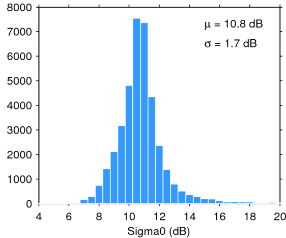
Figure 25. Histogram of flag-valid sigma0 over oceans and lakes for 23/10/2015. The mean ( \mu ) and standard deviation ( \sigma ) are also shown. Note that values outside [4 20] dB are excluded from the histogram for the sake of readability but not from the computation of \mu and \sigma .
