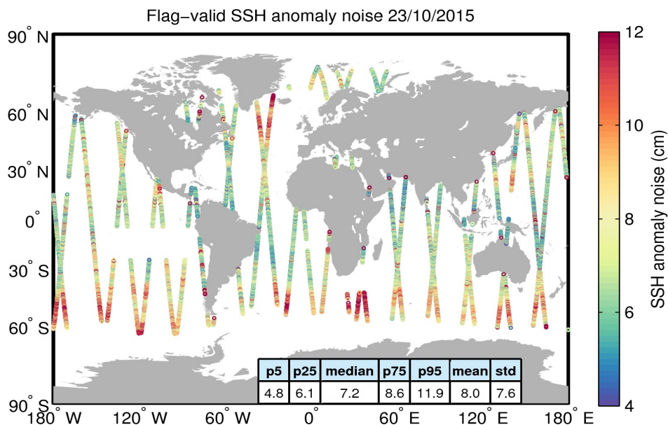
Figure 8. Geographical distribution of flag-valid 20-Hz SSH anomaly measurement noise over oceans and lakes for 23/10/2015. The statistical values shown in the table refer to the SSH anomaly noise and are calculated over all measurements shown in the figure.
