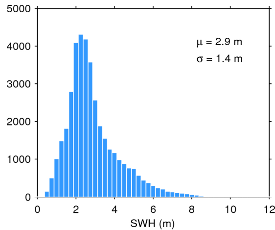
Figure 17. Histogram of flag-valid SWH over oceans and lakes for 23/10/2015. The mean ( \mu ) and standard deviation ( \sigma ) are also shown. Note that values larger than 12 m are excluded from the histogram for the sake of readability but not from the computation of \mu and \sigma .
