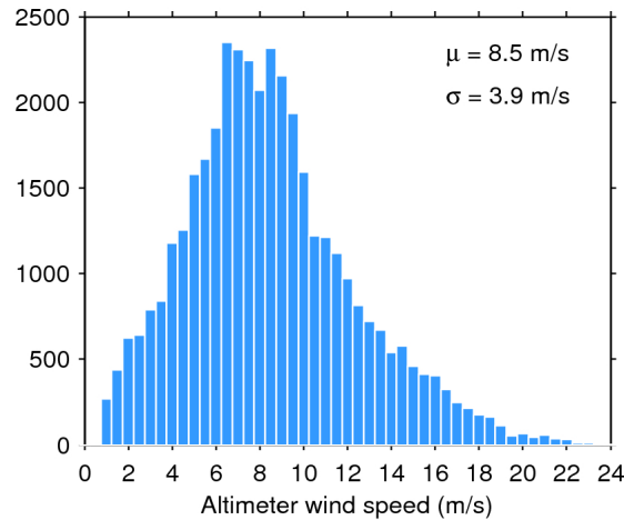
Figure 33. Histogram of flag-valid wind over oceans and lakes for 23/10/2015. The mean ( \mu ) and standard deviation ( \sigma ) are also shown. Note that values larger than 24 m/s are excluded from the histogram for the sake of readability but not from the computation of \mu and \sigma .
