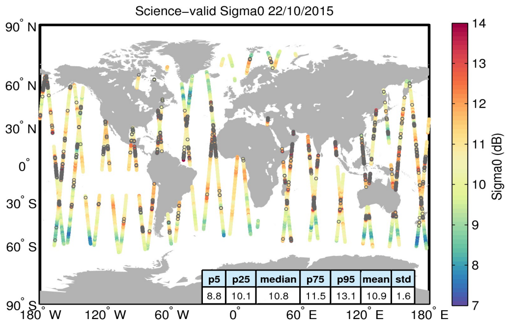
Figure 27. Geographical distribution of science-valid sigma0 data over oceans and lakes for 22/10/2015. The statistical values shown in the table refer to the sigma0 in dB and are calculated over all measurements shown in the figure. Gray circles denote records that have been rejected based on the editing criteria described in Table 4.
