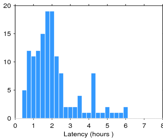
Figure 2. Histogram of the data latency for 22/10/2015. The y-axis denotes the number of files that are made available with a delay of x-hours with respect to the mean time of the records stored in the file.
