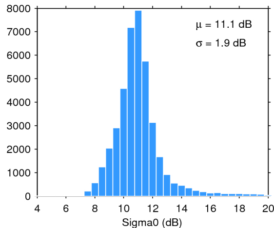
Figure 25. Histogram of flag-valid sigma0 over oceans and lakes for 22/10/2015. The mean ( \mu ) and standard deviation ( \sigma ) are also shown. Note that values outside [4 20] dB are excluded from the histogram for the sake of readability but not from the computation of \mu and \sigma .
