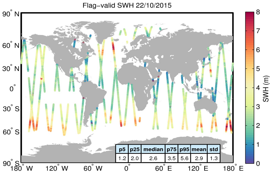
Figure 15. Geographical distribution of flag-valid SWH data over oceans and lakes for 22/10/2015. The statistical values shown in the table refer to the SWH in m and are calculated over all measurements shown in the figure.
