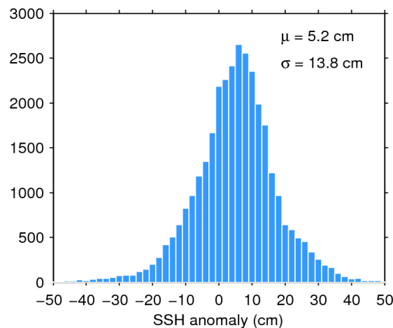
Figure 11. Histogram of science-valid SSH anomaly over oceans and lakes for 22/10/2015. The mean ( \mu ) and standard deviation ( \sigma ) are also shown. Note that values outside [-50 50] cm are excluded from the histogram for the sake of readability but not from the computation of \mu and \sigma .
