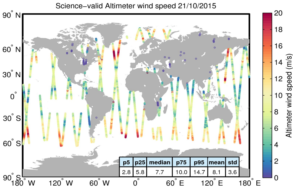
Figure 34. Geographical distribution of science-valid wind data over oceans and lakes for 21/10/2015. The statistical values shown in the table refer to the wind in m/s and are calculated over all measurements shown in the figure. Gray circles denote records that have been rejected based on the editing criteria described in Table 5.
