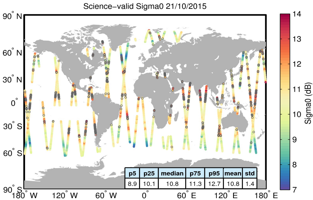
Figure 27. Geographical distribution of science-valid sigma0 data over oceans and lakes for 21/10/2015. The statistical values shown in the table refer to the sigma0 in dB and are calculated over all measurements shown in the figure. Gray circles denote records that have been rejected based on the editing criteria described in Table 4.
