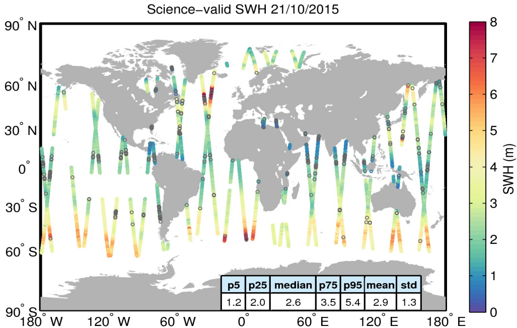
Figure 19. Geographical distribution of science-valid SWH data over oceans and lakes for 21/10/2015. The statistical values shown in the table refer to the SWH in m and are calculated over all measurements shown in the figure. Gray circles denote records that have been rejected based on the editing criteria described in Table 3.
