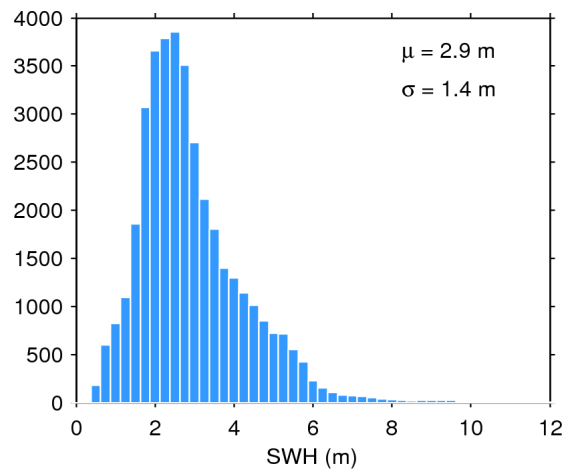
Figure 17. Histogram of flag-valid SWH over oceans and lakes for 21/10/2015. The mean ( \mu ) and standard deviation ( \sigma ) are also shown. Note that values larger than 12 m are excluded from the histogram for the sake of readability but not from the computation of \mu and \sigma .
