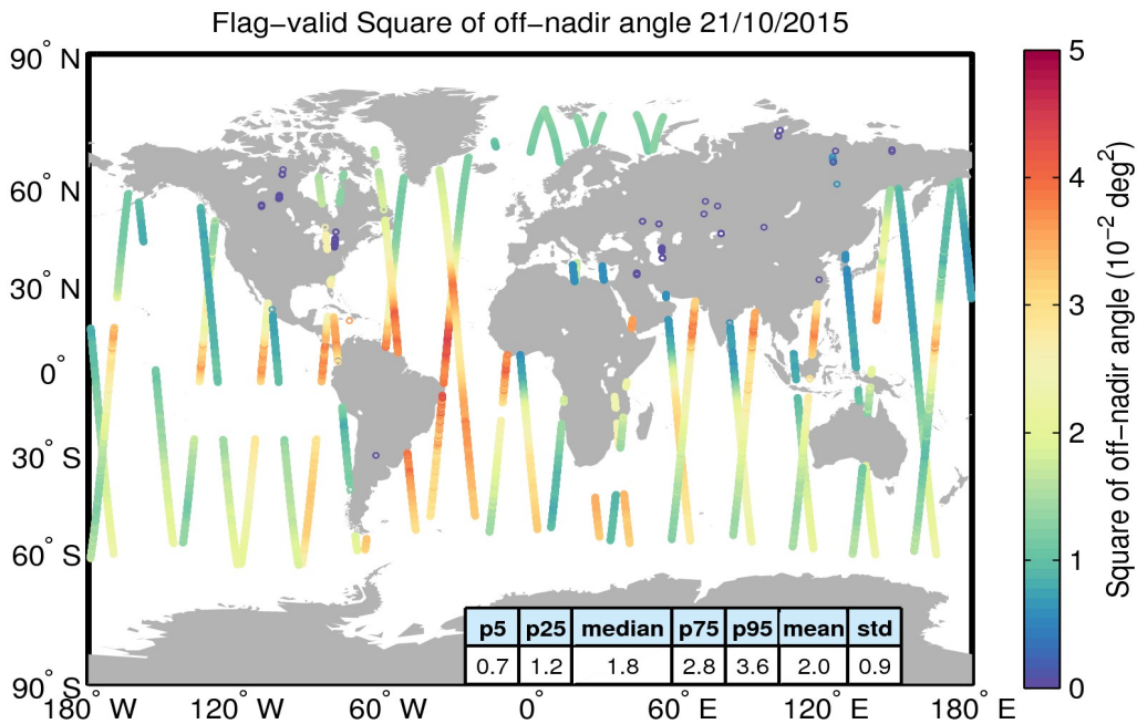
Figure 37. Geographical distribution of flag-valid mispointing data over oceans and lakes for 21/10/2015. The statistical values shown in the table refer to the mispointing in 10^{-2} deg 2 and are calculated over all measurements shown in the figure.
