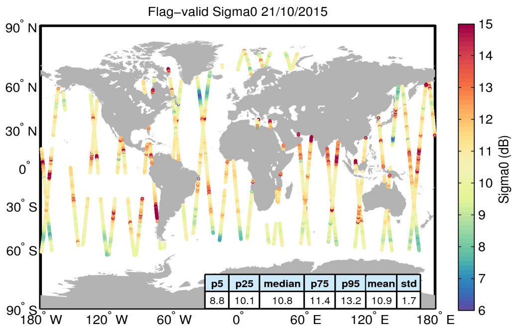
Figure 23. Geographical distribution of flag-valid sigma0 data over oceans and lakes for 21/10/2015. The statistical values shown in the table refer to the sigma0 in dB and are calculated over all measurements shown in the figure.
