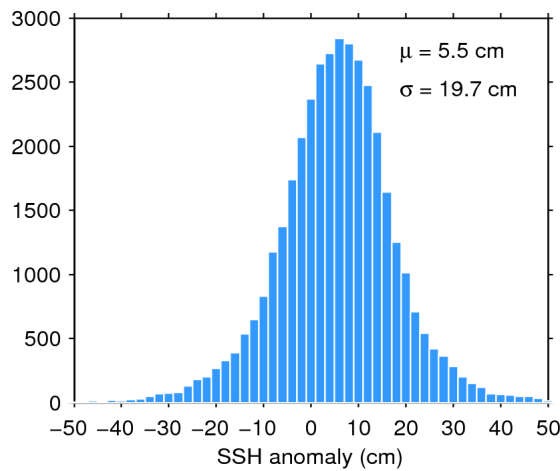
Figure 7. Histogram of flag-valid SSH anomaly over oceans and lakes for 21/10/2015. The mean ( \mu ) and standard deviation ( \sigma ) are also shown. Note that values outside [-50\ 50] cm are excluded from the histogram for the sake of readability but not from the computation of \mu and \sigma .
