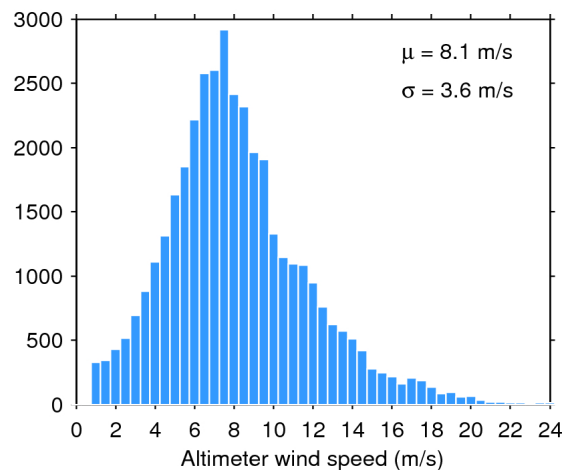
Figure 35. Histogram of science-valid wind over oceans and lakes for 21/10/2015. The mean ( \mu ) and standard deviation ( \sigma ) are also shown. Note that values larger than 24 m/s are excluded from the histogram for the sake of readability but not from the computation of \mu and \sigma .
