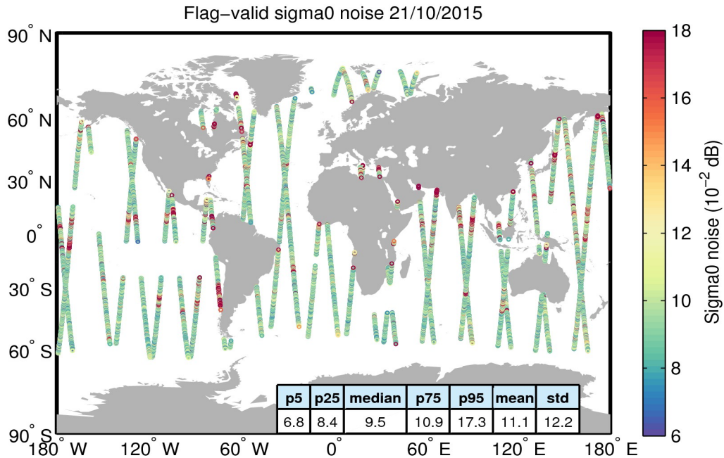
Figure 26. Geographical distribution of flag-valid 20-Hz sigma0 measurement noise over oceans and lakes for 21/10/2015. The statistical values shown in the table refer to the sigma0 noise and are calculated over all measurements shown in the figure.
