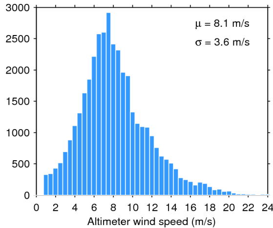
Figure 33. Histogram of flag-valid wind over oceans and lakes for 21/10/2015. The mean ( \mu ) and standard deviation ( \sigma ) are also shown. Note that values larger than 24 m/s are excluded from the histogram for the sake of readability but not from the computation of \mu and \sigma .
