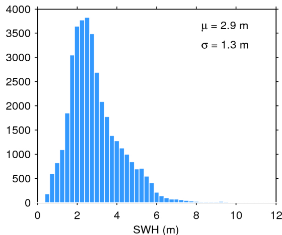
Figure 20. Histogram of science-valid SWH over oceans and lakes for 21/10/2015. The mean ( \mu ) and standard deviation ( \sigma ) are also shown. Note that values larger than 12 m are excluded from the histogram for the sake of readability but not from the computation of \mu and \sigma .
