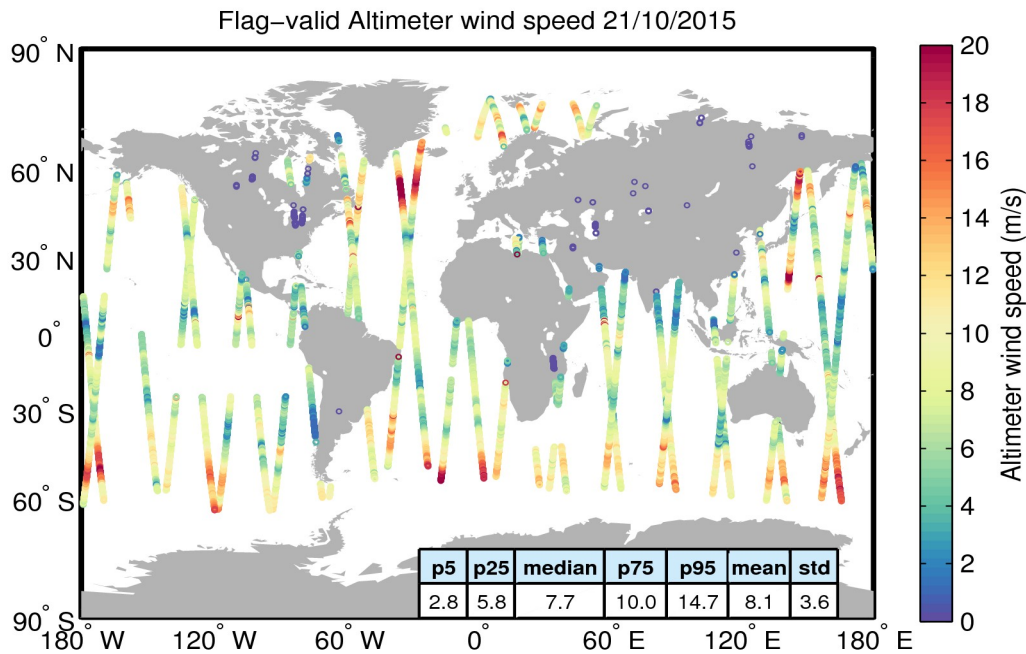
Figure 31. Geographical distribution of flag-valid wind data over oceans and lakes for 21/10/2015. The statistical values shown in the table refer to the wind in m/s and are calculated over all measurements shown in the figure.
