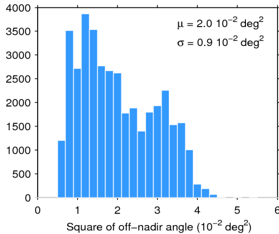
Figure 39. Histogram of flag-valid mispointing over oceans and lakes for 21/10/2015. The mean ( \mu ) and standard deviation ( \sigma ) are also shown. Note that values larger than 6 \cdot 10^{-2} \text{ deg}^2 are excluded from the histogram for the sake of readability but not from the computation of \mu and \sigma .
