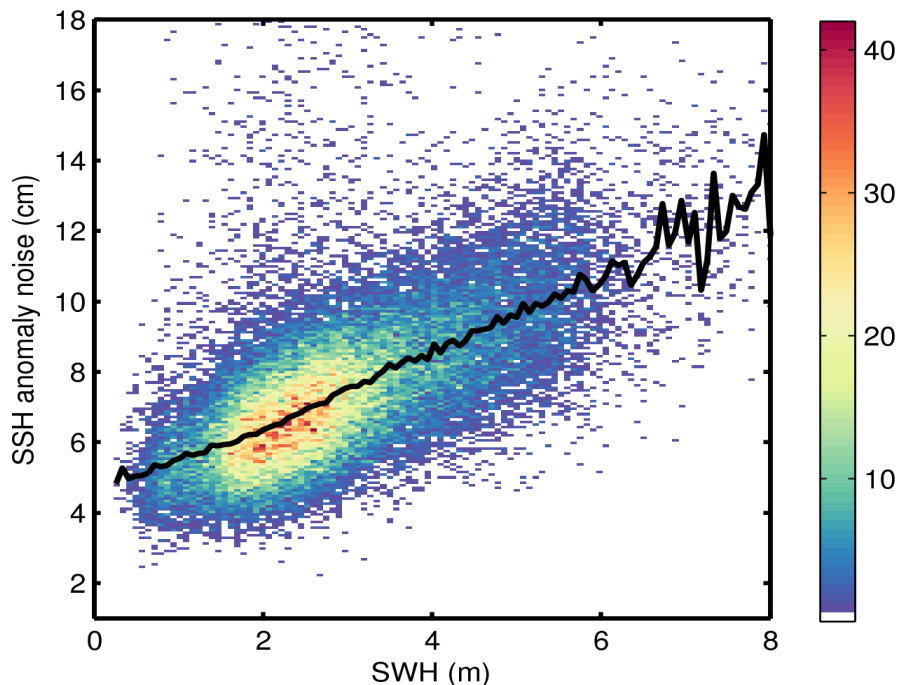
Figure 9. 2D histogram showing flag-valid SSH anomaly noise as a function of SWH for 21/10/2015. The black line denotes the median SSH anomaly noise as a function of SWH.
