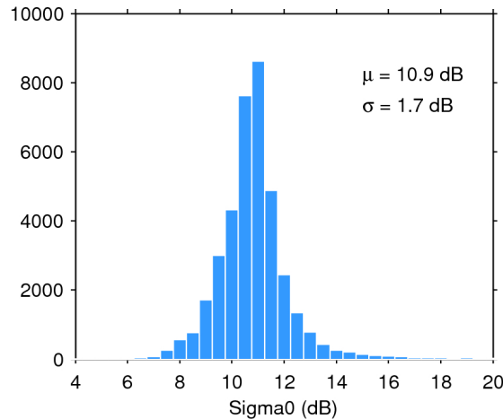
Figure 25. Histogram of flag-valid sigma0 over oceans and lakes for 21/10/2015. The mean ( \mu ) and standard deviation ( \sigma ) are also shown. Note that values outside [4 20] dB are excluded from the histogram for the sake of readability but not from the computation of \mu and \sigma .
