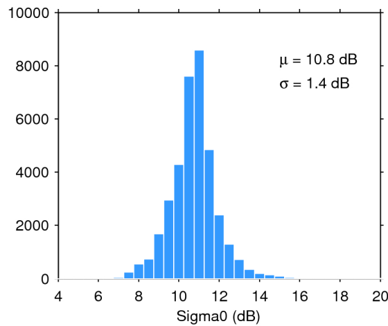
Figure 28. Histogram of science-valid sigma0 over oceans and lakes for 21/10/2015. The mean ( \mu ) and standard deviation ( \sigma ) are also shown. Note that values outside [4 20] dB are excluded from the histogram for the sake of readability but not from the computation of \mu and \sigma .
