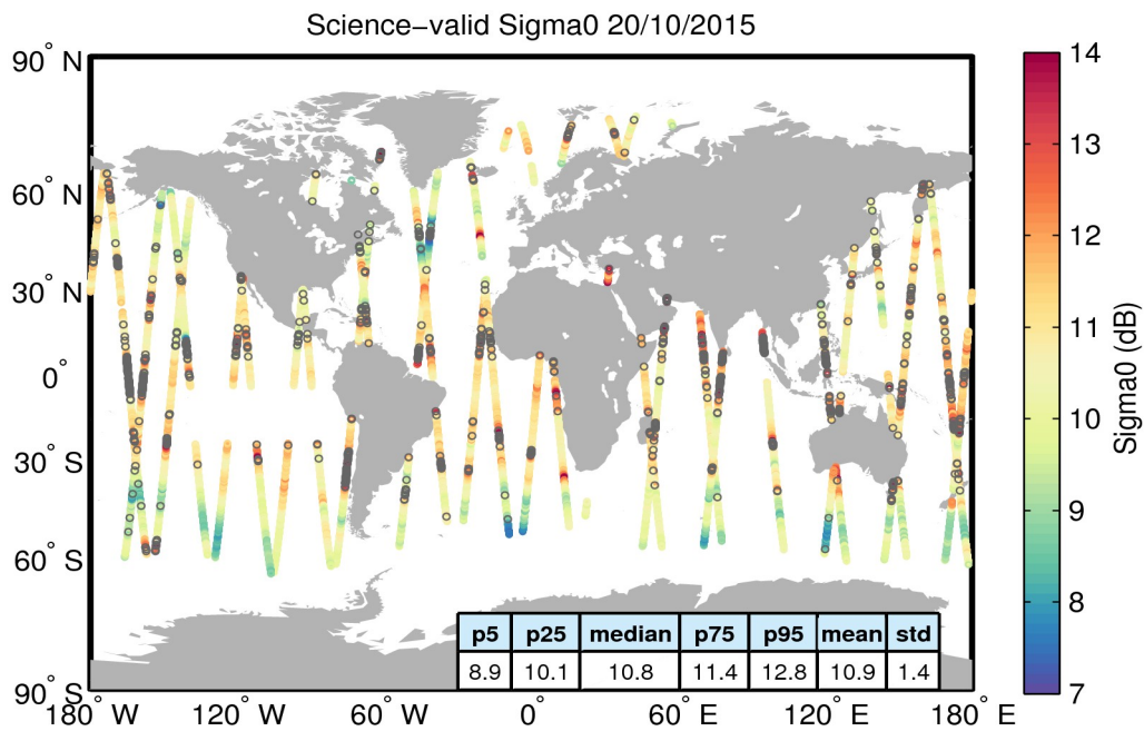
Figure 27. Geographical distribution of science-valid sigma0 data over oceans and lakes for 20/10/2015. The statistical values shown in the table refer to the sigma0 in dB and are calculated over all measurements shown in the figure. Gray circles denote records that have been rejected based on the editing criteria described in Table 4.
