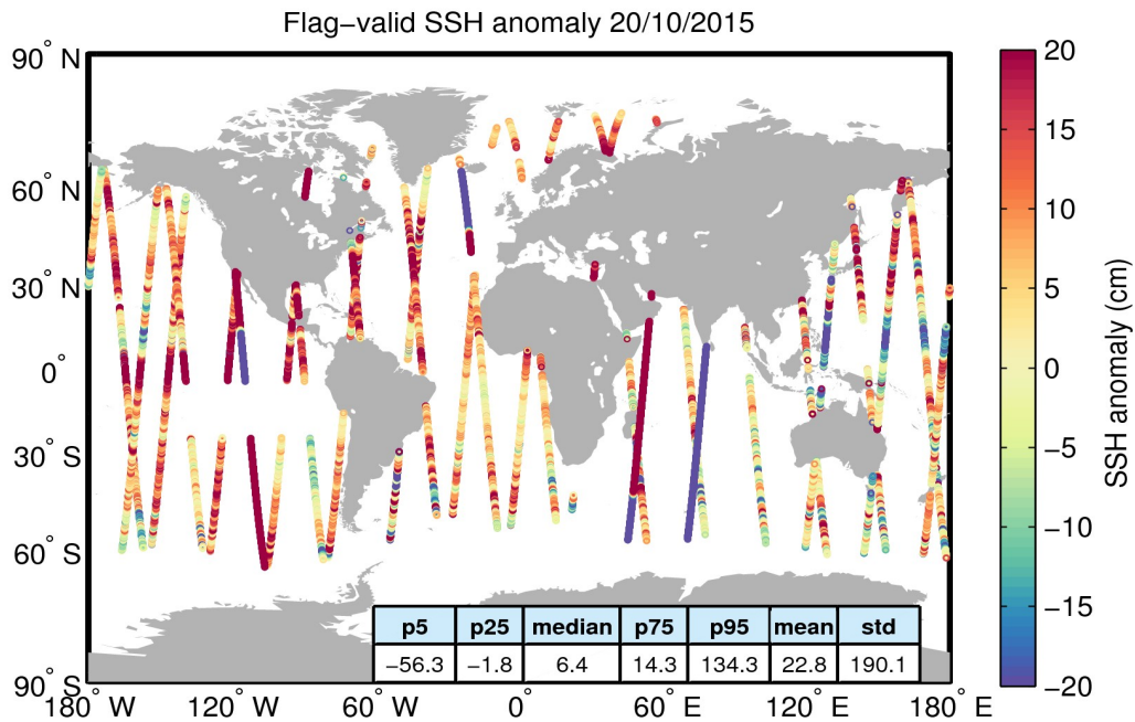
Figure 5. Geographical distribution of flag-valid 1-Hz SSH anomaly data over oceans and lakes for 20/10/2015. The statistical values shown in the table refer to the SSH anomaly in cm and are calculated over all measurements shown in the figure.
