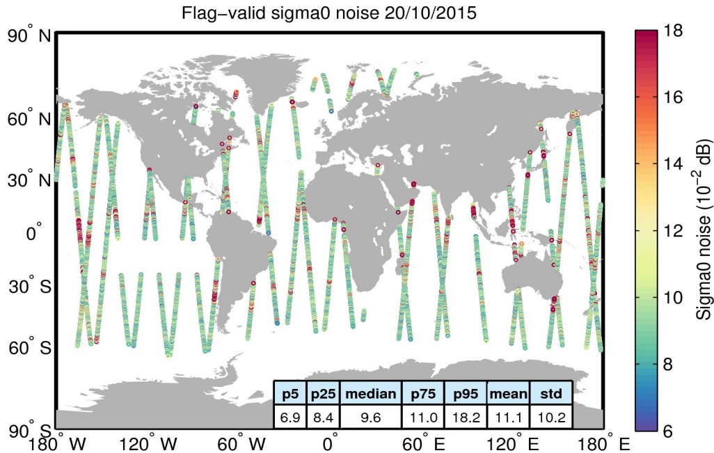
Figure 26. Geographical distribution of flag-valid 20-Hz sigma0 measurement noise over oceans and lakes for 20/10/2015. The statistical values shown in the table refer to the sigma0 noise and are calculated over all measurements shown in the figure.
