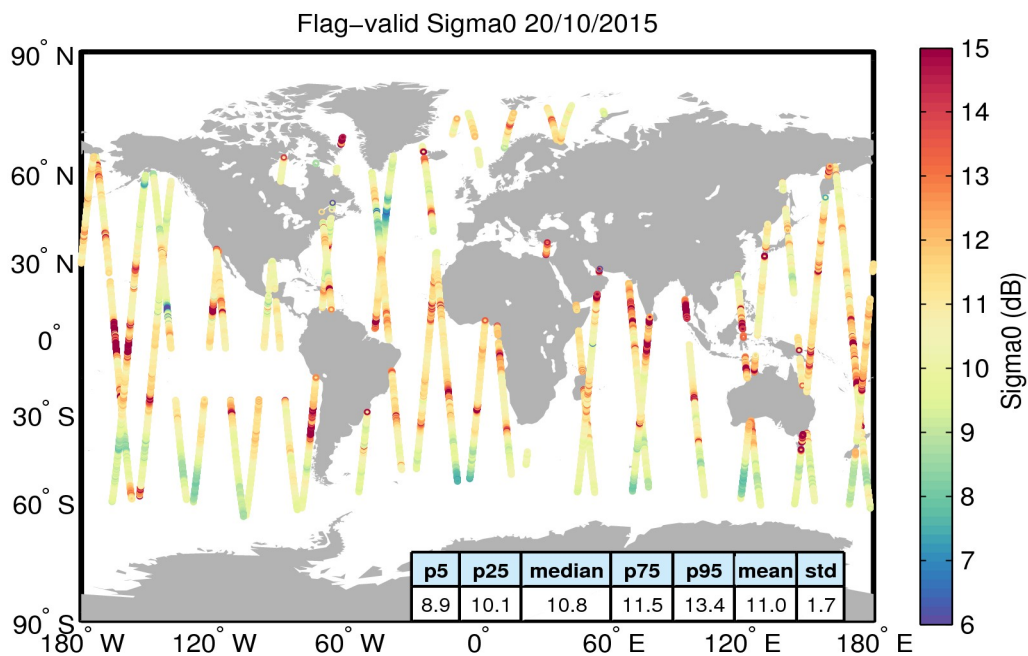
Figure 23. Geographical distribution of flag-valid sigma0 data over oceans and lakes for 20/10/2015. The statistical values shown in the table refer to the sigma0 in dB and are calculated over all measurements shown in the figure.
