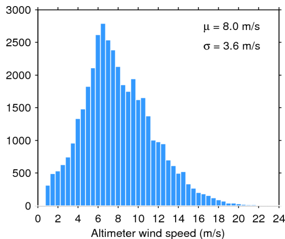
Figure 35. Histogram of science-valid wind over oceans and lakes for 20/10/2015. The mean ( \mu ) and standard deviation ( \sigma ) are also shown. Note that values larger than 24 m/s are excluded from the histogram for the sake of readability but not from the computation of \mu and \sigma .
