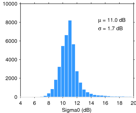
Figure 25. Histogram of flag-valid sigma0 over oceans and lakes for 20/10/2015. The mean ( \mu ) and standard deviation ( \sigma ) are also shown. Note that values outside [4 20] dB are excluded from the histogram for the sake of readability but not from the computation of \mu and \sigma .
