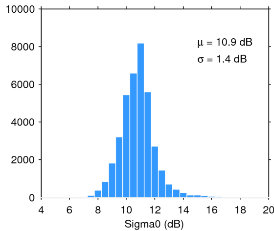
Figure 28. Histogram of science-valid sigma0 over oceans and lakes for 20/10/2015. The mean ( \mu ) and standard deviation ( \sigma ) are also shown. Note that values outside [4 20] dB are excluded from the histogram for the sake of readability but not from the computation of \mu and \sigma .
