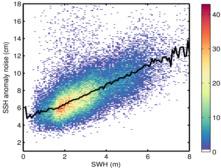
Figure 9. 2D histogram showing flag-valid SSH anomaly noise as a function of SWH for 20/10/2015. The black line denotes the median SSH anomaly noise as a function of SWH.
