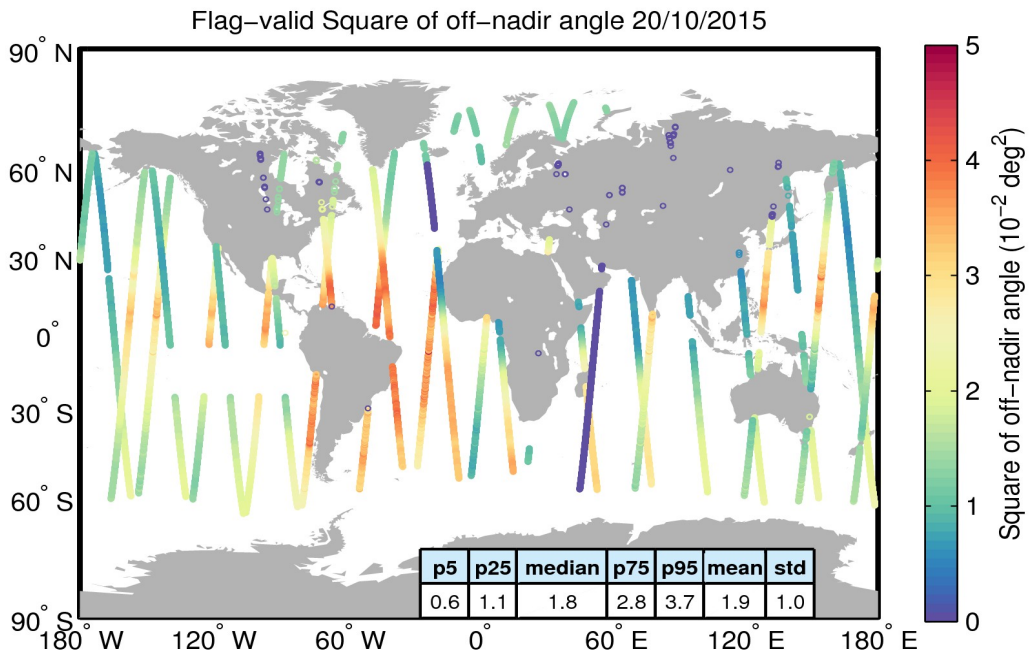
Figure 37. Geographical distribution of flag-valid mispointing data over oceans and lakes for 20/10/2015. The statistical values shown in the table refer to the mispointing in 10^{-2} \text{ deg}^2 and are calculated over all measurements shown in the figure.
