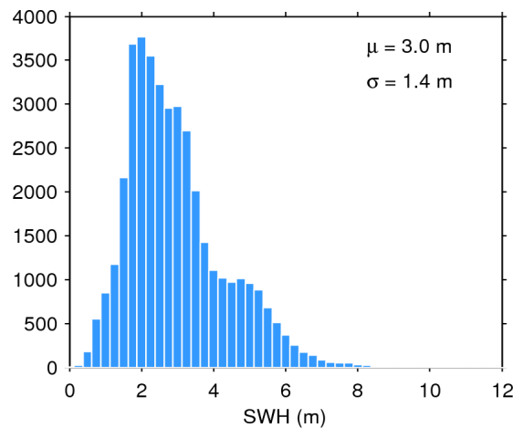
Figure 17. Histogram of flag-valid SWH over oceans and lakes for 20/10/2015. The mean ( \mu ) and standard deviation ( \sigma ) are also shown. Note that values larger than 12 m are excluded from the histogram for the sake of readability but not from the computation of \mu and \sigma .
