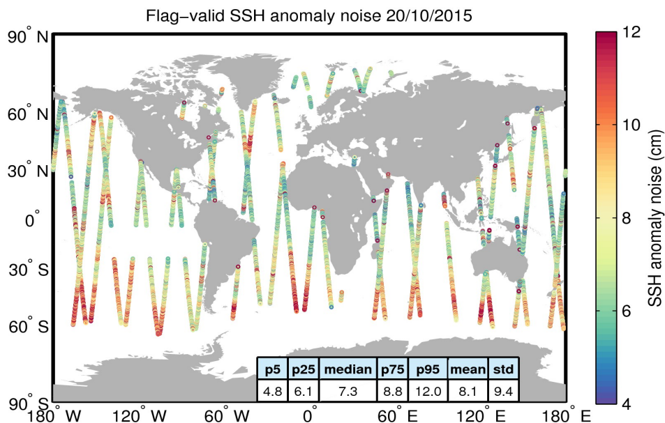
Figure 8. Geographical distribution of flag-valid 20-Hz SSH anomaly measurement noise over oceans and lakes for 20/10/2015. The statistical values shown in the table refer to the SSH anomaly noise and are calculated over all measurements shown in the figure.
