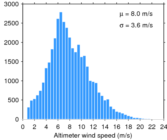
Figure 33. Histogram of flag-valid wind over oceans and lakes for 20/10/2015. The mean ( \mu ) and standard deviation ( \sigma ) are also shown. Note that values larger than 24 m/s are excluded from the histogram for the sake of readability but not from the computation of \mu and \sigma .
