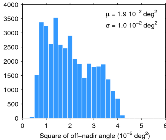
Figure 39. Histogram of flag-valid mispointing over oceans and lakes for 20/10/2015. The mean ( \mu ) and standard deviation ( \sigma ) are also shown. Note that values larger than 6 \cdot 10^{-2} \text{ deg}^2 are excluded from the histogram for the sake of readability but not from the computation of \mu and \sigma .
