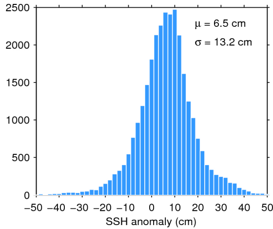
Figure 11. Histogram of science-valid SSH anomaly over oceans and lakes for 20/10/2015. The mean ( \mu ) and standard deviation ( \sigma ) are also shown. Note that values outside [-50 50] cm are excluded from the histogram for the sake of readability but not from the computation of \mu and \sigma .
