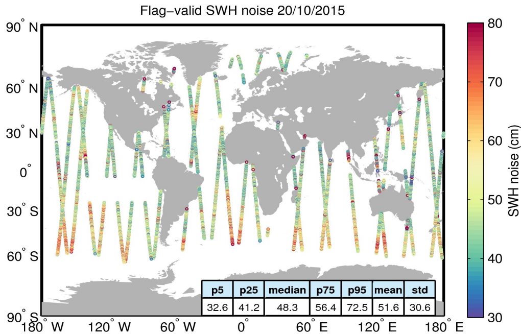
Figure 18. Geographical distribution of flag-valid 20-Hz SWH measurement noise over oceans and lakes for 20/10/2015. The statistical values shown in the table refer to the SWH noise and are calculated over all measurements shown in the figure.
