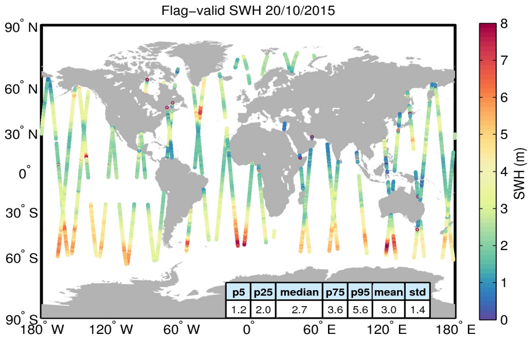
Figure 15. Geographical distribution of flag-valid SWH data over oceans and lakes for 20/10/2015. The statistical values shown in the table refer to the SWH in m and are calculated over all measurements shown in the figure.
