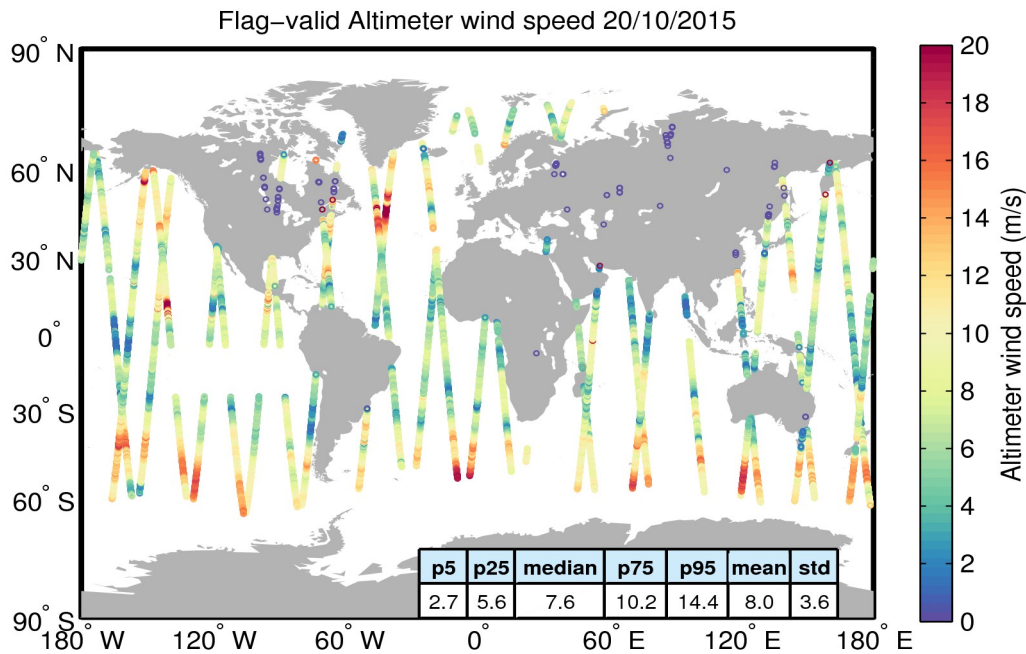
Figure 31. Geographical distribution of flag-valid wind data over oceans and lakes for 20/10/2015. The statistical values shown in the table refer to the wind in m/s and are calculated over all measurements shown in the figure.
