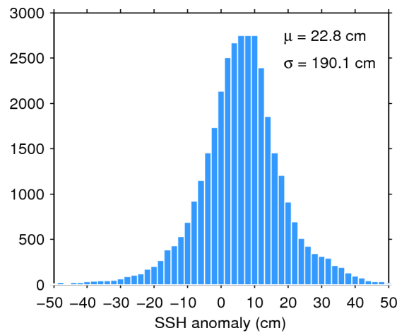
Figure 7. Histogram of flag-valid SSH anomaly over oceans and lakes for 20/10/2015. The mean ( \mu ) and standard deviation ( \sigma ) are also shown. Note that values outside [-50\ 50] cm are excluded from the histogram for the sake of readability but not from the computation of \mu and \sigma .
