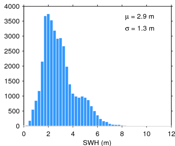
Figure 20. Histogram of science-valid SWH over oceans and lakes for 20/10/2015. The mean ( \mu ) and standard deviation ( \sigma ) are also shown. Note that values larger than 12 m are excluded from the histogram for the sake of readability but not from the computation of \mu and \sigma .
