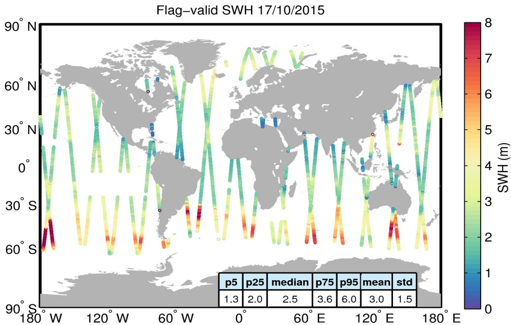
Figure 15. Geographical distribution of flag-valid SWH data over oceans and lakes for 17/10/2015. The statistical values shown in the table refer to the SWH in m and are calculated over all measurements shown in the figure.
