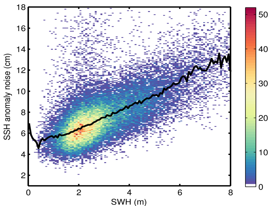
Figure 9. 2D histogram showing flag-valid SSH anomaly noise as a function of SWH for 17/10/2015. The black line denotes the median SSH anomaly noise as a function of SWH.
