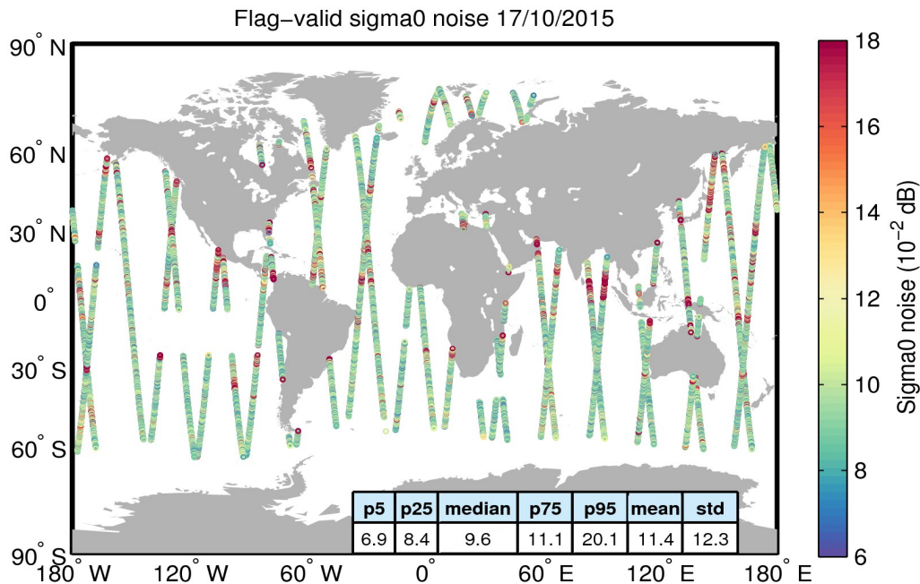
Figure 26. Geographical distribution of flag-valid 20-Hz sigma0 measurement noise over oceans and lakes for 17/10/2015. The statistical values shown in the table refer to the sigma0 noise and are calculated over all measurements shown in the figure.
