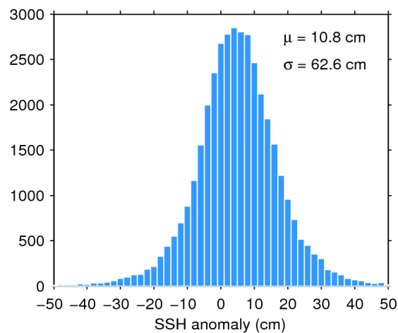
Figure 7. Histogram of flag-valid SSH anomaly over oceans and lakes for 17/10/2015. The mean ( \mu ) and standard deviation ( \sigma ) are also shown. Note that values outside [-50 50] cm are excluded from the histogram for the sake of readability but not from the computation of \mu and \sigma .
