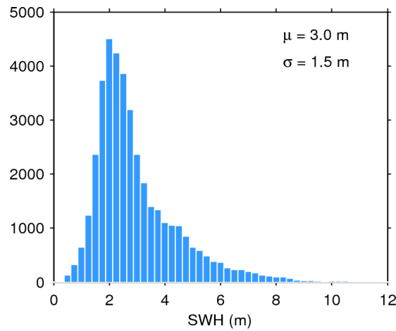
Figure 17. Histogram of flag-valid SWH over oceans and lakes for 17/10/2015. The mean ( \mu ) and standard deviation ( \sigma ) are also shown. Note that values larger than 12 m are excluded from the histogram for the sake of readability but not from the computation of \mu and \sigma .
