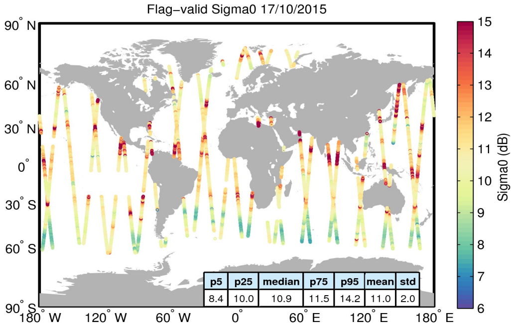
Figure 23. Geographical distribution of flag-valid sigma0 data over oceans and lakes for 17/10/2015. The statistical values shown in the table refer to the sigma0 in dB and are calculated over all measurements shown in the figure.
