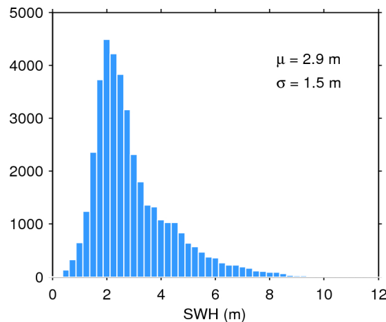
Figure 20. Histogram of science-valid SWH over oceans and lakes for 17/10/2015. The mean ( \mu ) and standard deviation ( \sigma ) are also shown. Note that values larger than 12 m are excluded from the histogram for the sake of readability but not from the computation of \mu and \sigma .
