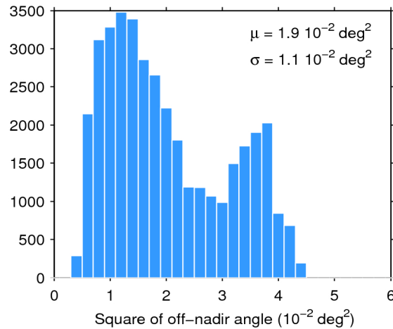
Figure 39. Histogram of flag-valid mispointing over oceans and lakes for 17/10/2015. The mean ( \mu ) and standard deviation ( \sigma ) are also shown. Note that values larger than 6 \cdot 10^{-2} \text{ deg}^2 are excluded from the histogram for the sake of readability but not from the computation of \mu and \sigma .
