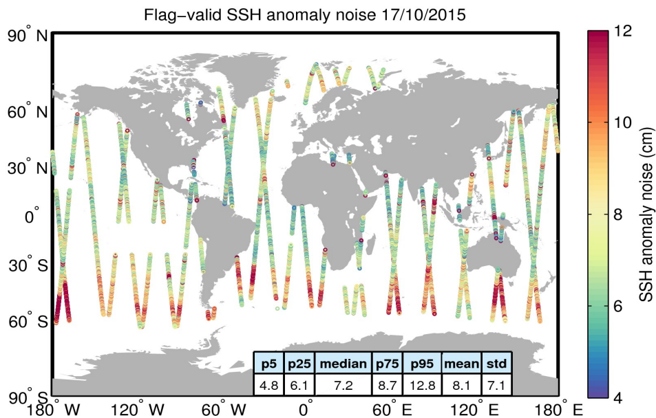
Figure 8. Geographical distribution of flag-valid 20-Hz SSH anomaly measurement noise over oceans and lakes for 17/10/2015. The statistical values shown in the table refer to the SSH anomaly noise and are calculated over all measurements shown in the figure.
