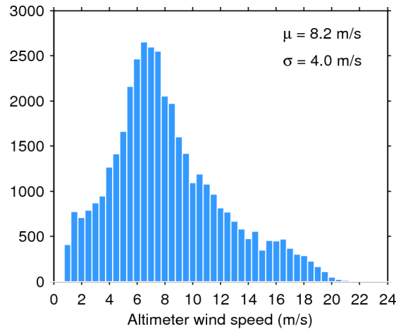
Figure 33. Histogram of flag-valid wind over oceans and lakes for 17/10/2015. The mean ( \mu ) and standard deviation ( \sigma ) are also shown. Note that values larger than 24 m/s are excluded from the histogram for the sake of readability but not from the computation of \mu and \sigma .
