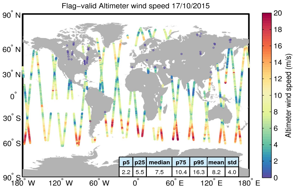
Figure 31. Geographical distribution of flag-valid wind data over oceans and lakes for 17/10/2015. The statistical values shown in the table refer to the wind in m/s and are calculated over all measurements shown in the figure.
