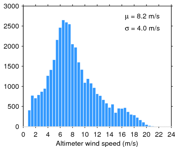
Figure 35. Histogram of science-valid wind over oceans and lakes for 17/10/2015. The mean ( \mu ) and standard deviation ( \sigma ) are also shown. Note that values larger than 24 m/s are excluded from the histogram for the sake of readability but not from the computation of \mu and \sigma .
