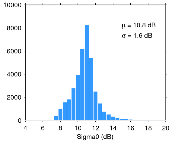
Figure 28. Histogram of science-valid sigma0 over oceans and lakes for 17/10/2015. The mean ( \mu ) and standard deviation ( \sigma ) are also shown. Note that values outside [4 20] dB are excluded from the histogram for the sake of readability but not from the computation of \mu and \sigma .
