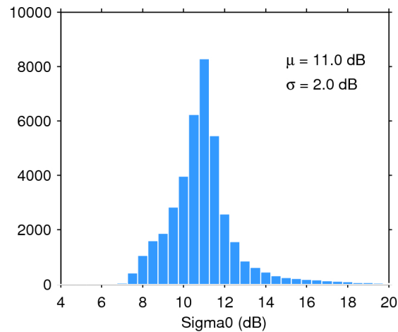
Figure 25. Histogram of flag-valid sigma0 over oceans and lakes for 17/10/2015. The mean ( \mu ) and standard deviation ( \sigma ) are also shown. Note that values outside [4 20] dB are excluded from the histogram for the sake of readability but not from the computation of \mu and \sigma .
