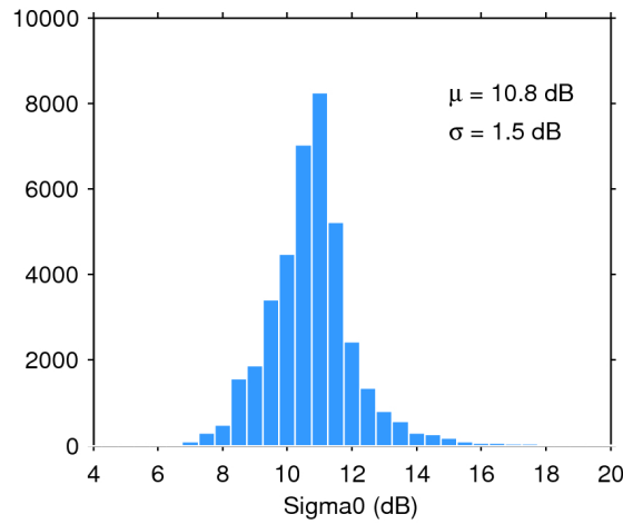
Figure 28. Histogram of science-valid sigma0 over oceans and lakes for 16/10/2015. The mean ( \mu ) and standard deviation ( \sigma ) are also shown. Note that values outside [4 20] dB are excluded from the histogram for the sake of readability but not from the computation of \mu and \sigma .
