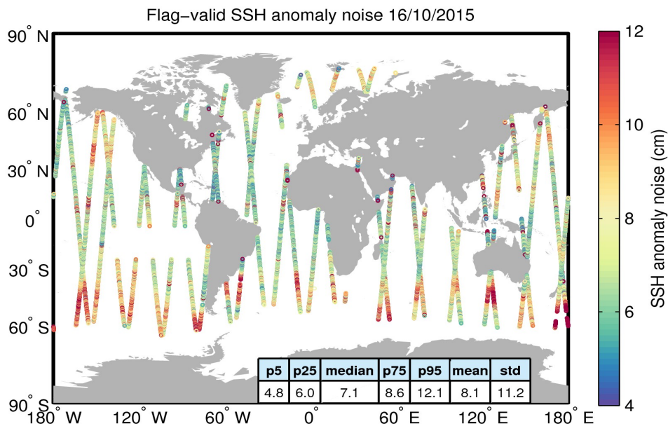
Figure 8. Geographical distribution of flag-valid 20-Hz SSH anomaly measurement noise over oceans and lakes for 16/10/2015. The statistical values shown in the table refer to the SSH anomaly noise and are calculated over all measurements shown in the figure.
