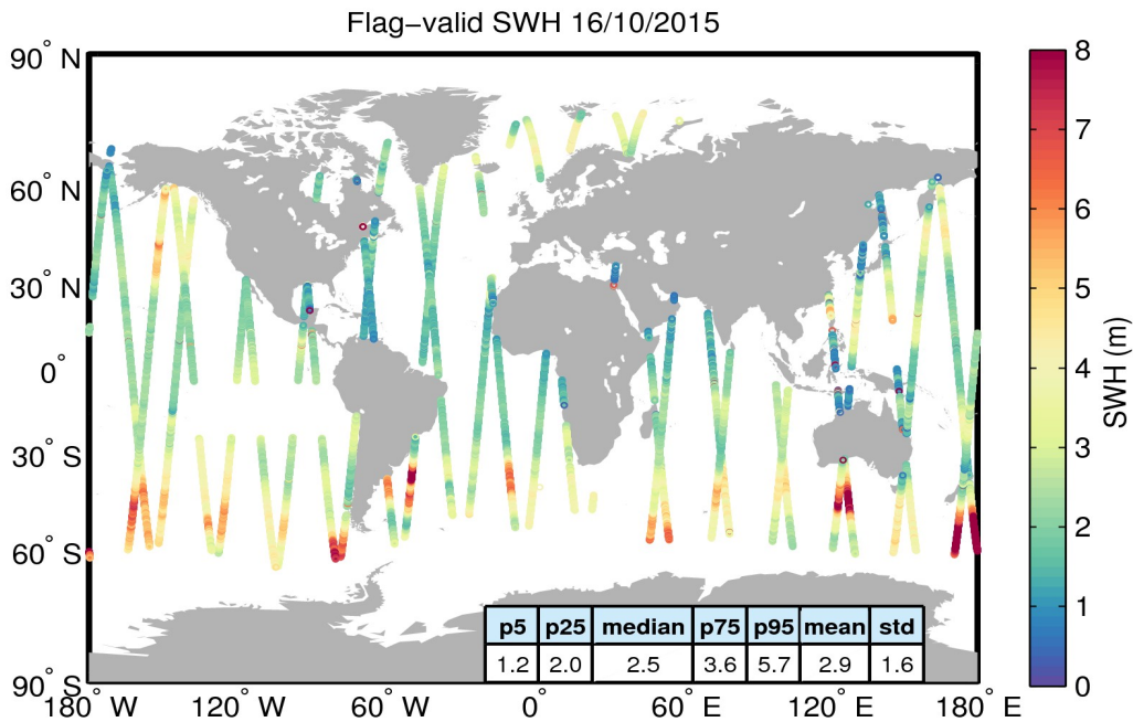
Figure 15. Geographical distribution of flag-valid SWH data over oceans and lakes for 16/10/2015. The statistical values shown in the table refer to the SWH in m and are calculated over all measurements shown in the figure.
