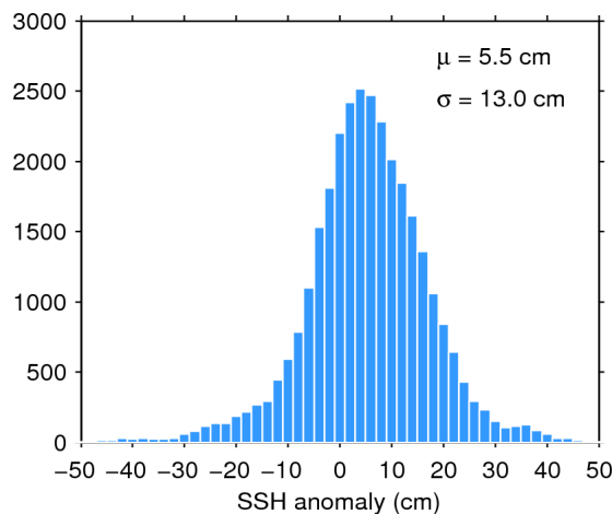
Figure 11. Histogram of science-valid SSH anomaly over oceans and lakes for 16/10/2015. The mean ( \mu ) and standard deviation ( \sigma ) are also shown. Note that values outside [-50 50] cm are excluded from the histogram for the sake of readability but not from the computation of \mu and \sigma .
