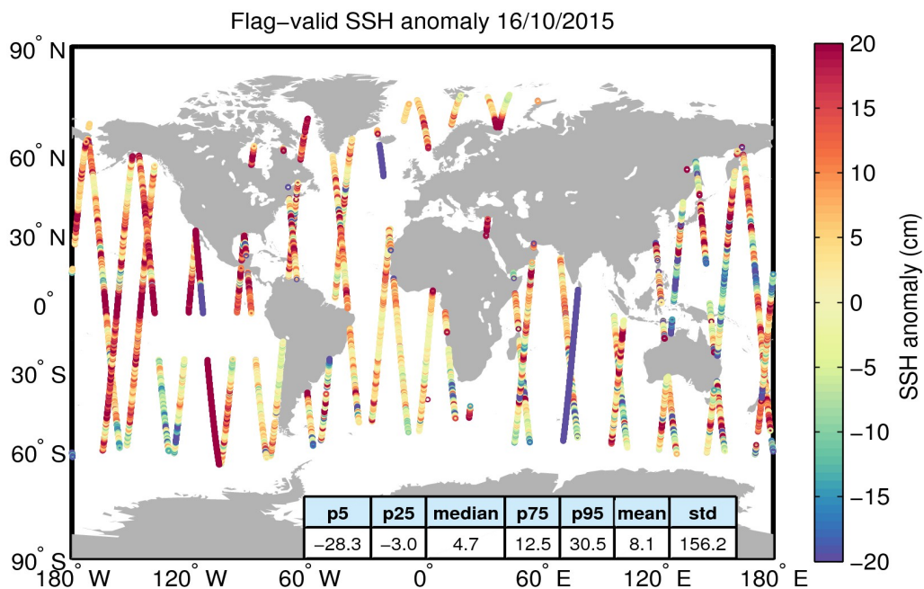
Figure 5. Geographical distribution of flag-valid 1-Hz SSH anomaly data over oceans and lakes for 16/10/2015. The statistical values shown in the table refer to the SSH anomaly in cm and are calculated over all measurements shown in the figure.
