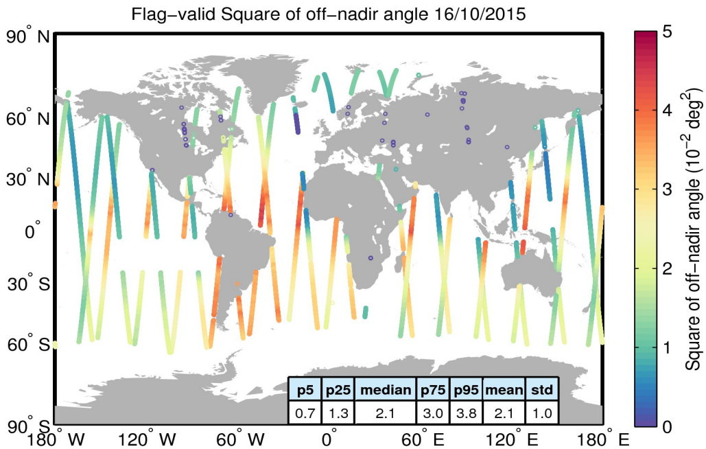
Figure 37. Geographical distribution of flag-valid mispointing data over oceans and lakes for 16/10/2015. The statistical values shown in the table refer to the mispointing in 10^{-2} deg 2 and are calculated over all measurements shown in the figure.
