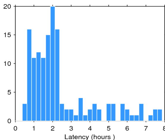
Figure 2. Histogram of the data latency for 16/10/2015. The y-axis denotes the number of files that are made available with a delay of x-hours with respect to the mean time of the records stored in the file.
