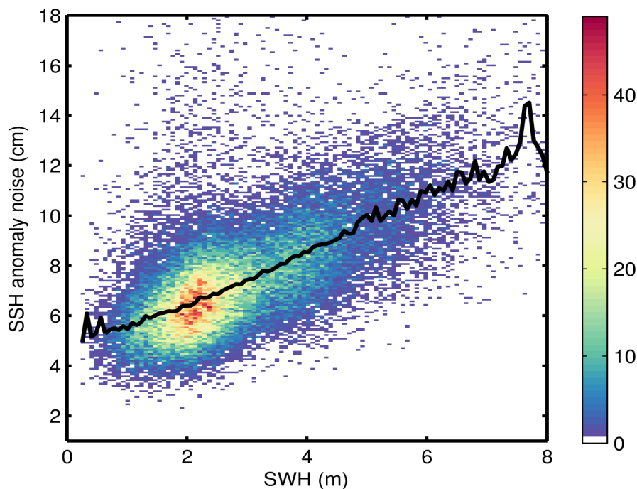
Figure 9. 2D histogram showing flag-valid SSH anomaly noise as a function of SWH for 16/10/2015. The black line denotes the median SSH anomaly noise as a function of SWH.
