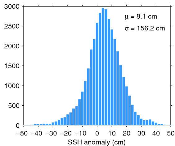
Figure 7. Histogram of flag-valid SSH anomaly over oceans and lakes for 16/10/2015. The mean ( \mu ) and standard deviation ( \sigma ) are also shown. Note that values outside [-50 50] cm are excluded from the histogram for the sake of readability but not from the computation of \mu and \sigma .
