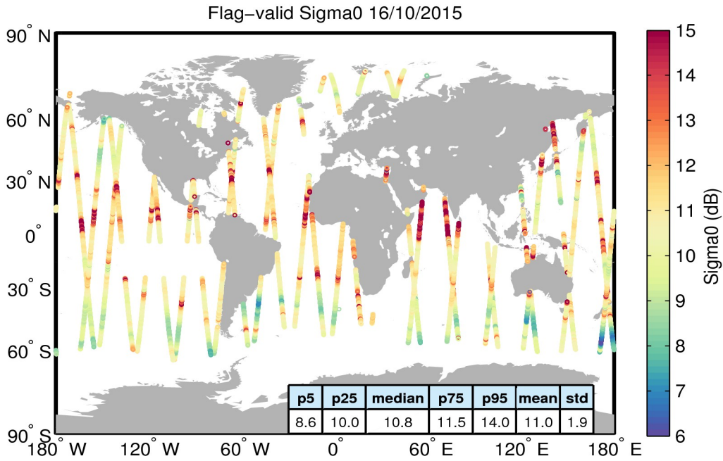
Figure 23. Geographical distribution of flag-valid sigma0 data over oceans and lakes for 16/10/2015. The statistical values shown in the table refer to the sigma0 in dB and are calculated over all measurements shown in the figure.
