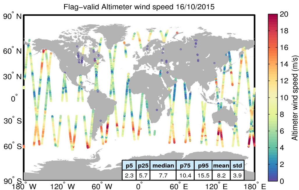
Figure 31. Geographical distribution of flag-valid wind data over oceans and lakes for 16/10/2015. The statistical values shown in the table refer to the wind in m/s and are calculated over all measurements shown in the figure.
