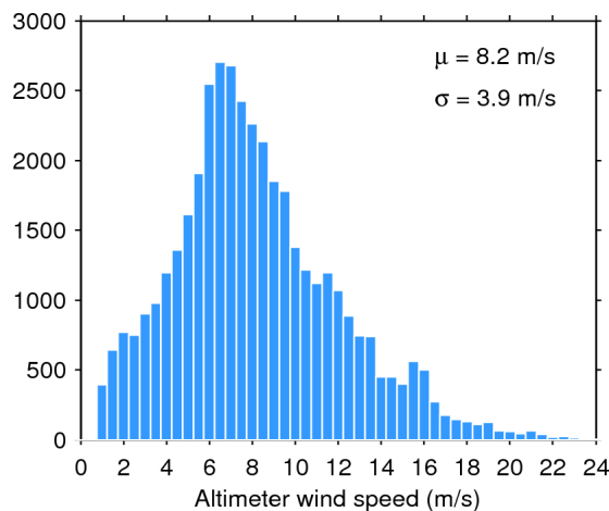
Figure 35. Histogram of science-valid wind over oceans and lakes for 16/10/2015. The mean ( \mu ) and standard deviation ( \sigma ) are also shown. Note that values larger than 24 m/s are excluded from the histogram for the sake of readability but not from the computation of \mu and \sigma .
