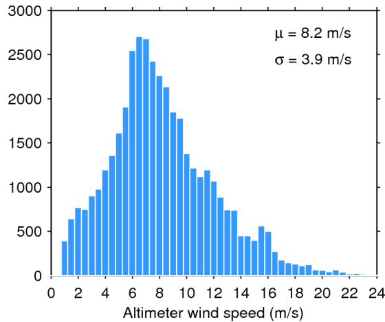
Figure 33. Histogram of flag-valid wind over oceans and lakes for 16/10/2015. The mean ( \mu ) and standard deviation ( \sigma ) are also shown. Note that values larger than 24 m/s are excluded from the histogram for the sake of readability but not from the computation of \mu and \sigma .
