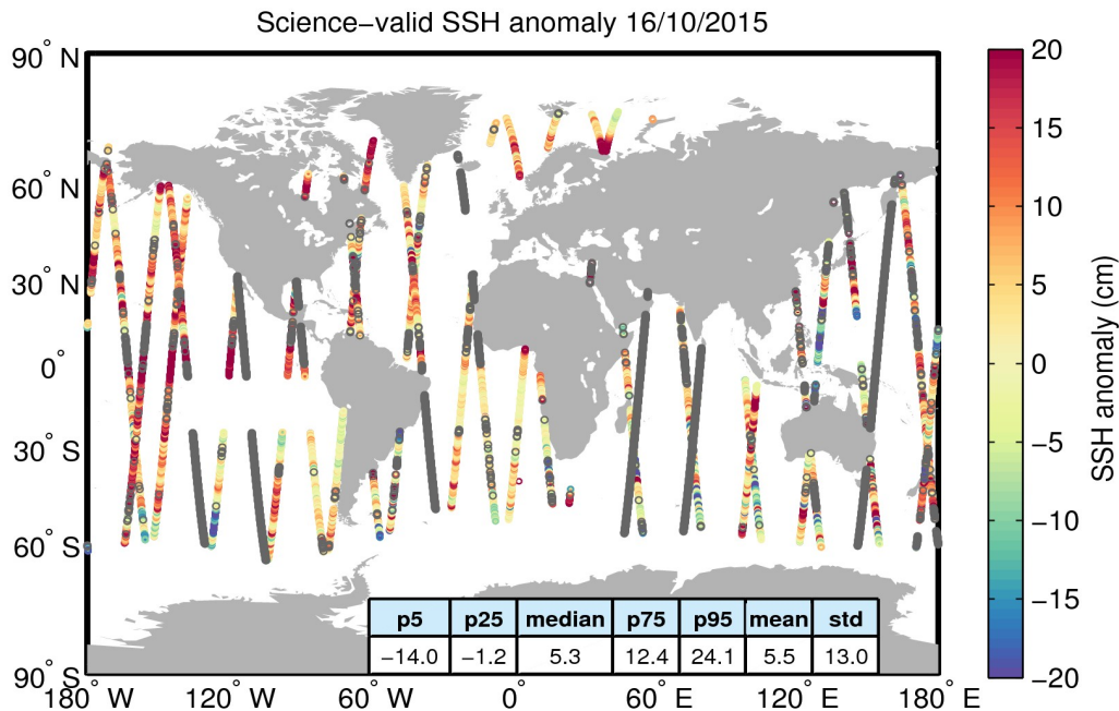
Figure 10. Geographical distribution of science-valid SSH anomaly data over oceans and lakes for 16/10/2015. The statistical values shown in the table refer to the SSH anomaly in cm and are calculated over all measurements shown in the figure. Gray circles denote records that have been rejected based on the editing criteria described in Table 2.
