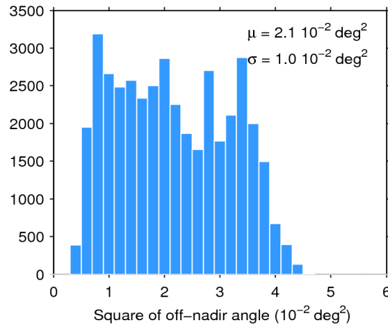
Figure 39. Histogram of flag-valid mispointing over oceans and lakes for 16/10/2015. The mean ( \mu ) and standard deviation ( \sigma ) are also shown. Note that values larger than 6 \cdot 10^{-2} \text{ deg}^2 are excluded from the histogram for the sake of readability but not from the computation of \mu and \sigma .
