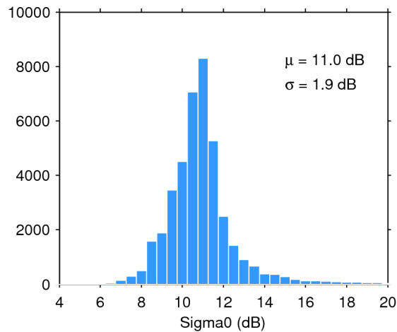
Figure 25. Histogram of flag-valid sigma0 over oceans and lakes for 16/10/2015. The mean ( \mu ) and standard deviation ( \sigma ) are also shown. Note that values outside [4 20] dB are excluded from the histogram for the sake of readability but not from the computation of \mu and \sigma .
