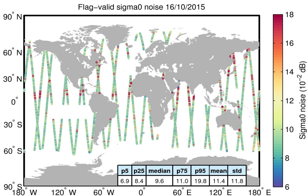
Figure 26. Geographical distribution of flag-valid 20-Hz sigma0 measurement noise over oceans and lakes for 16/10/2015. The statistical values shown in the table refer to the sigma0 noise and are calculated over all measurements shown in the figure.
