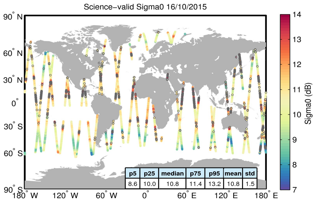
Figure 27. Geographical distribution of science-valid sigma0 data over oceans and lakes for 16/10/2015. The statistical values shown in the table refer to the sigma0 in dB and are calculated over all measurements shown in the figure. Gray circles denote records that have been rejected based on the editing criteria described in Table 4.
