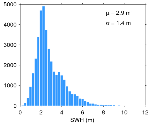
Figure 20. Histogram of science-valid SWH over oceans and lakes for 16/10/2015. The mean ( \mu ) and standard deviation ( \sigma ) are also shown. Note that values larger than 12 m are excluded from the histogram for the sake of readability but not from the computation of \mu and \sigma .
