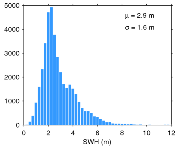
Figure 17. Histogram of flag-valid SWH over oceans and lakes for 16/10/2015. The mean ( \mu ) and standard deviation ( \sigma ) are also shown. Note that values larger than 12 m are excluded from the histogram for the sake of readability but not from the computation of \mu and \sigma .
