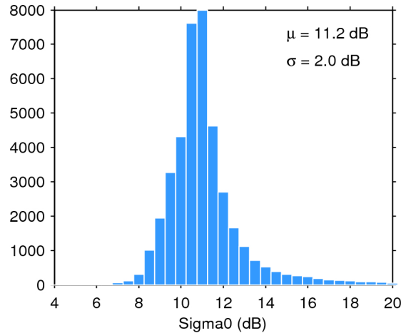
Figure 25. Histogram of flag-valid sigma0 over oceans and lakes for 13/10/2015. The mean ( \mu ) and standard deviation ( \sigma ) are also shown. Note that values outside [4 20] dB are excluded from the histogram for the sake of readability but not from the computation of \mu and \sigma .
