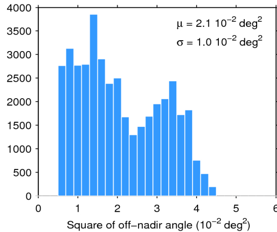
Figure 39. Histogram of flag-valid mispointing over oceans and lakes for 13/10/2015. The mean ( \mu ) and standard deviation ( \sigma ) are also shown. Note that values larger than 6 \cdot 10^{-2} \text{ deg}^2 are excluded from the histogram for the sake of readability but not from the computation of \mu and \sigma .
