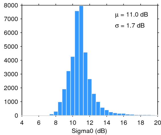
Figure 28. Histogram of science-valid sigma0 over oceans and lakes for 13/10/2015. The mean ( \mu ) and standard deviation ( \sigma ) are also shown. Note that values outside [4 20] dB are excluded from the histogram for the sake of readability but not from the computation of \mu and \sigma .
