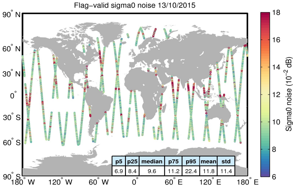
Figure 26. Geographical distribution of flag-valid 20-Hz sigma0 measurement noise over oceans and lakes for 13/10/2015. The statistical values shown in the table refer to the sigma0 noise and are calculated over all measurements shown in the figure.
