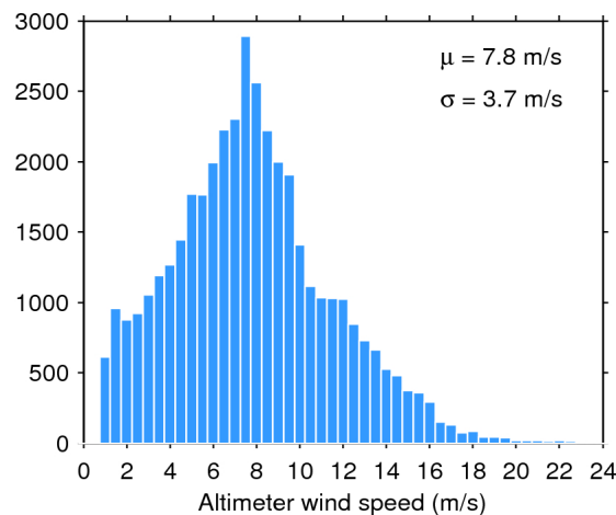
Figure 35. Histogram of science-valid wind over oceans and lakes for 13/10/2015. The mean ( \mu ) and standard deviation ( \sigma ) are also shown. Note that values larger than 24 m/s are excluded from the histogram for the sake of readability but not from the computation of \mu and \sigma .
