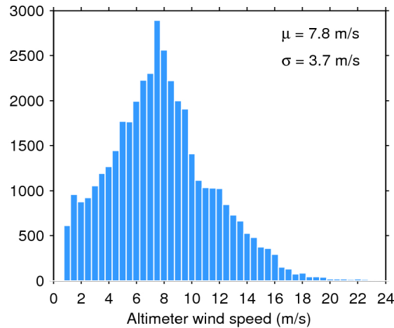
Figure 33. Histogram of flag-valid wind over oceans and lakes for 13/10/2015. The mean ( \mu ) and standard deviation ( \sigma ) are also shown. Note that values larger than 24 m/s are excluded from the histogram for the sake of readability but not from the computation of \mu and \sigma .
