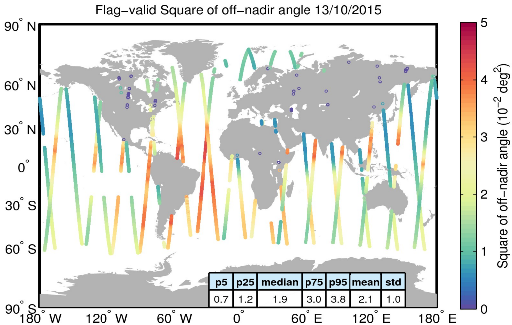
Figure 37. Geographical distribution of flag-valid mispointing data over oceans and lakes for 13/10/2015. The statistical values shown in the table refer to the mispointing in 10^{-2} deg 2 and are calculated over all measurements shown in the figure.
