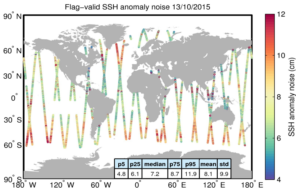
Figure 8. Geographical distribution of flag-valid 20-Hz SSH anomaly measurement noise over oceans and lakes for 13/10/2015. The statistical values shown in the table refer to the SSH anomaly noise and are calculated over all measurements shown in the figure.
