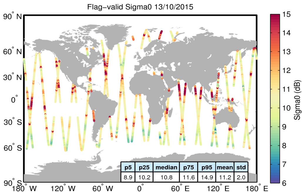
Figure 23. Geographical distribution of flag-valid sigma0 data over oceans and lakes for 13/10/2015. The statistical values shown in the table refer to the sigma0 in dB and are calculated over all measurements shown in the figure.
