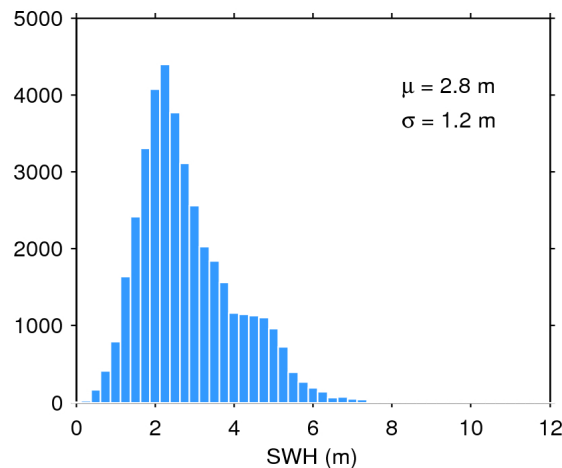
Figure 20. Histogram of science-valid SWH over oceans and lakes for 13/10/2015. The mean ( \mu ) and standard deviation ( \sigma ) are also shown. Note that values larger than 12 m are excluded from the histogram for the sake of readability but not from the computation of \mu and \sigma .
