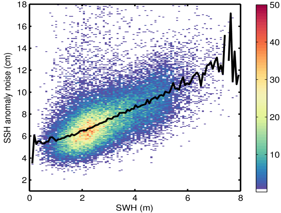
Figure 9. 2D histogram showing flag-valid SSH anomaly noise as a function of SWH for 13/10/2015. The black line denotes the median SSH anomaly noise as a function of SWH.
