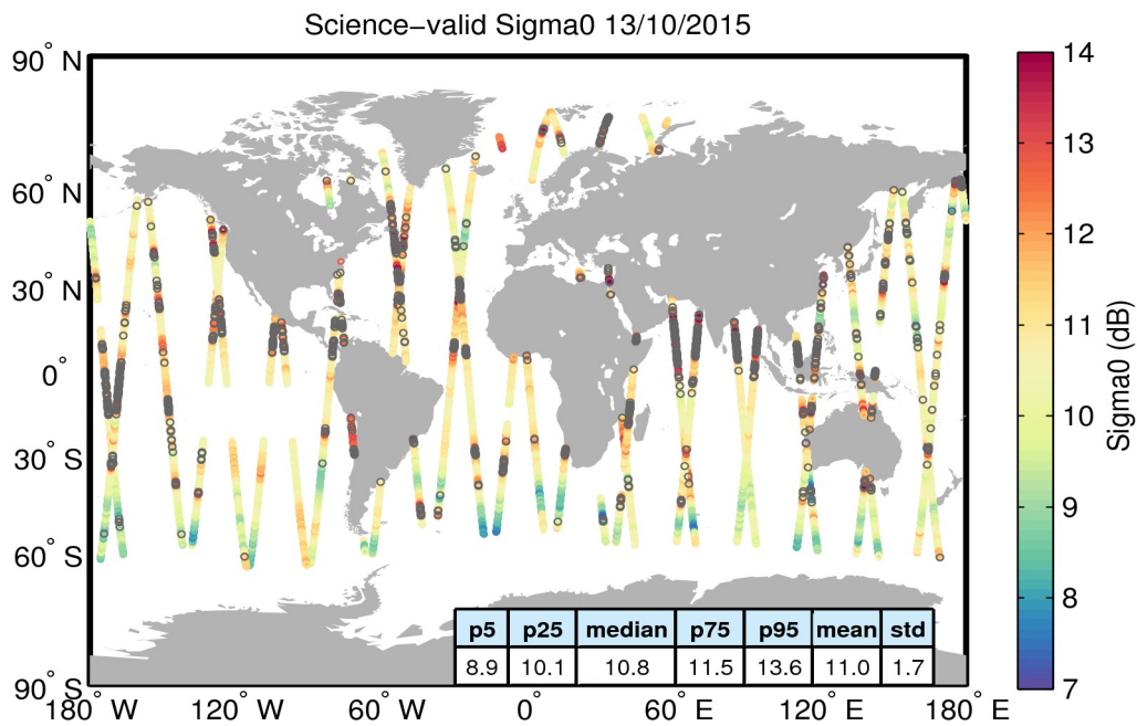
Figure 27. Geographical distribution of science-valid sigma0 data over oceans and lakes for 13/10/2015. The statistical values shown in the table refer to the sigma0 in dB and are calculated over all measurements shown in the figure. Gray circles denote records that have been rejected based on the editing criteria described in Table 4.
