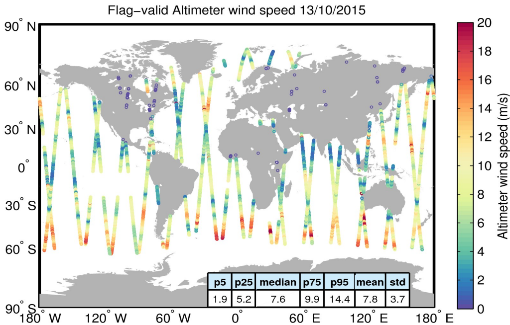
Figure 31. Geographical distribution of flag-valid wind data over oceans and lakes for 13/10/2015. The statistical values shown in the table refer to the wind in m/s and are calculated over all measurements shown in the figure.
