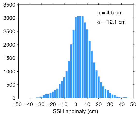
Figure 11. Histogram of science-valid SSH anomaly over oceans and lakes for 13/10/2015. The mean ( \mu ) and standard deviation ( \sigma ) are also shown. Note that values outside [-50 50] cm are excluded from the histogram for the sake of readability but not from the computation of \mu and \sigma .
