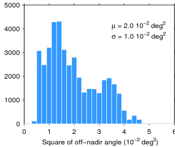
Figure 39. Histogram of flag-valid mispointing over oceans and lakes for 10/10/2015. The mean ( \mu ) and standard deviation ( \sigma ) are also shown. Note that values larger than 6 \cdot 10^{-2} \text{ deg}^2 are excluded from the histogram for the sake of readability but not from the computation of \mu and \sigma .
