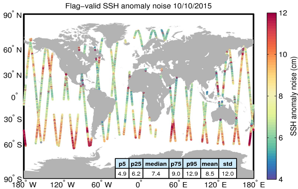
Figure 8. Geographical distribution of flag-valid 20-Hz SSH anomaly measurement noise over oceans and lakes for 10/10/2015. The statistical values shown in the table refer to the SSH anomaly noise and are calculated over all measurements shown in the figure.
