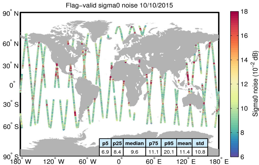
Figure 26. Geographical distribution of flag-valid 20-Hz sigma0 measurement noise over oceans and lakes for 10/10/2015. The statistical values shown in the table refer to the sigma0 noise and are calculated over all measurements shown in the figure.
