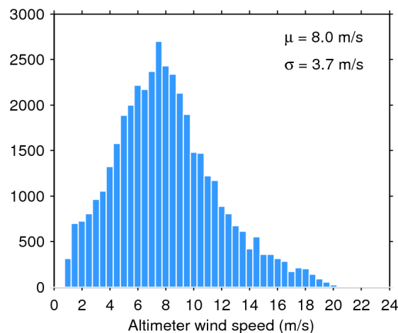
Figure 35. Histogram of science-valid wind over oceans and lakes for 10/10/2015. The mean ( \mu ) and standard deviation ( \sigma ) are also shown. Note that values larger than 24 m/s are excluded from the histogram for the sake of readability but not from the computation of \mu and \sigma .
