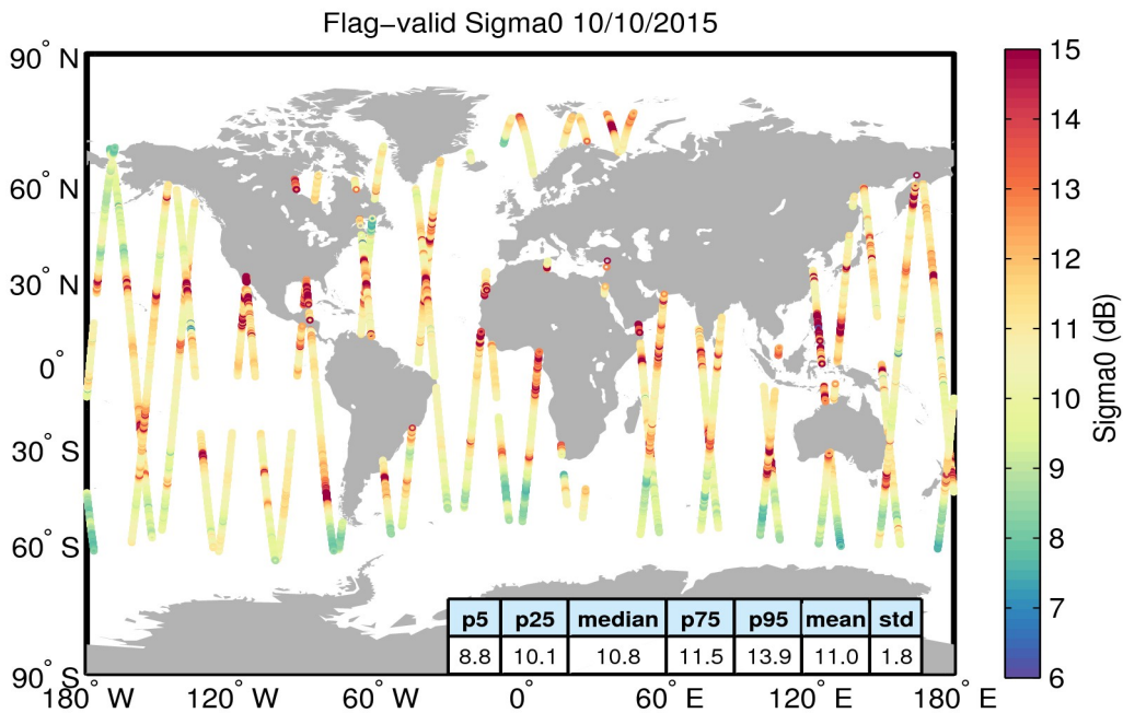
Figure 23. Geographical distribution of flag-valid sigma0 data over oceans and lakes for 10/10/2015. The statistical values shown in the table refer to the sigma0 in dB and are calculated over all measurements shown in the figure.
