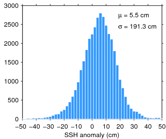
Figure 7. Histogram of flag-valid SSH anomaly over oceans and lakes for 10/10/2015. The mean ( \mu ) and standard deviation ( \sigma ) are also shown. Note that values outside [-50\ 50] cm are excluded from the histogram for the sake of readability but not from the computation of \mu and \sigma .
