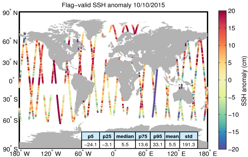
Figure 5. Geographical distribution of flag-valid 1-Hz SSH anomaly data over oceans and lakes for 10/10/2015. The statistical values shown in the table refer to the SSH anomaly in cm and are calculated over all measurements shown in the figure.
