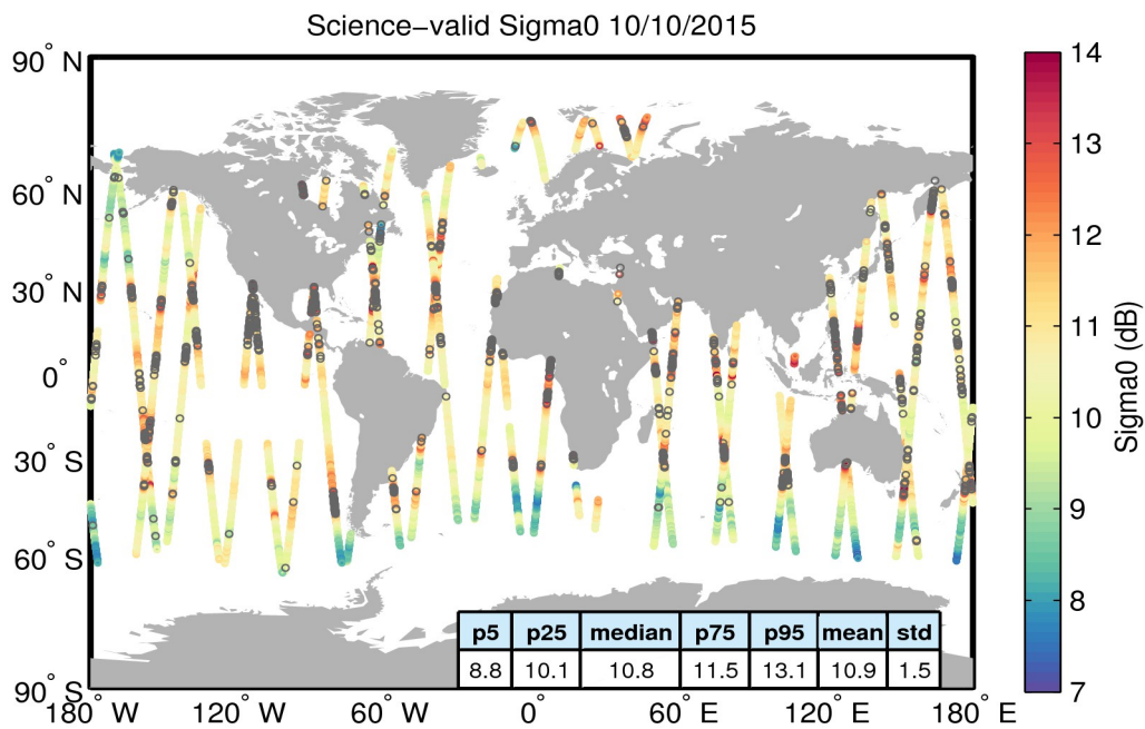
Figure 27. Geographical distribution of science-valid sigma0 data over oceans and lakes for 10/10/2015. The statistical values shown in the table refer to the sigma0 in dB and are calculated over all measurements shown in the figure. Gray circles denote records that have been rejected based on the editing criteria described in Table 4.
