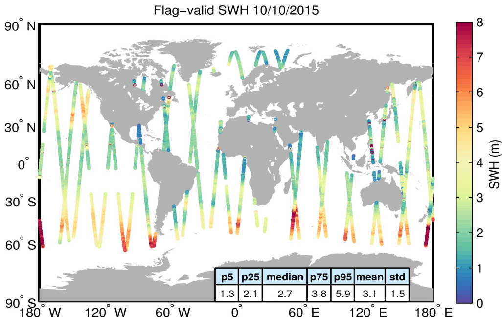
Figure 15. Geographical distribution of flag-valid SWH data over oceans and lakes for 10/10/2015. The statistical values shown in the table refer to the SWH in m and are calculated over all measurements shown in the figure.
