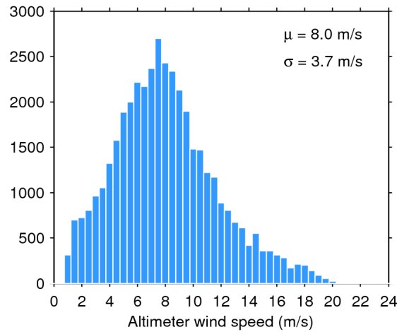
Figure 33. Histogram of flag-valid wind over oceans and lakes for 10/10/2015. The mean ( \mu ) and standard deviation ( \sigma ) are also shown. Note that values larger than 24 m/s are excluded from the histogram for the sake of readability but not from the computation of \mu and \sigma .
