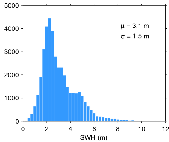
Figure 17. Histogram of flag-valid SWH over oceans and lakes for 10/10/2015. The mean ( \mu ) and standard deviation ( \sigma ) are also shown. Note that values larger than 12 m are excluded from the histogram for the sake of readability but not from the computation of \mu and \sigma .
