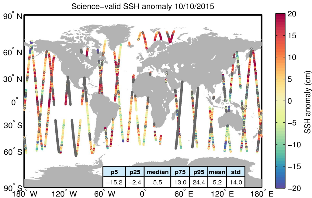
Figure 10. Geographical distribution of science-valid SSH anomaly data over oceans and lakes for 10/10/2015. The statistical values shown in the table refer to the SSH anomaly in cm and are calculated over all measurements shown in the figure. Gray circles denote records that have been rejected based on the editing criteria described in Table 2.
