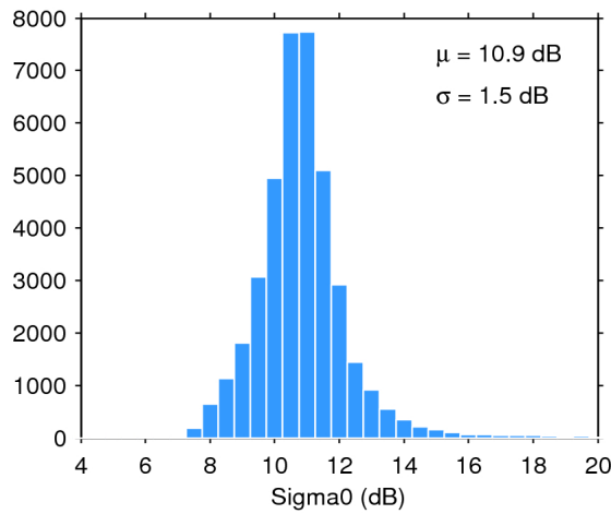
Figure 28. Histogram of science-valid sigma0 over oceans and lakes for 10/10/2015. The mean ( \mu ) and standard deviation ( \sigma ) are also shown. Note that values outside [4 20] dB are excluded from the histogram for the sake of readability but not from the computation of \mu and \sigma .
