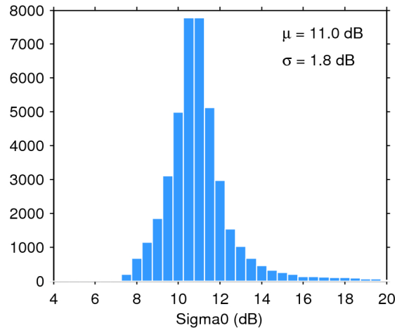
Figure 25. Histogram of flag-valid sigma0 over oceans and lakes for 10/10/2015. The mean ( \mu ) and standard deviation ( \sigma ) are also shown. Note that values outside [4 20] dB are excluded from the histogram for the sake of readability but not from the computation of \mu and \sigma .
