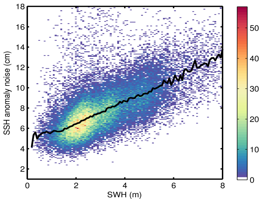
Figure 9. 2D histogram showing flag-valid SSH anomaly noise as a function of SWH for 10/10/2015. The black line denotes the median SSH anomaly noise as a function of SWH.
