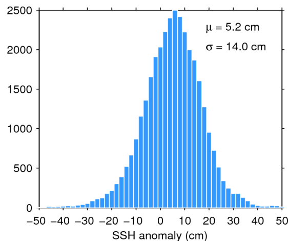
Figure 11. Histogram of science-valid SSH anomaly over oceans and lakes for 10/10/2015. The mean ( \mu ) and standard deviation ( \sigma ) are also shown. Note that values outside [-50 50] cm are excluded from the histogram for the sake of readability but not from the computation of \mu and \sigma .
