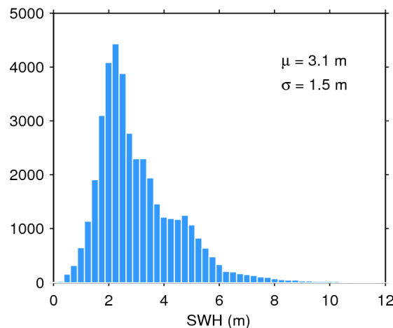
Figure 20. Histogram of science-valid SWH over oceans and lakes for 10/10/2015. The mean ( \mu ) and standard deviation ( \sigma ) are also shown. Note that values larger than 12 m are excluded from the histogram for the sake of readability but not from the computation of \mu and \sigma .
