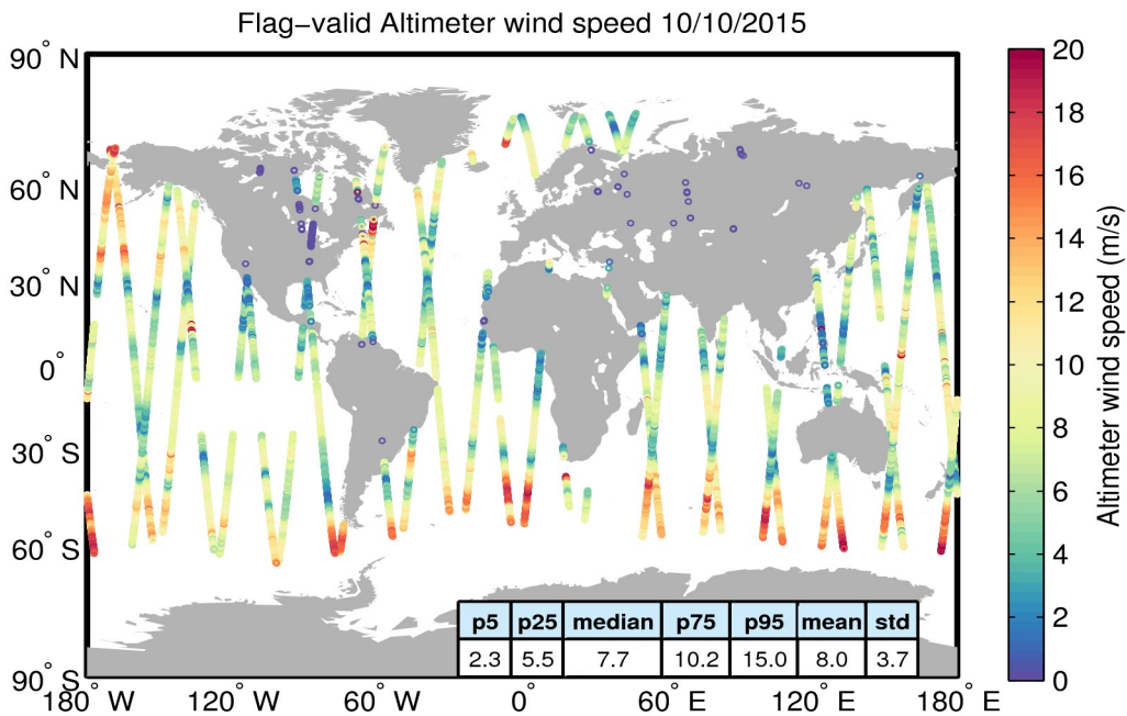
Figure 31. Geographical distribution of flag-valid wind data over oceans and lakes for 10/10/2015. The statistical values shown in the table refer to the wind in m/s and are calculated over all measurements shown in the figure.
