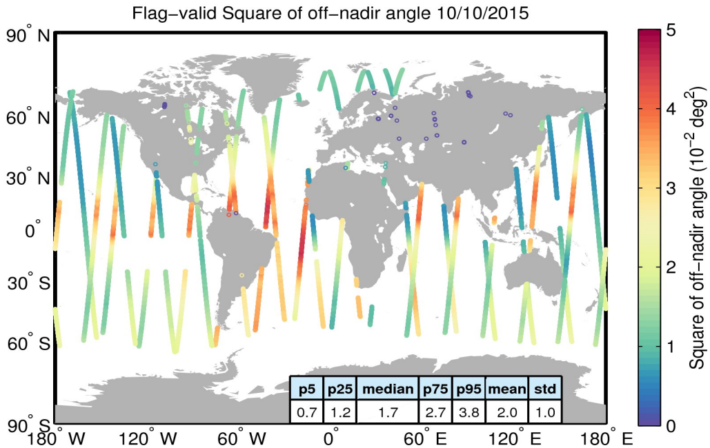
Figure 37. Geographical distribution of flag-valid mispointing data over oceans and lakes for 10/10/2015. The statistical values shown in the table refer to the mispointing in 10^{-2} \text{ deg}^2 and are calculated over all measurements shown in the figure.
