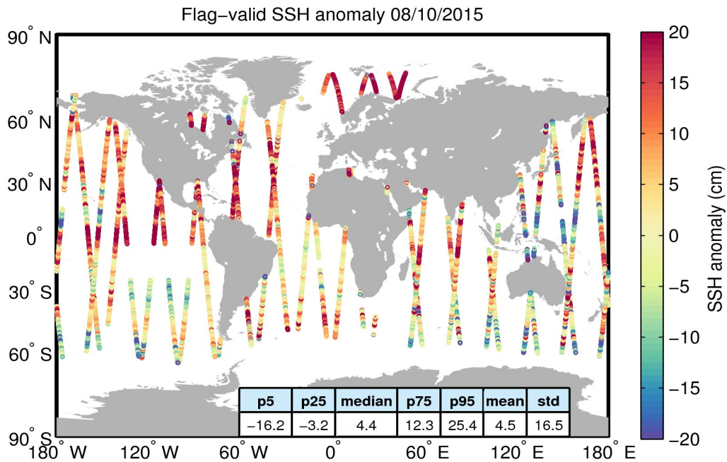
Figure 5. Geographical distribution of flag-valid 1-Hz SSH anomaly data over oceans and lakes for 08/10/2015. The statistical values shown in the table refer to the SSH anomaly in cm and are calculated over all measurements shown in the figure.
