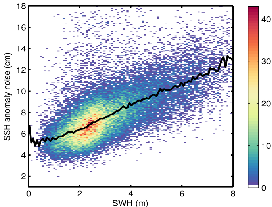
Figure 9. 2D histogram showing flag-valid SSH anomaly noise as a function of SWH for 08/10/2015. The black line denotes the median SSH anomaly noise as a function of SWH.
