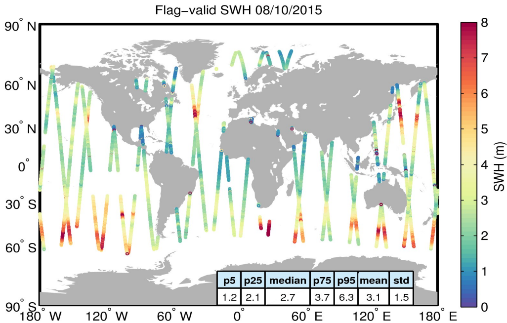
Figure 15. Geographical distribution of flag-valid SWH data over oceans and lakes for 08/10/2015. The statistical values shown in the table refer to the SWH in m and are calculated over all measurements shown in the figure.
