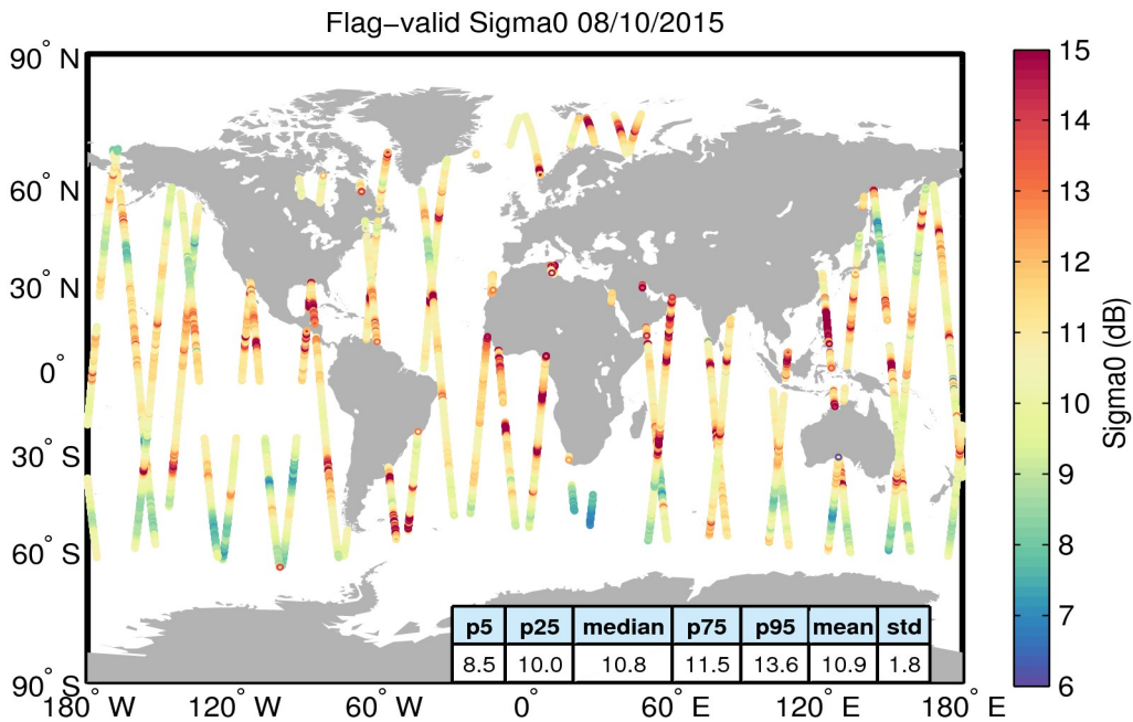
Figure 23. Geographical distribution of flag-valid sigma0 data over oceans and lakes for 08/10/2015. The statistical values shown in the table refer to the sigma0 in dB and are calculated over all measurements shown in the figure.
