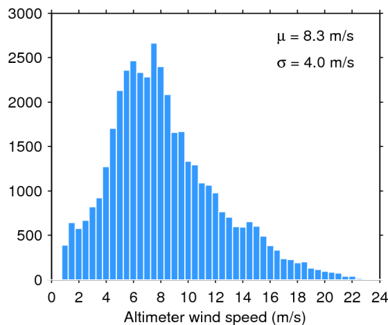
Figure 35. Histogram of science-valid wind over oceans and lakes for 08/10/2015. The mean ( \mu ) and standard deviation ( \sigma ) are also shown. Note that values larger than 24 m/s are excluded from the histogram for the sake of readability but not from the computation of \mu and \sigma .
