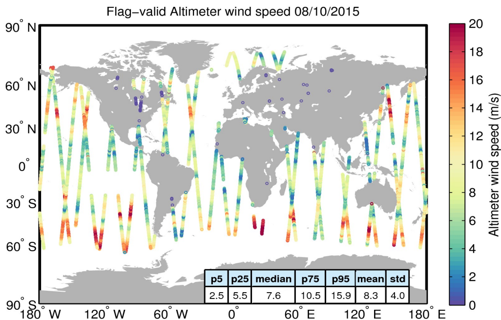
Figure 31. Geographical distribution of flag-valid wind data over oceans and lakes for 08/10/2015. The statistical values shown in the table refer to the wind in m/s and are calculated over all measurements shown in the figure.
