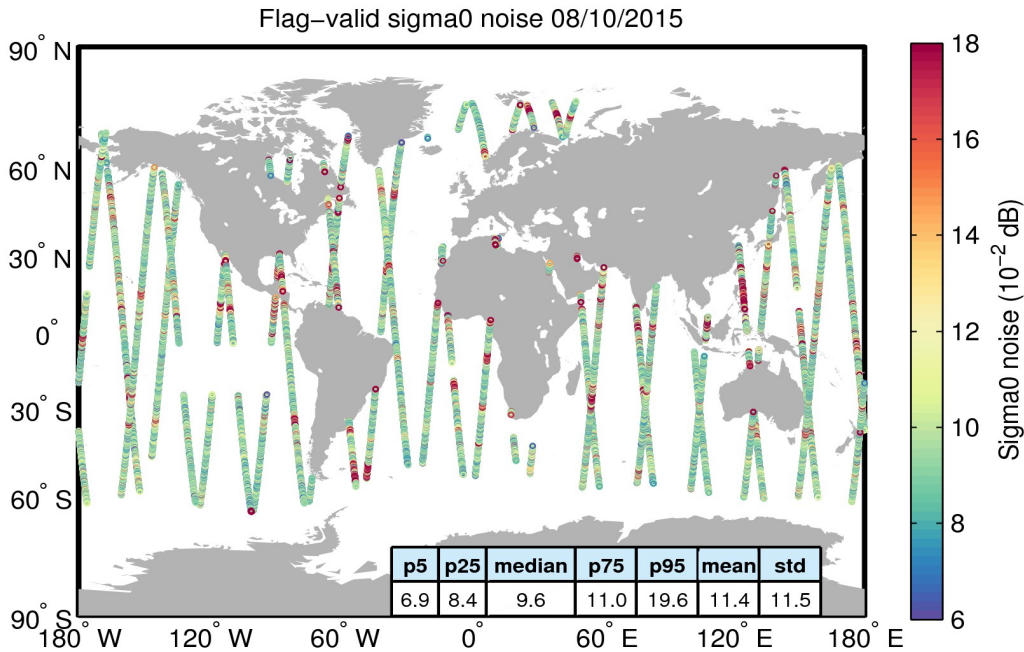
Figure 26. Geographical distribution of flag-valid 20-Hz sigma0 measurement noise over oceans and lakes for 08/10/2015. The statistical values shown in the table refer to the sigma0 noise and are calculated over all measurements shown in the figure.
