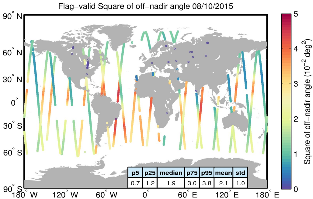
Figure 37. Geographical distribution of flag-valid mispointing data over oceans and lakes for 08/10/2015. The statistical values shown in the table refer to the mispointing in 10^{-2} \text{ deg}^2 and are calculated over all measurements shown in the figure.
