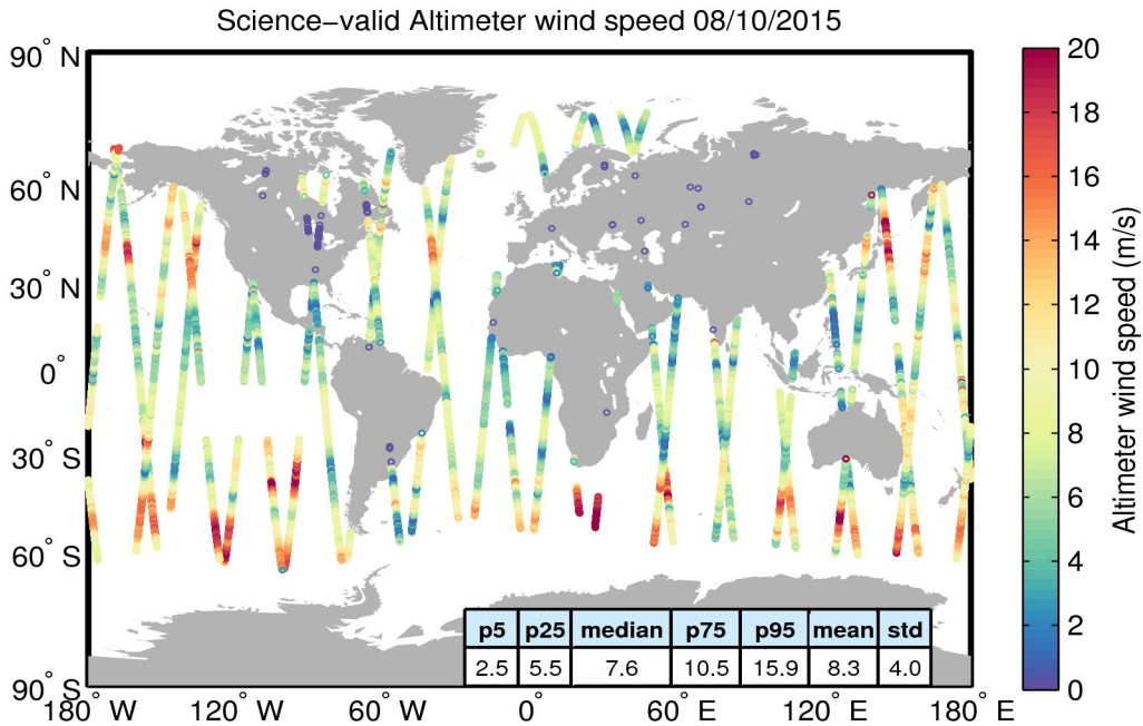
Figure 34. Geographical distribution of science-valid wind data over oceans and lakes for 08/10/2015. The statistical values shown in the table refer to the wind in m/s and are calculated over all measurements shown in the figure. Gray circles denote records that have been rejected based on the editing criteria described in Table 5.
