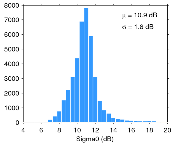
Figure 25. Histogram of flag-valid sigma0 over oceans and lakes for 08/10/2015. The mean ( \mu ) and standard deviation ( \sigma ) are also shown. Note that values outside [4 20] dB are excluded from the histogram for the sake of readability but not from the computation of \mu and \sigma .
