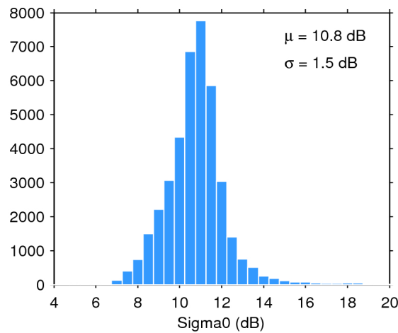
Figure 28. Histogram of science-valid sigma0 over oceans and lakes for 08/10/2015. The mean ( \mu ) and standard deviation ( \sigma ) are also shown. Note that values outside [4 20] dB are excluded from the histogram for the sake of readability but not from the computation of \mu and \sigma .
