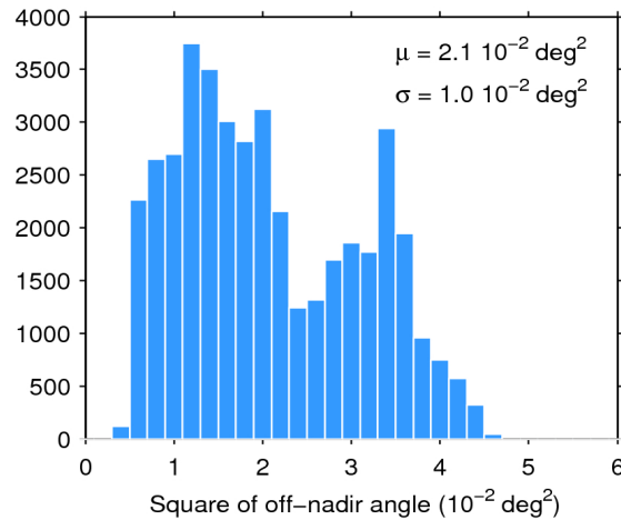
Figure 39. Histogram of flag-valid mispointing over oceans and lakes for 08/10/2015. The mean ( \mu ) and standard deviation ( \sigma ) are also shown. Note that values larger than 6 \cdot 10^{-2} \text{ deg}^2 are excluded from the histogram for the sake of readability but not from the computation of \mu and \sigma .
