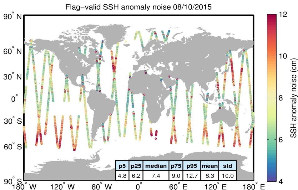
Figure 8. Geographical distribution of flag-valid 20-Hz SSH anomaly measurement noise over oceans and lakes for 08/10/2015. The statistical values shown in the table refer to the SSH anomaly noise and are calculated over all measurements shown in the figure.
