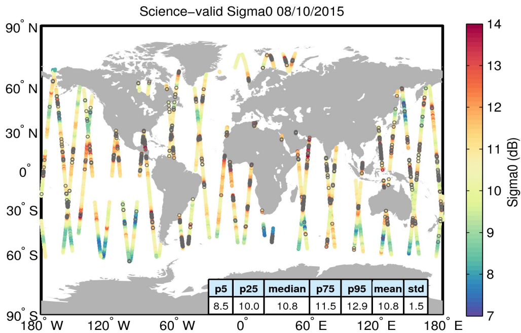
Figure 27. Geographical distribution of science-valid sigma0 data over oceans and lakes for 08/10/2015. The statistical values shown in the table refer to the sigma0 in dB and are calculated over all measurements shown in the figure. Gray circles denote records that have been rejected based on the editing criteria described in Table 4.
