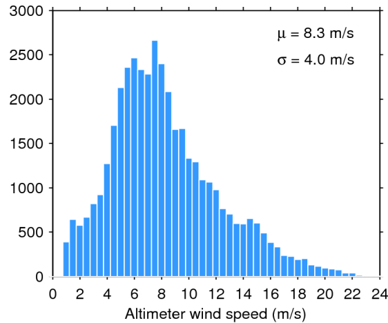
Figure 33. Histogram of flag-valid wind over oceans and lakes for 08/10/2015. The mean ( \mu ) and standard deviation ( \sigma ) are also shown. Note that values larger than 24 m/s are excluded from the histogram for the sake of readability but not from the computation of \mu and \sigma .
